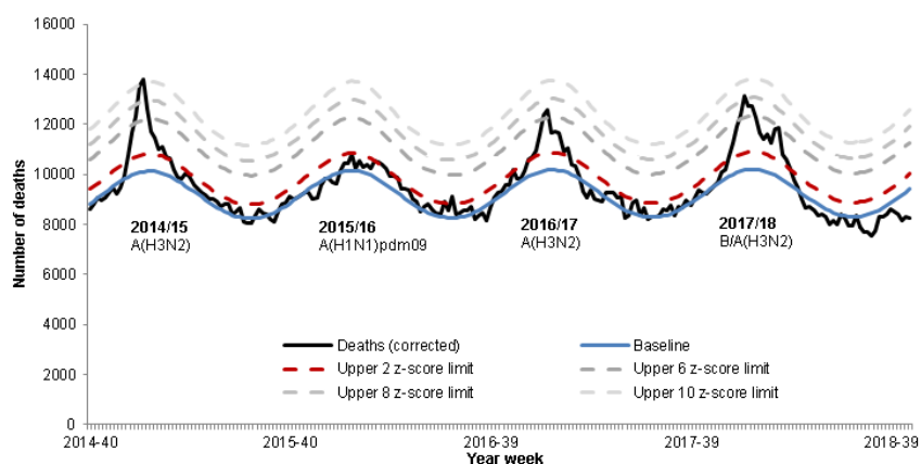
Figure 1: Weekly observed and expected number of all-cause deaths in all ages, with the dominant circulating influenza A subtype, England, 2014 to week 44 2018
