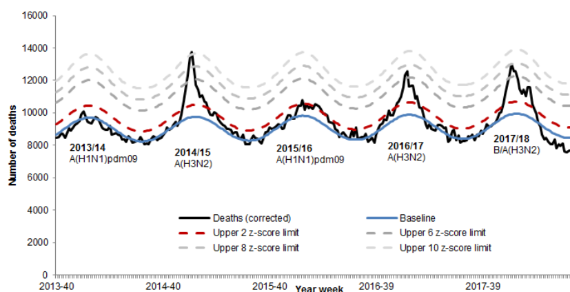
Figure 1: Weekly observed and expected number of all-cause deaths in all ages, with the dominant circulating influenza A subtype, England, 2013 to week 30 2018
