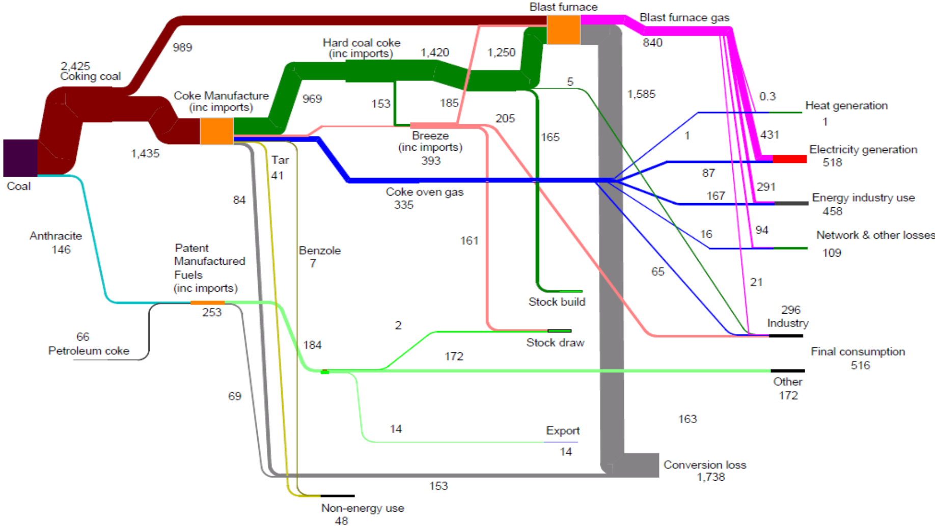
Chart H.6: Manufactured Solid Fuels flow chart 2017 (thousand tonnes of oil equivalent)
