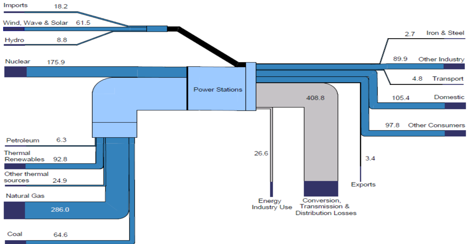
Chart H.4: Electricity flow chart 2017 (TWh)
