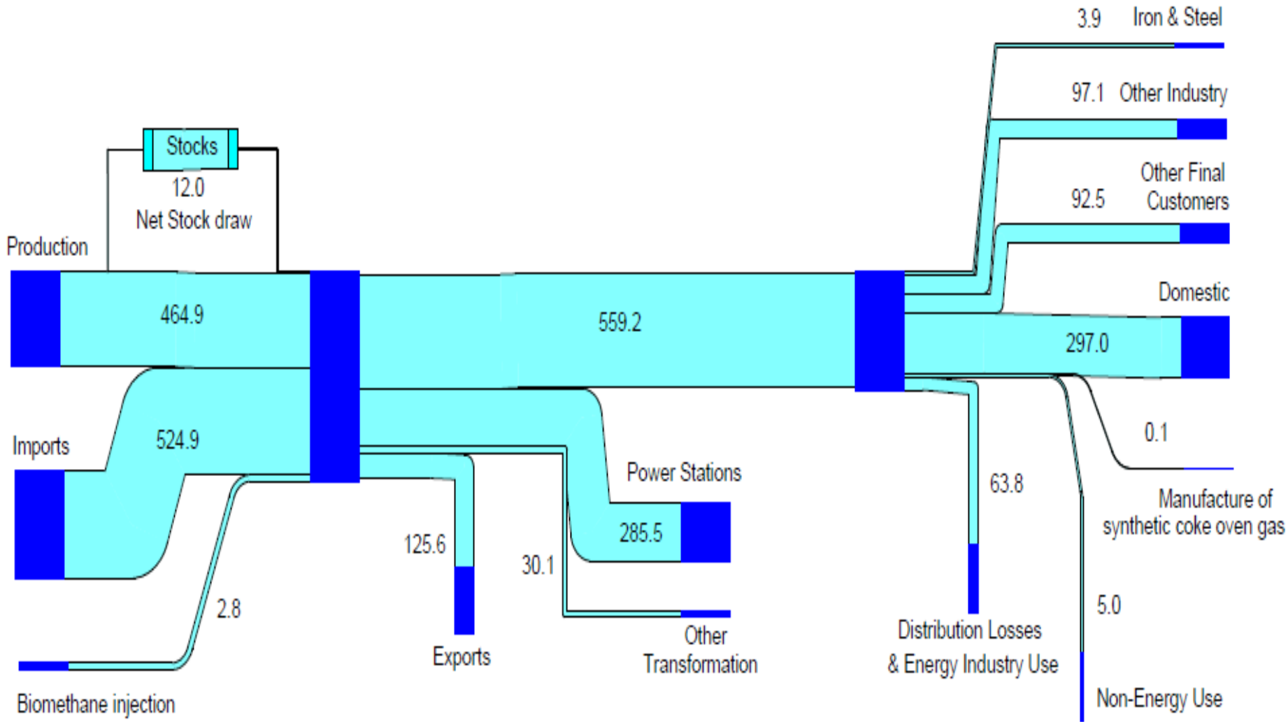
Chart H.3: Natural gas flow chart 2017 (TWh)
