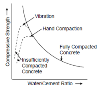
Figure 1b: ...but insufficiently compacted dry concrete is much weaker than fully compacted wetter concrete
