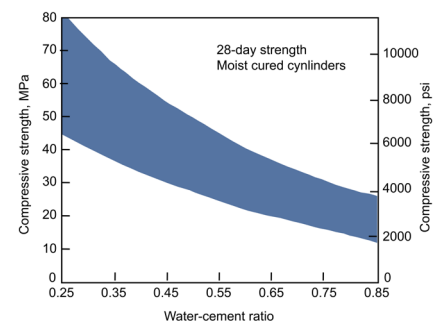
Figure 1a: Concrete is stronger when poured with a lower water-cement ratio
