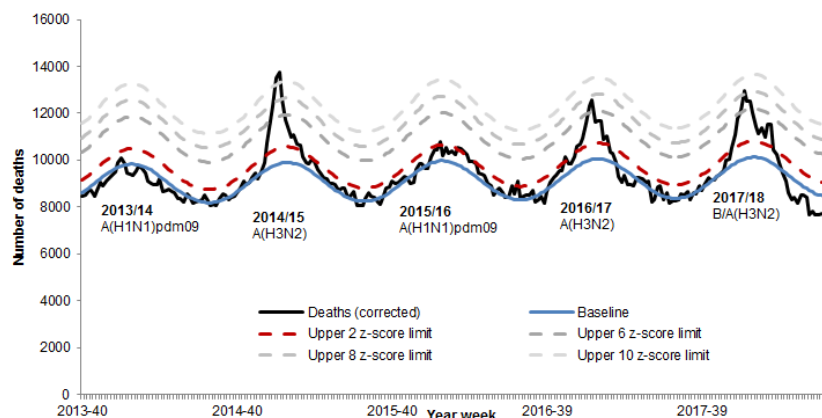
Figure 1: Weekly observed and expected number of all-cause deaths in all ages, with the dominant circulating influenza A subtype, England, 2013 to week 28 2018
