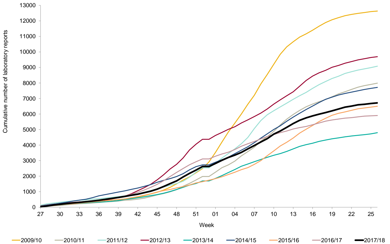
Figure 3: Cumulative number of laboratory reports of norovirus by season 2009/10-2017/18 (England and Wales)
