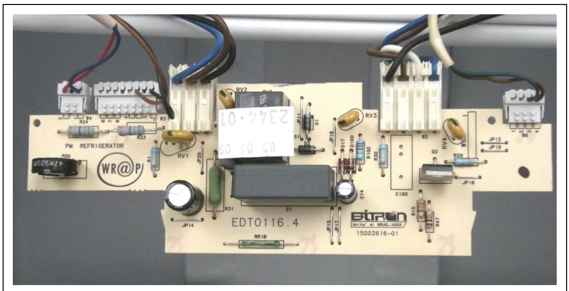
Control PCB
