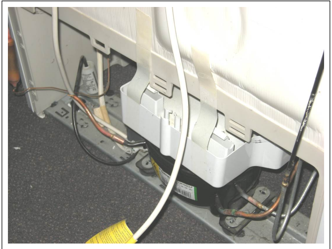
Rear lower section, showing water tray (defrost) above the compressor
