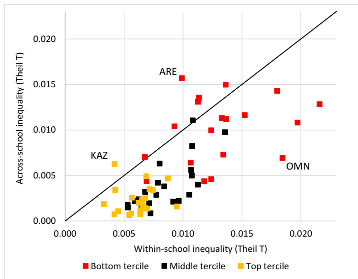
Figure 22: Within- and between-school inequality using TIMSS IRT scores
