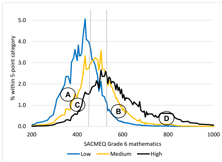
Figure 7: Distribution of SACMEQ cognitive skills using IRT scores
