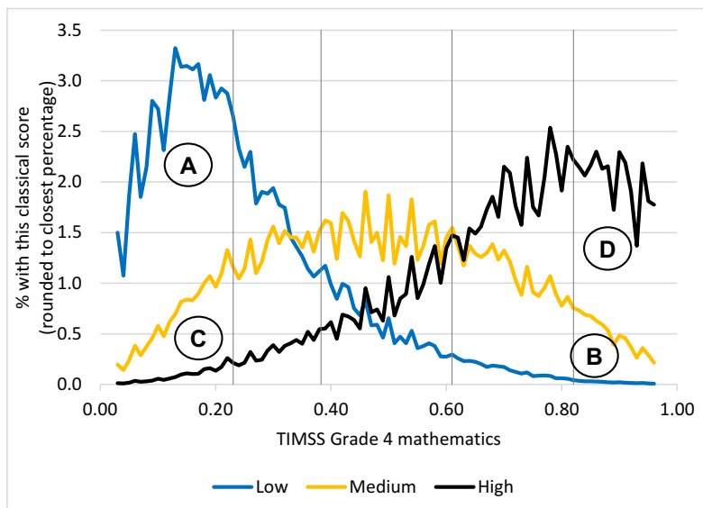
Figure 6: Distribution of TIMSS cognitive skills using classical scores
