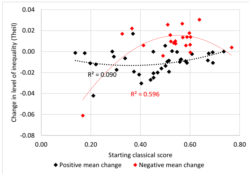
Figure 15: Changes in measures of inequality (TIMSS classical)
