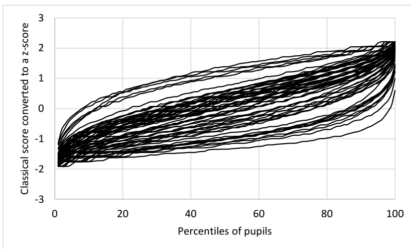
Figure 20: Country distributions of TIMSS classical scores converted to z-scores
