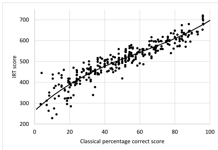
Figure 3: Classical and IRT scores in 2015 TIMSS Grade 4 mathematics
