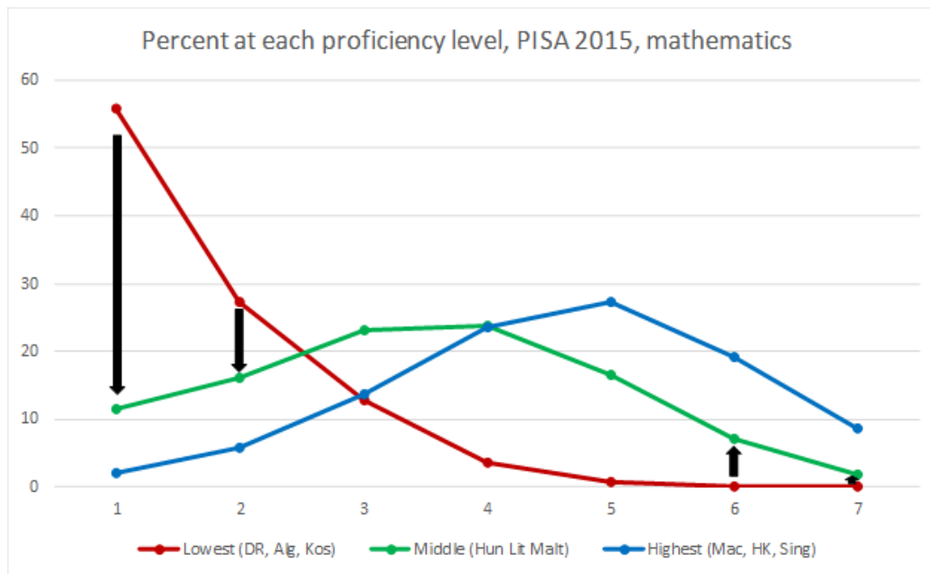
Figure 2. "Histograms" of PISA 2015 mathematics results
