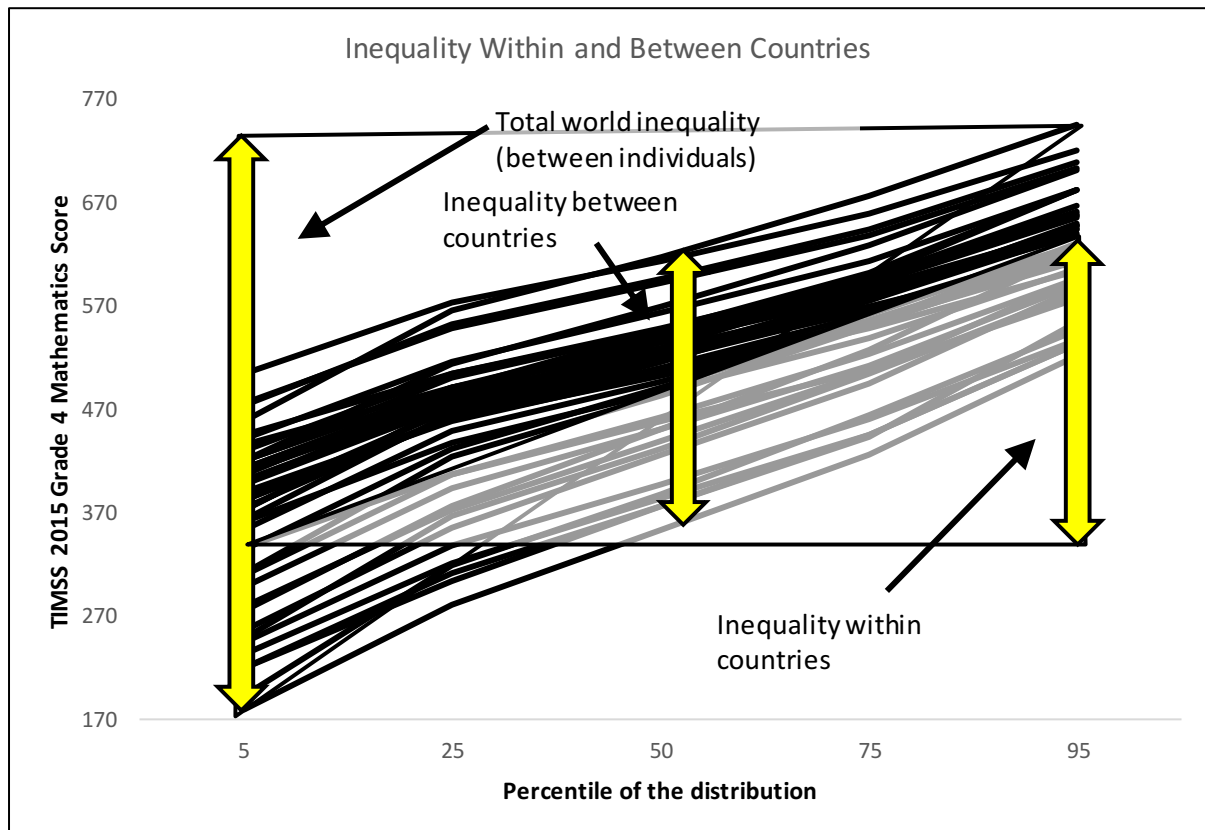
Figure 21. TIMSS 2015 Grade 4 mathematics approximation to between- and within-country inequality
