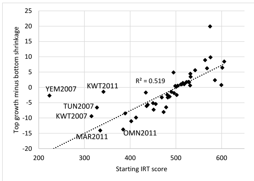
Figure 9: TIMSS shrinkage at the bottom versus growth at the top
