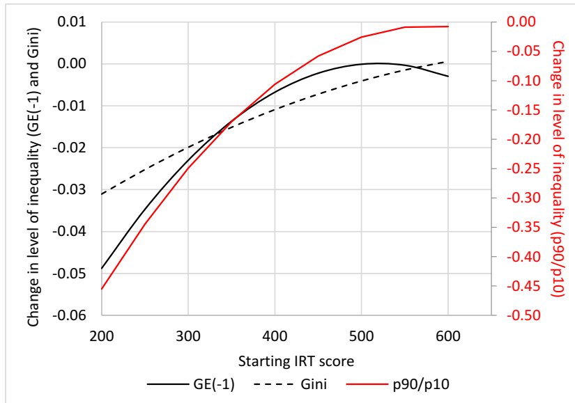
Figure 13: Changes in measures of inequality (TIMSS II)
