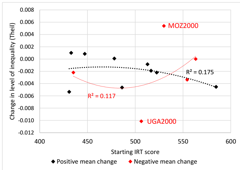
Figure 14: Changes in measures of inequality (SACMEQ)
