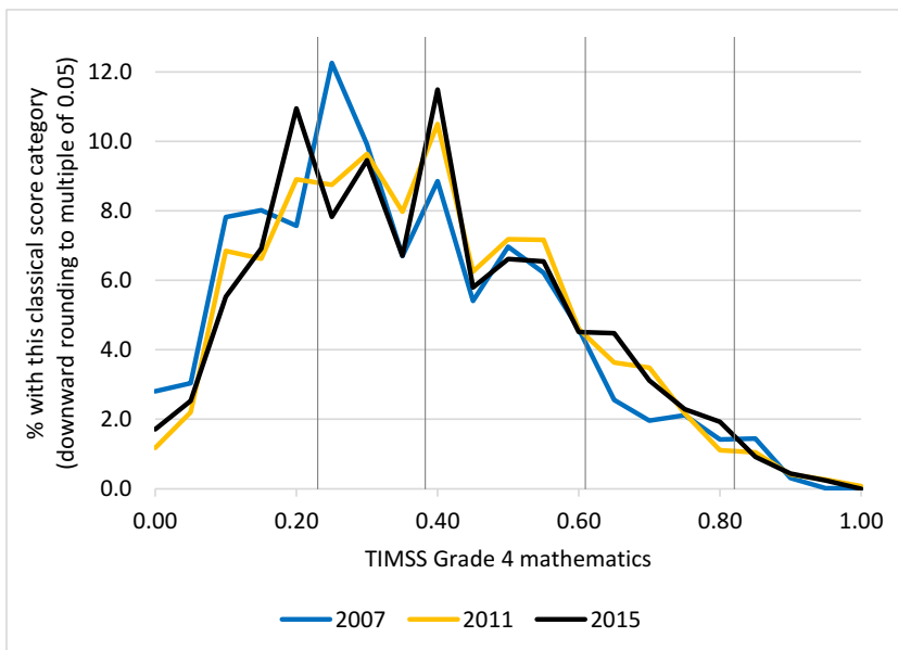
Figure 17: Classical score distribution in Georgia over time
