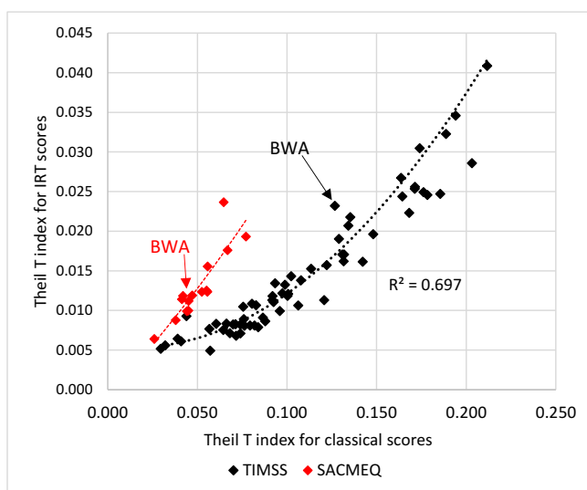
Figure 11: Classical versus IRT scores and measures of inequality
