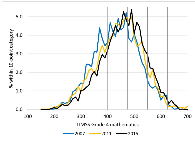
Figure 16: IRT score distribution in Georgia over time
