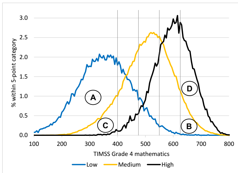
Figure 5: Distribution of TIMSS cognitive skills using IRT scores
