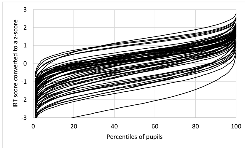
Figure 19: Country distributions of TIMSS IRT scores converted to z-scores
