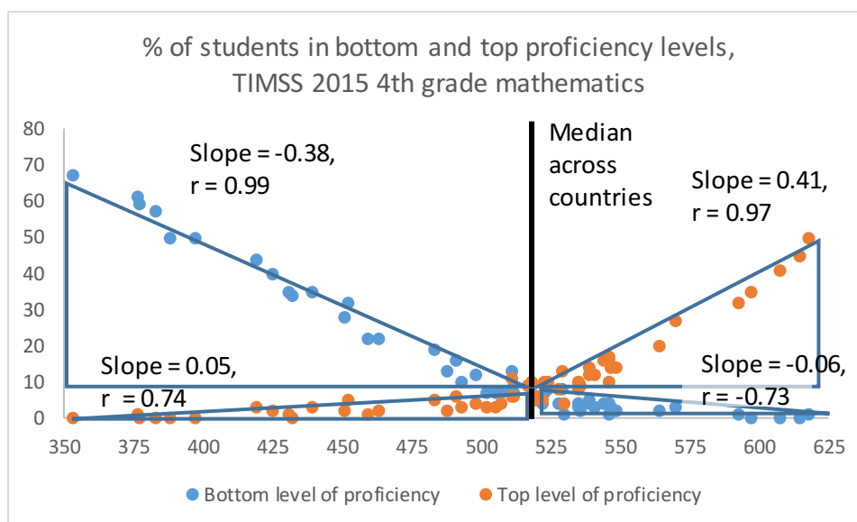
Figure 1. Relationship between mean performance and percentage of students at two key benchmarks
