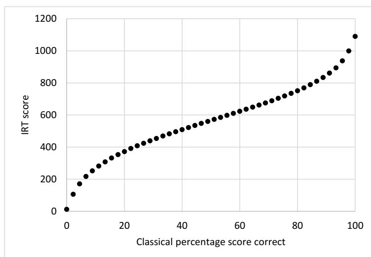
Figure 4: Classical and IRT scores in 2007 SACMEQ Grade 6 mathematics
