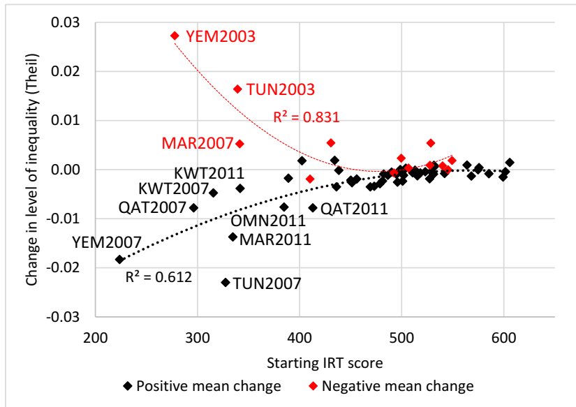
Figure 12: Changes in measures of inequality (TIMSS I)
