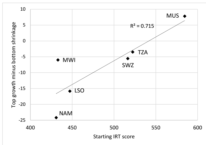
Figure 10: SACMEQ shrinkage at the bottom versus growth at the top
