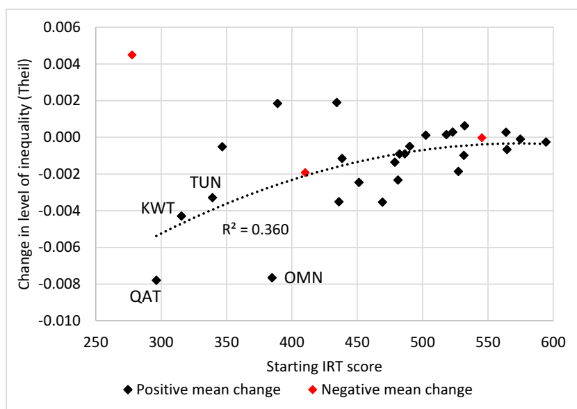
Figure 18: Changes in measures of inequality (TIMSS III)
