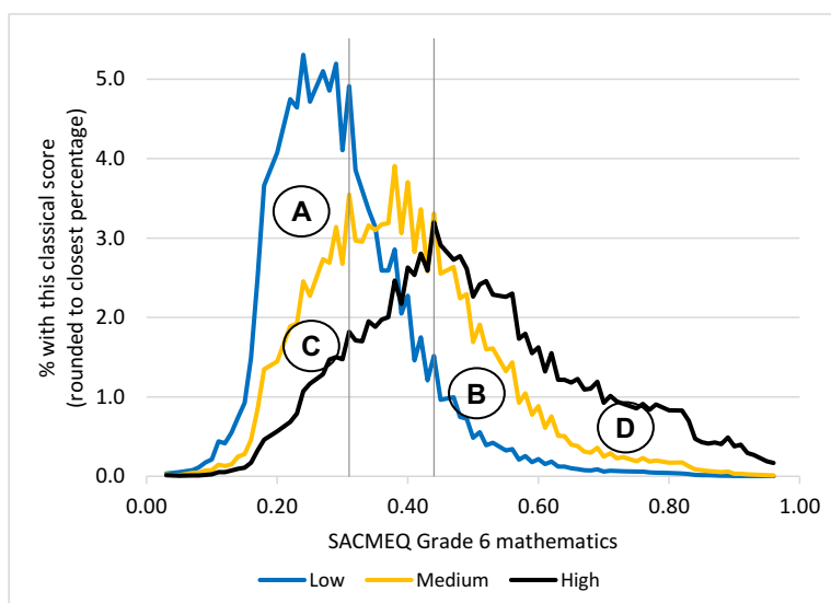
Figure 8: Distribution of SACMEQ cognitive skills using classical scores
