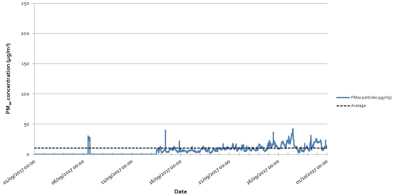
Figure 5 – Construction dust 15-minute mean indicative PM 10 concentration for monitor AQ001. (Periods of 0 \mu\text{g}/\text{m}^3 PM 10 represent power outages)
