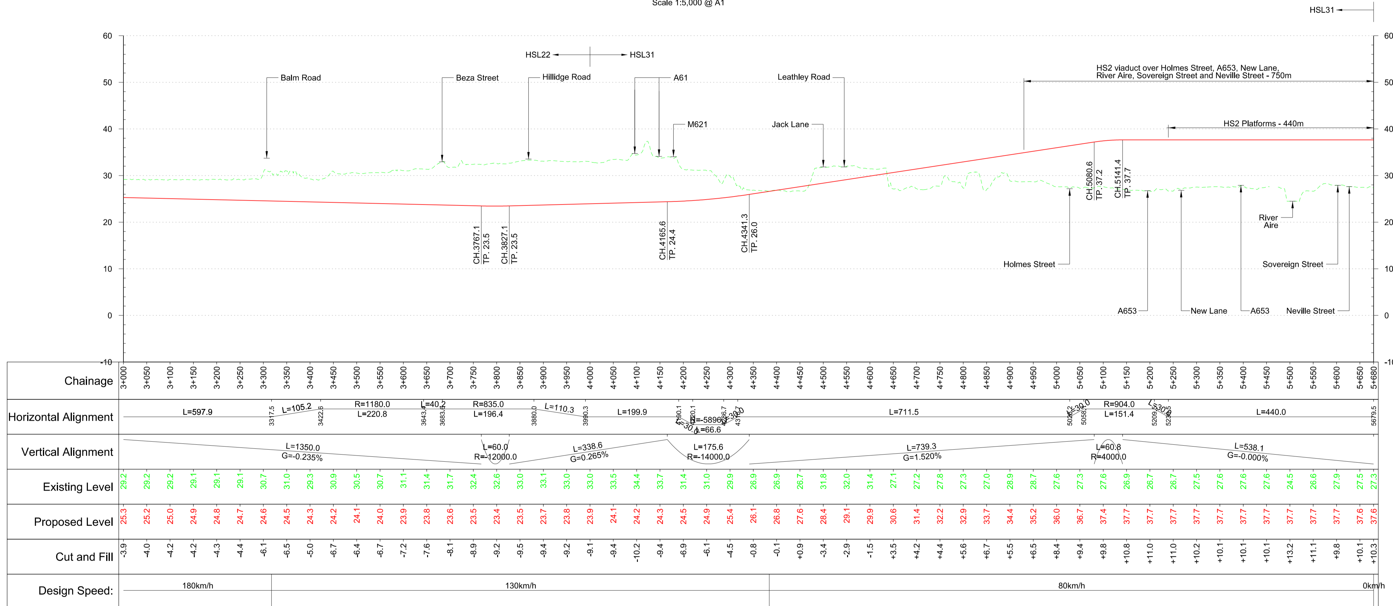
Profile Scale H:1:5,000 V:1:500 @ A1
