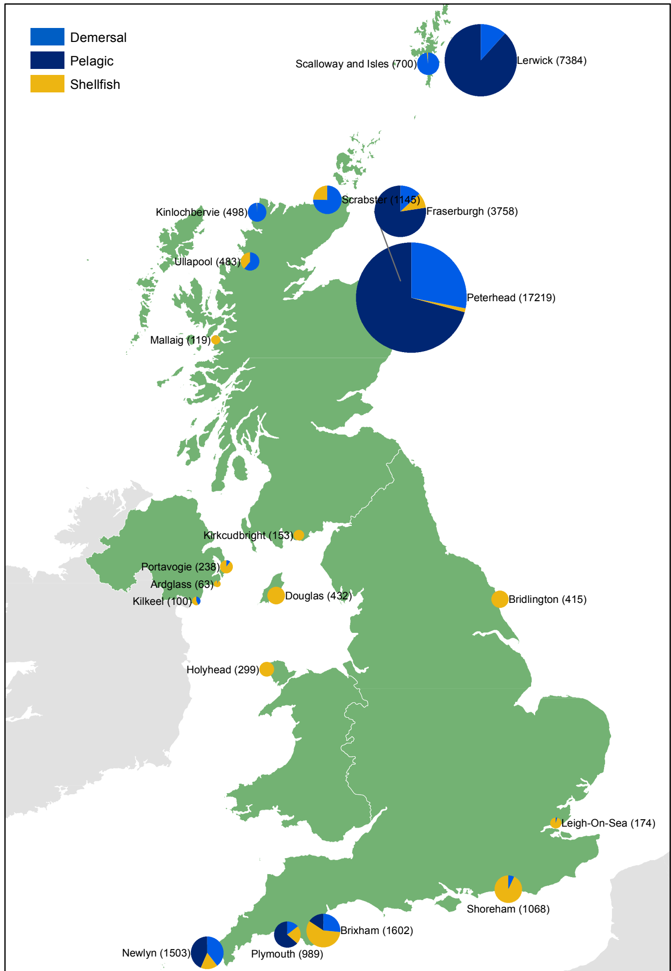
Chart 1: Landings into the top 20 UK ports (a) by UK vessels by species type: October 2016 (tonnes)
