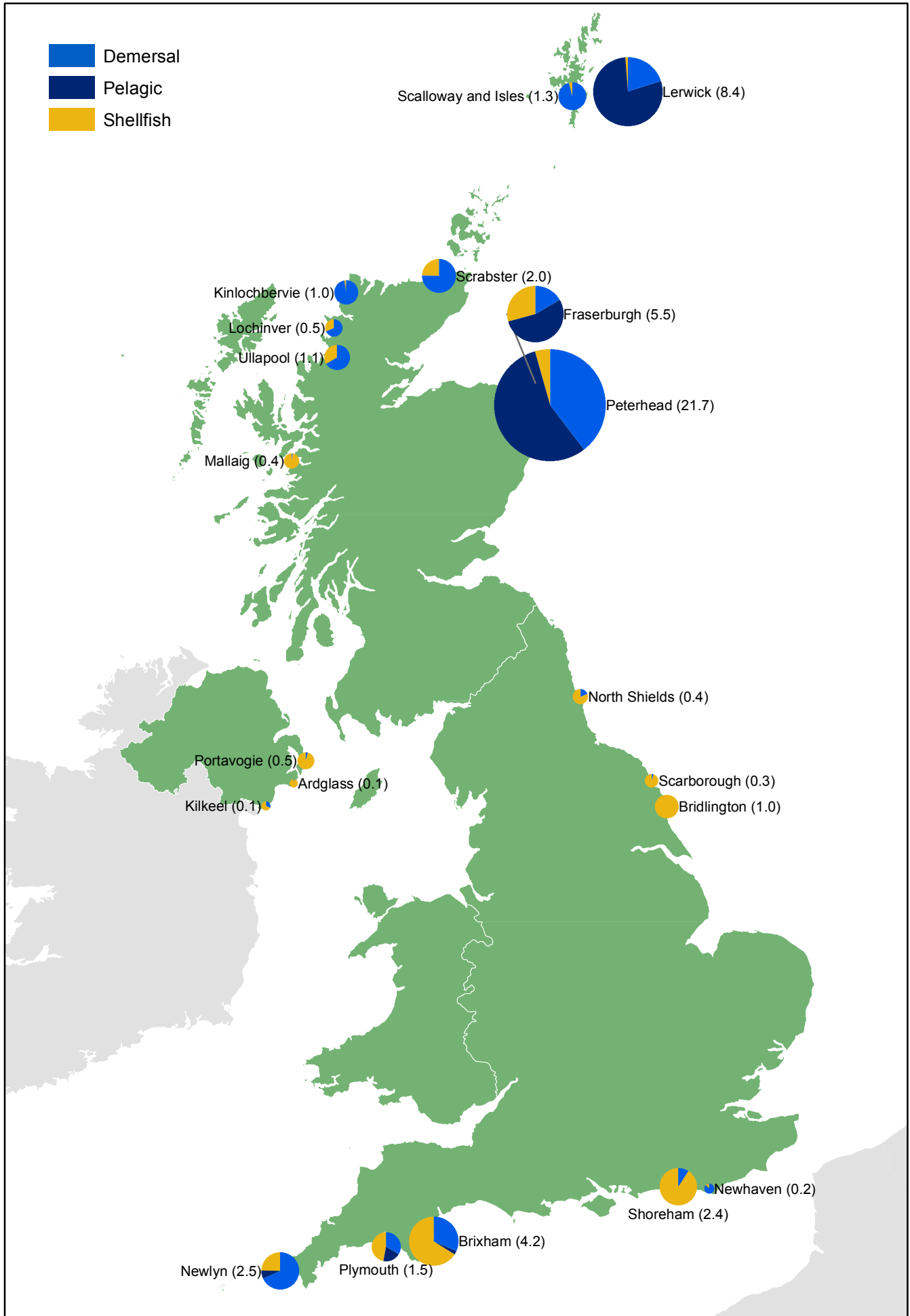
Chart 2: Value of landings into the top 20 UK ports (a) by UK vessels by species type: October 2016 (£million)
