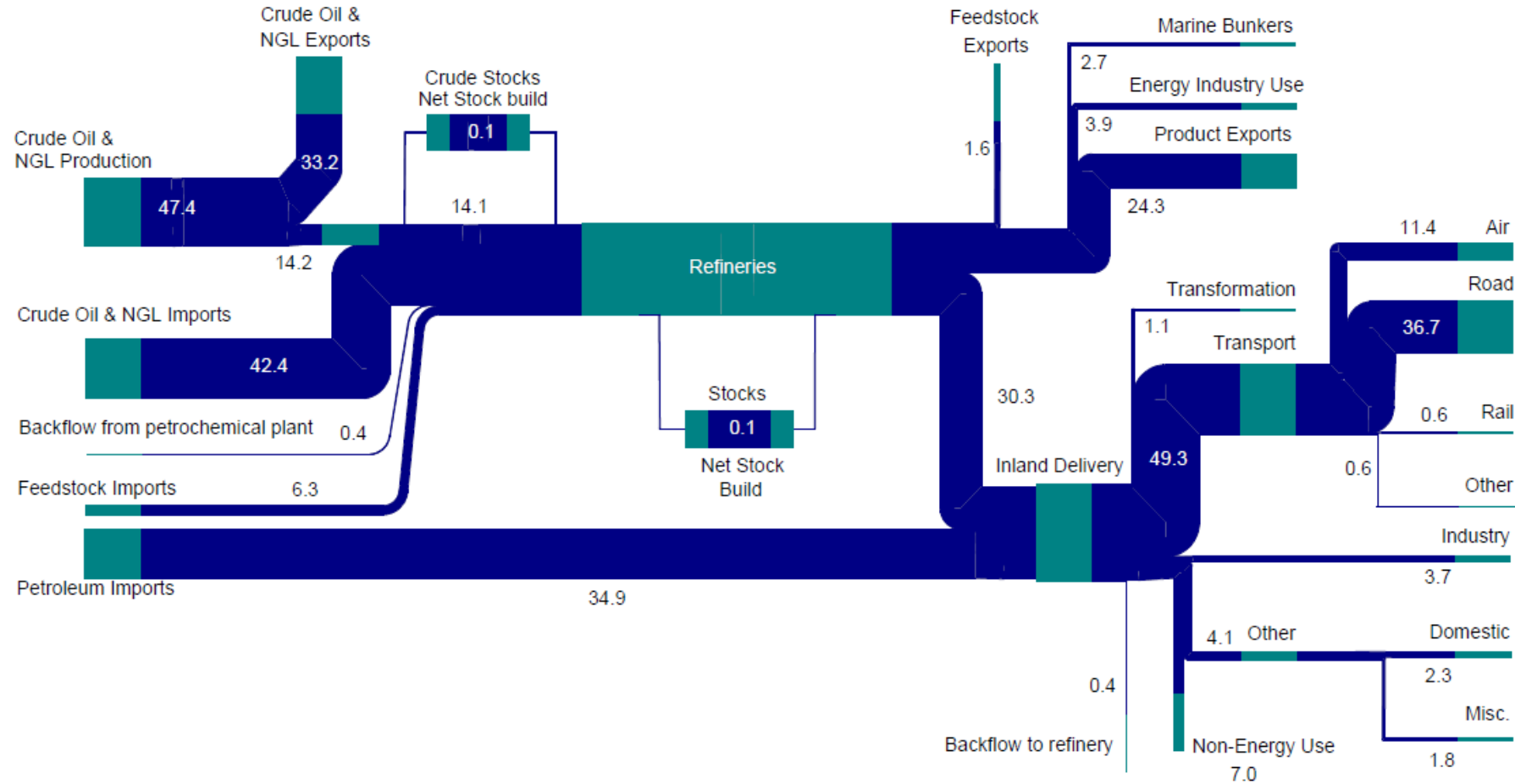
Chart H.2: Petroleum flow chart 2016 (million tonnes)
