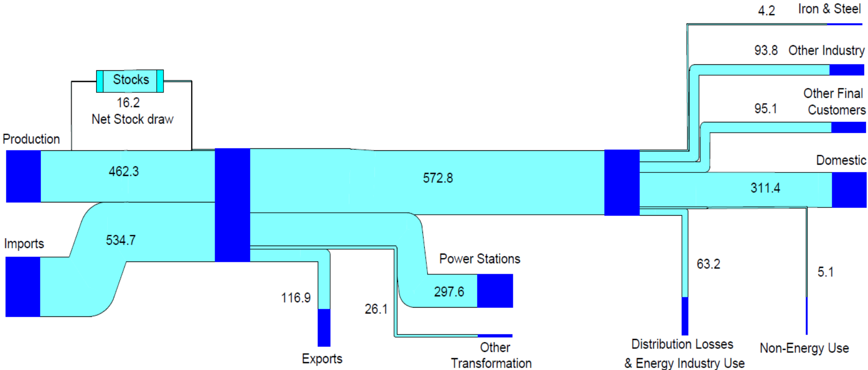
Chart H.3: Natural gas flow chart 2016 (TWh)
