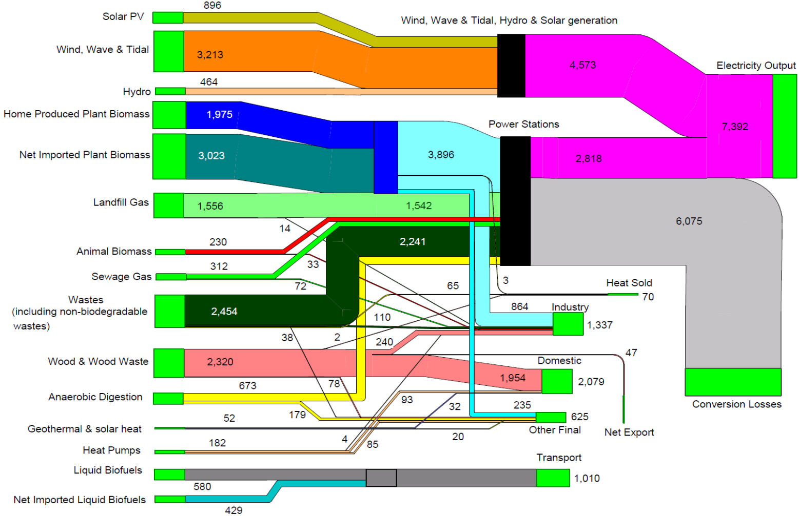
Chart H.5: Renewables flow chart 2016 (thousand tonnes of oil equivalent)
