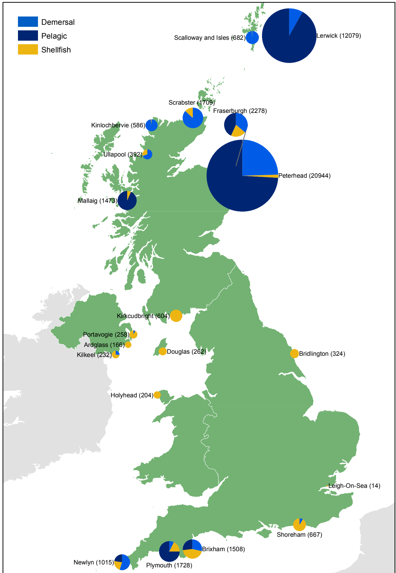
Chart 1: Landings into the top 20 UK ports (a) by UK vessels by species type: November 2016 (tonnes)
