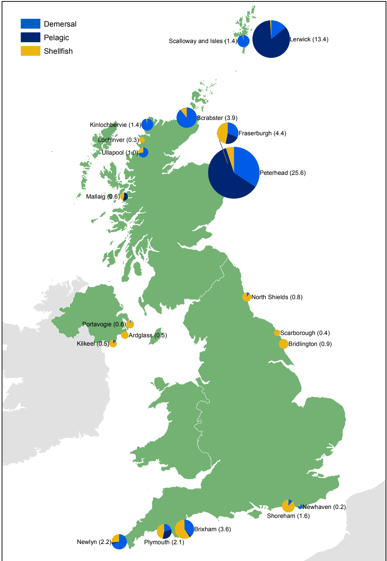
Chart 2: Value of landings into the top 20 UK ports (a) by UK vessels by species type: November 2016 (£million)
