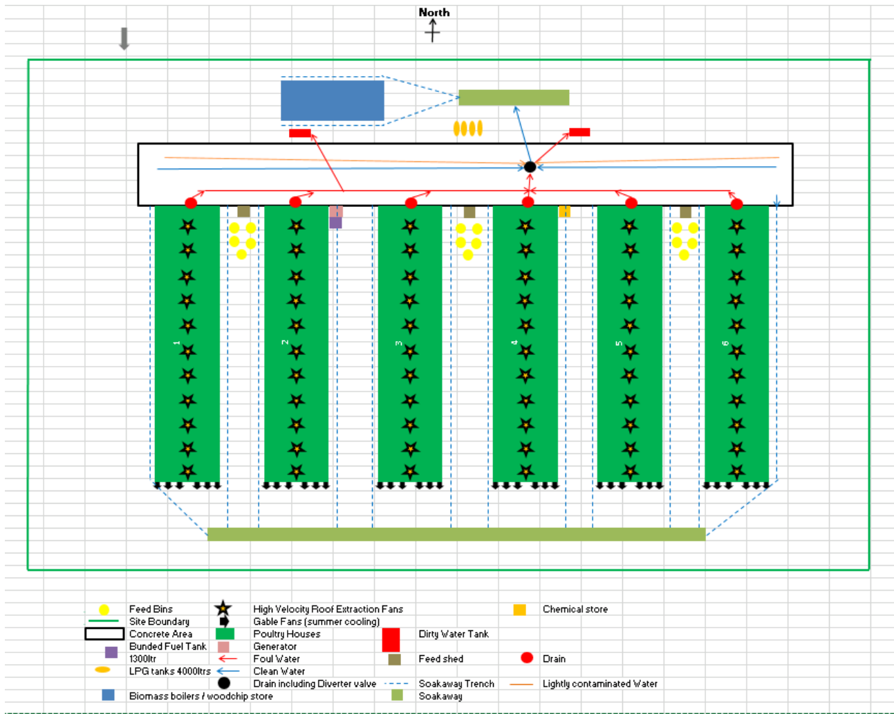
Site layout plan – showing emission points referred to in Tables S3.1 and S3.2
