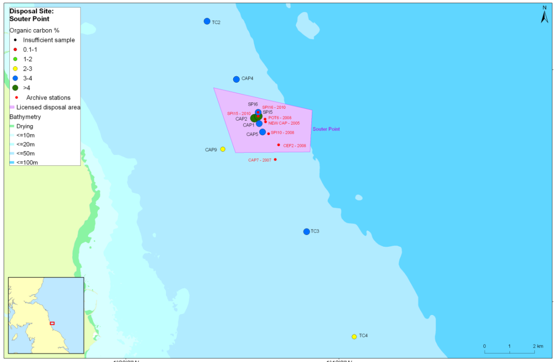
Figure A2.2.8. Organic carbon (%m/m) in the silt/clay fraction (<63µm) at Souter Point, 2010.
