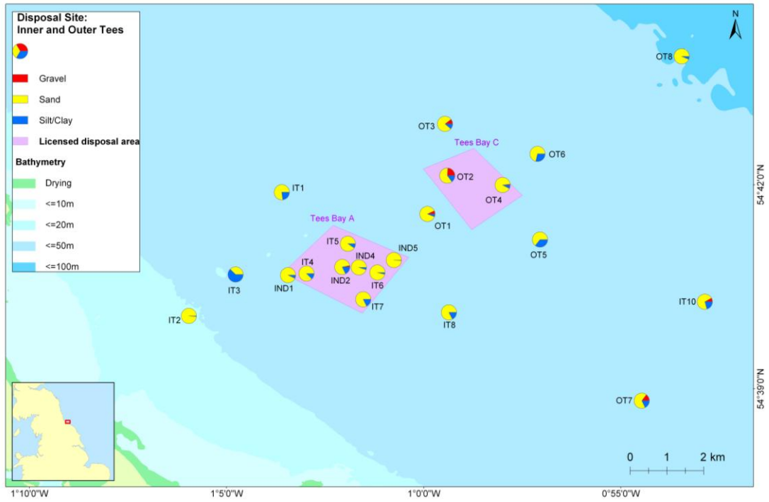
Figure A2.3.6. Pie charts of gravel, sand and silt/clay at Inner Tees (Tees Bay A) and Outer Tees (Tees Bay C) in 2010.
