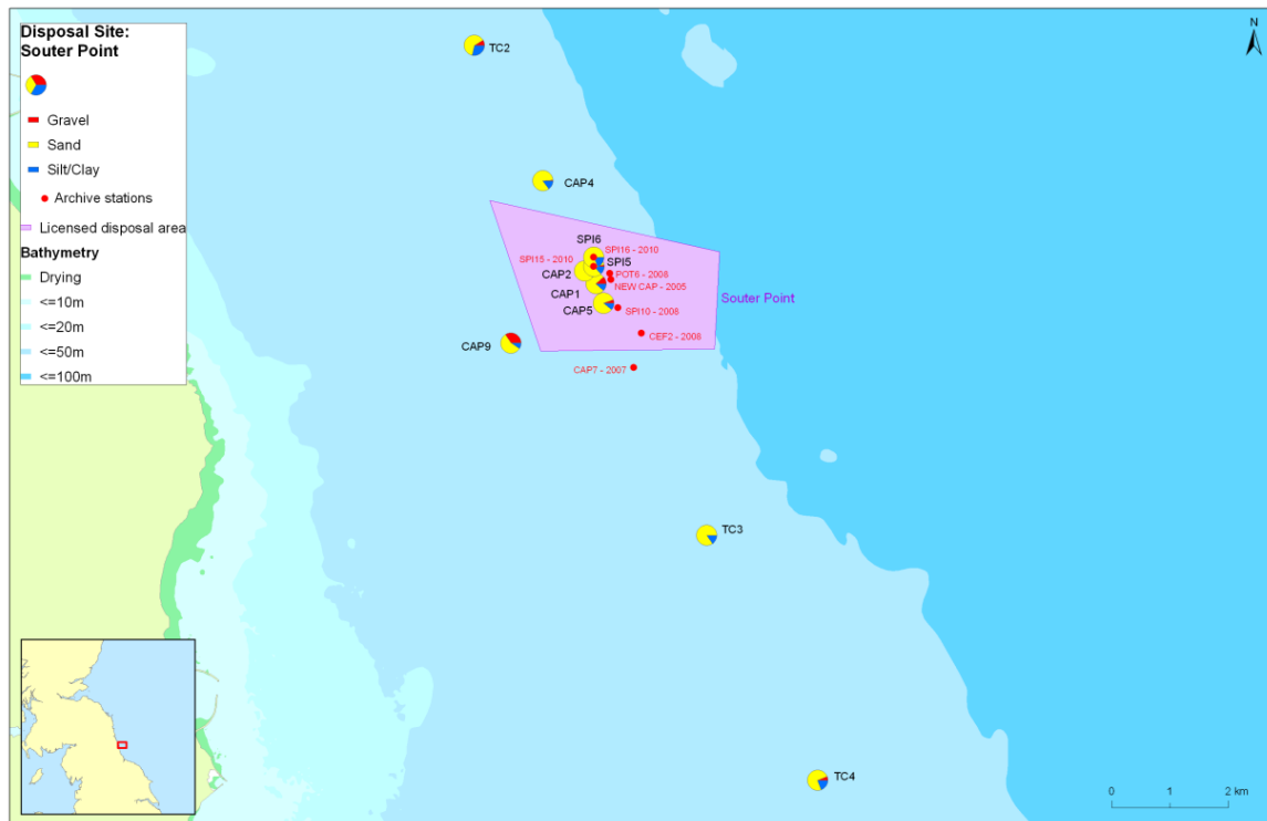
Figure A2.2.6. Pie charts of gravel, sand and silt/clay at Souter Point, 2010.
