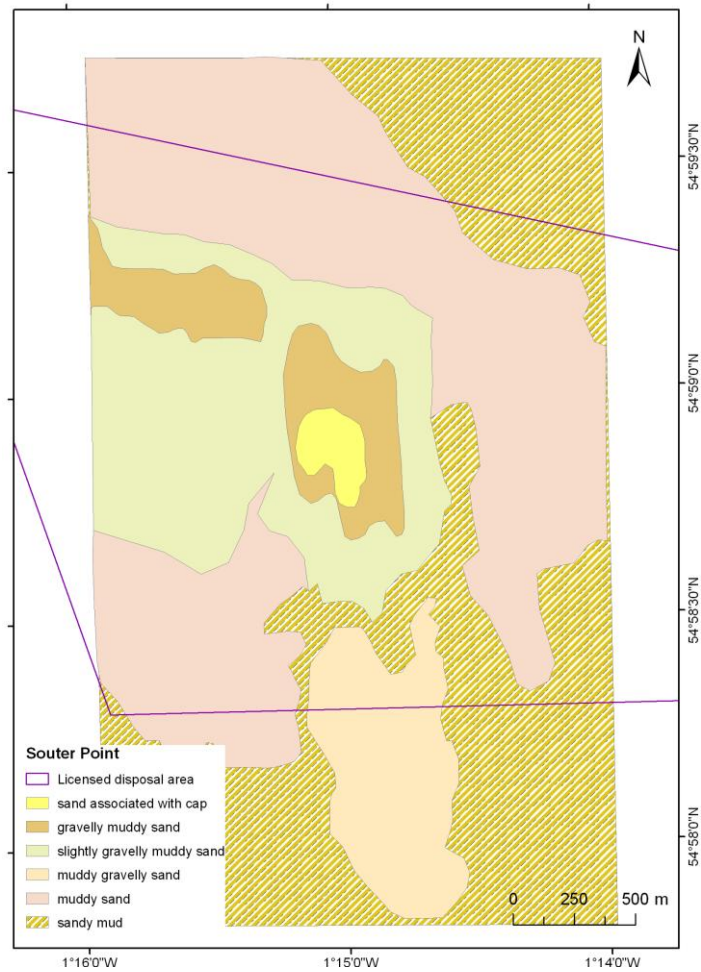
Figure A2.2.4. Interpretation of the multibeam backscatter and sidescan sonar at Souter Point, 2010.
