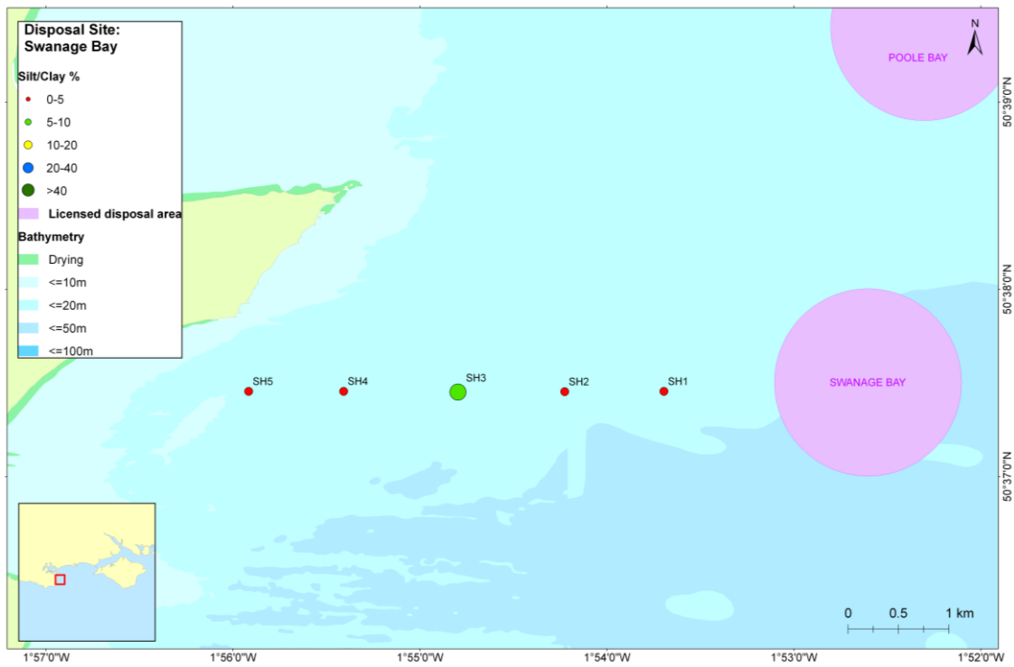
Figure A2.7.3. Silt/clay (%) at Swanage in 2010.
