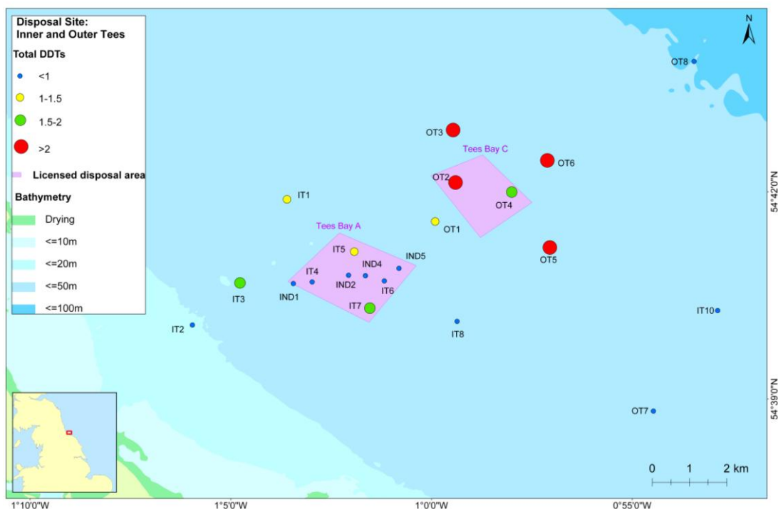
Figure A2.3.16. \Sigma DDTs concentrations for the Inner and Outer Tees Stations, 2010.
