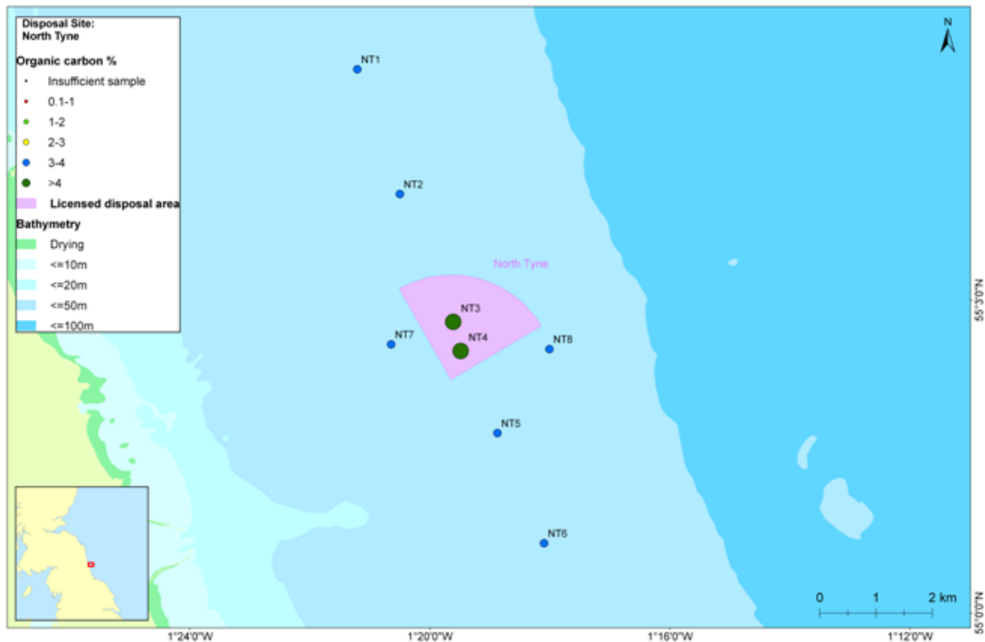
Figure A2.1.4. Organic carbon (%m/m) in the silt/clay fraction (<63µm) at North Tyne in 2010.
