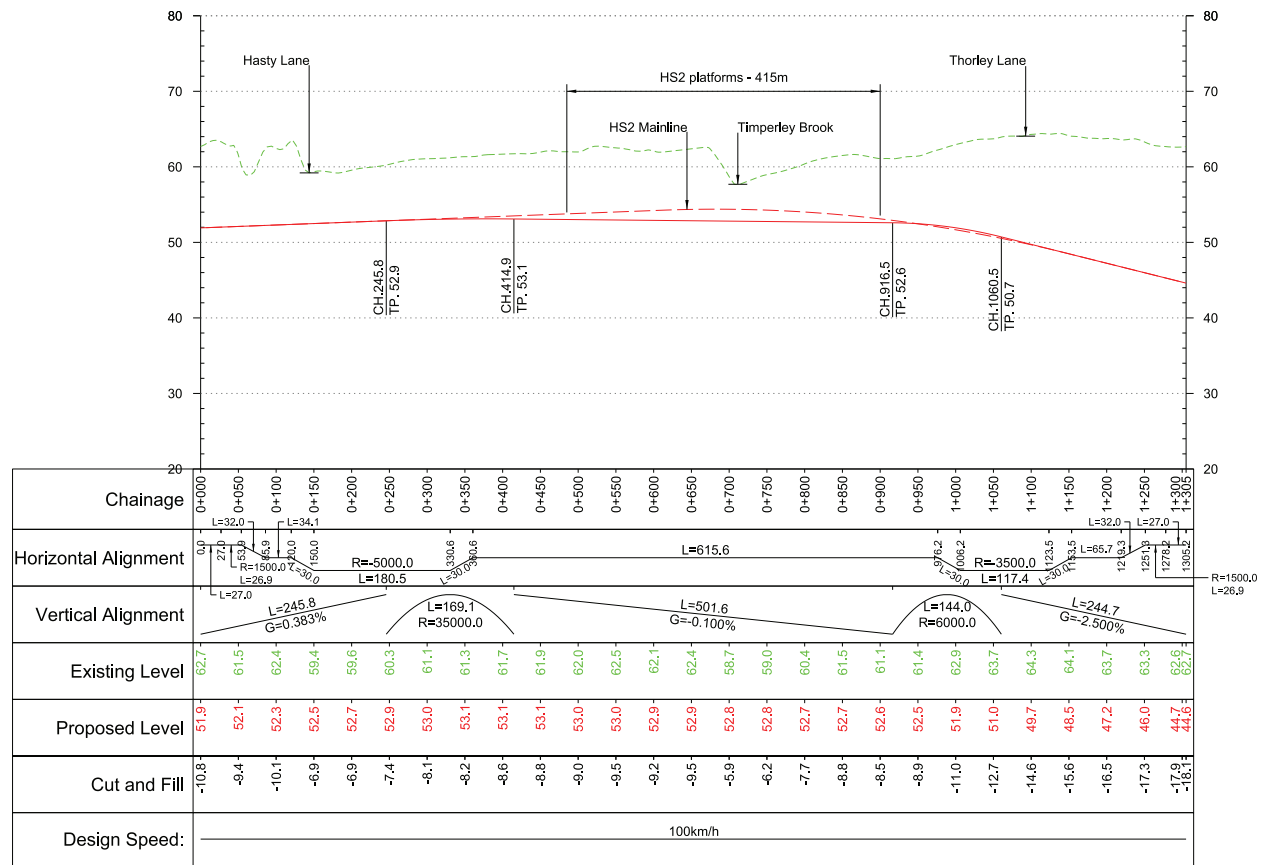
Profile - Platform Tracks Scale H:1:5,000 V:1:500 @ A1
