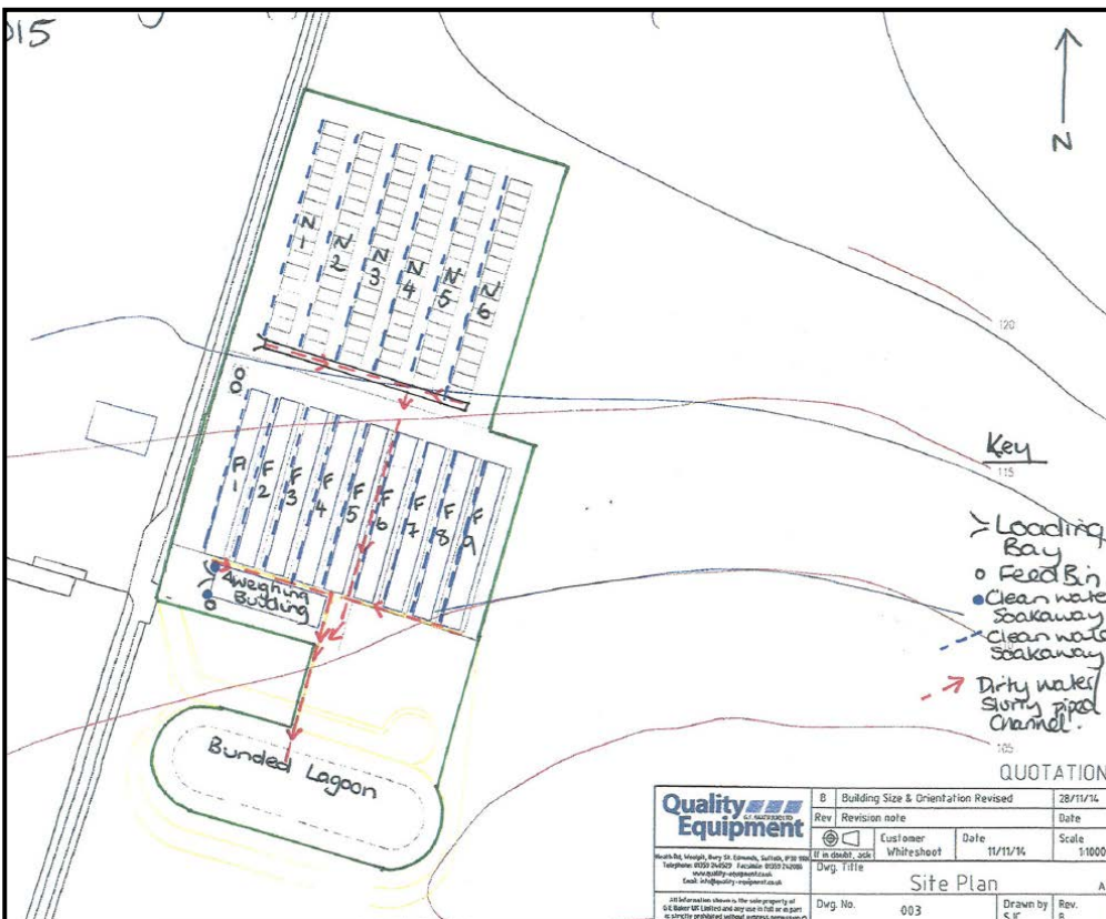
Drainage plan
