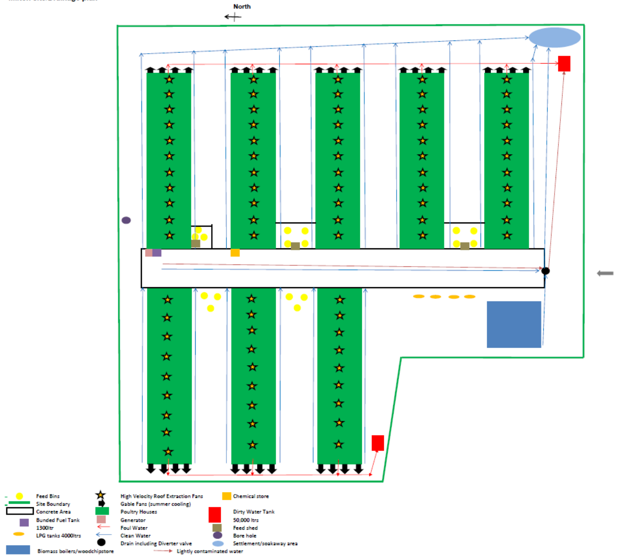
Milton site/Drainage plan
