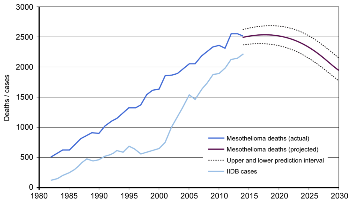
Figure 2: Mesothelioma in Great Britain – annual actual and predicted deaths
