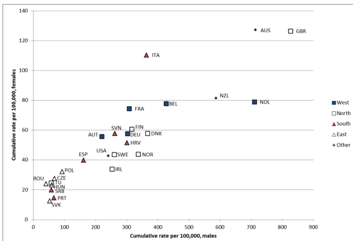
Figure 2: Cumulative death rates per 100,000 to age 85 in males vs females in the European region and selected other countries, 2008-2012
