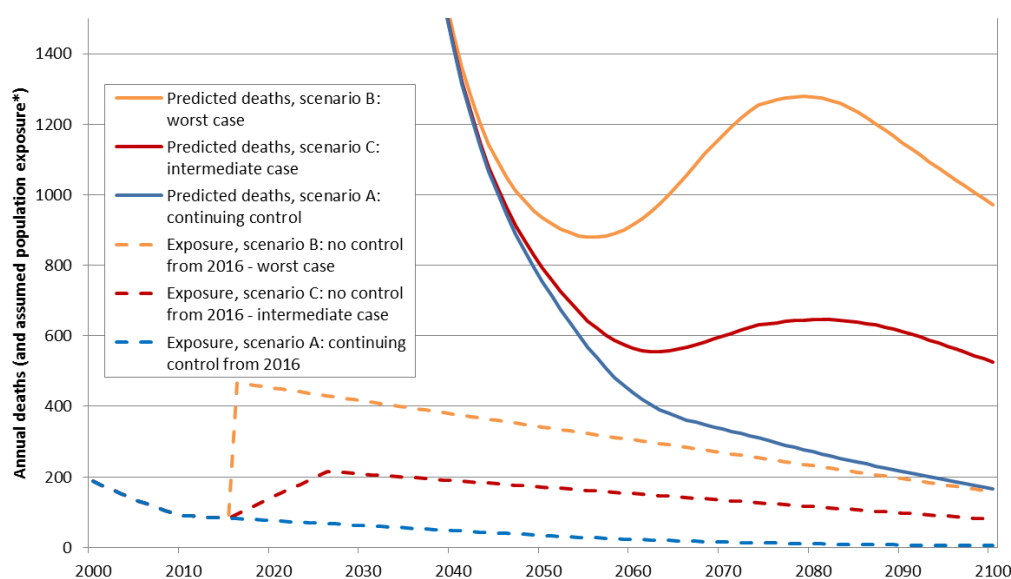
Figure 8: Predicted annual cancer deaths for three scenarios for population asbestos exposure from 2016
