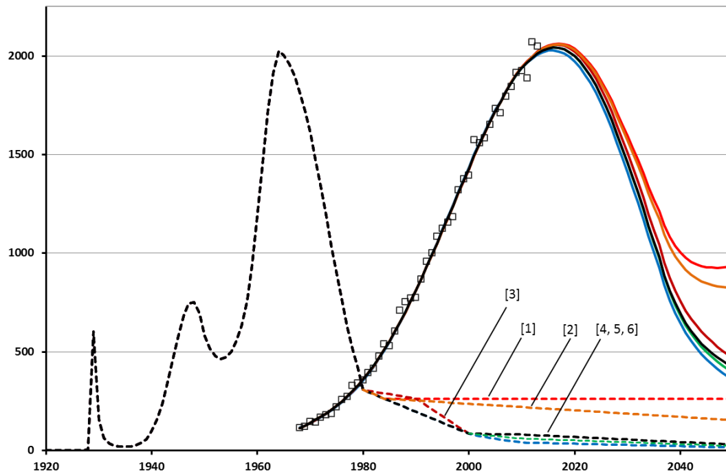
Figure 7: Observed and predicted annual mesothelioma mortality under six alternative scenarios for annual population exposure from 1980, males aged 20-89
