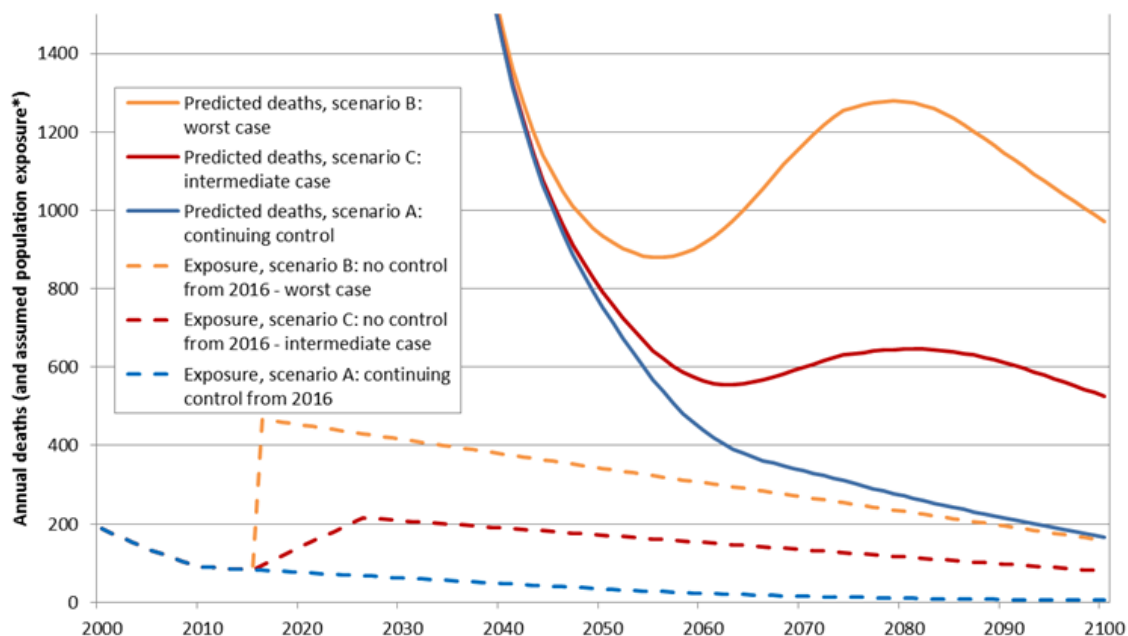
Figure 1 – Predicted annual deaths and exposures from the different scenarios
