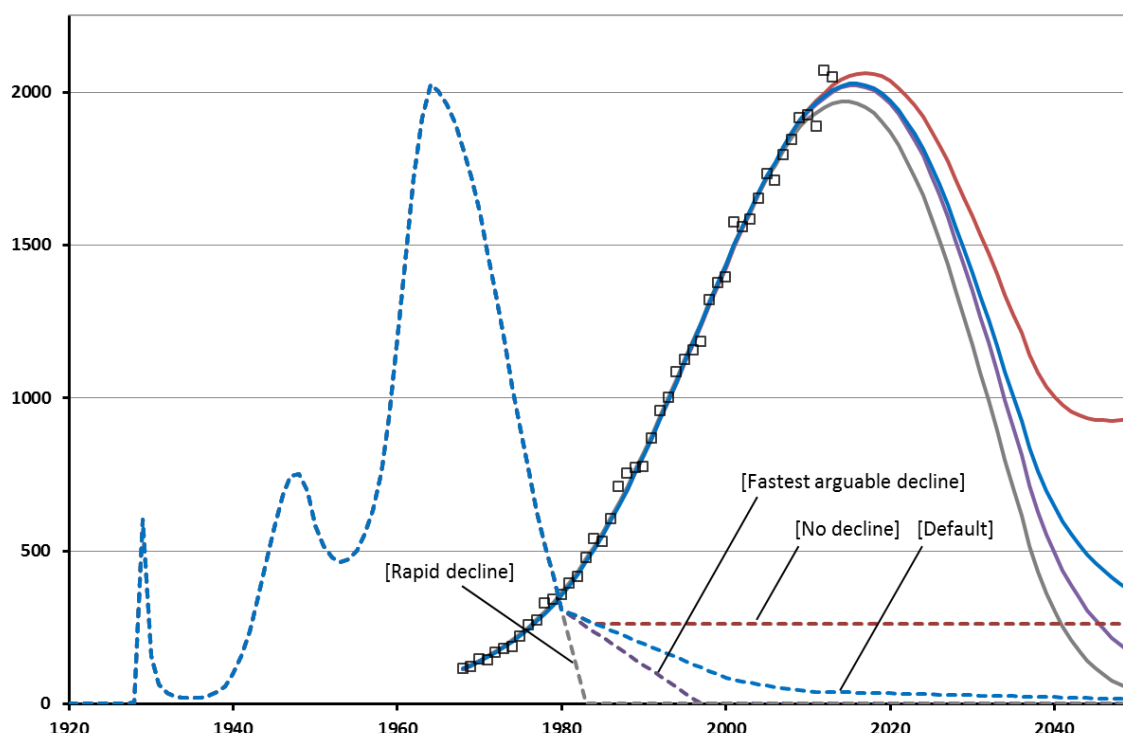
Figure 4: Observed and predicted annual mesothelioma mortality for various possible annual population exposure profiles from 1980, males aged 20-89
