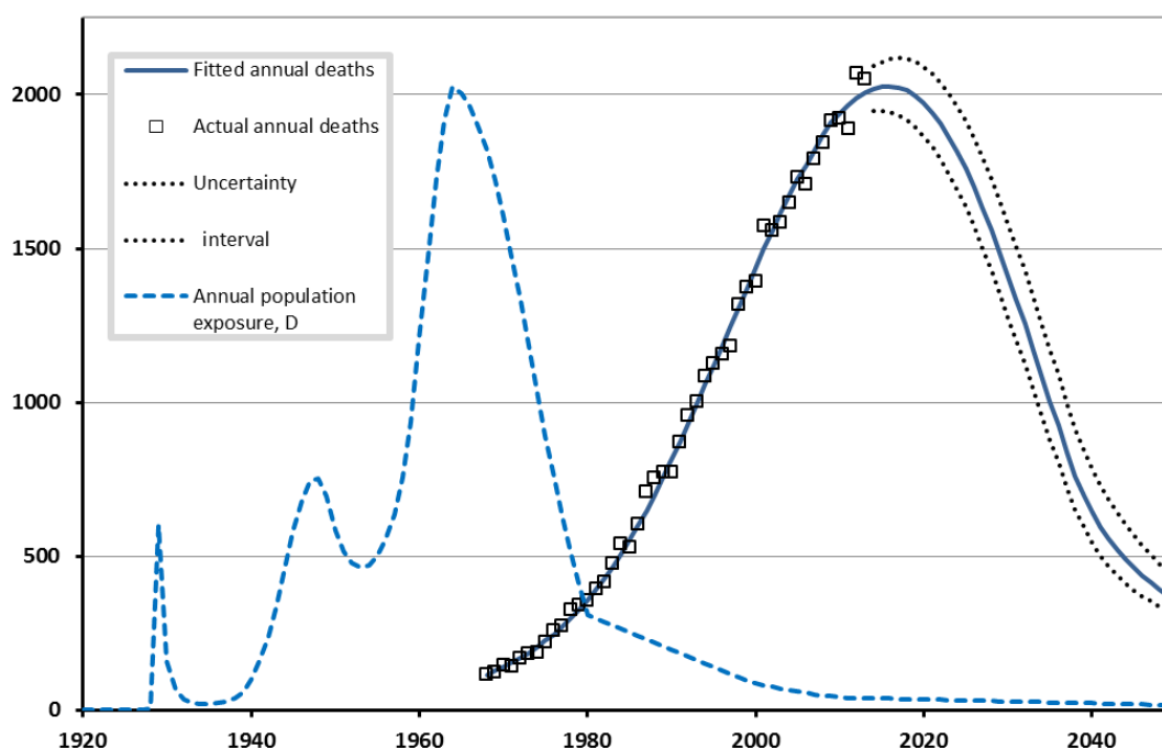
Figure 3: Observed and predicted annual mesothelioma mortality, with annual population exposure, males aged 20-89
