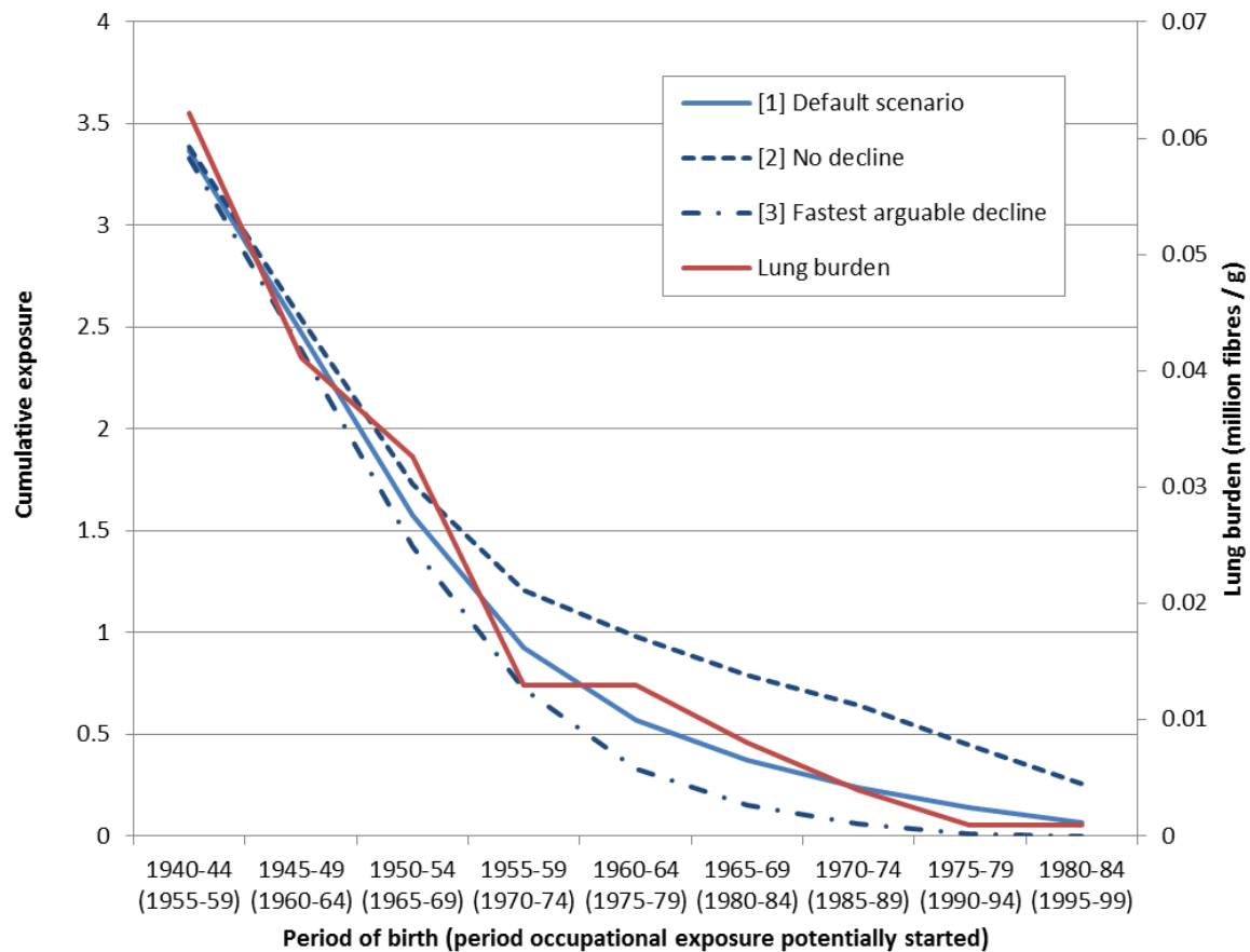
Figure 6A: Average population lung burdens of amphibole asbestos by period of birth and implied cumulative exposures under three scenarios
