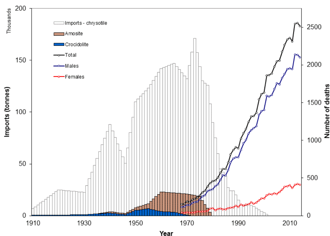
Figure 1: Annual asbestos imports and mesothelioma deaths in Great Britain, 1910-2014
