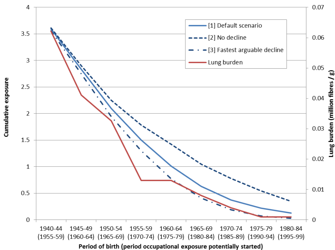
Figure 6B: Average population lung burdens of amphibole asbestos by period of birth and implied cumulative exposures with higher exposure potential below working age
