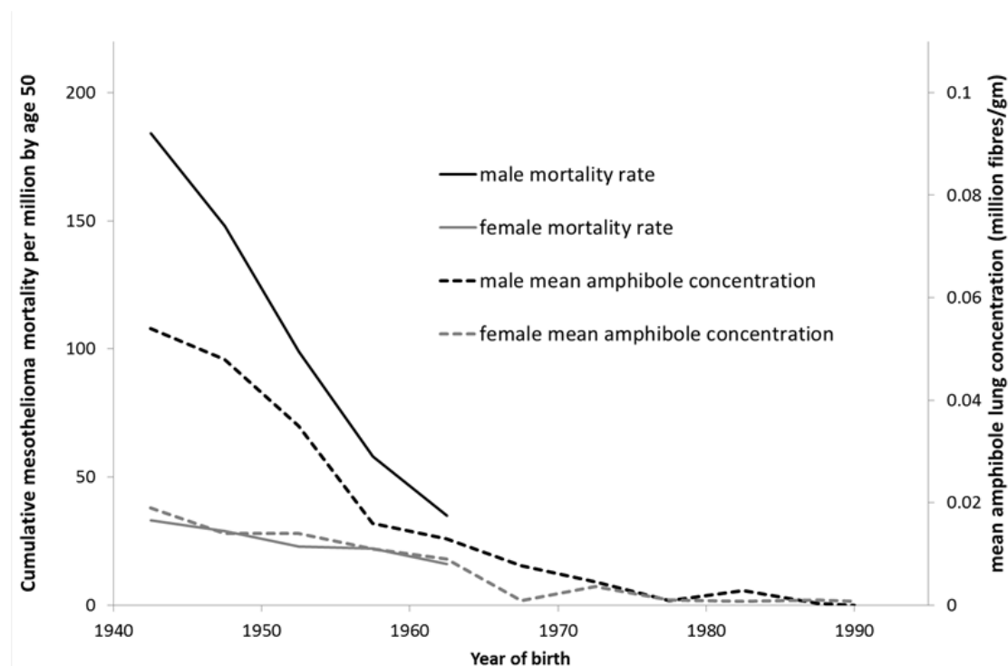
Figure 5: National mesothelioma mortality and average amphibole asbestos lung burdens* in Britain by period of birth (million fibres/gm longer than 5 microns)
