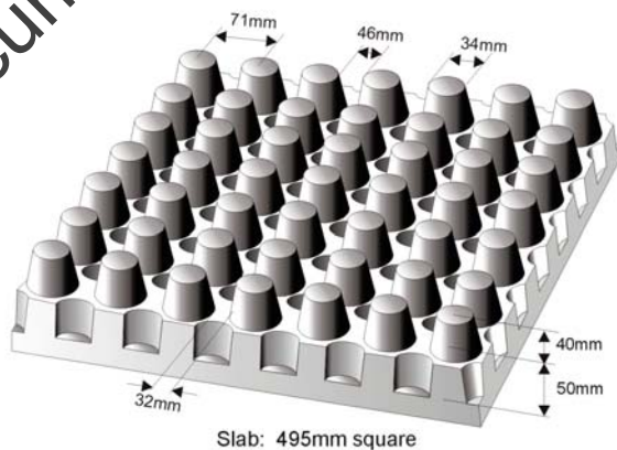
Figure 5.6 “Pelcar” concrete substrate
