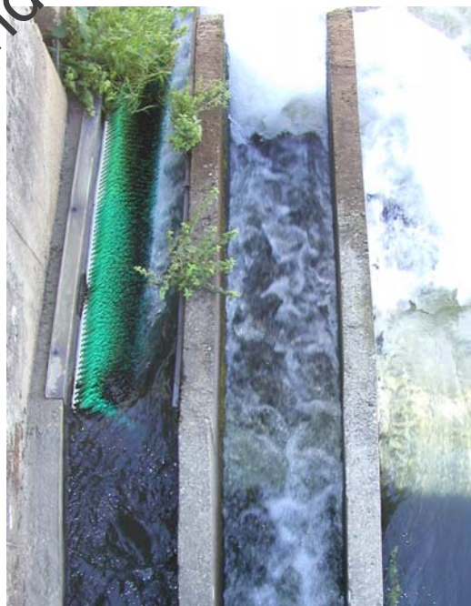
Figure 6.2. Detail of eel pass at Moulin a Pigné
