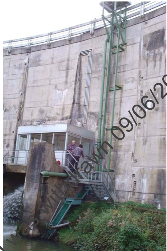
Figure 6.12. The Ville Hatte Dam eel lift. The substrate ramps can be seen below the platform.
