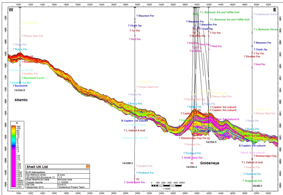
Figure 5-15: West to east cross-section from the Atlantic field to the Goldeneye field showing the effective permeability distribution.
