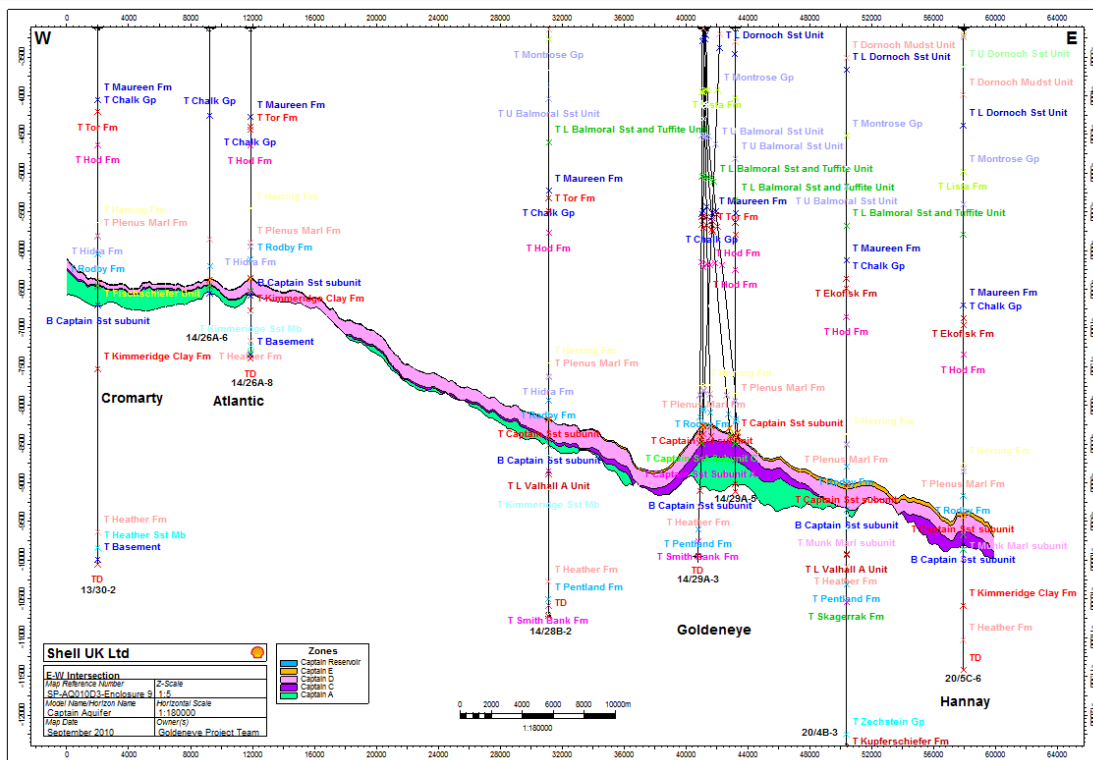
Figure 5-9: West-east intersection from the Cromarty field through Atlantic and Goldeneye and Hannay field.
