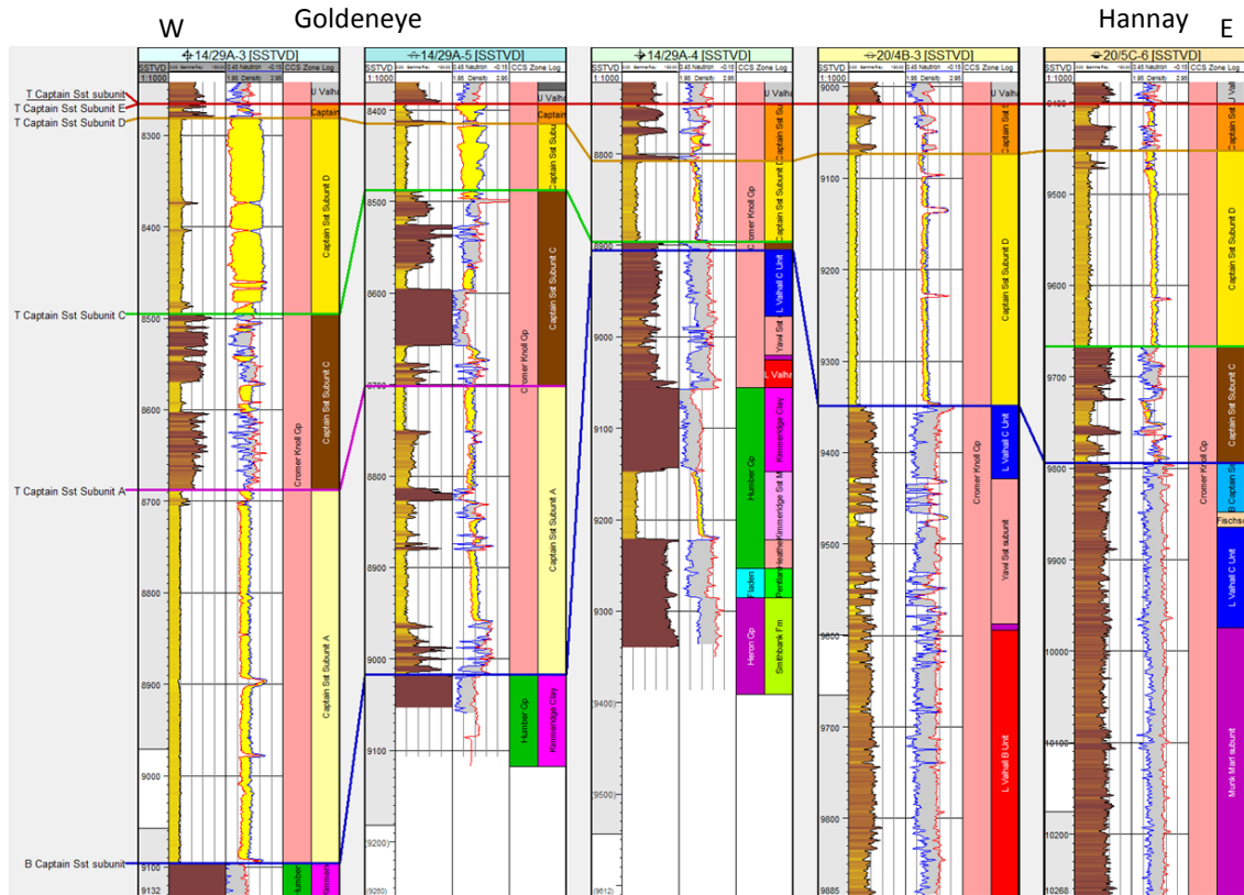
Figure 4-7: Reference case correlation through Wells 14/29a-3, 14/29a-5, 14/29a-4, 20/4b-3 and 20/5c-6 from Goldeneye to Hannay.
