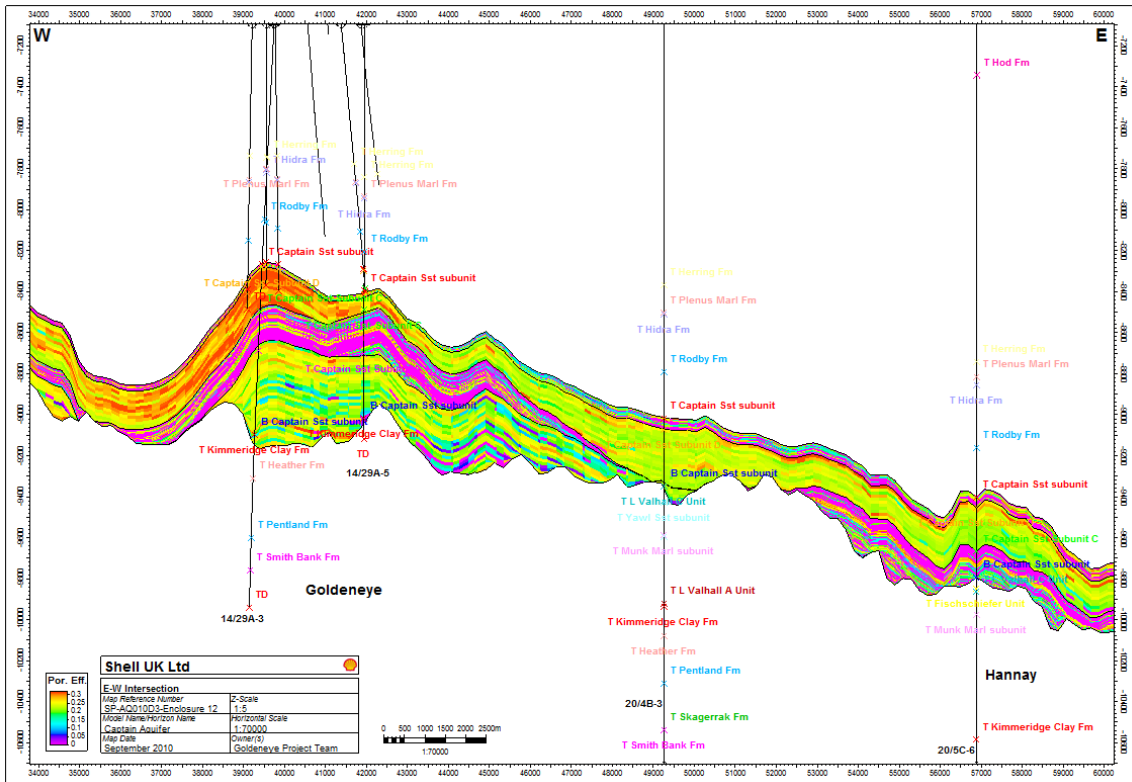
Figure 5-14: West to east cross-section from the Goldeneye field to the Hannay field showing the effective porosity distribution.
