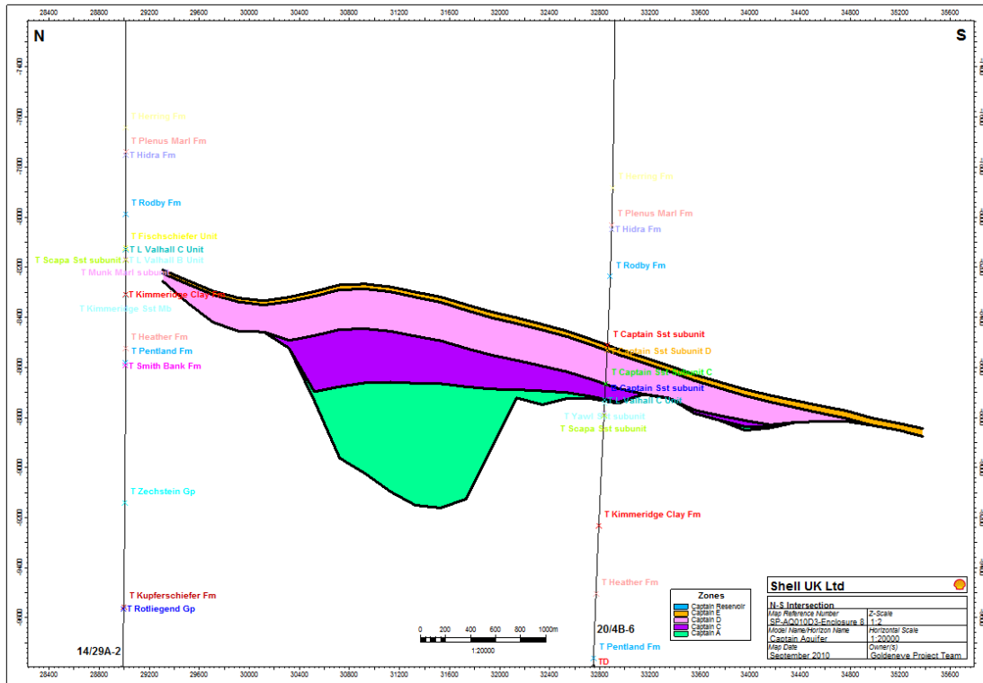
Figure 5-8: North-south intersection of aquifer model through the Goldeneye field.
