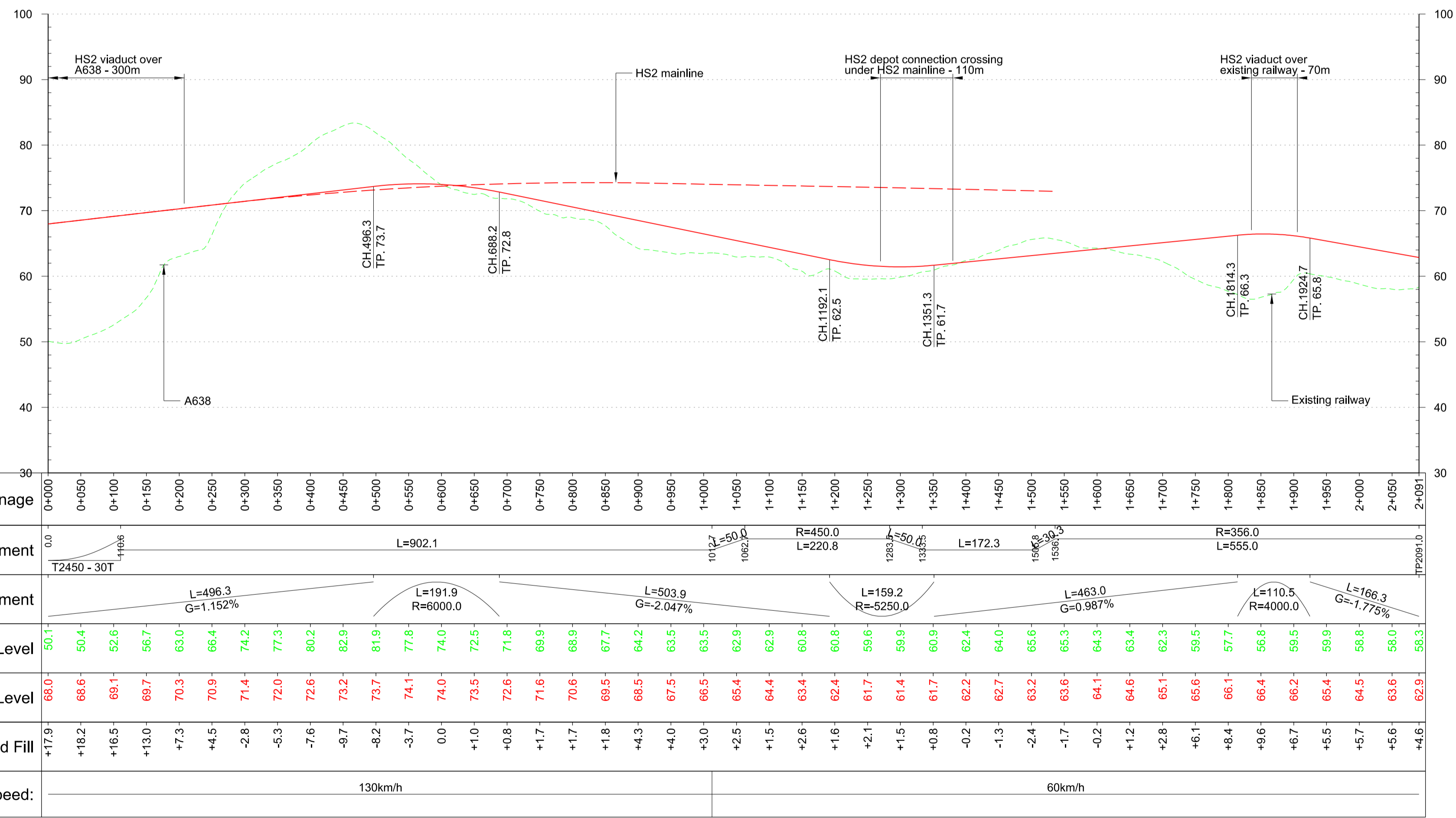
Profile Scale H:1:5,000 V:1:500 @ A1
