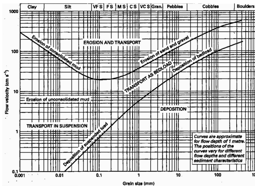
Figure 5.8 Hjulstrom Curve
