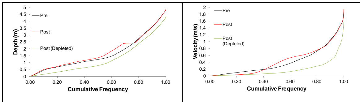
Figure 6.1 Cumulative frequency plots – Pershore (left Q20 depth, right Q20 velocity)
