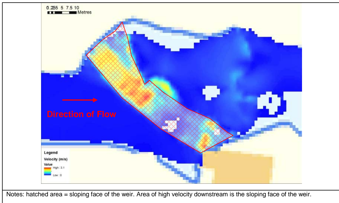
Figure 5.3 Example output from an instream 2D hydraulic model (JBA, model of Salts Mill Weir)
