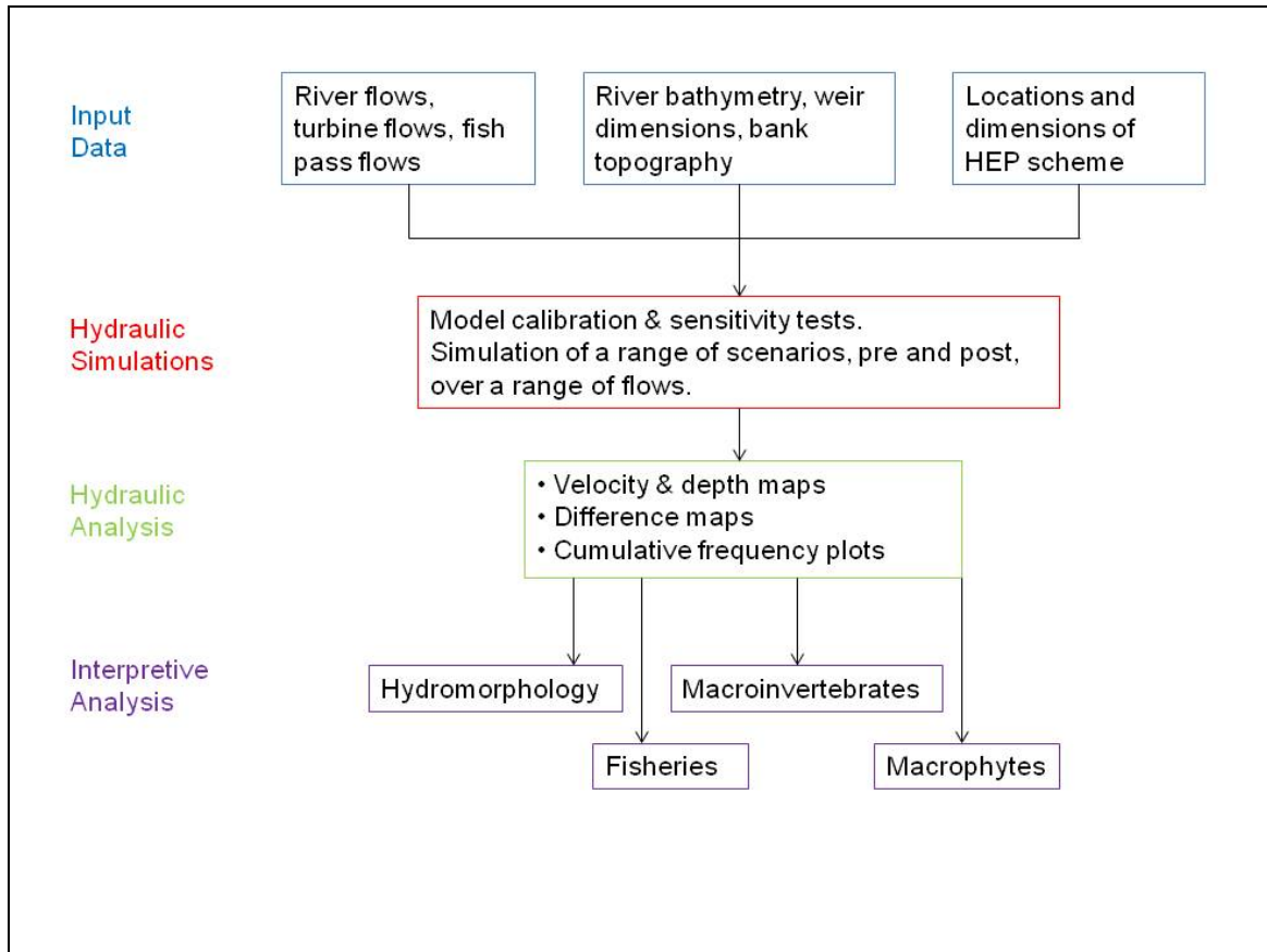
Figure 5.6 Modelling process chart
