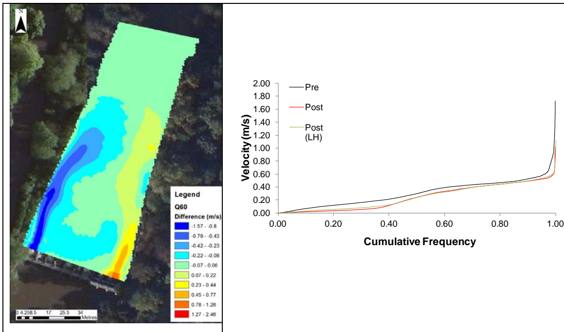
Figure 5.7 Example data analysis techniques
