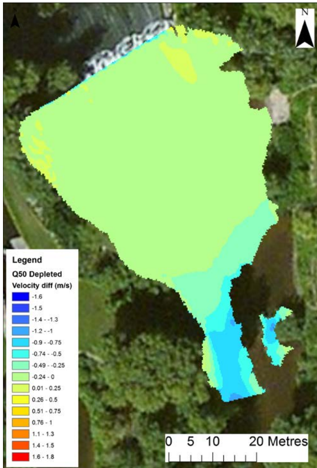
Figure 6.2 Q50 Depleted reach depth difference map (post-change – pre-change)
