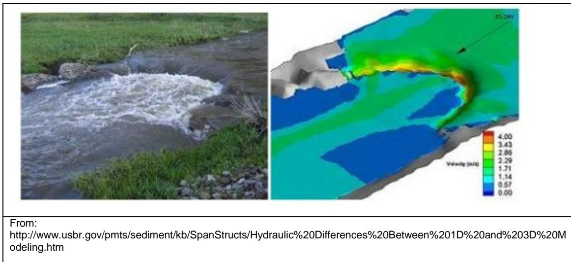
Figure 5.4 Example 3D outputs from Holmquist-Johnson (2009)
