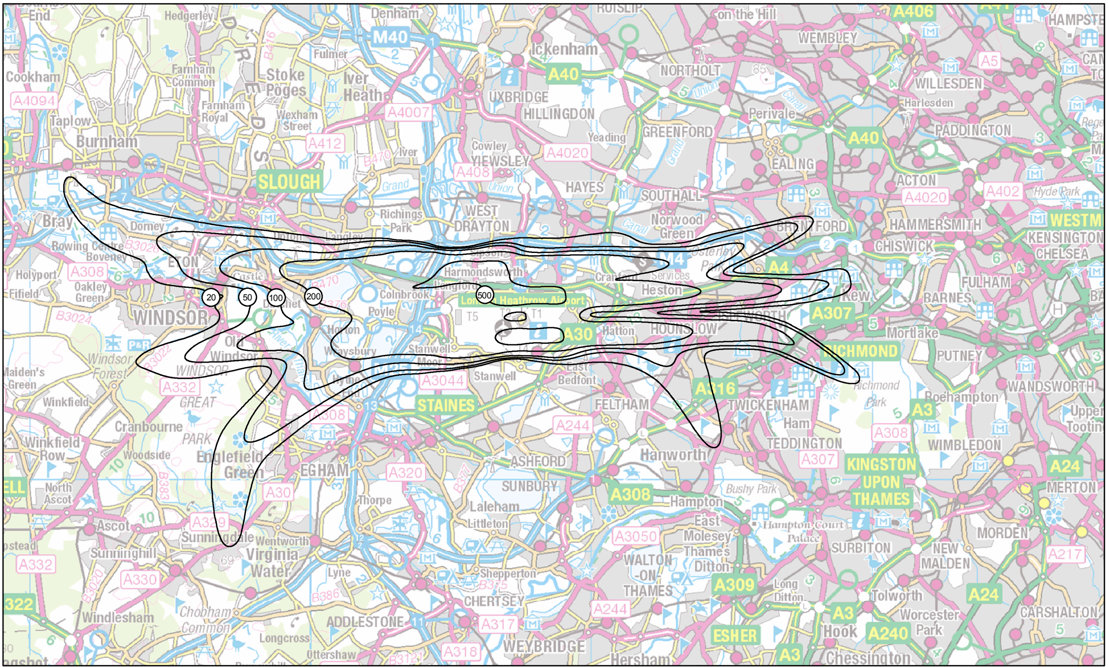
H30-3R-T: Heathrow 2030 do-something, HAL - Minimise total affected Summer average daytime N70
