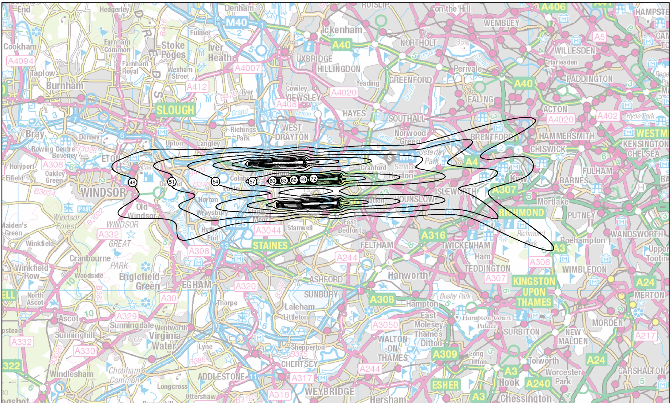
H40-3R-T: Heathrow 2040 do-something, HAL - Minimise total affected Summer average 8-hour night-time LAeq,8h
