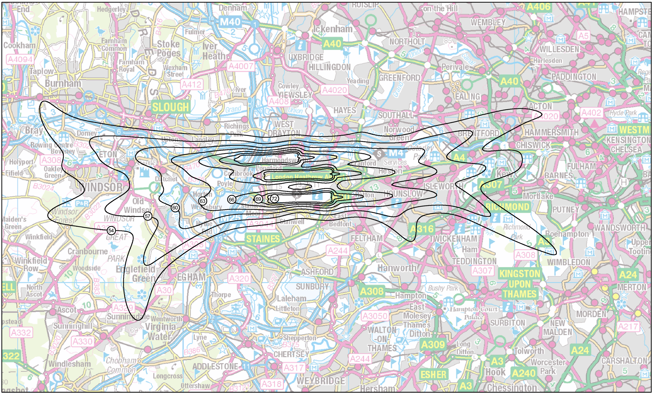
H30-3R-T: Heathrow 2030 do-something, HAL - Minimise total affected Summer average 16-hour daytime LAeq,16h
