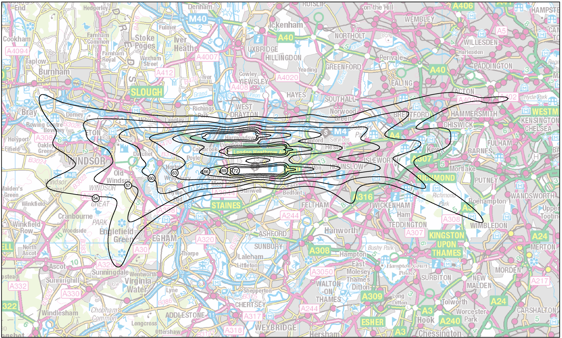
H40-3R-T: Heathrow 2040 do-something, HAL - Minimise total affected Summer average 16-hour daytime LAeq,16h
