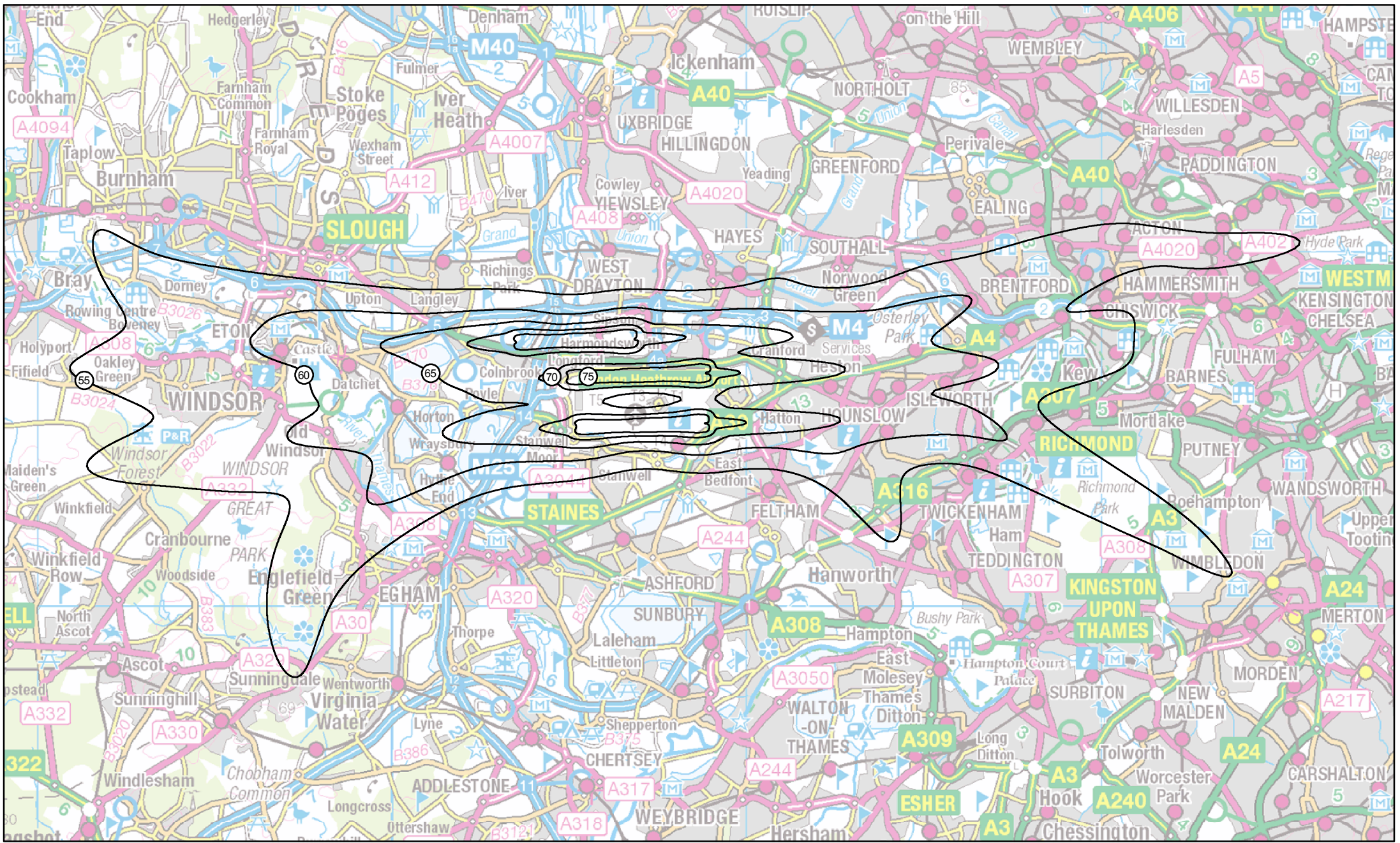
H30-3R-T: Heathrow 2030 do-something, HAL - Minimise total affected Annual average Lden
