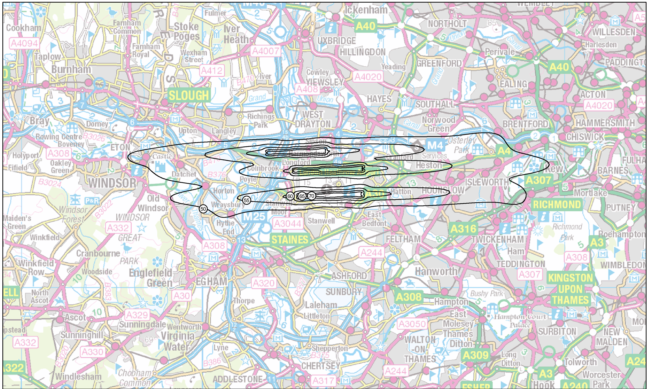
H50-3R-R: Heathrow 2050 do-something, HAL - Respite Annual average Night
