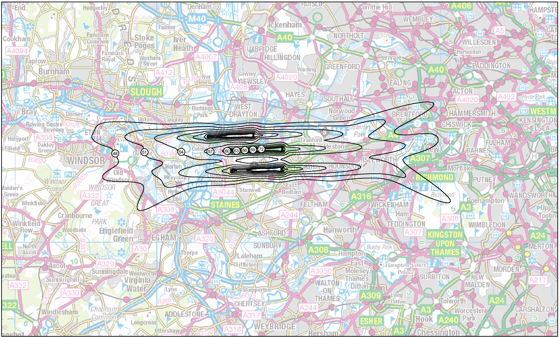
H30-3R-T: Heathrow 2030 do-something, HAL - Minimise total affected Summer average 8-hour night-time LAeq,8h
