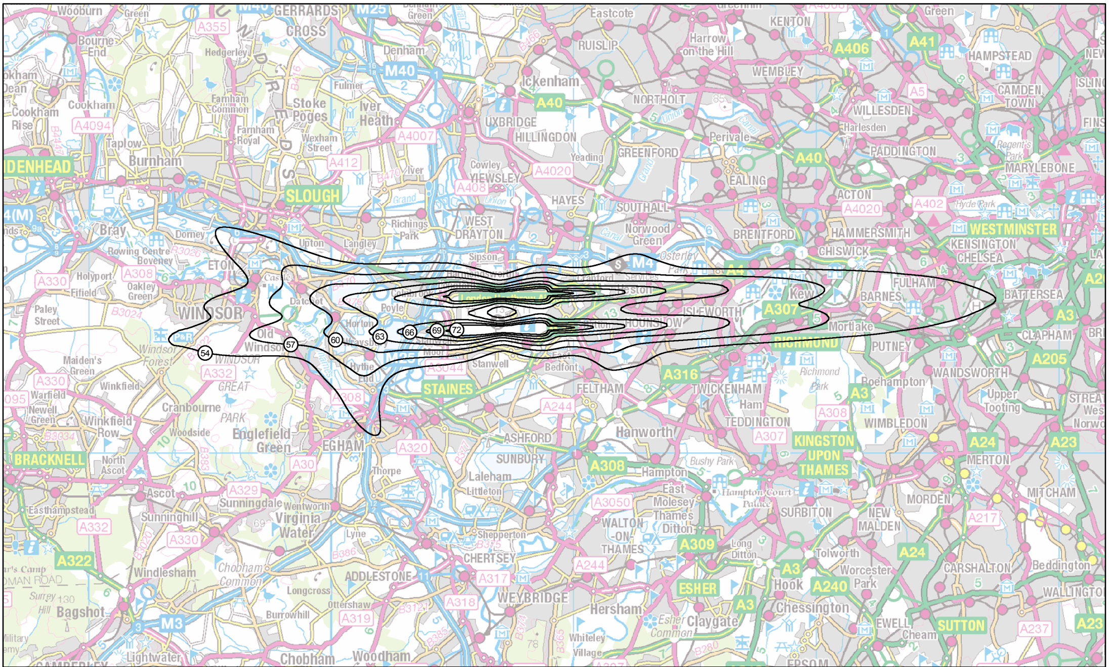
H50-2R: Heathrow 2050 do-minimum Summer average 16-hour daytime LAeq,16h
