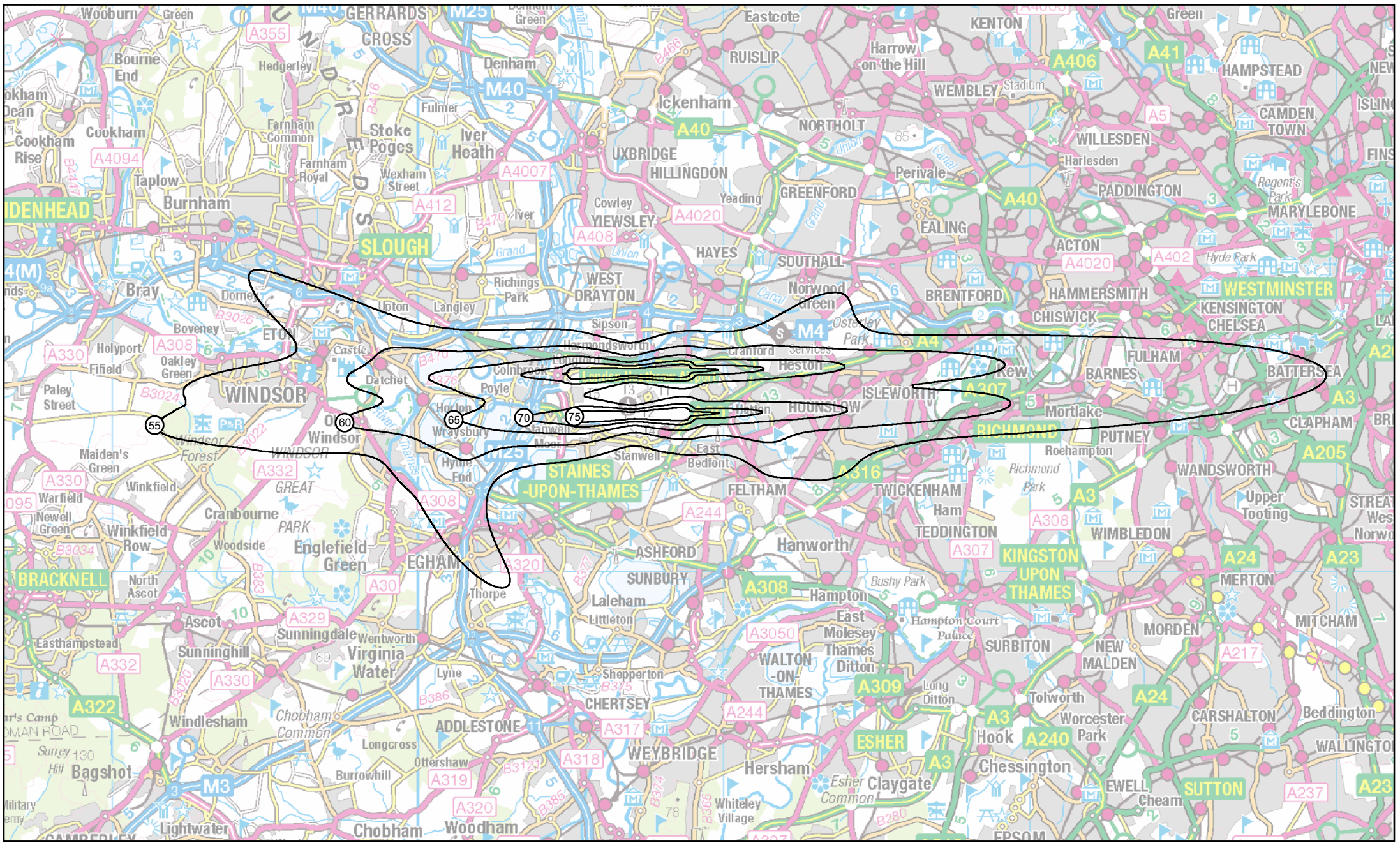
H40-2R-NCT: Heathrow 2040 do-minimum, Need Carbon Traded Annual average Lden
