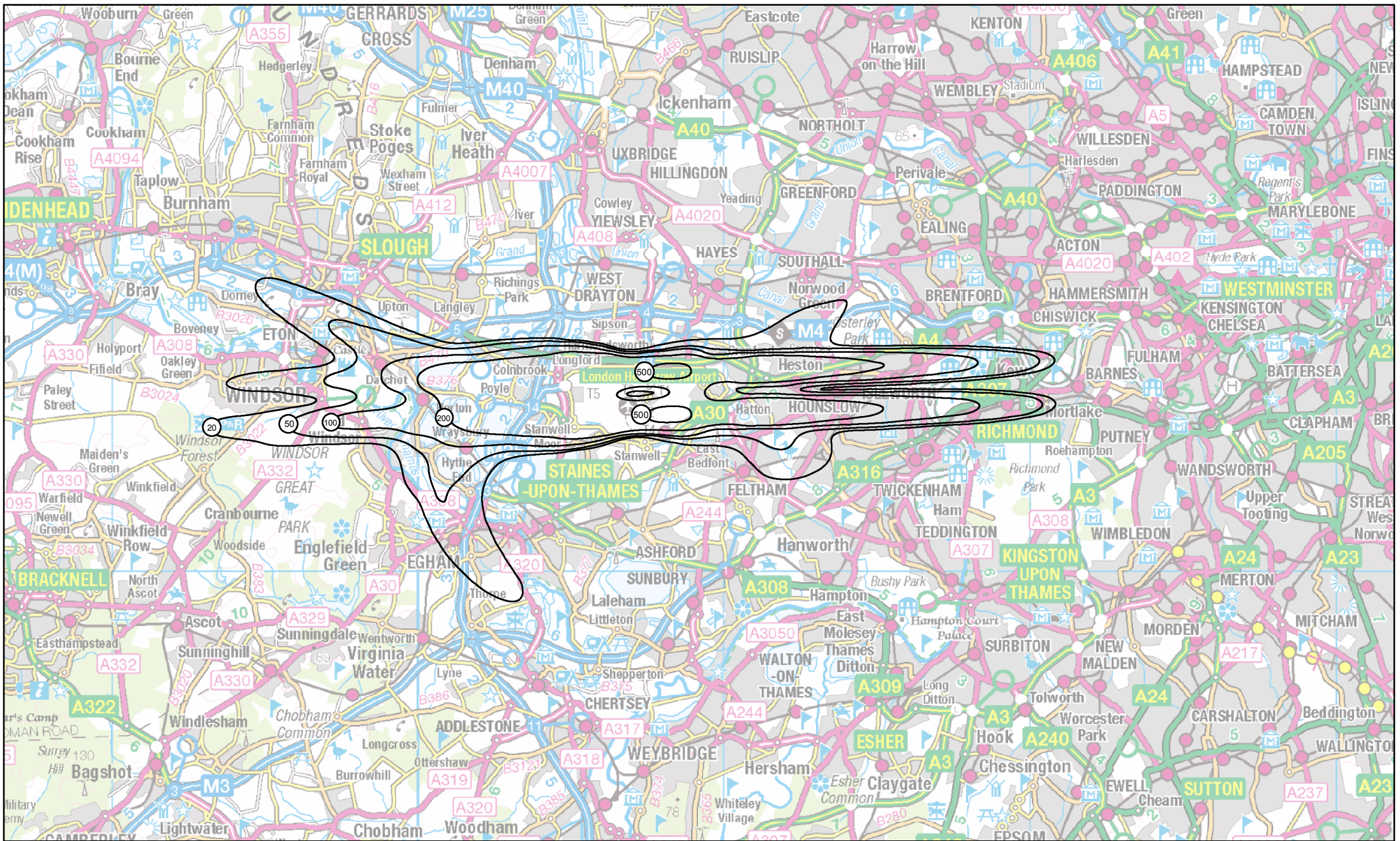
H40-2R-NCT: Heathrow 2040 do-minimum, Need Carbon Traded Summer average daytime N70
