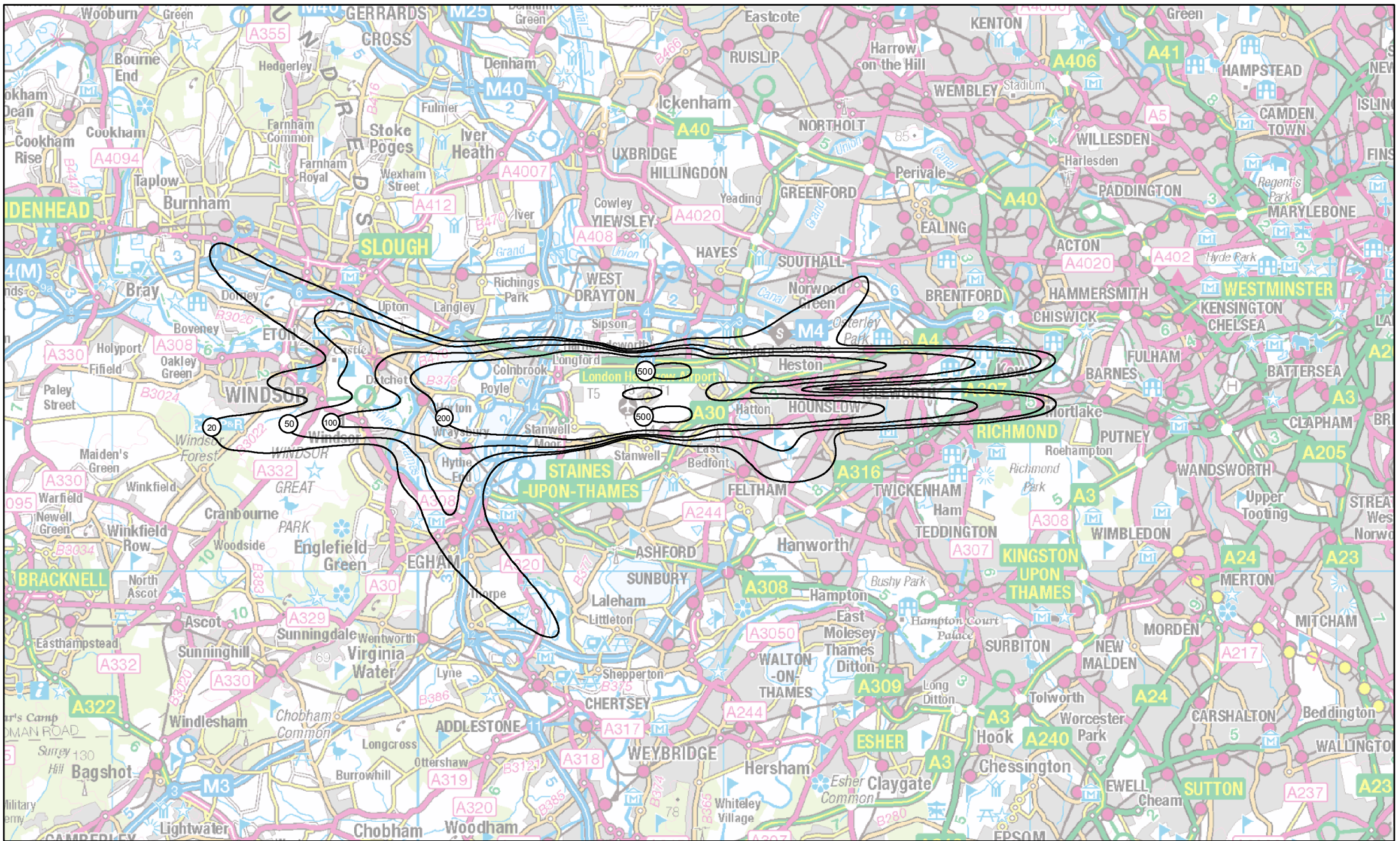
H30-2R-NCT: Heathrow 2030 do-minimum, Need Carbon Traded Summer average daytime N70
