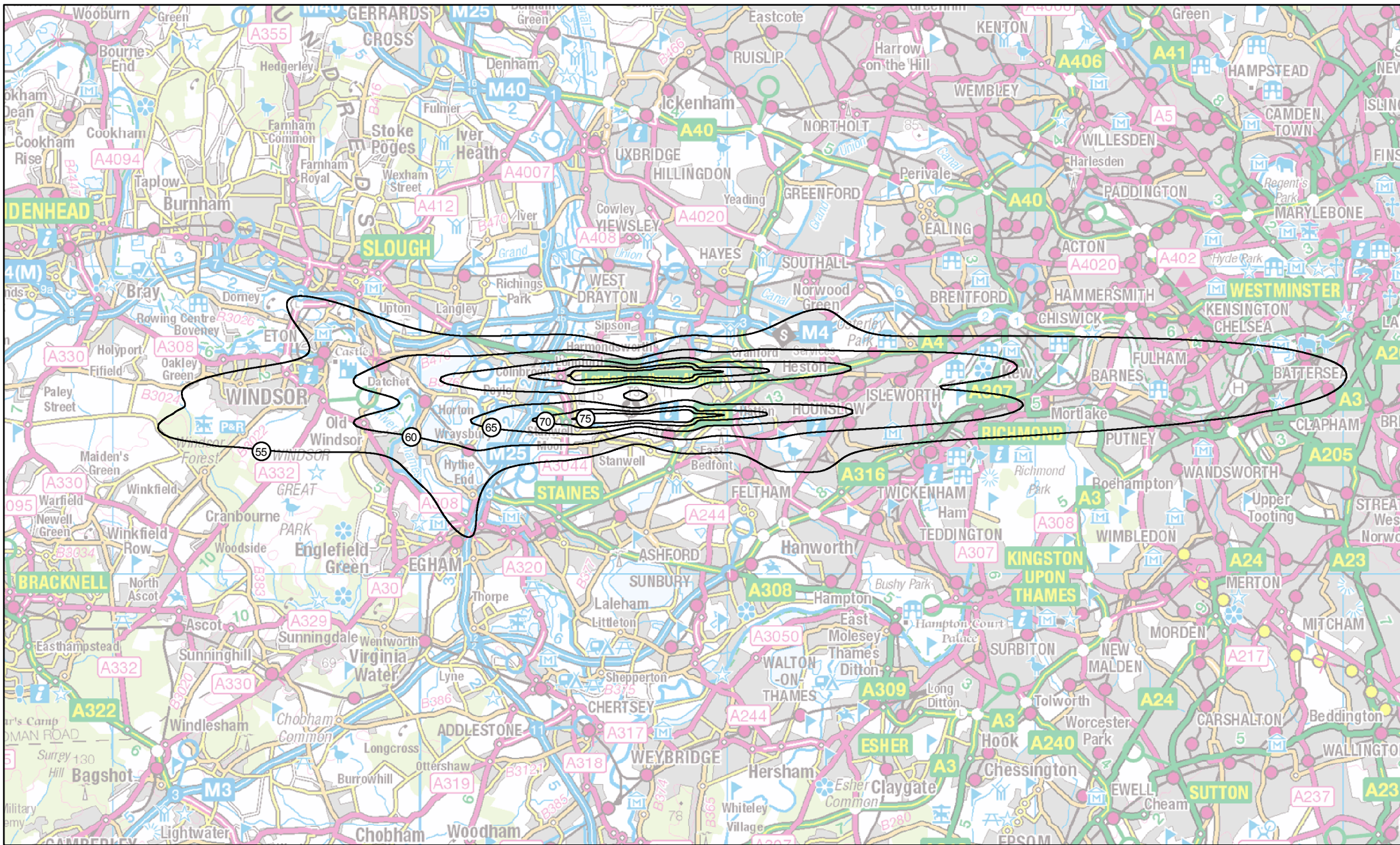
H50-2R: Heathrow 2050 do-minimum Annual average Lden
