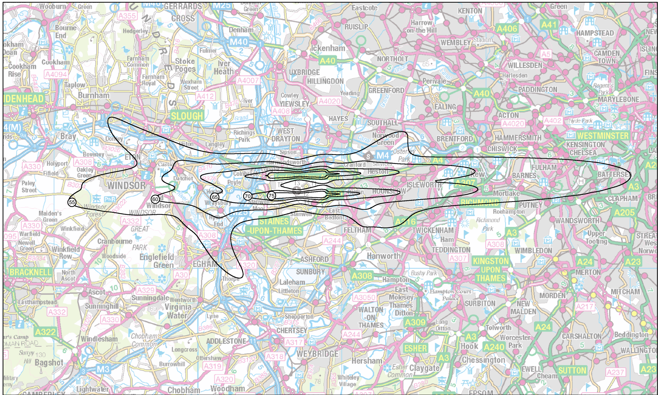
H30-2R-NCT: Heathrow 2030 do-minimum, Need Carbon Traded Annual average Lden
