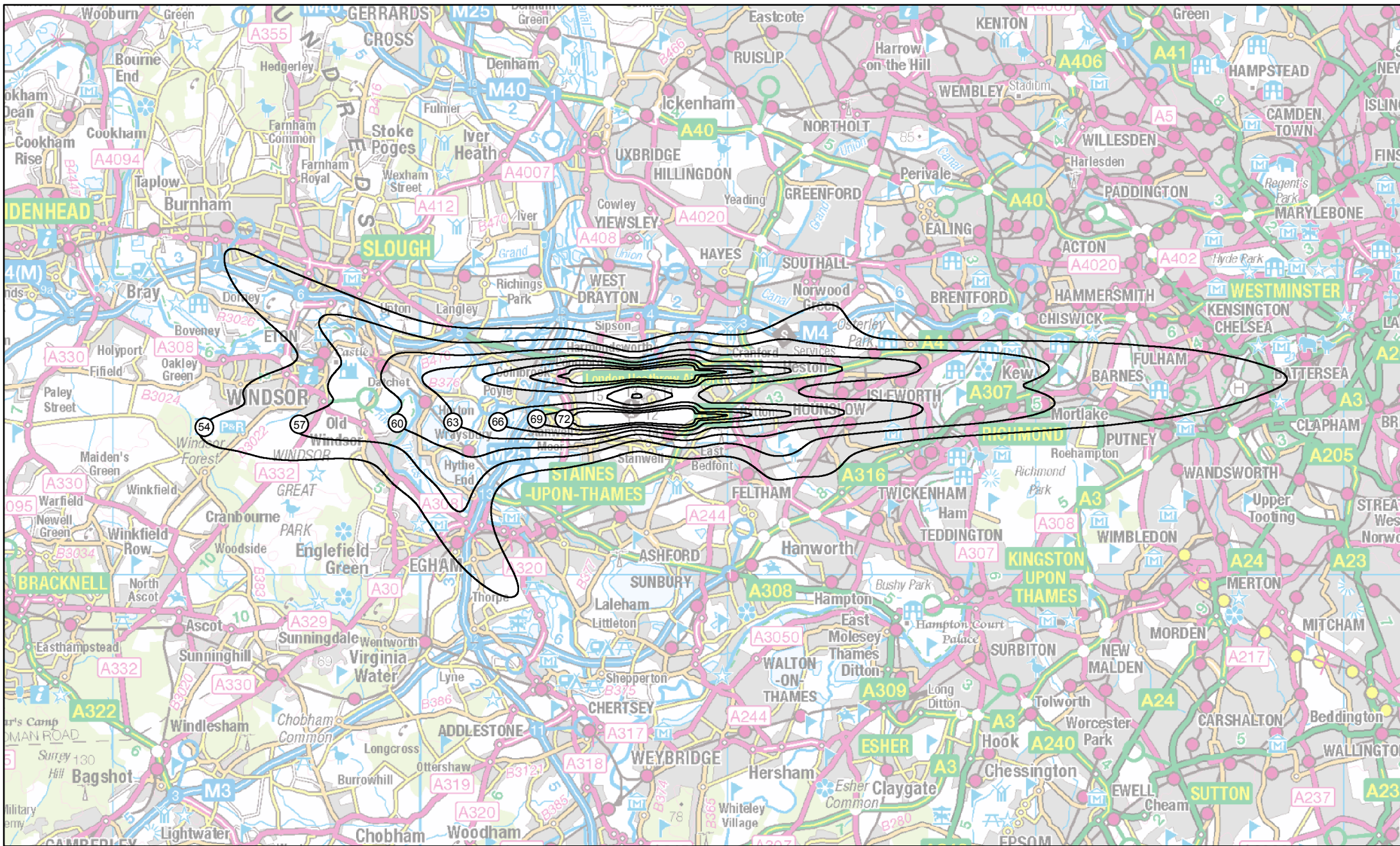
H30-2R-NCT: Heathrow 2030 do-minimum, Need Carbon Traded Summer average 16-hour daytime LAeq,16h
