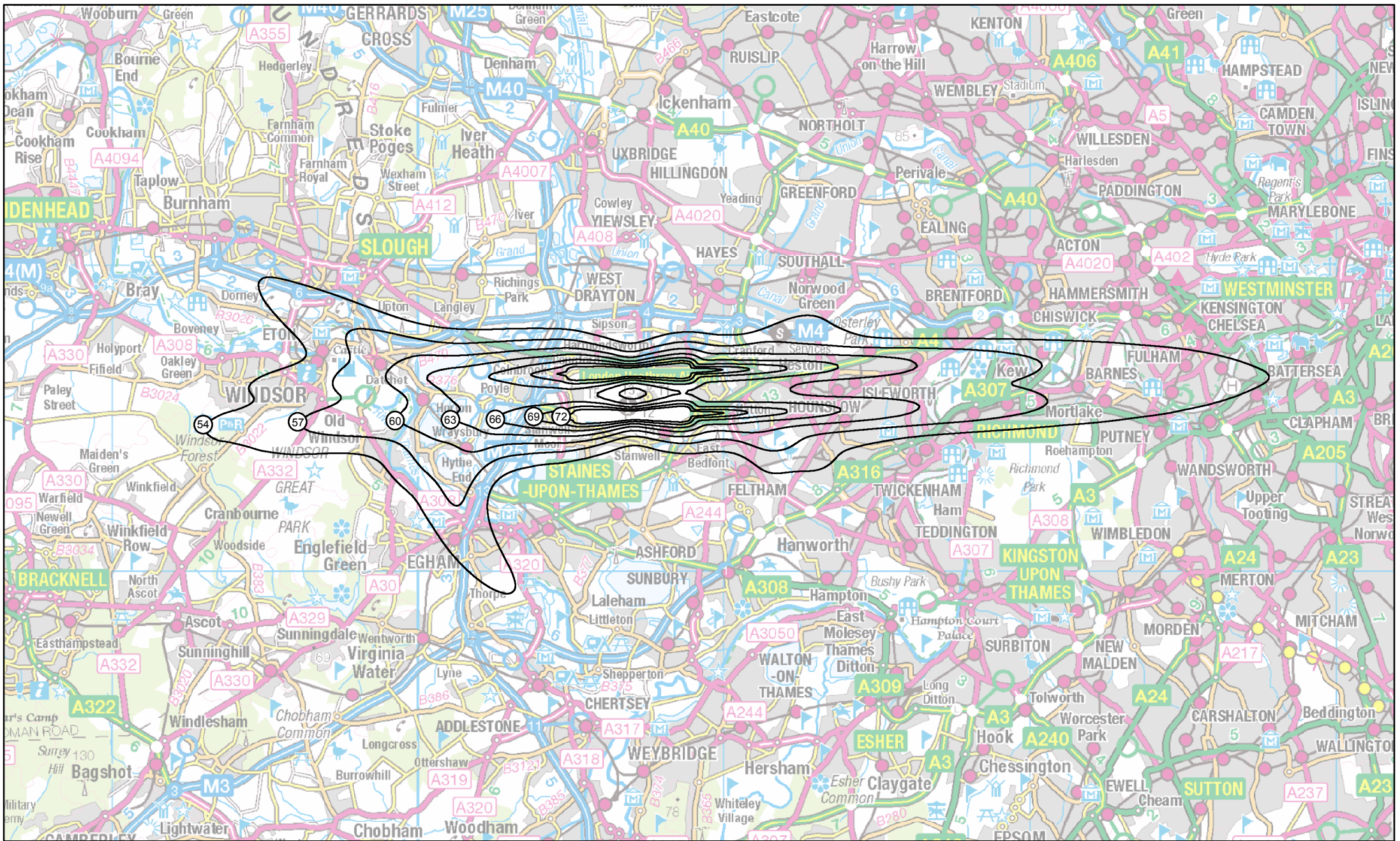
H40-2R-NCT: Heathrow 2040 do-minimum, Need Carbon Traded Summer average 16-hour daytime LAeq,16h
