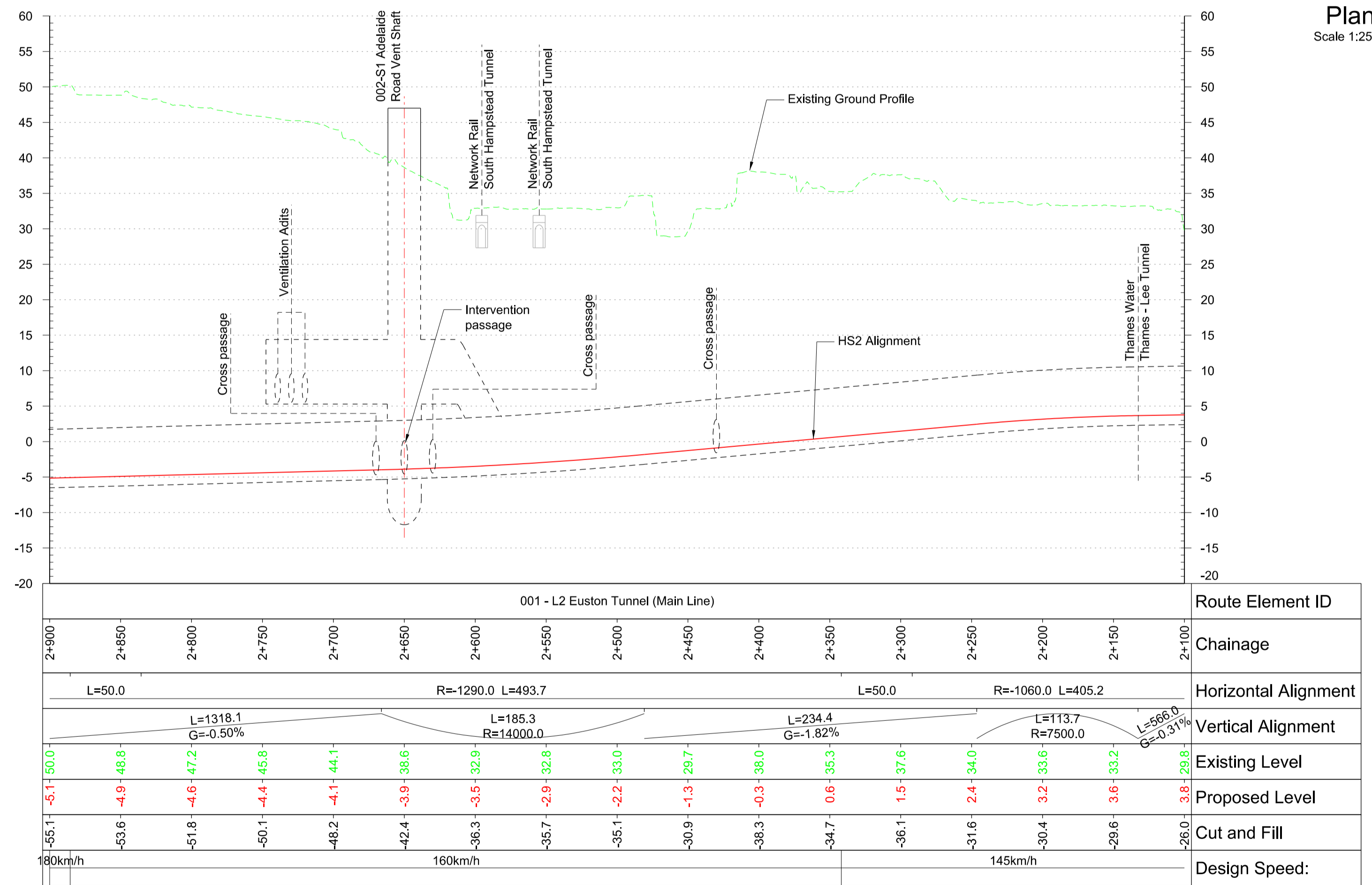
Profile Scale H 1:2500 V 1:500
