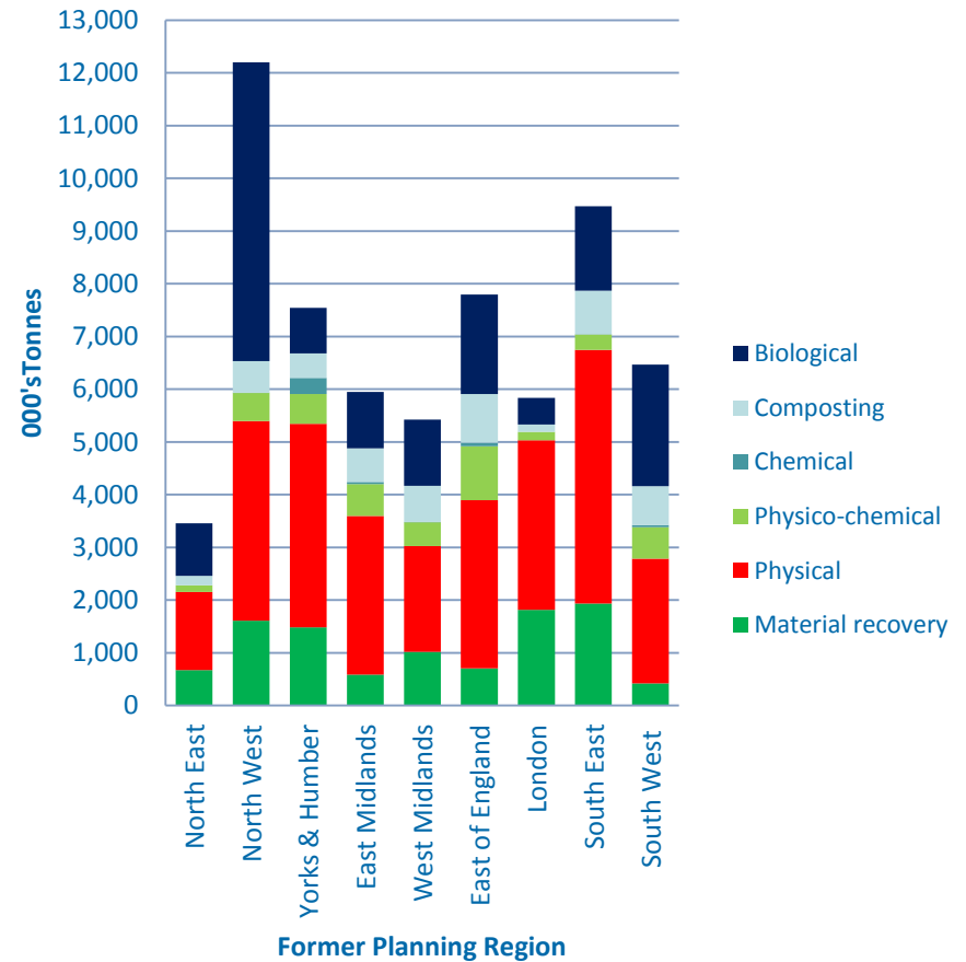
Inputs to treatment facilities by site type England 2015
