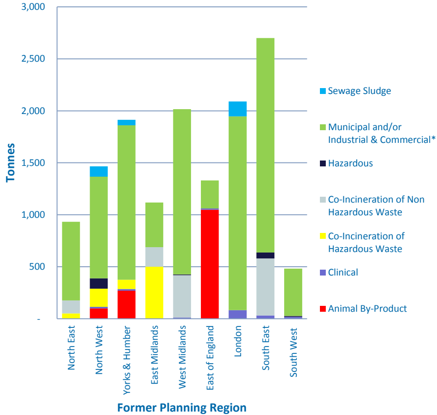
Incineration capacity by type England 2015
