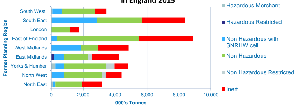
Landfill inputs by site type in England 2015
