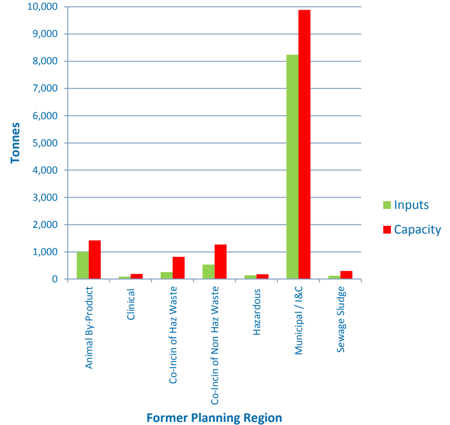
Utilisation of incineration capacity by type in England 2015
