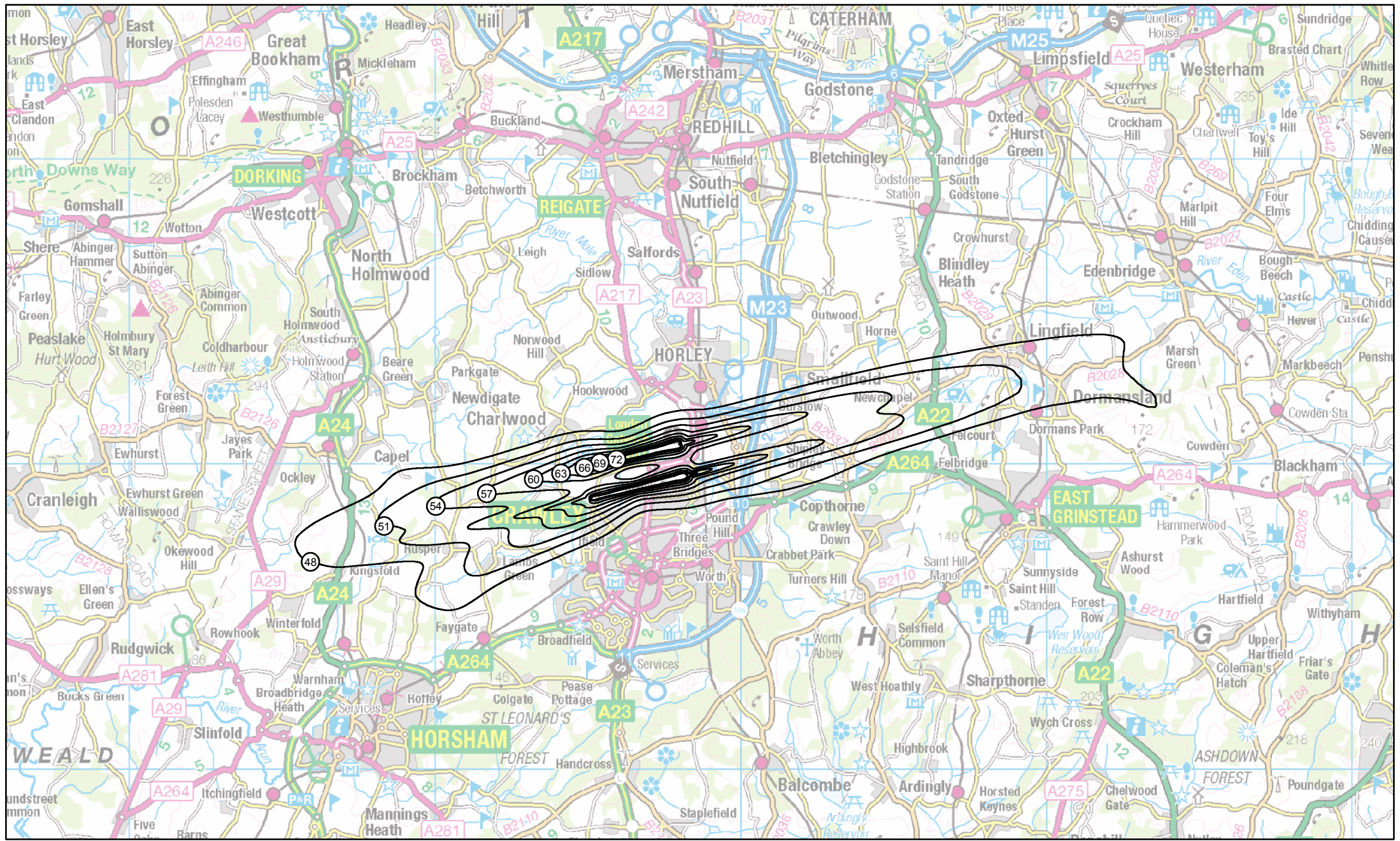
G50-2R-X-NCT: Gatwick 2050 do-something, GAL - Need Carbon Traded Summer average 8-hour night-time LAeq,8h
