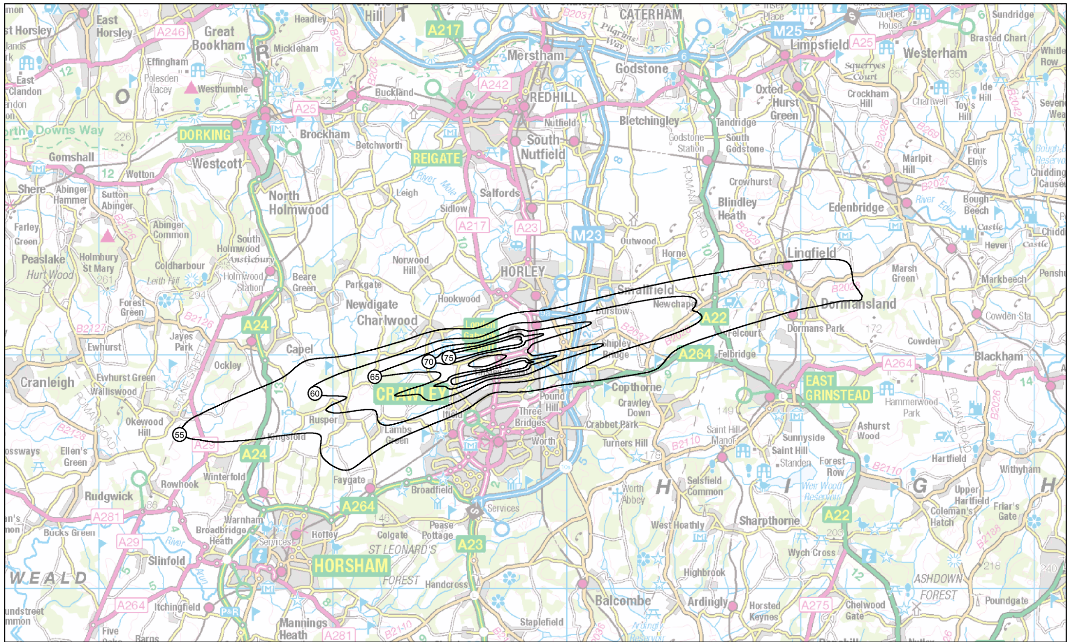
G40-2R-X-NCT: Gatwick 2040 do-something, GAL - Need Carbon Traded Annual average Lden
