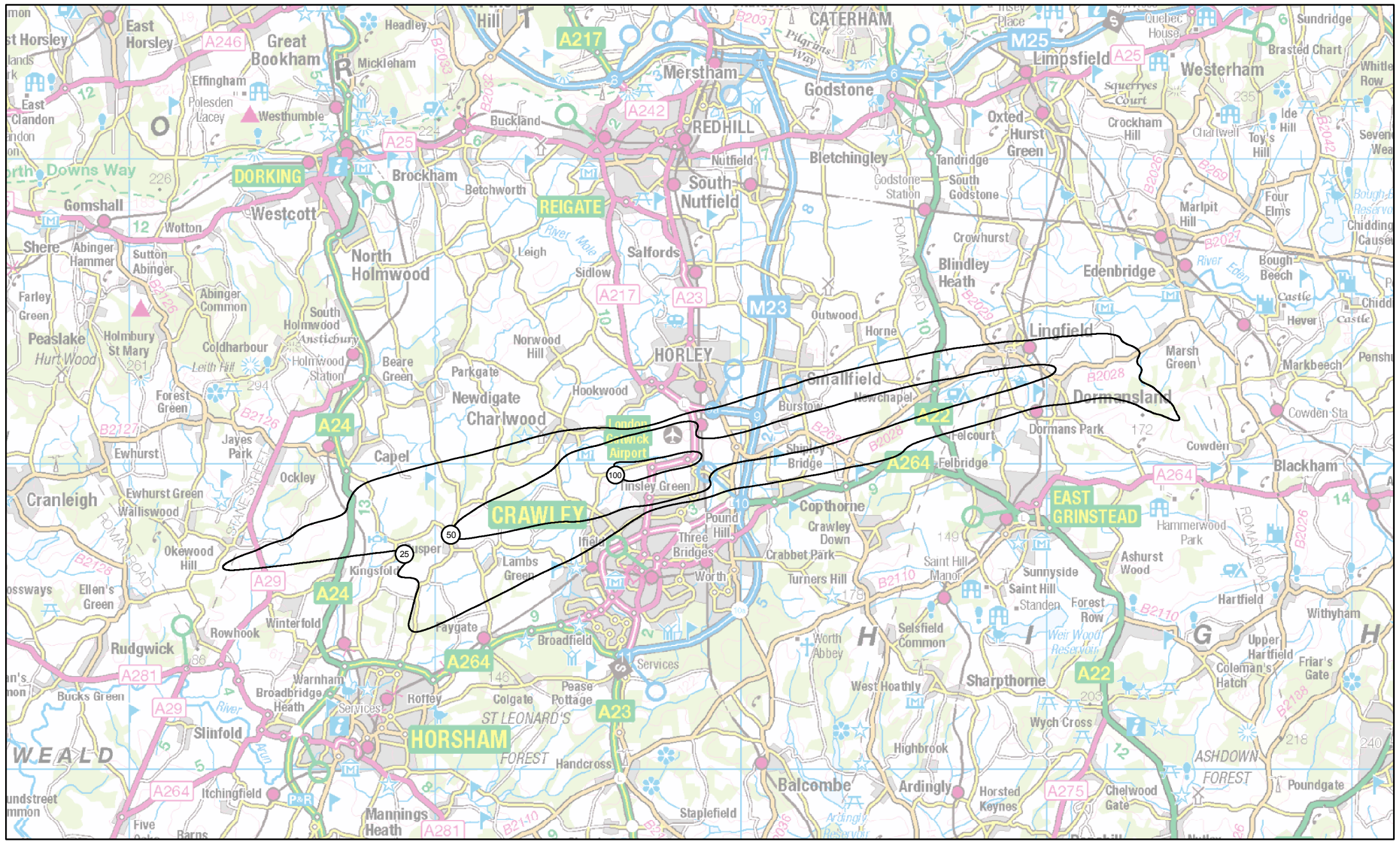
G30-2R-X-NCT: Gatwick 2030 do-something, GAL - Need Carbon Traded Summer average night-time N60
