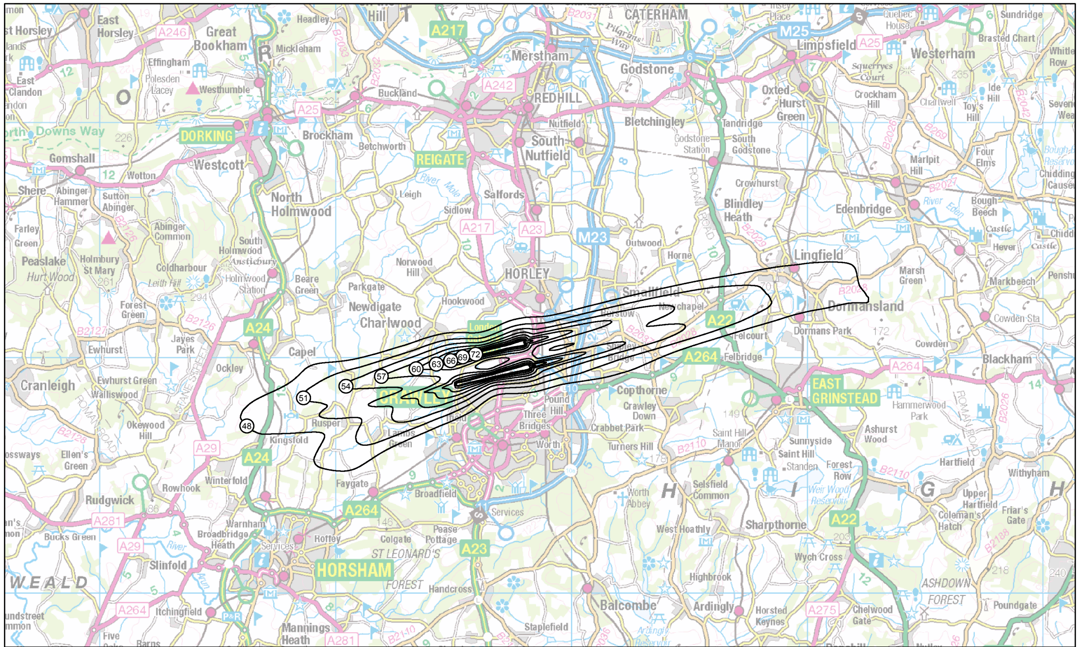
G40-2R-X-NCT: Gatwick 2030 do-something, GAL - Need Carbon Traded Summer average 8-hour night-time LAeq,8h
