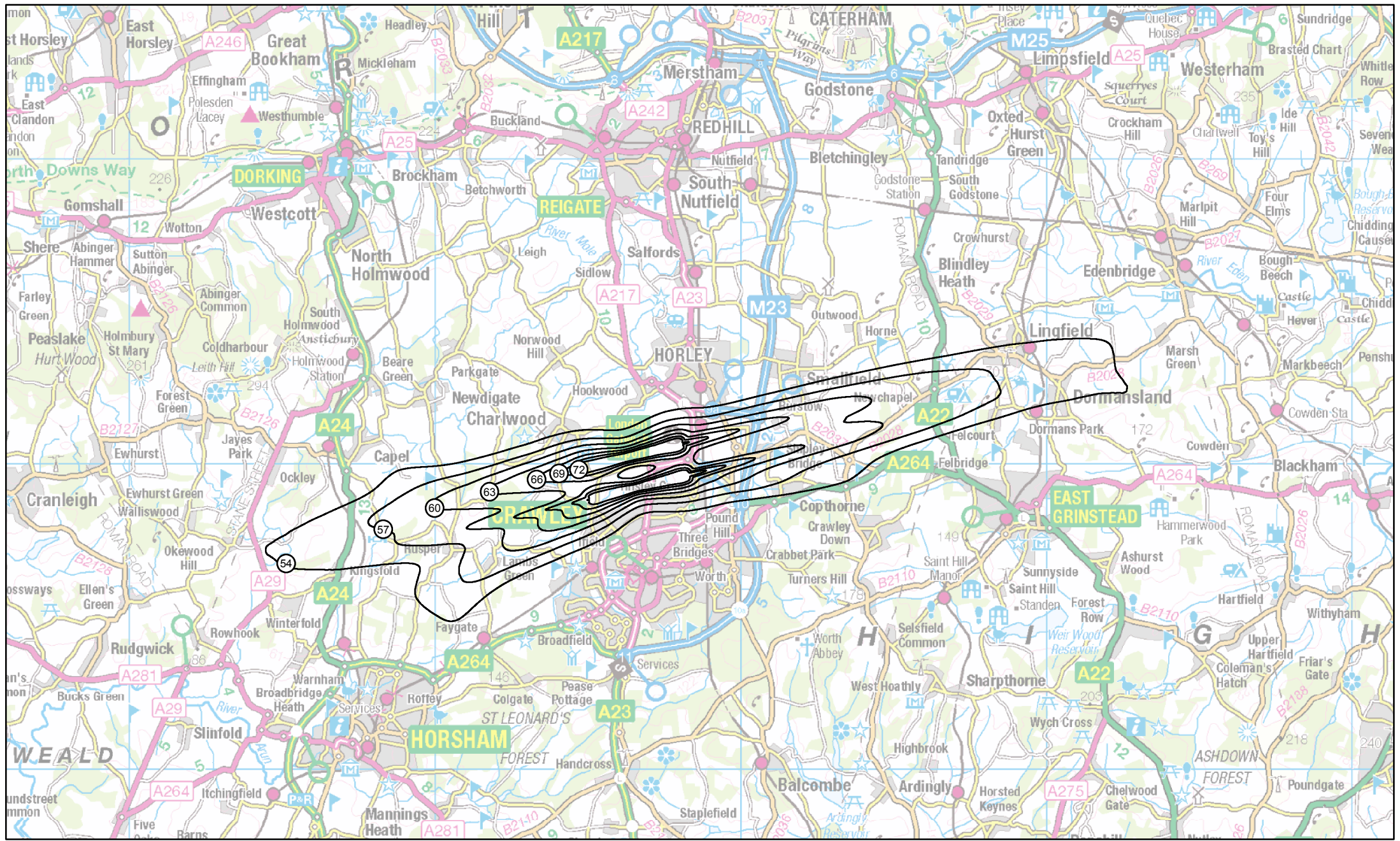
G40-2R-X-NCT: Gatwick 2040 do-something, GAL - Need Carbon Traded Summer average 16-hour daytime LAeq,16h
