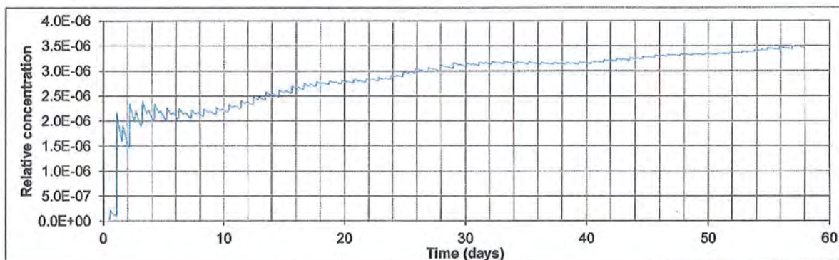
Figure 3.1: Cumulative average relative concentration at 100m from the discharge tower for a daily discharge
