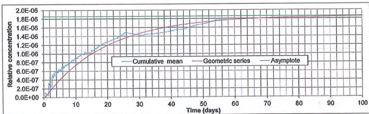
Figure 3.3: Average concentration and extrapolation forward at a point upstream of the discharge tower
