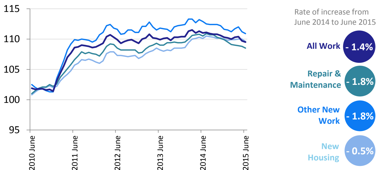
Chart 1: Construction Material Price Indices, UK Index, 2010 = 100
