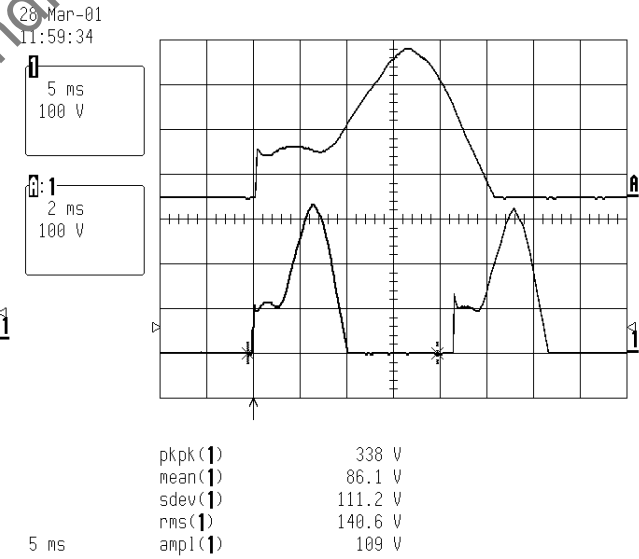
0 Hz No.10 setting 52.6Ω load PBR 200 V 2.5 A
