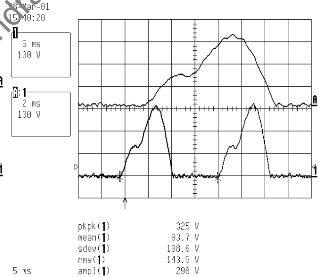
50 Hz Maximum setting 52.6Ω load PBR 230V 0A
