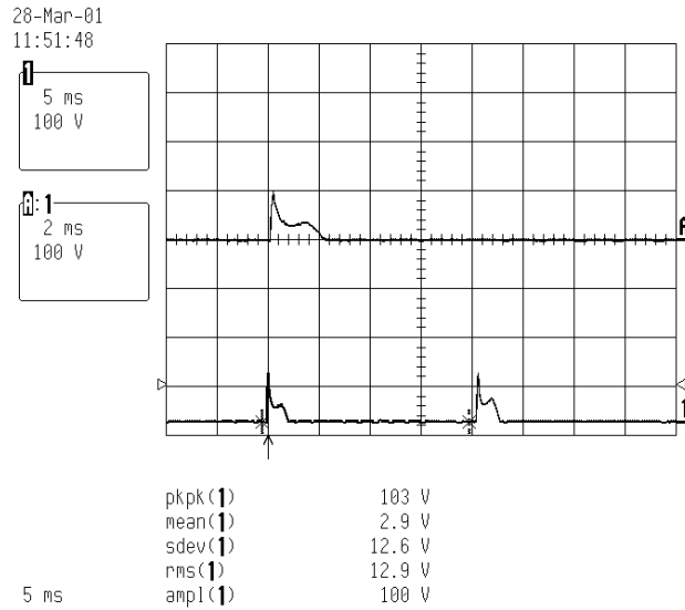
50 Hz No.1 setting 52.6Ω load PBR 200 V No Ammeter reading
