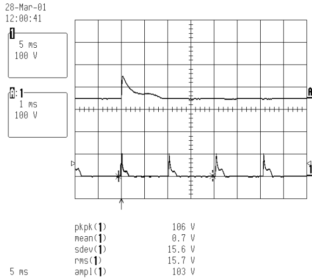
100 Hz No.1 setting 52.6Ω load PBR 200 V No Ammeter reading
