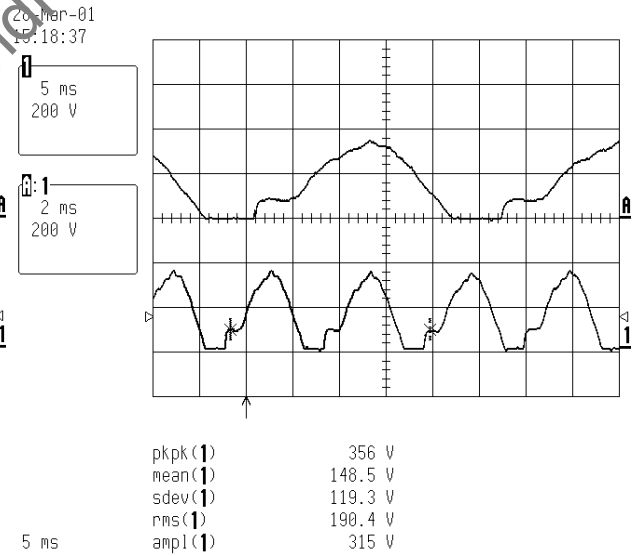
100 Hz 3/4 Maximum setting 52.6Ω load PBR 250V 3.0A
