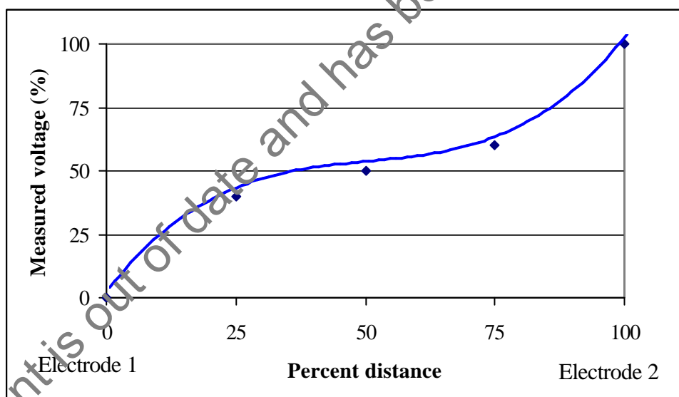
Figure 2.4 Voltage profile obtained from probe A.
