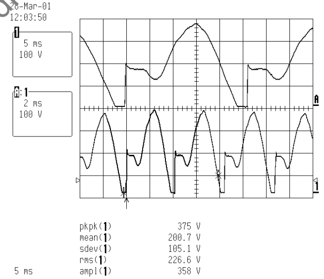
100 Hz No.10 setting 52.6Ω load PBR 200 V 4.0 A
