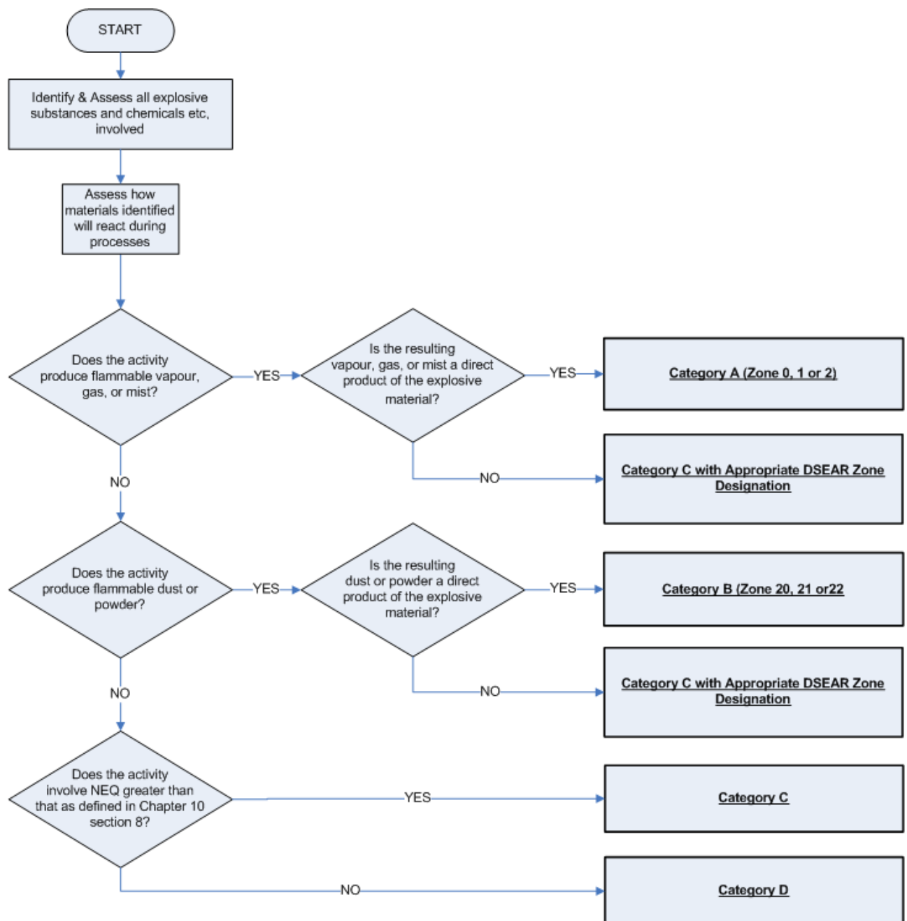
Fig 1 – Electrical Category Selection Algorithm
