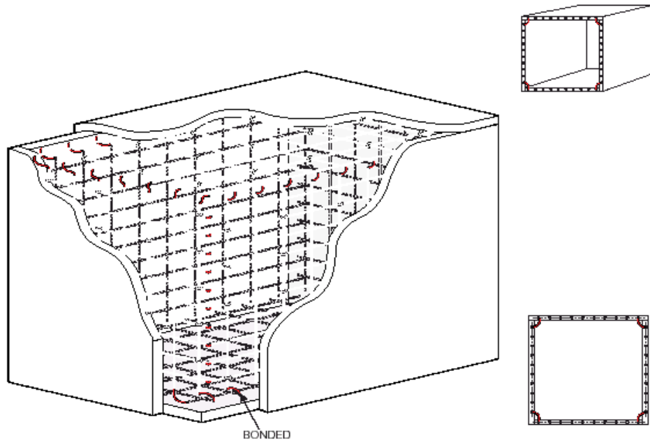
Fig D 11 Reinforced Concrete 'Faraday Cage' Structure
