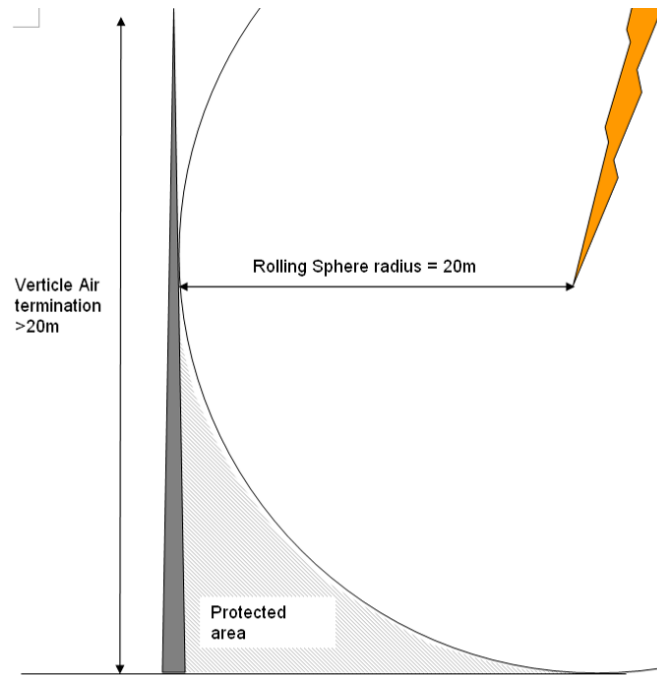
Fig D 3 20m Rolling Sphere Principle - 20m or Higher structure
