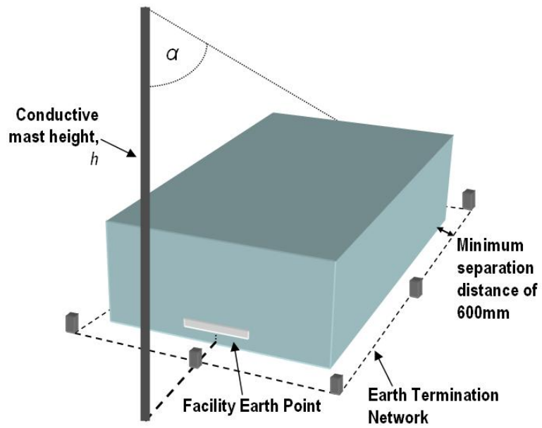
Angle \alpha varies with height h – see BS EN 62305 Part 3 Table 2
