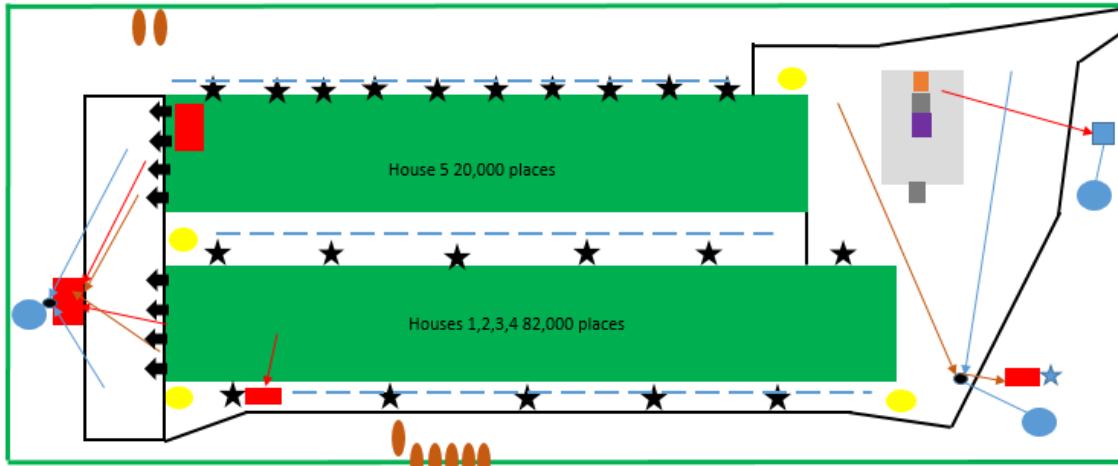
Steep Marsh Layout Drainage Plan
