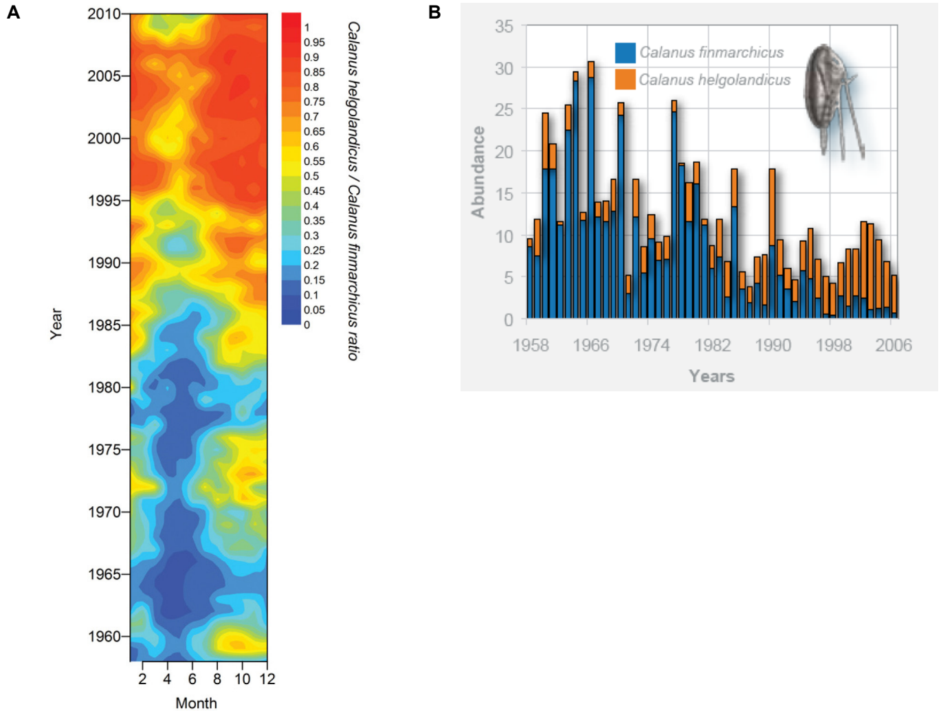
Figure A1a.4 – ratio of C. finmarchicus and C. helgolandicus abundances in the North Sea between A: 1958-2010 (by month); B: 1958-2006.
