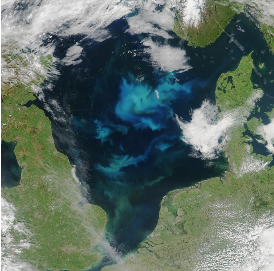
Figure A1a.2: Satellite image of a plankton bloom in the North Sea in 2015
