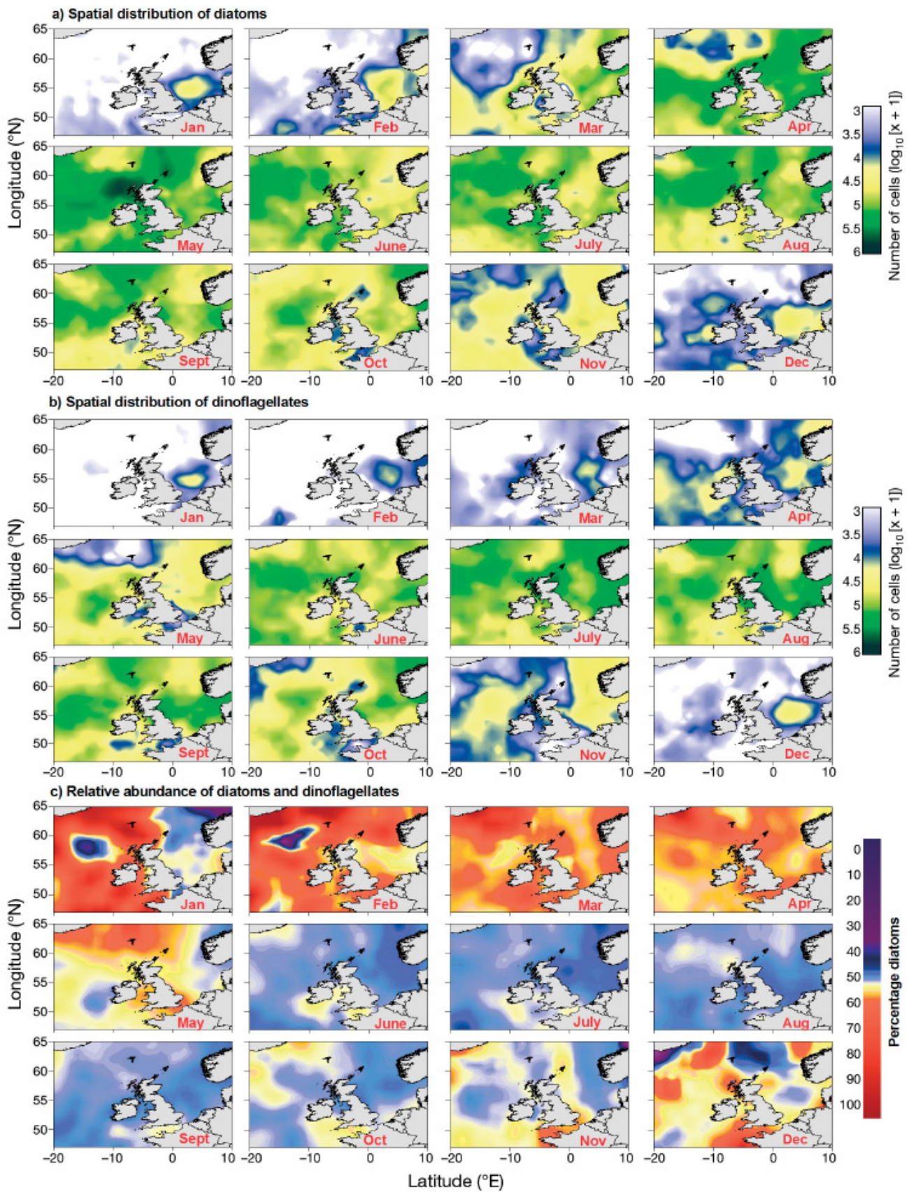
Figure A1a.1: Mean monthly spatial patterns of (a) diatoms, (b) dinoflagellates and (c) their relative community abundances (as percentage diatoms) in NE Atlantic between 1958-2003.
