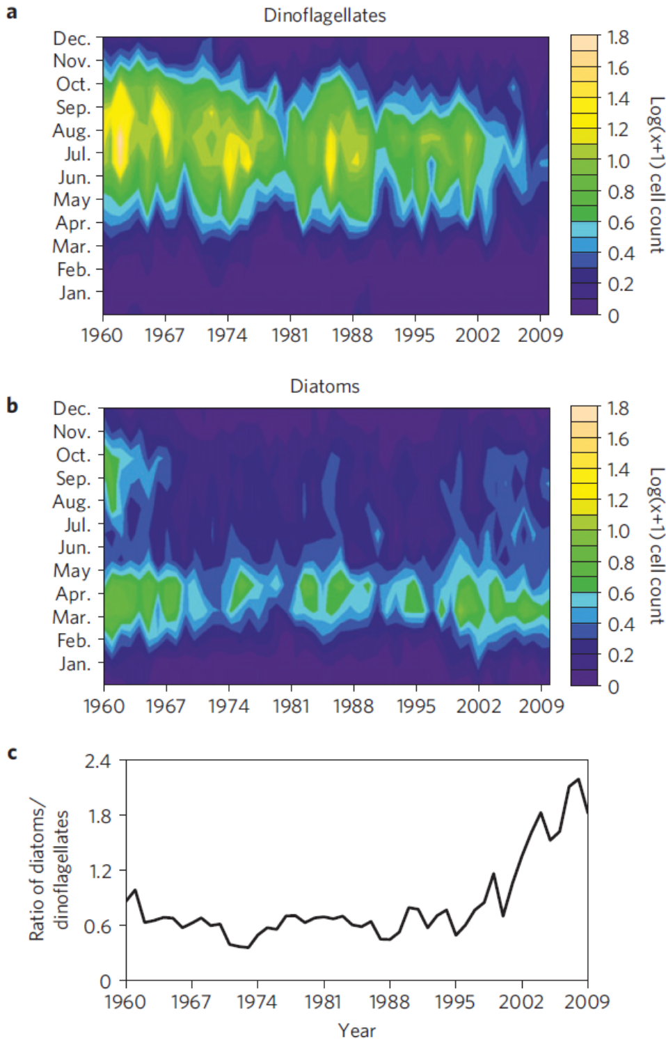
Figure A1a.3: Ratio of dinoflagellate and diatom abundance in the north-east Atlantic, 1950-2009
