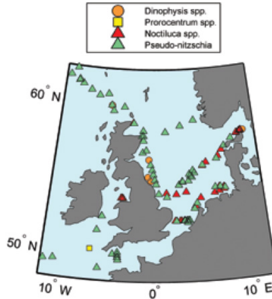
Figure A1a.5: Occurrences of large blooms in UK and northern European waters in 2012
