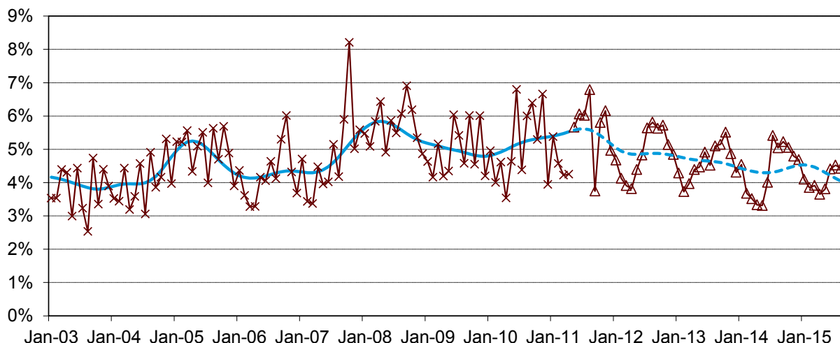
Figure 1: Herd incidence of bovine TB (bTB) in GB: number of new incidents of bTB leading to the withdrawal of officially TB free (OTF) herd status, as a percentage of tests carried out in OTF herds each month since 2003:
