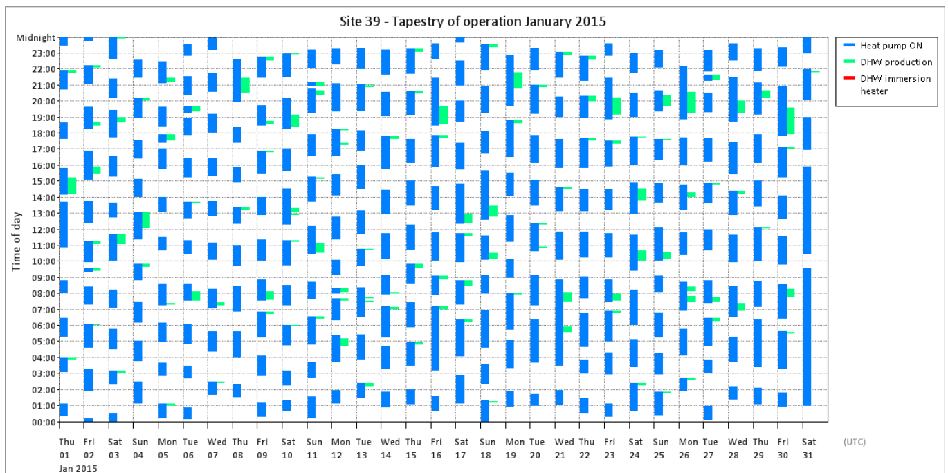
Figure T 103 – Site 39apestries of operation
