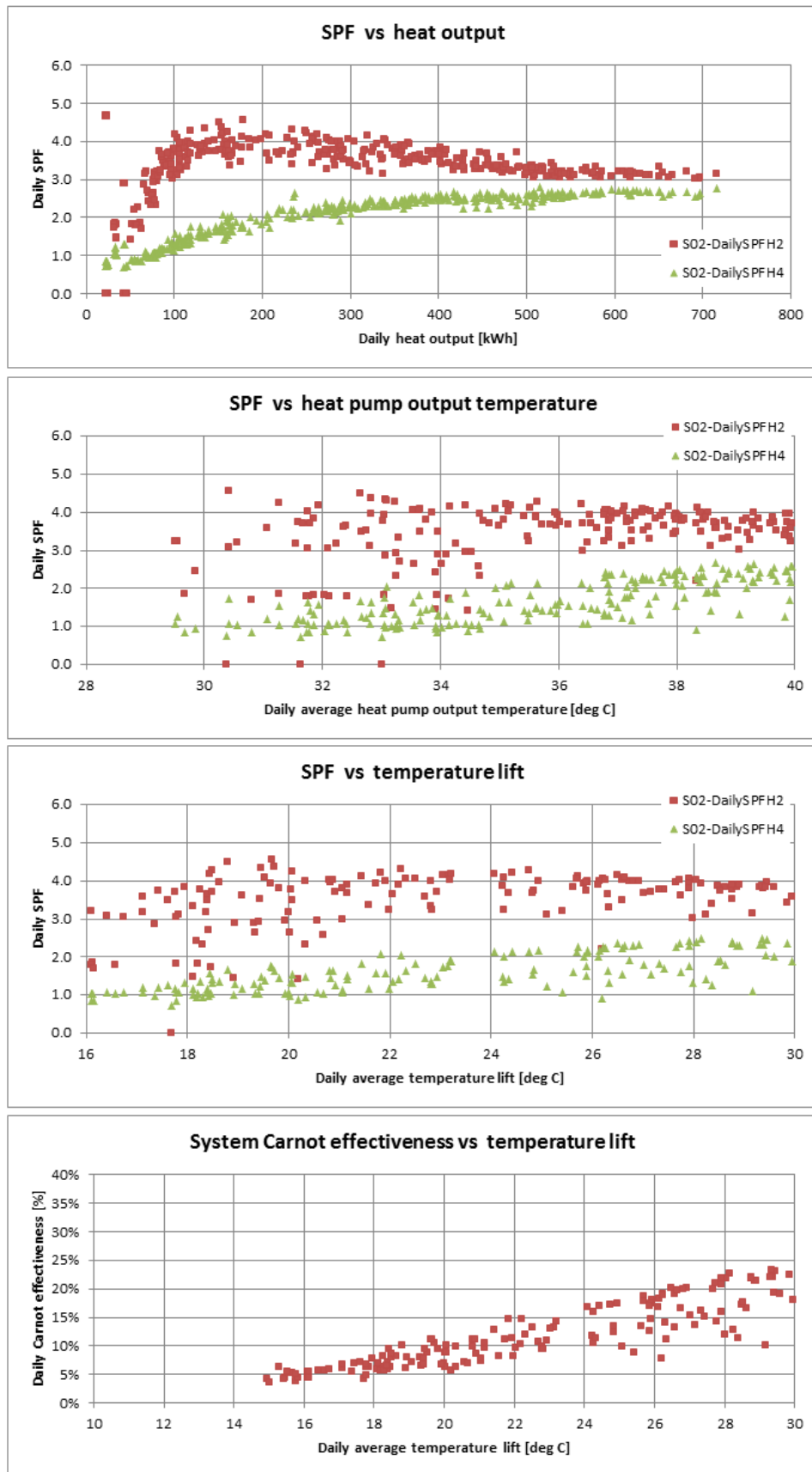
Figure T 32 – Site 02 system efficiency charts (2)
