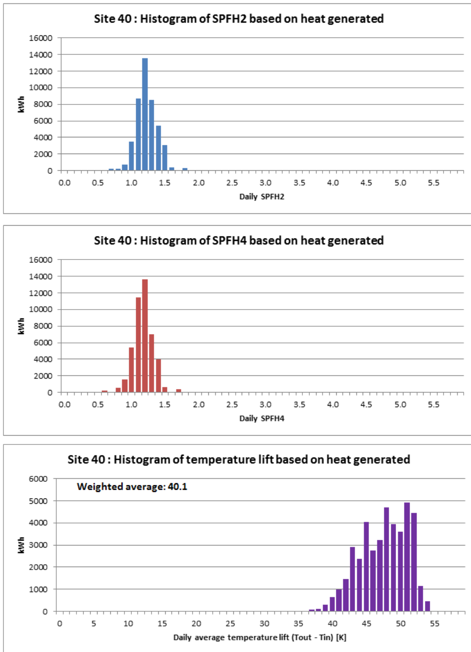
Figure T 160 – Site 40 histograms of SPF H2 , SPF H4 and temperature lift
