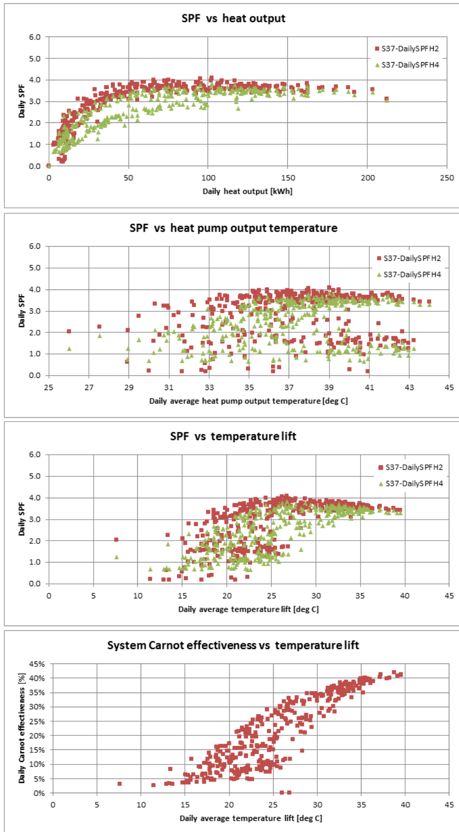
Figure T 64 – Site 37 system efficiency charts (2)
