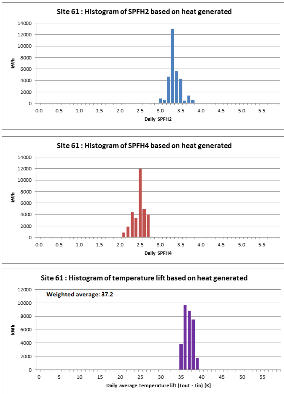
Figure T 167 – Site 61 histograms of SPF H2 , SPF H4 and temperature lift
