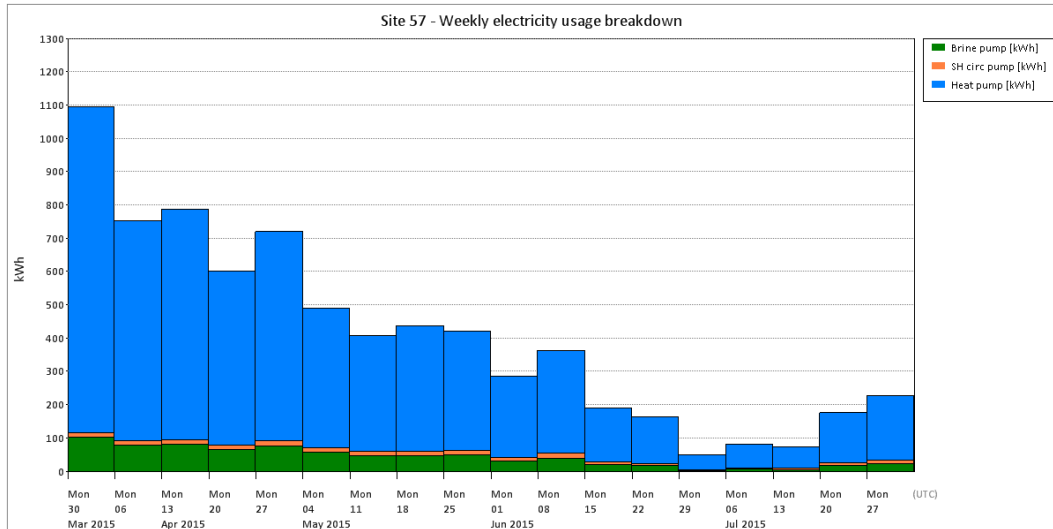
Figure T 186 – Site 57 electricity breakdown
