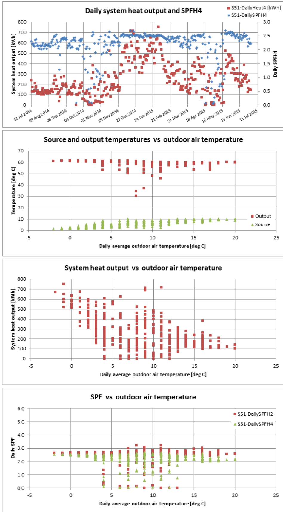
Figure T 71 – Site 51 system efficiency charts (1)
