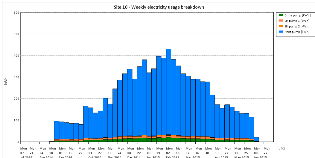
Figure T 173 – Site 10 electricity breakdown
