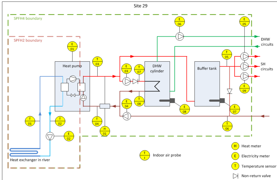
Figure T 13 – Site 29 system schematic
