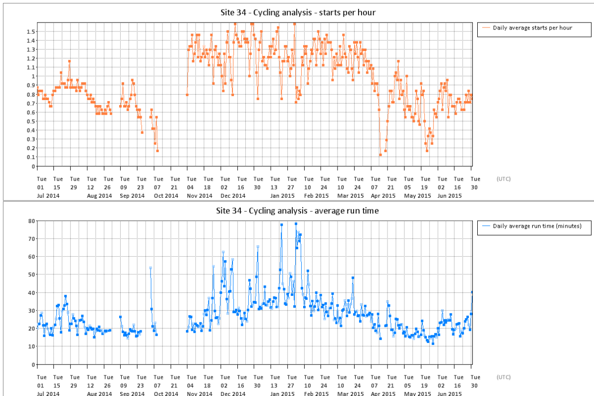
Figure T 128 – Site 34 cycling analysis
