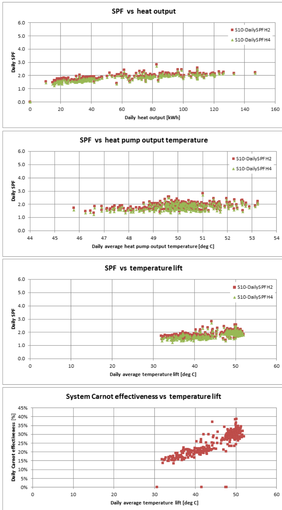
Figure T 40 – Site 10 system efficiency charts (2)
