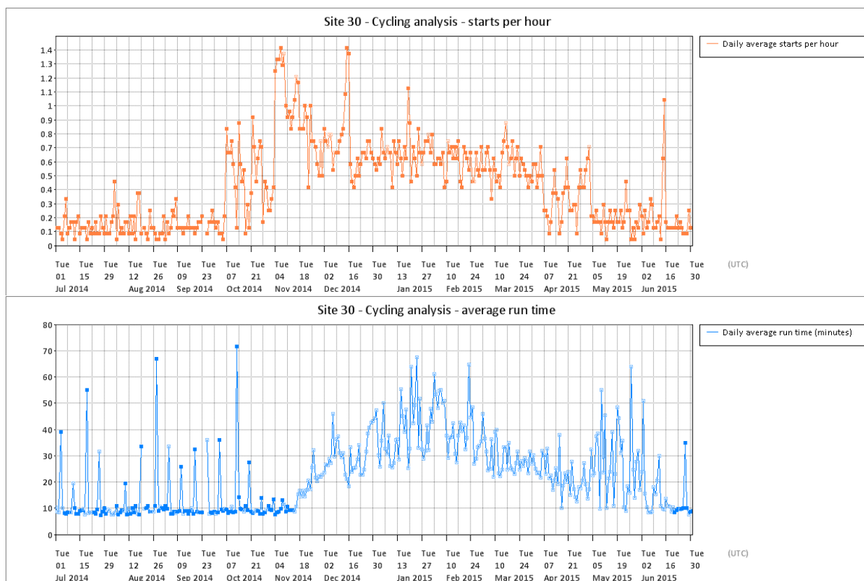
Figure T 126 – Site 30 cycling analysis
