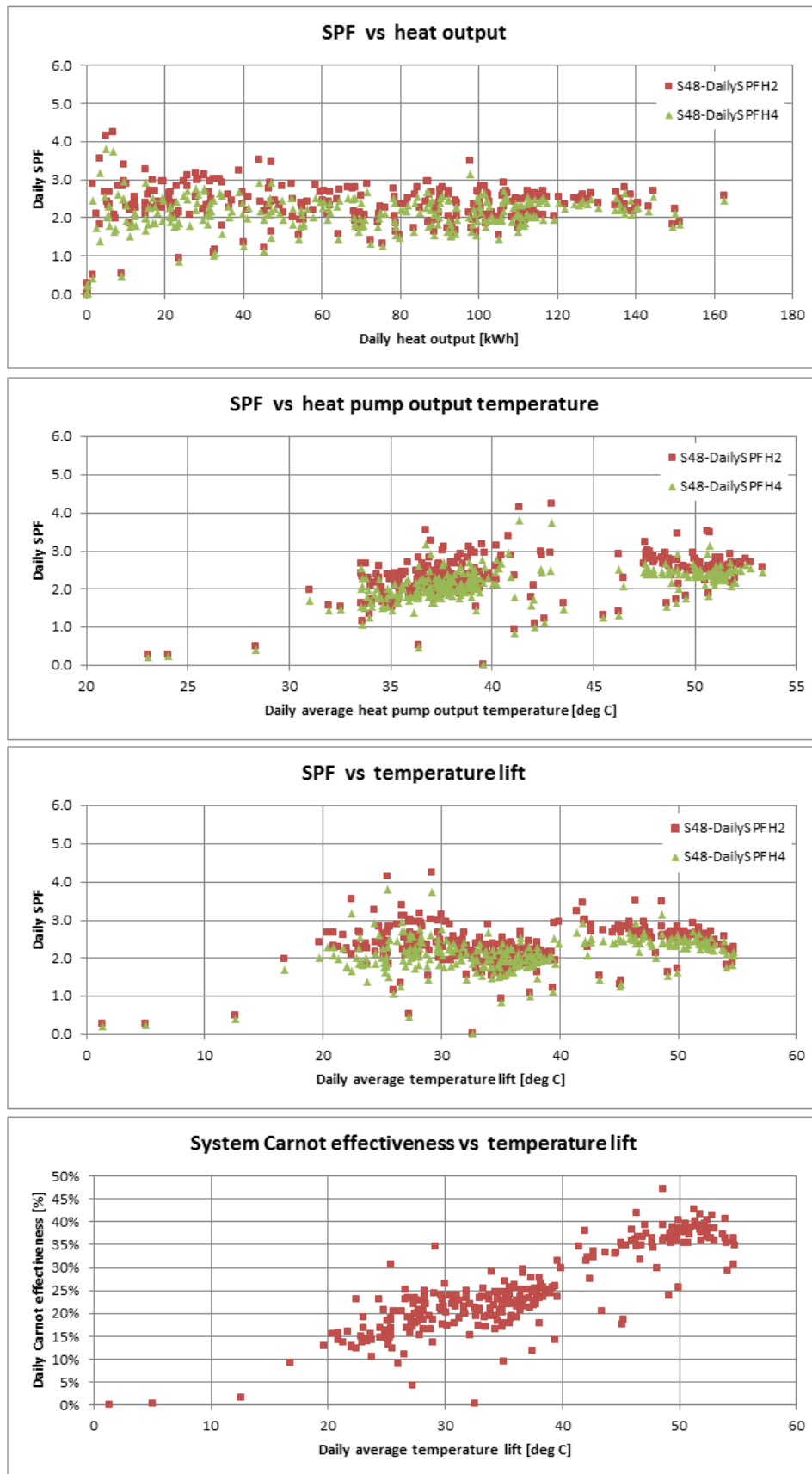
Figure T 70 – Site 48 system efficiency charts (2)
