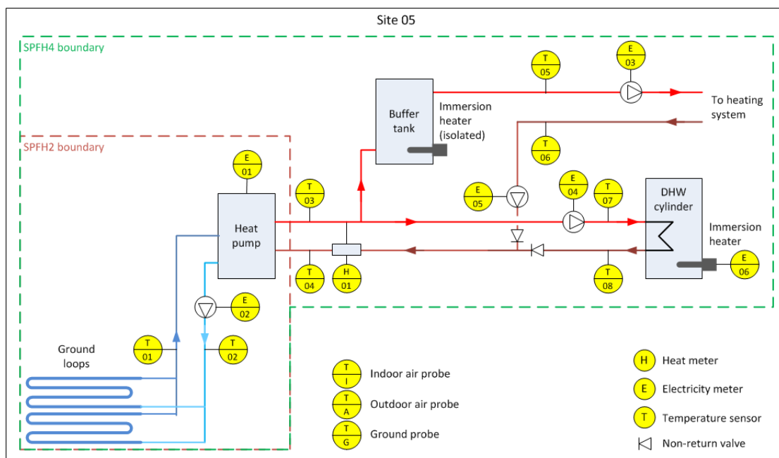
Figure T 4 – Site 05 system schematic
