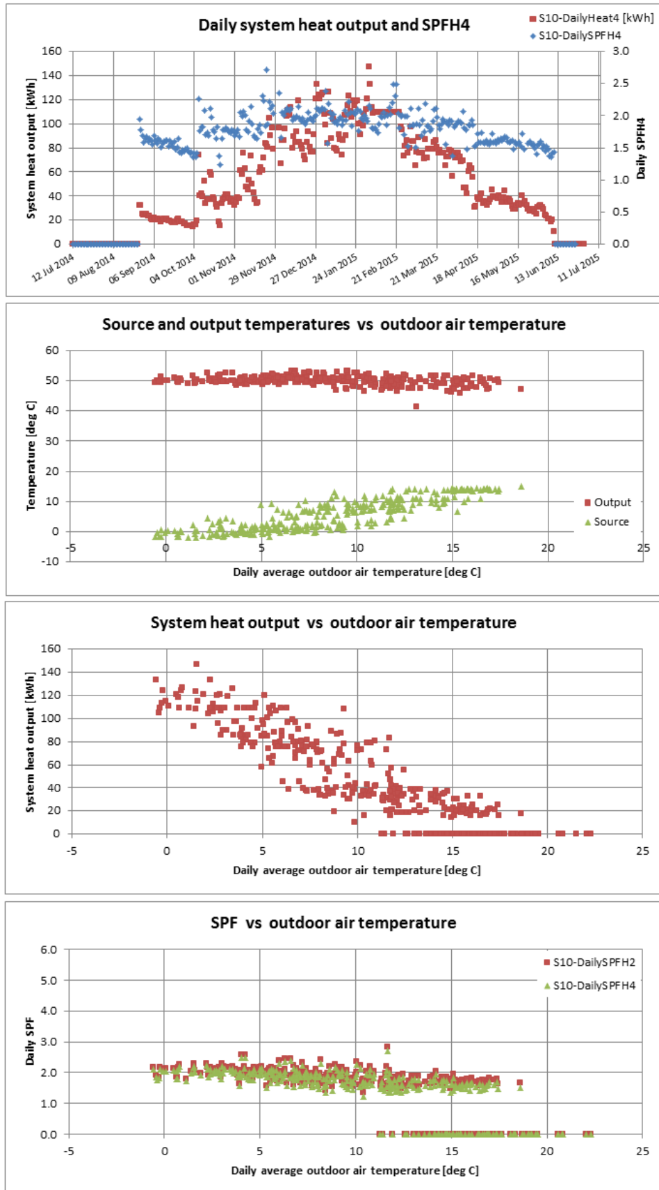
Figure T 39 – Site 10 system efficiency charts (1)
