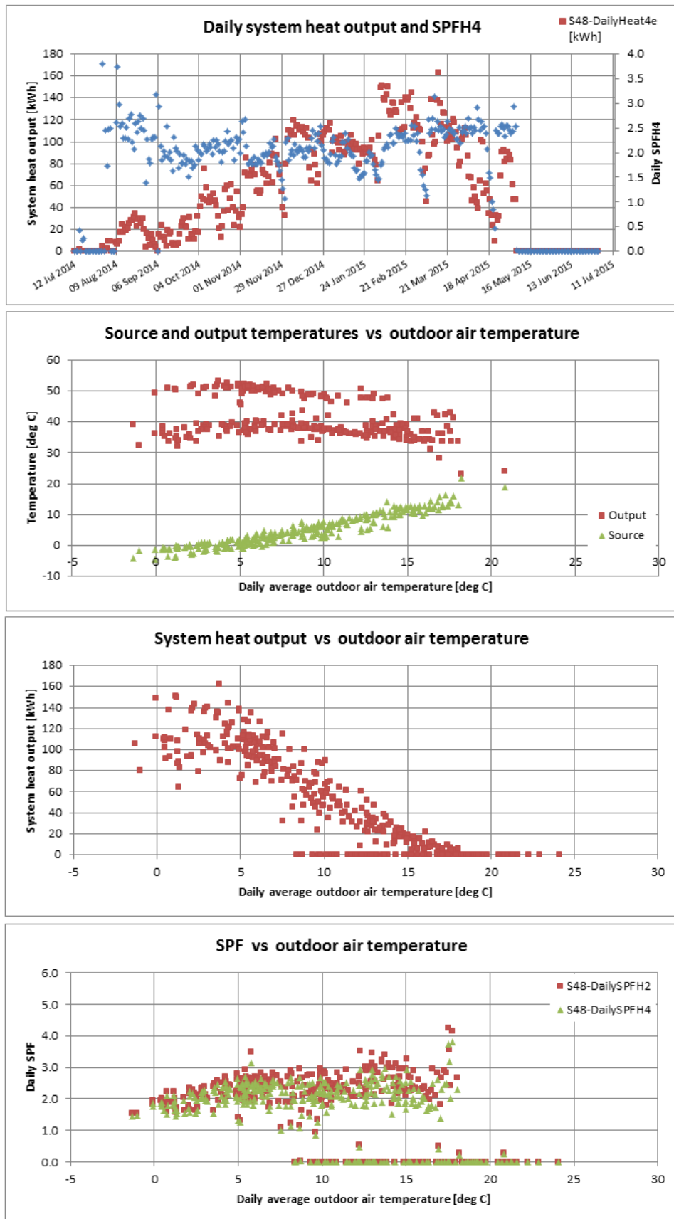
Figure T 69 – Site 48 system efficiency charts (1)
