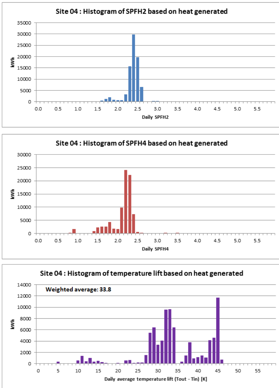
Figure T 143 – Site 04 histograms of SPF H2 , SPF H4 and temperature lift
