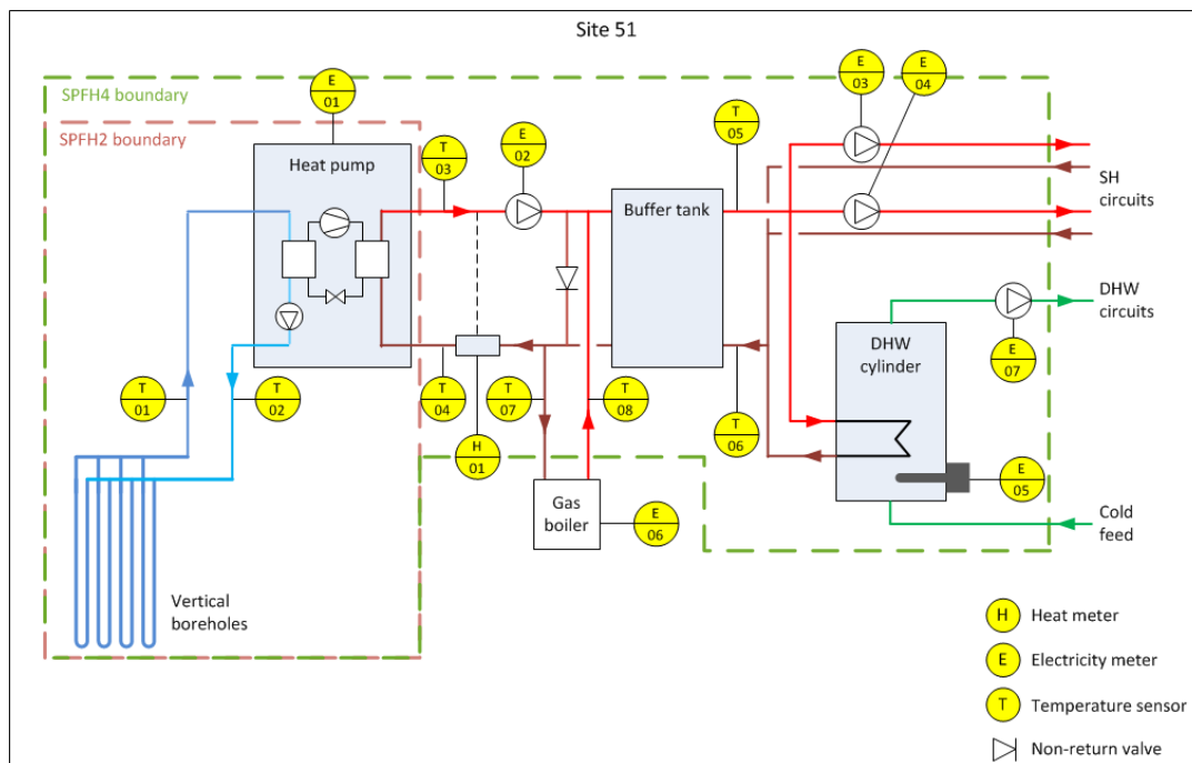
Figure T 23 – Site 51 system schematic
