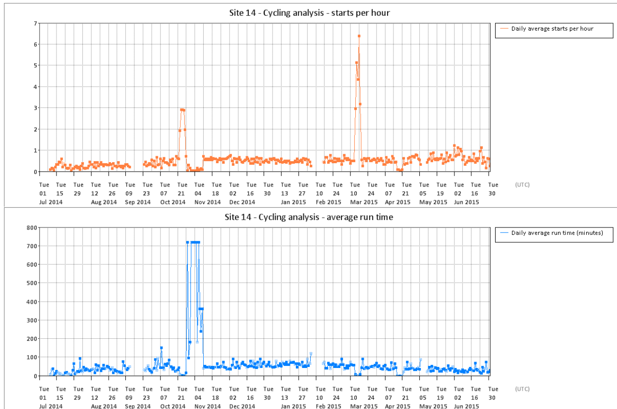
Figure T 120 – Site 14 cycling analysis
