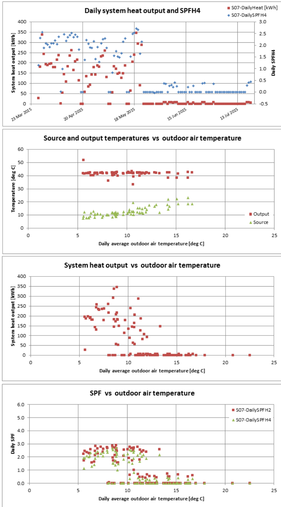
Figure T 37 – Site 07 system efficiency charts (1)
