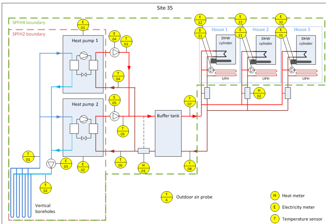
Figure T 17 – Site 35 system schematic
