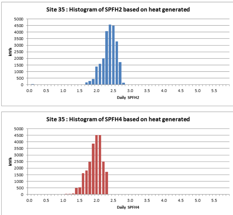
Figure T 157 – Site 35 histograms of SPF H2 , SPF H4 and temperature lift
