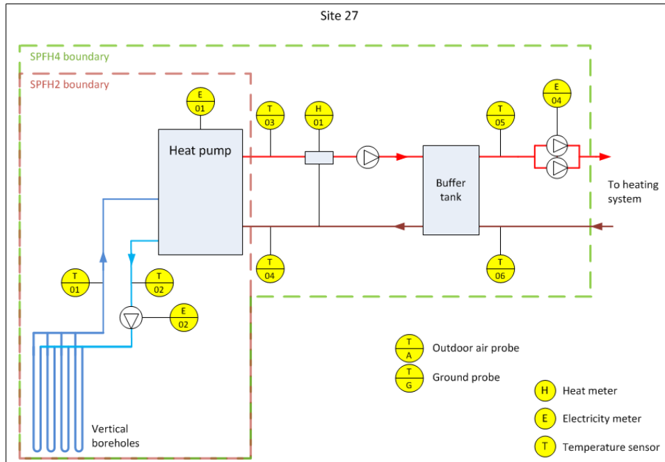
Figure T 11 – Site 27 system schematic
