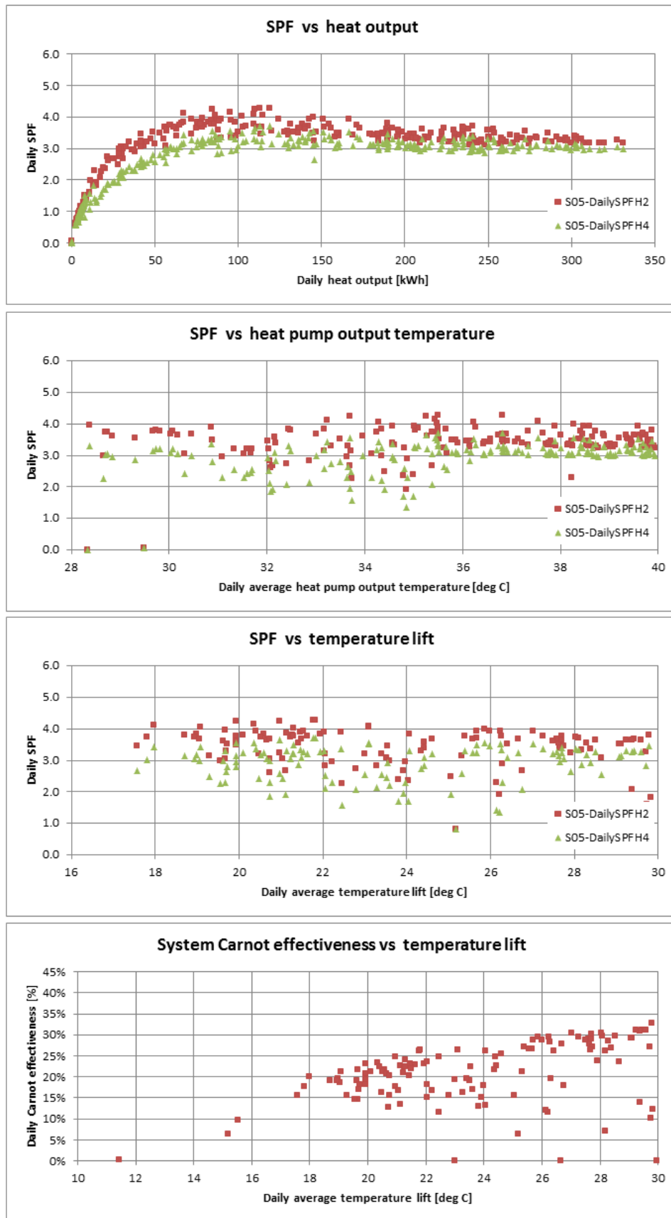
Figure T 36 – Site 05 system efficiency charts (2)
