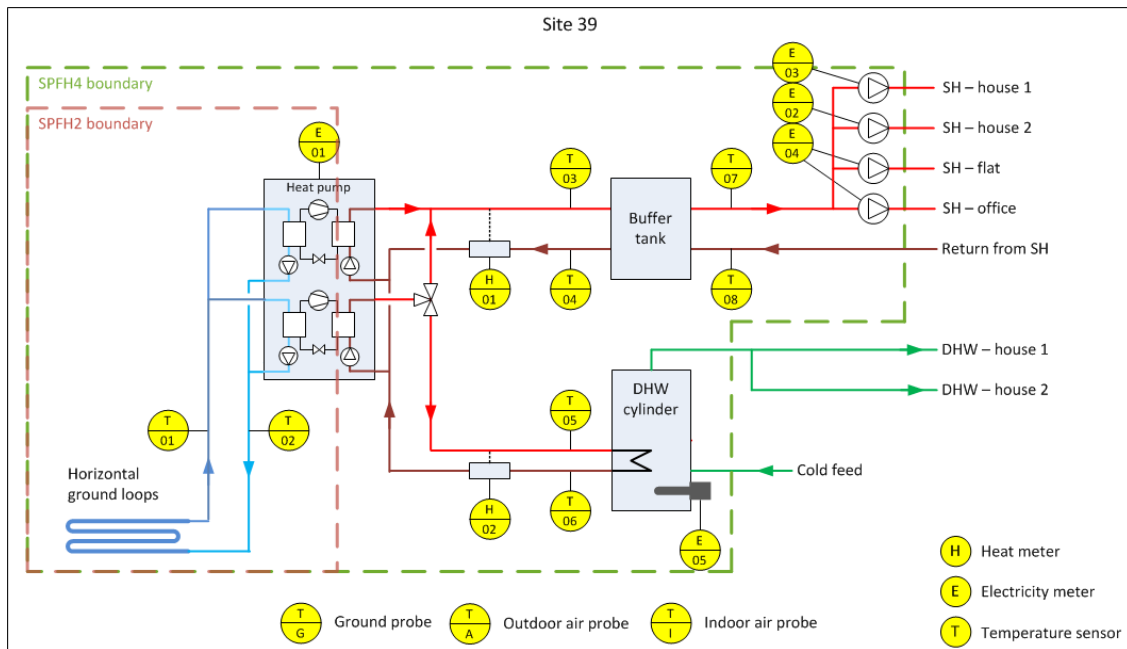
Figure T 19 – Site 39 system schematic
