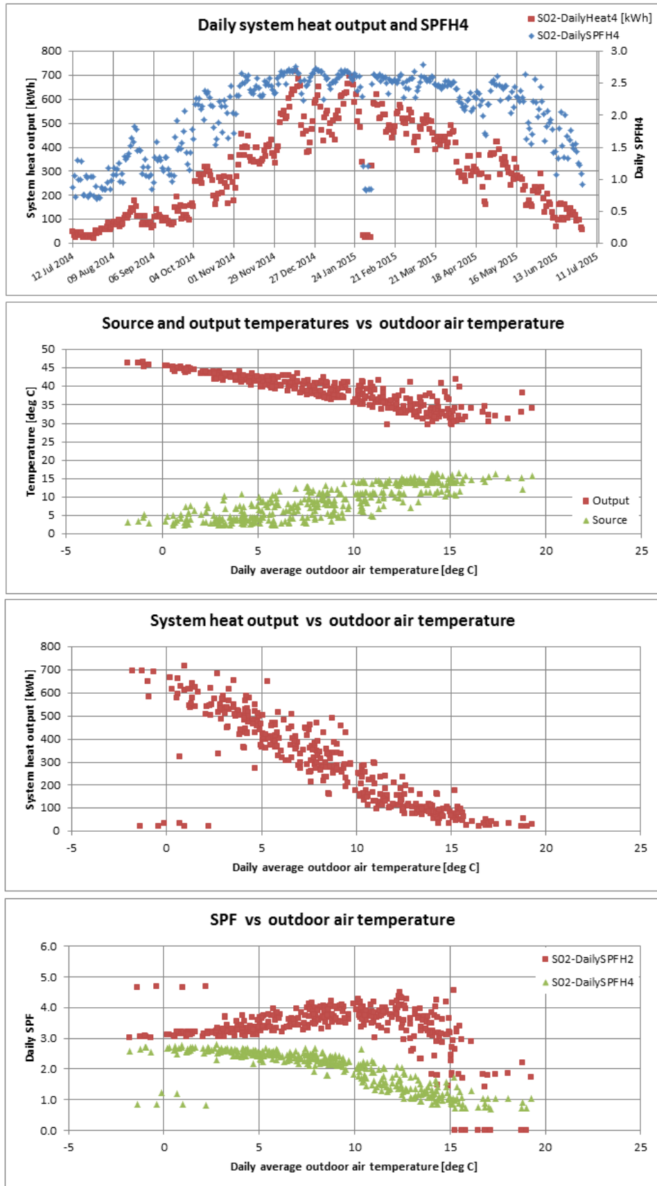
Figure T 31 – Site 02 system efficiency charts (1)
