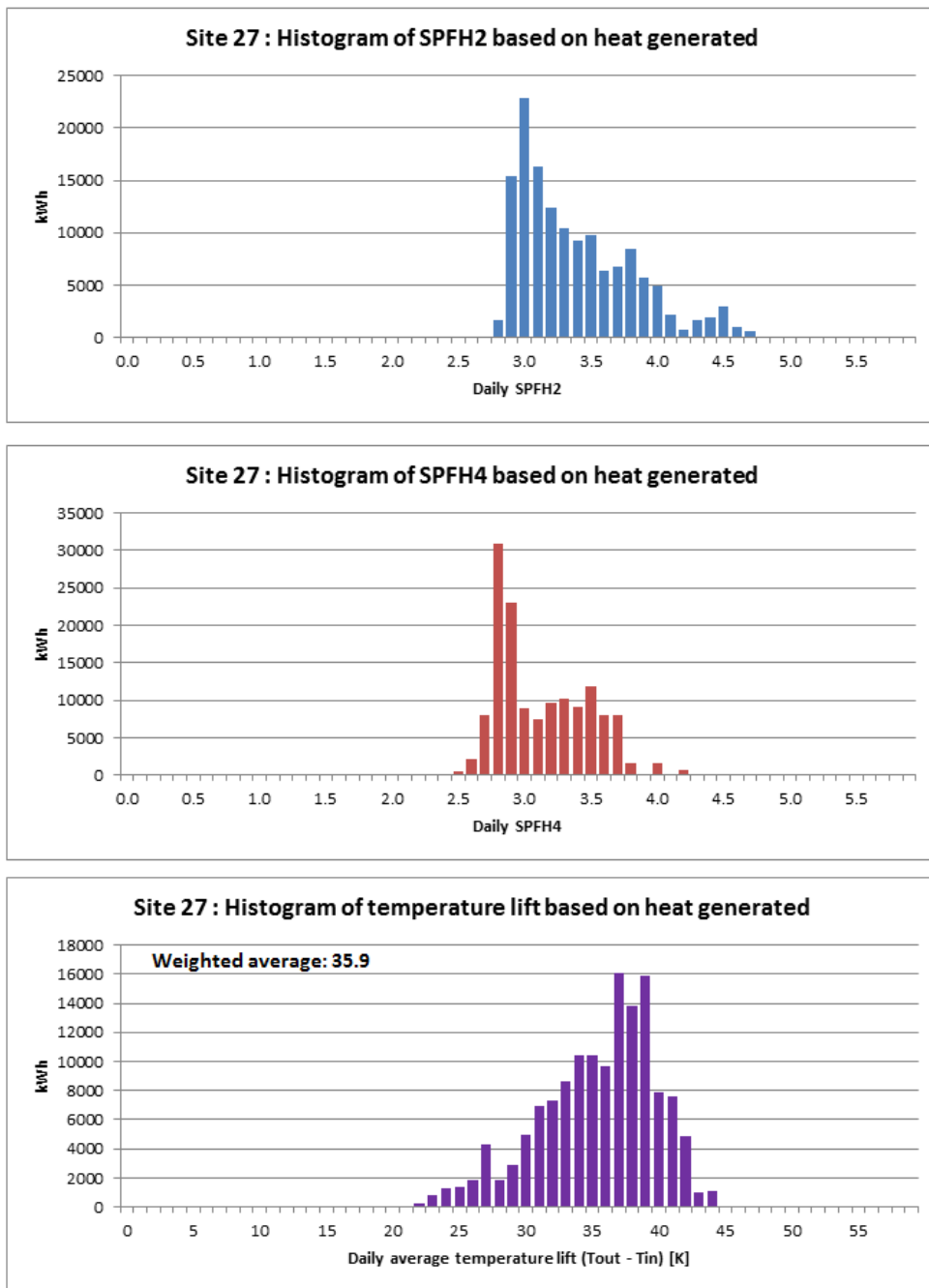
Figure T 151 – Site 27 histograms of SPF H2 , SPF H4 and temperature lift
