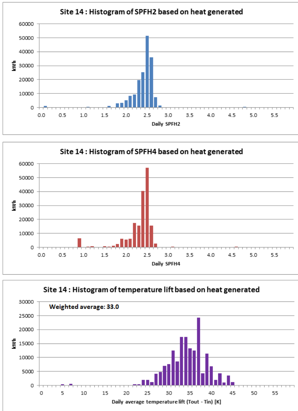
Figure T 148 – Site 14 histograms of SPF H2 , SPF H4 and temperature lift
