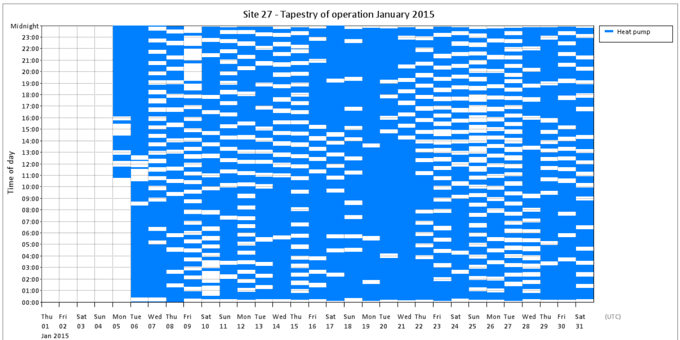
Figure T 95 – Site 27 tapestries of operation
