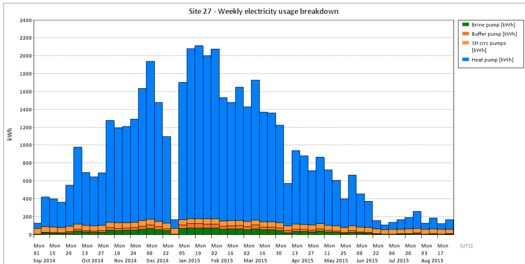
Figure T 178 – Site 27 electricity breakdown
