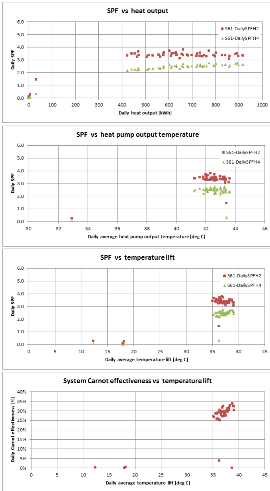
Figure T 82 – Site 61 system efficiency charts (2)
