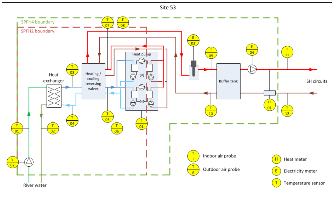
Figure T 24 – Site 53 system schematic
