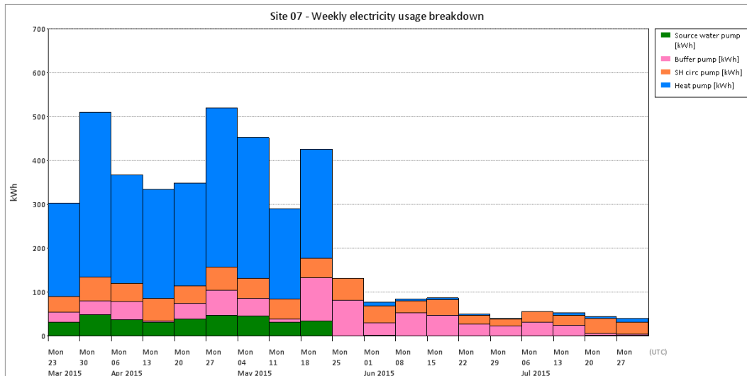
Figure T 172 – Site 07 electricity breakdown
