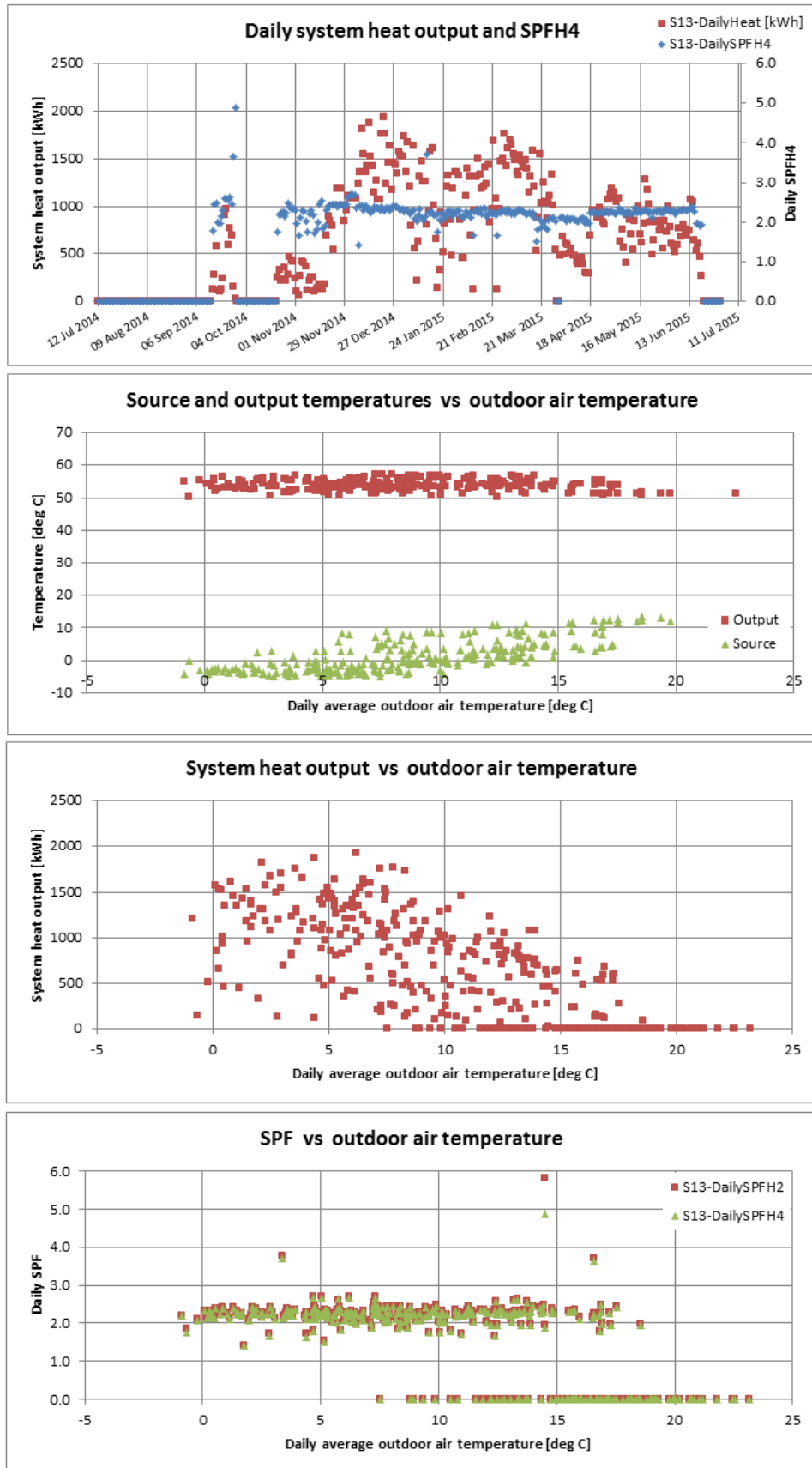
Figure T 41 – Site 13 system efficiency charts (1)
