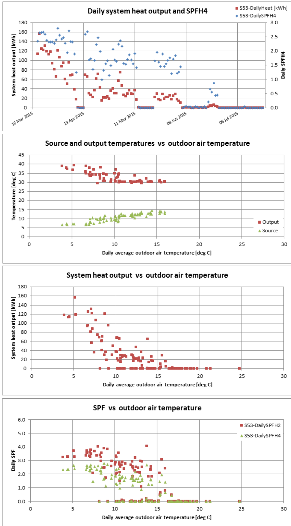
Figure T 73 – Site 53 system efficiency charts (1)
