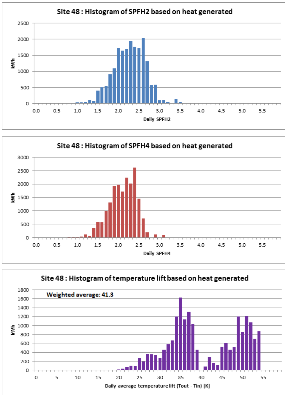
Figure T 161 – Site 48 histograms of SPF H2 , SPF H4 and temperature lift
