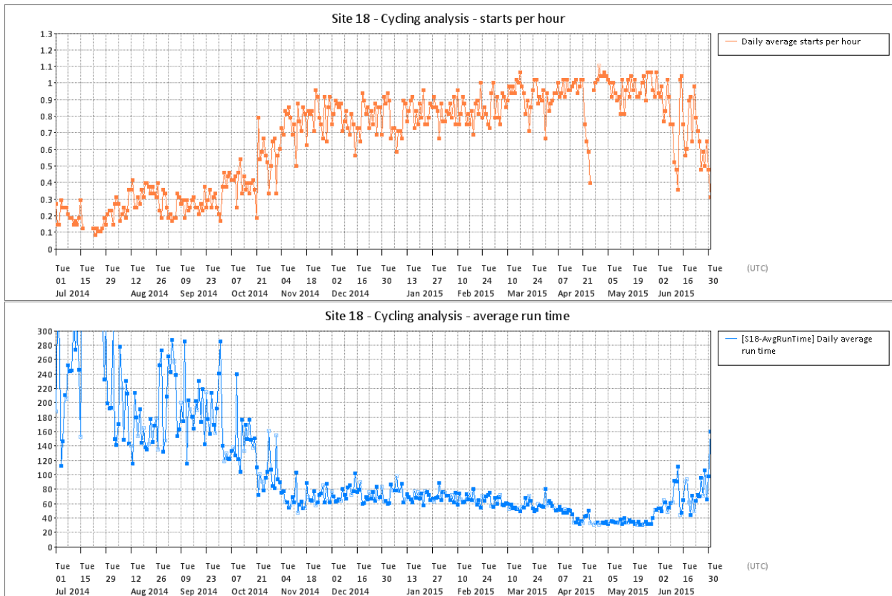
Figure T 122 – Site 18 cycling analysis
