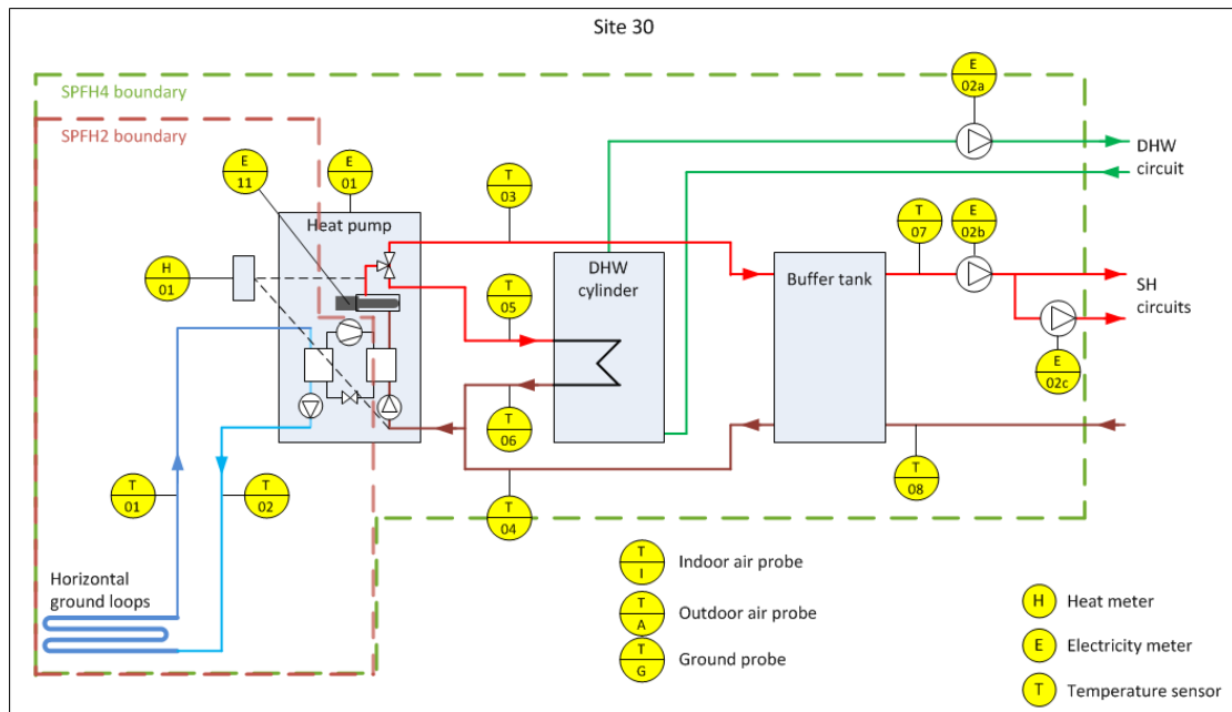
Figure T 14 – Site 30 system schematic
