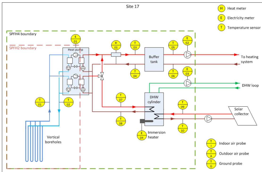
Figure T 9 – Site 17 system schematic
