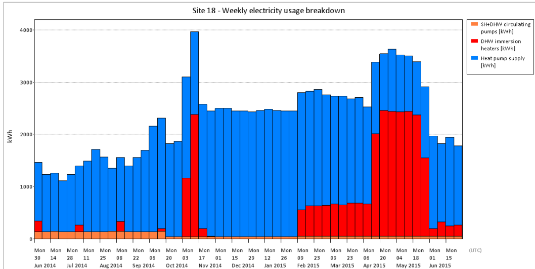
Figure T 177 – Site 18 electricity breakdown
