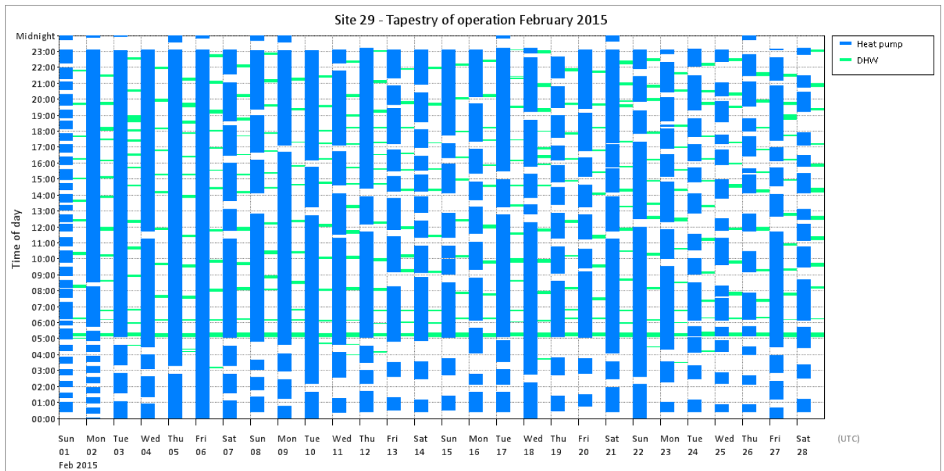
Figure T 97 – Site 29 tapestries of operation
