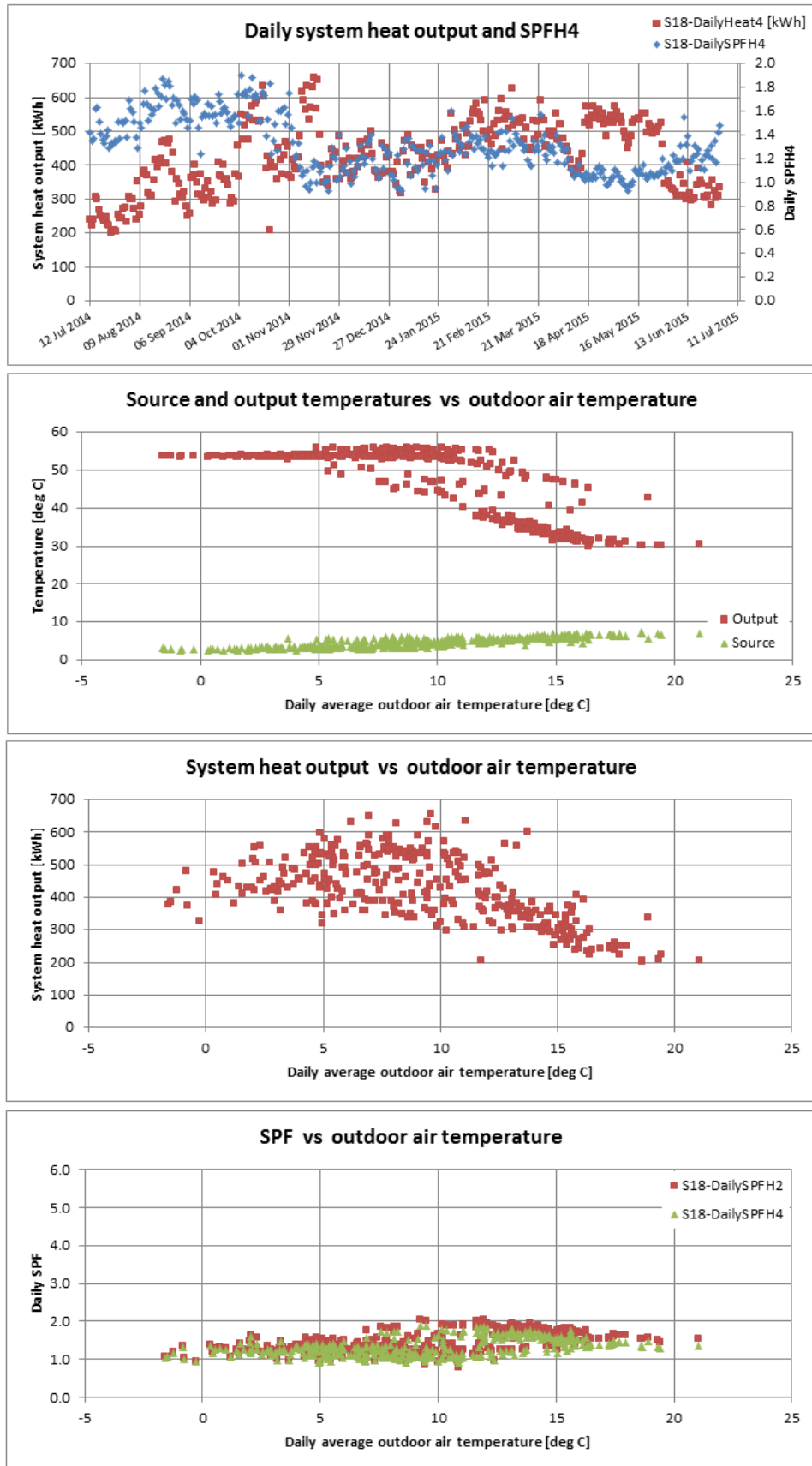
Figure T 47 – Site 18 system efficiency charts (1)
