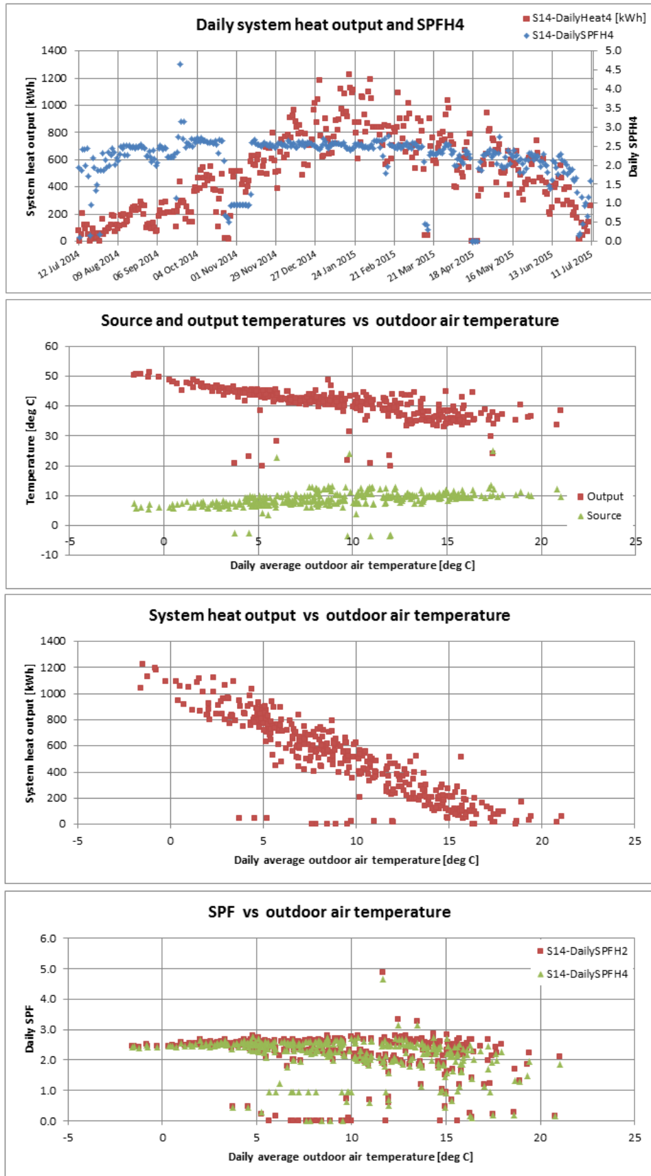
Figure T 43 – Site 14 system efficiency charts (1)
