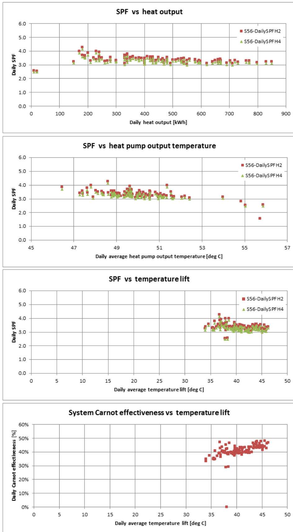
Figure T 76 – Site 56 system efficiency charts (2)
