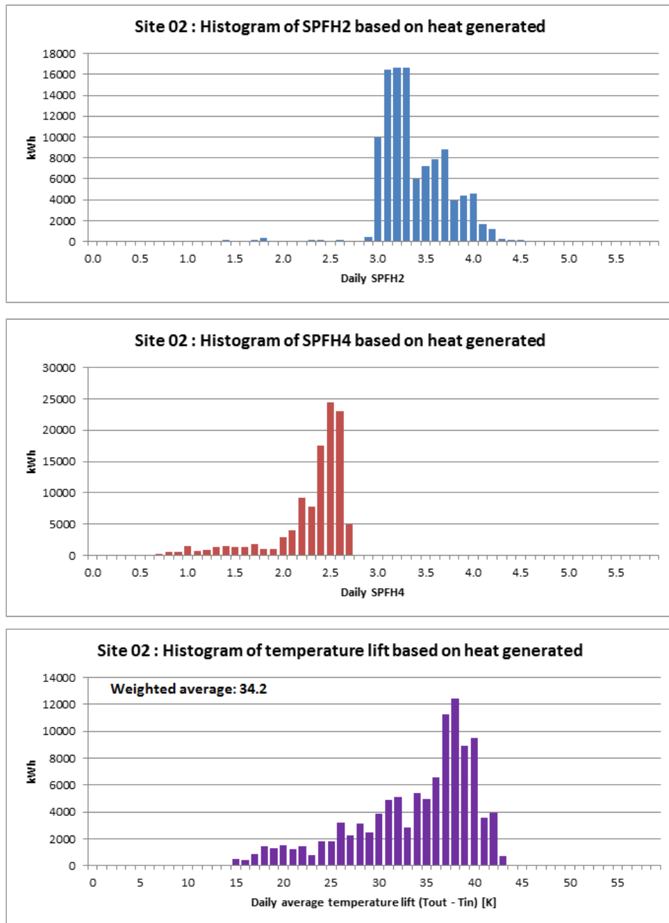
Figure T 142 – Site 02 histograms of SPF H2 , SPF H4 and temperature lift
