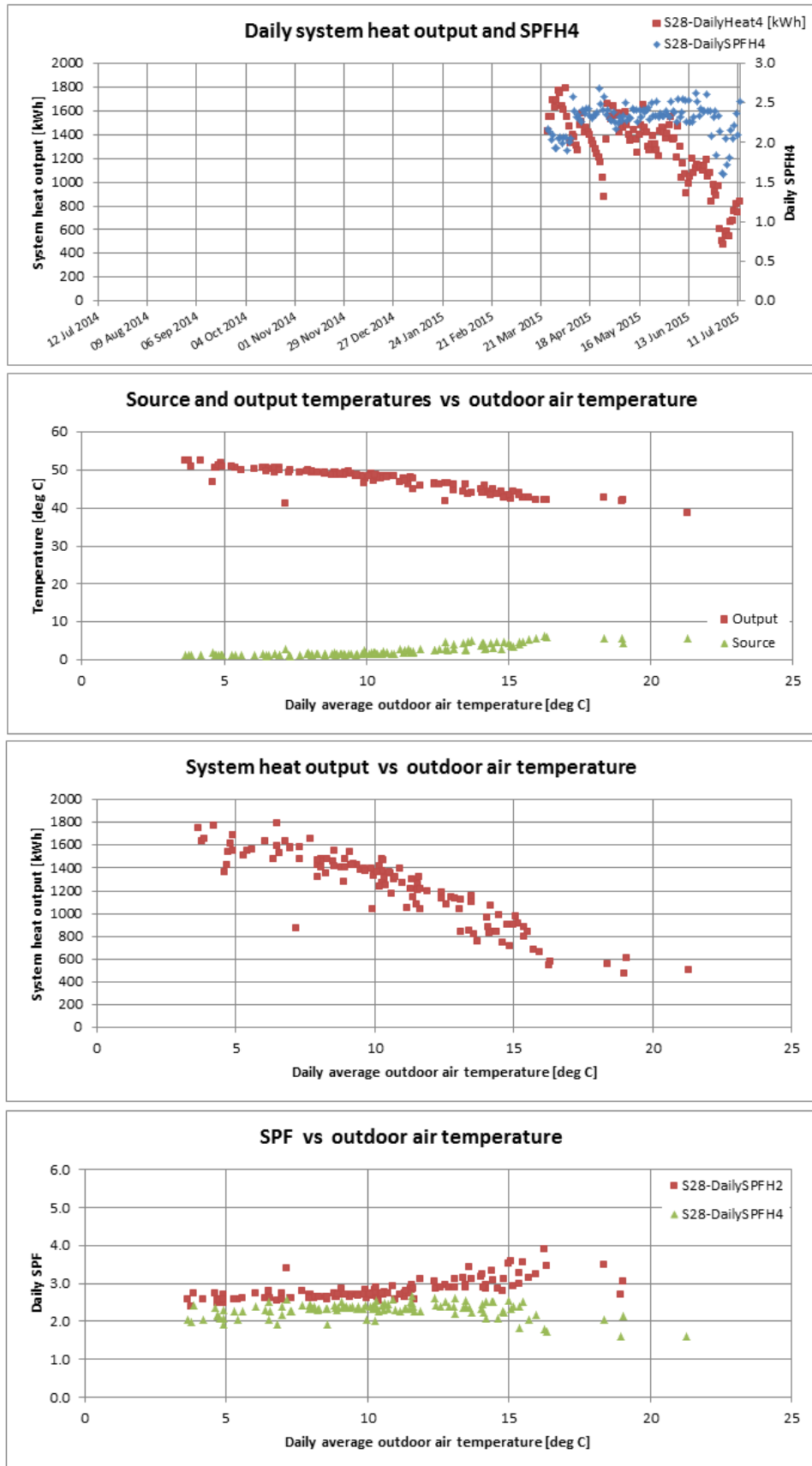
Figure T 51 – Site 28 system efficiency charts (2)
