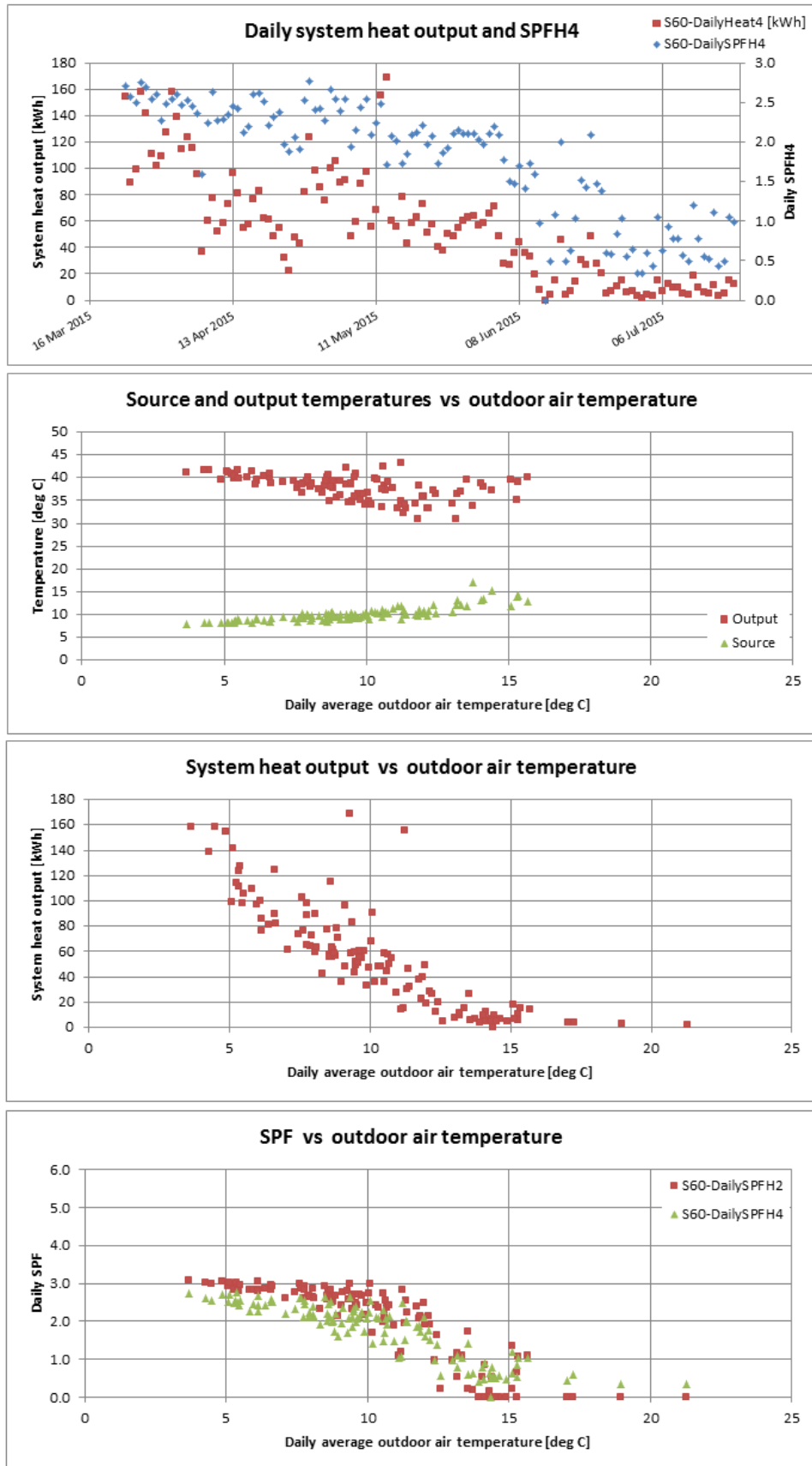
Figure T 79 – Site 60 system efficiency charts (1)
