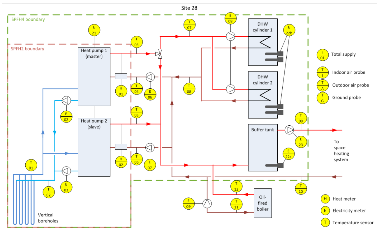
Figure T 12 – Site 28 system schematic
