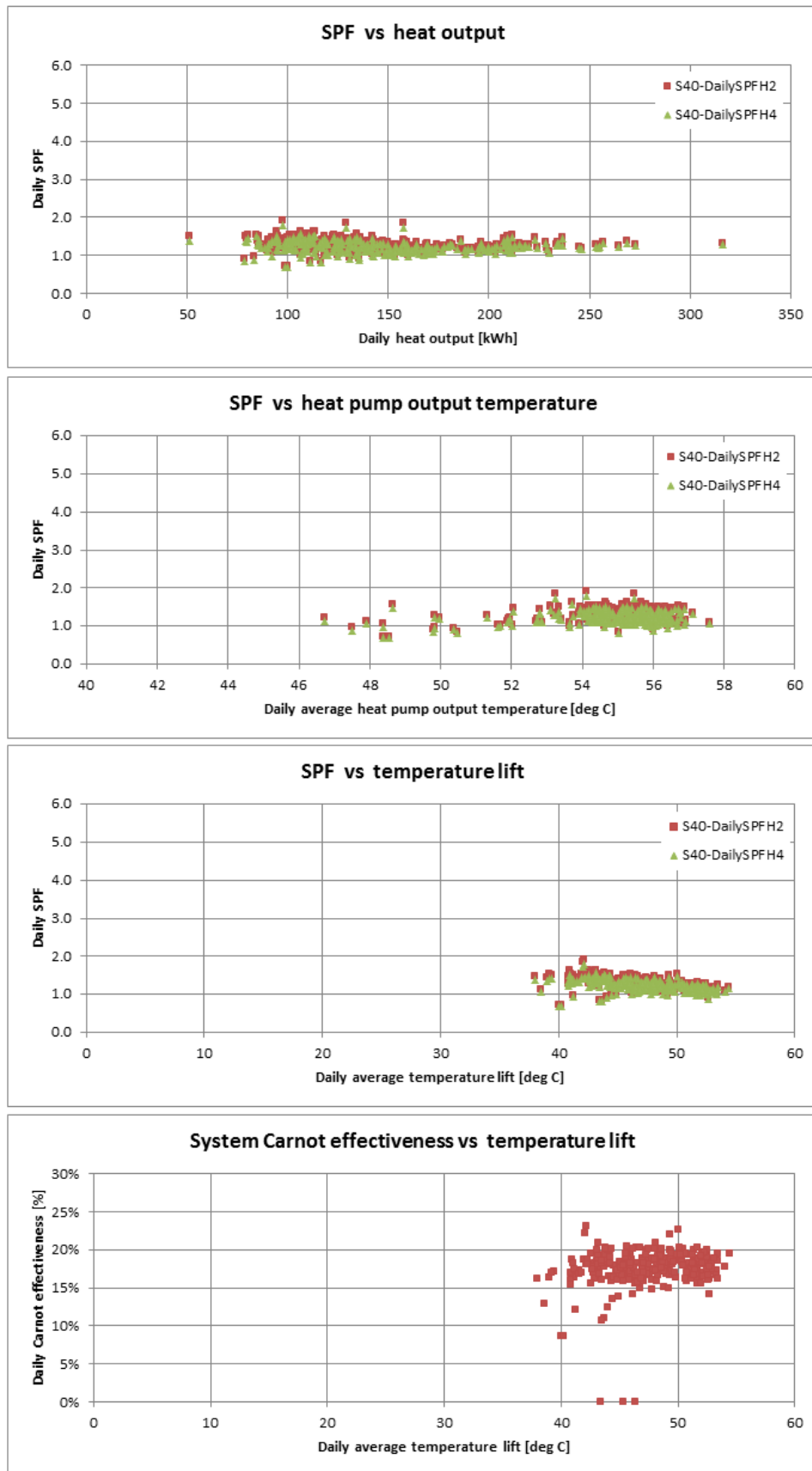
Figure T 68 – Site 40 system efficiency charts (2)
