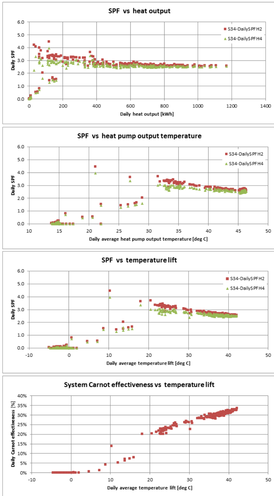
Figure T 60 – Site 34 system efficiency charts (2)
