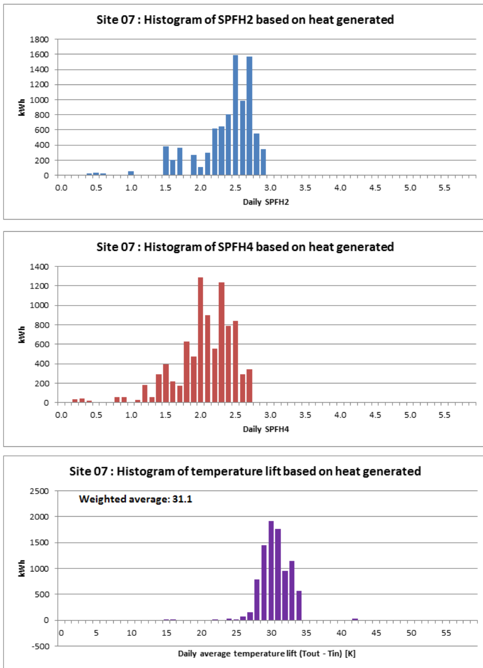
Figure T 145 – Site 07 histograms of SPF H2 , SPF H4 and temperature lift
