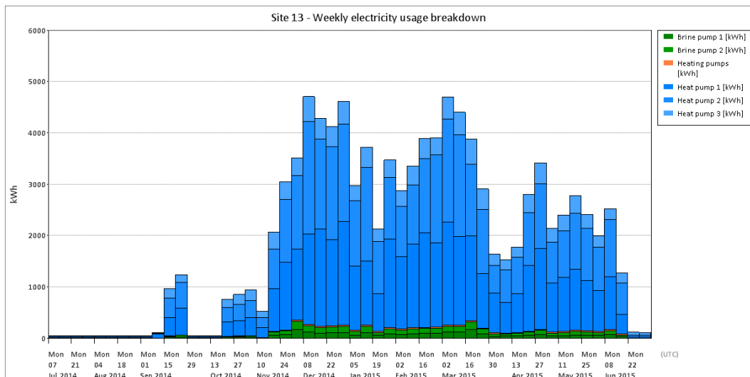
Figure T 174 – Site 13 electricity breakdown
