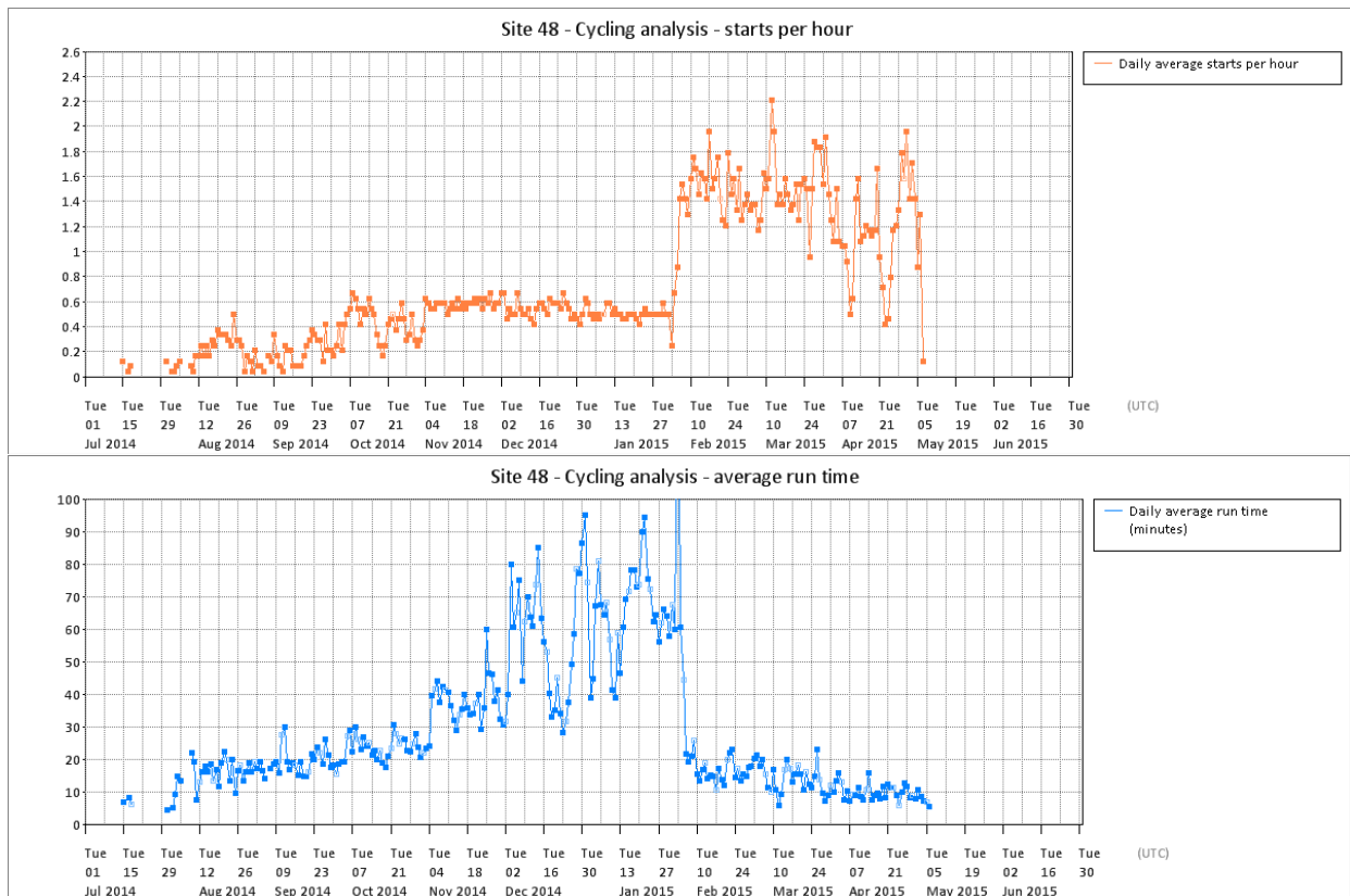
Figure T 133 – Site 48 cycling analysis
