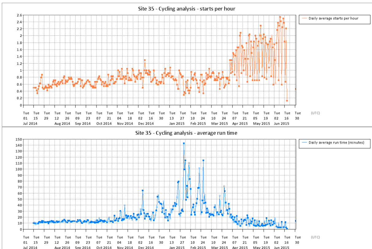
Figure T 129 – Site 35 cycling analysis
