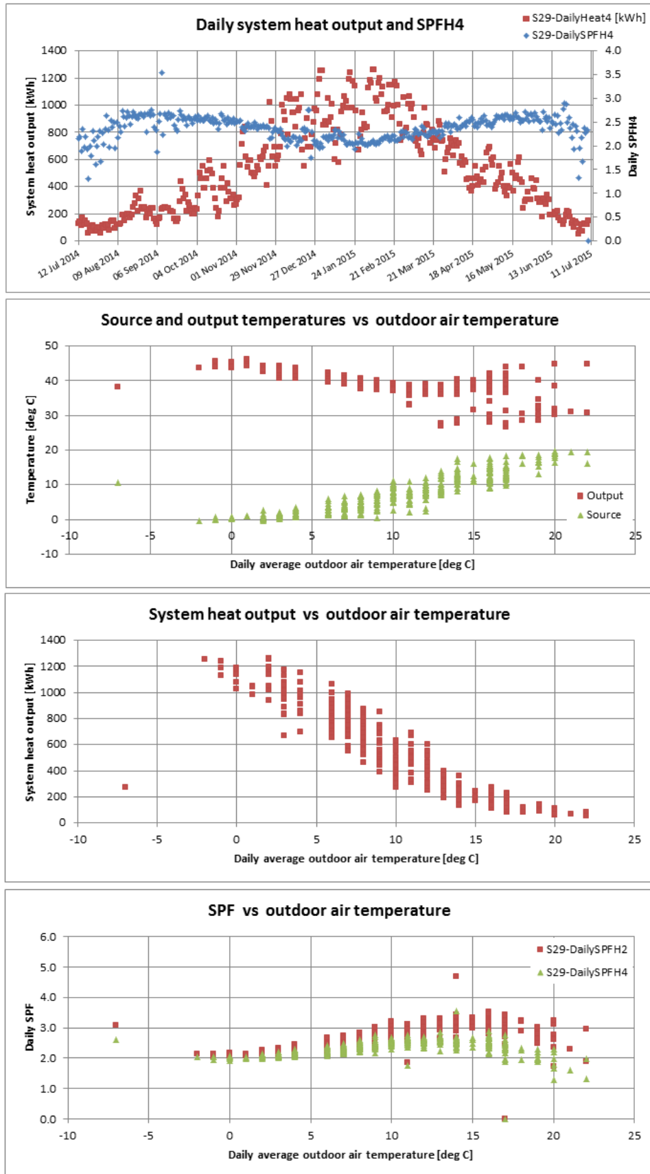
Figure T 53 – Site 29 system efficiency charts (1)
