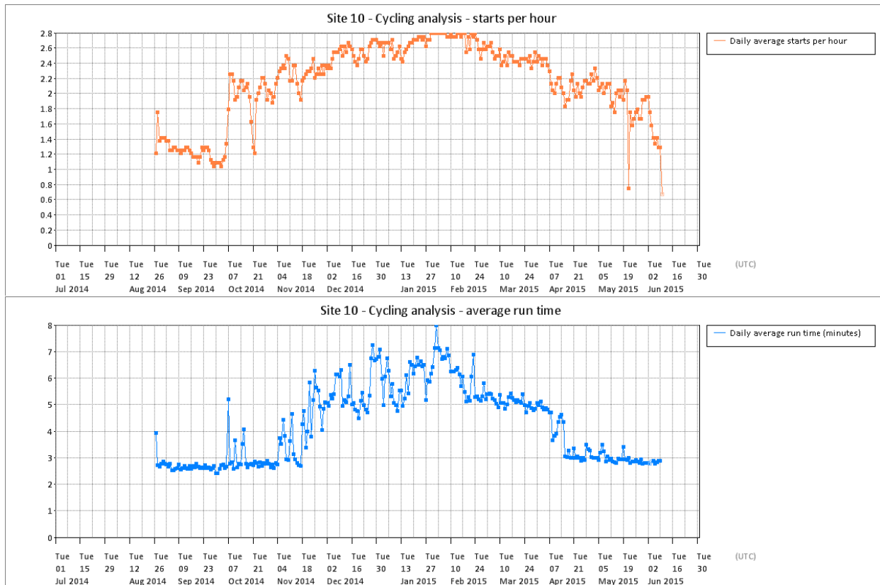
Figure T 118 – Site 10 cycling analysis
