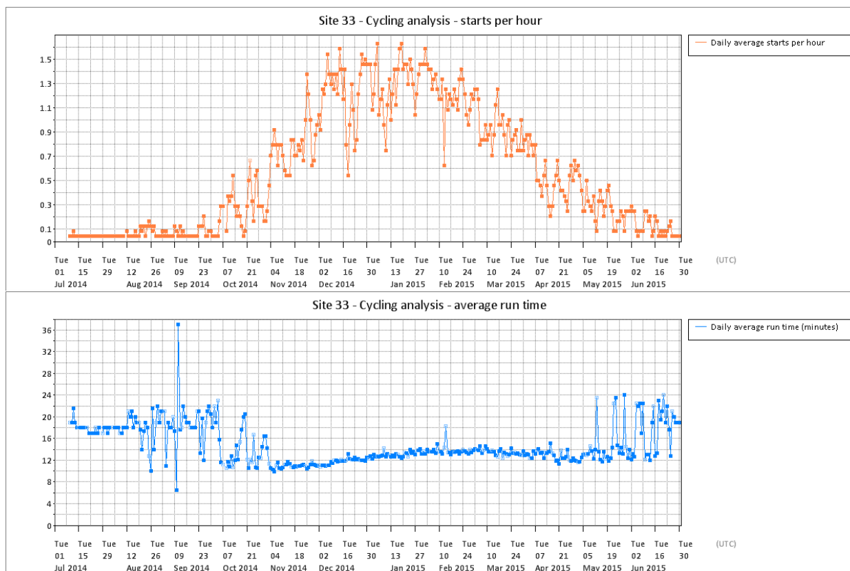
Figure T 127 – Site 33 cycling analysis
