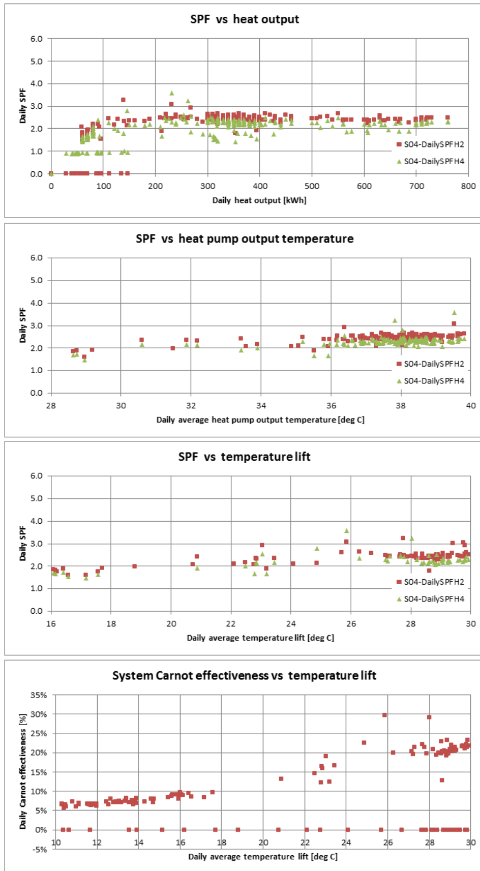
Figure T 34 – Site 04 system efficiency charts (2)
