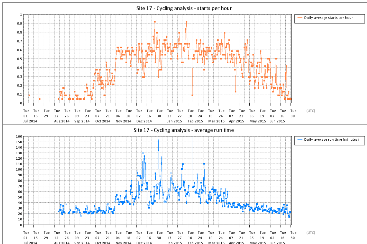
Figure T 121 – Site 17 cycling analysis
