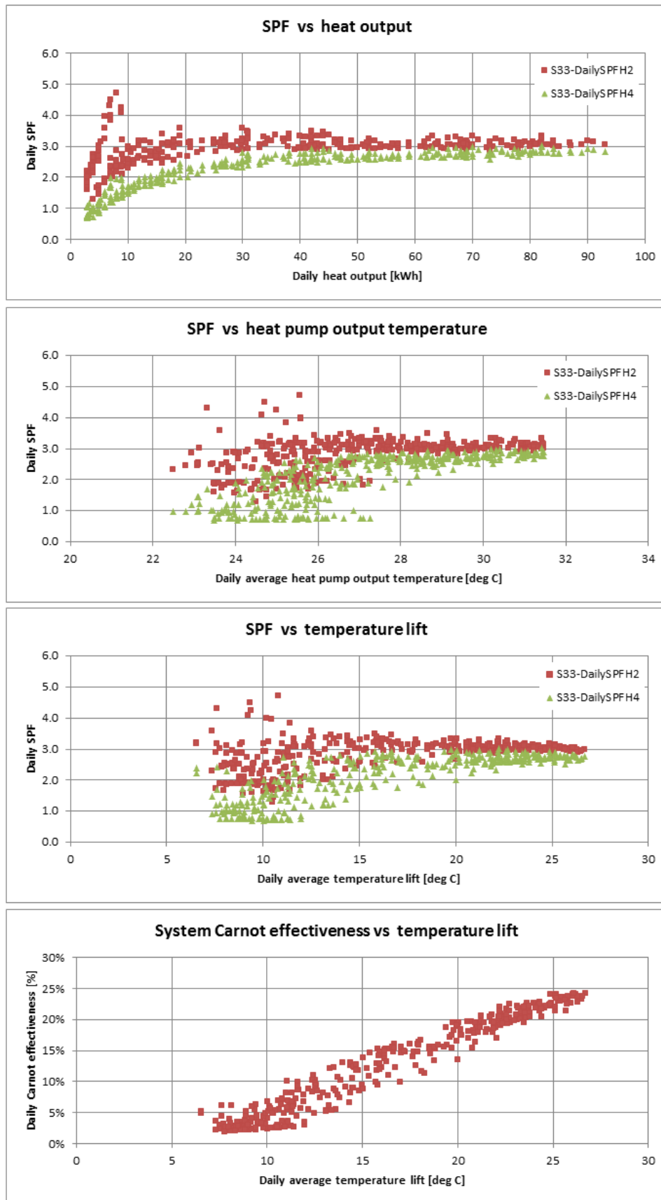
Figure T 58 – Site 33 system efficiency charts (2)
