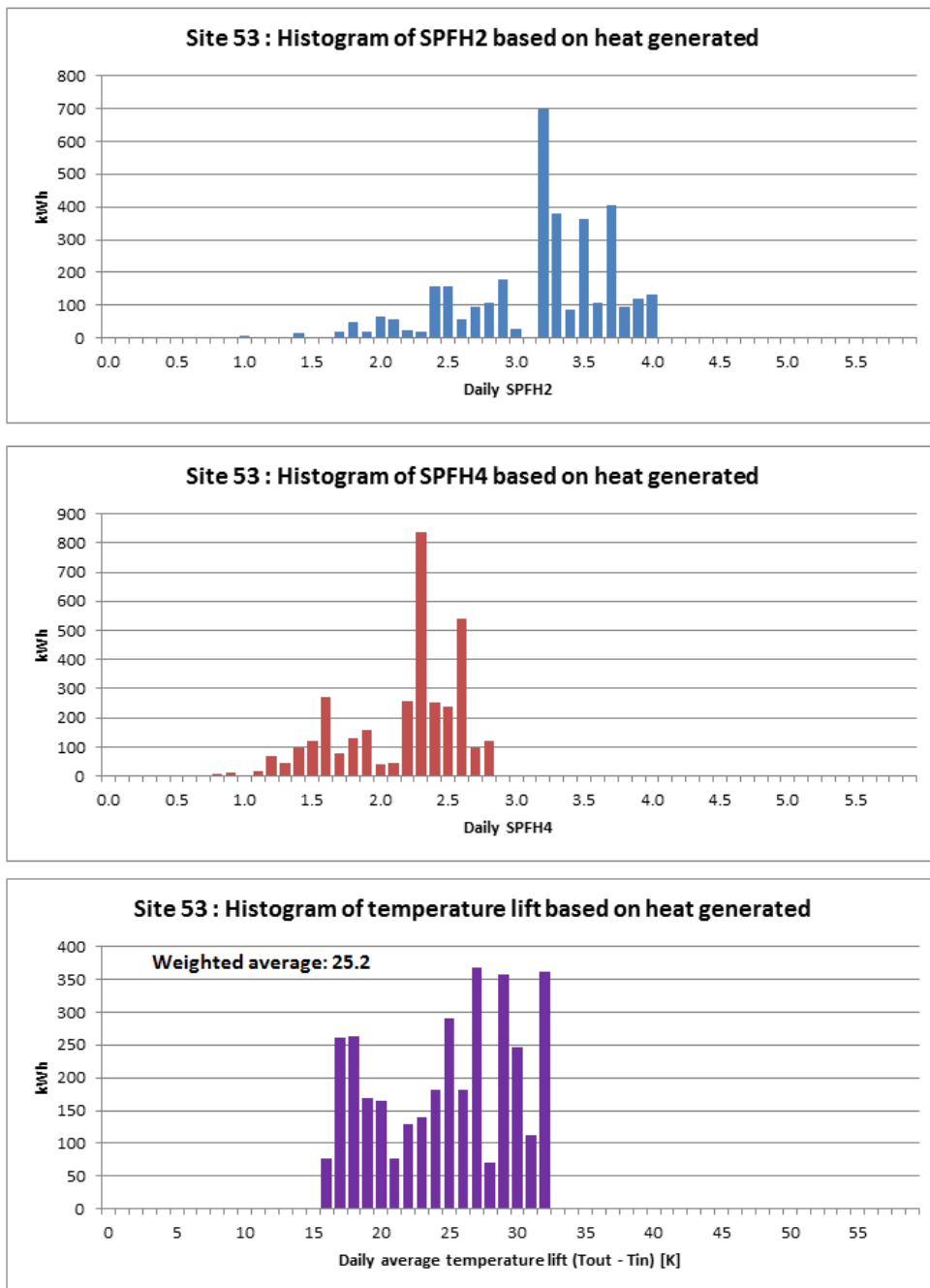
Figure T 163 – Site 53 histograms of SPF H2 , SPF H4 and temperature lift
