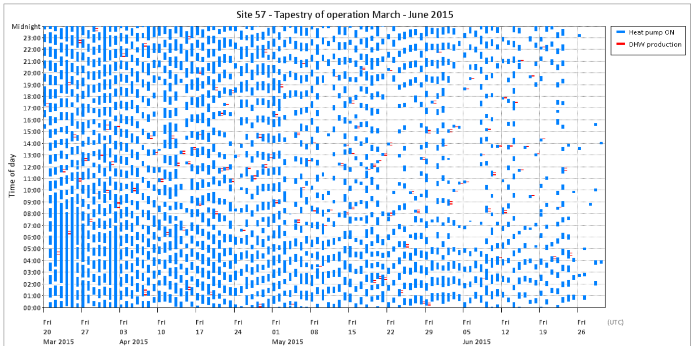
Figure T 109 – Site 57 tapestry of operation
