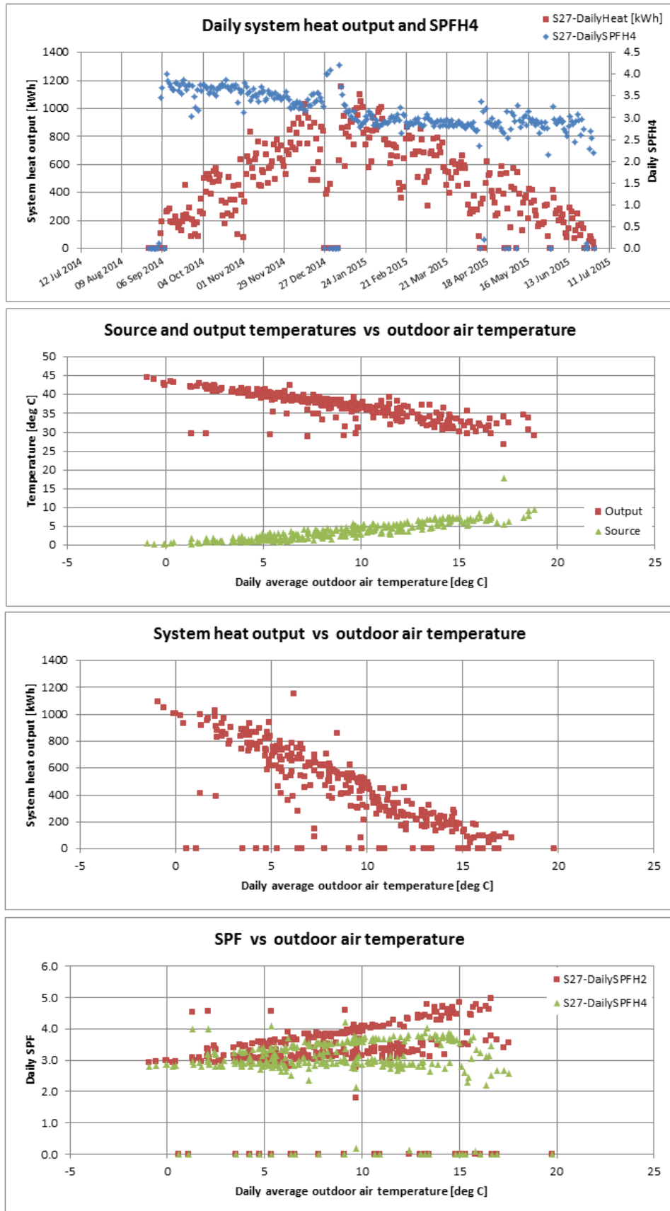
Figure T 49 – Site 27 system efficiency charts (1)
