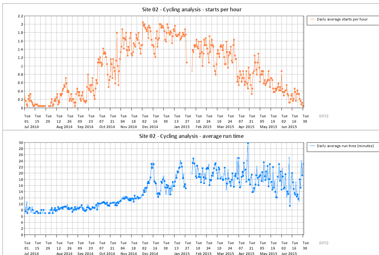
Figure T 114 – Site 02 cycling analysis
