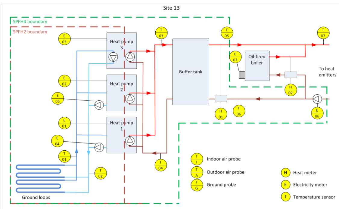
Figure T 7 – Site 13 system schematic
