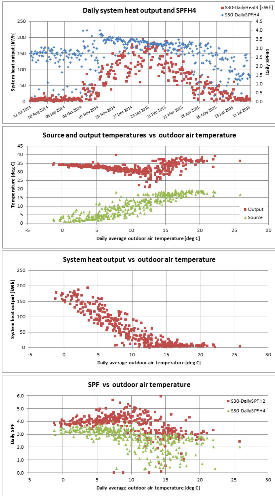
Figure T 55 – Site 30 system efficiency charts (1)
