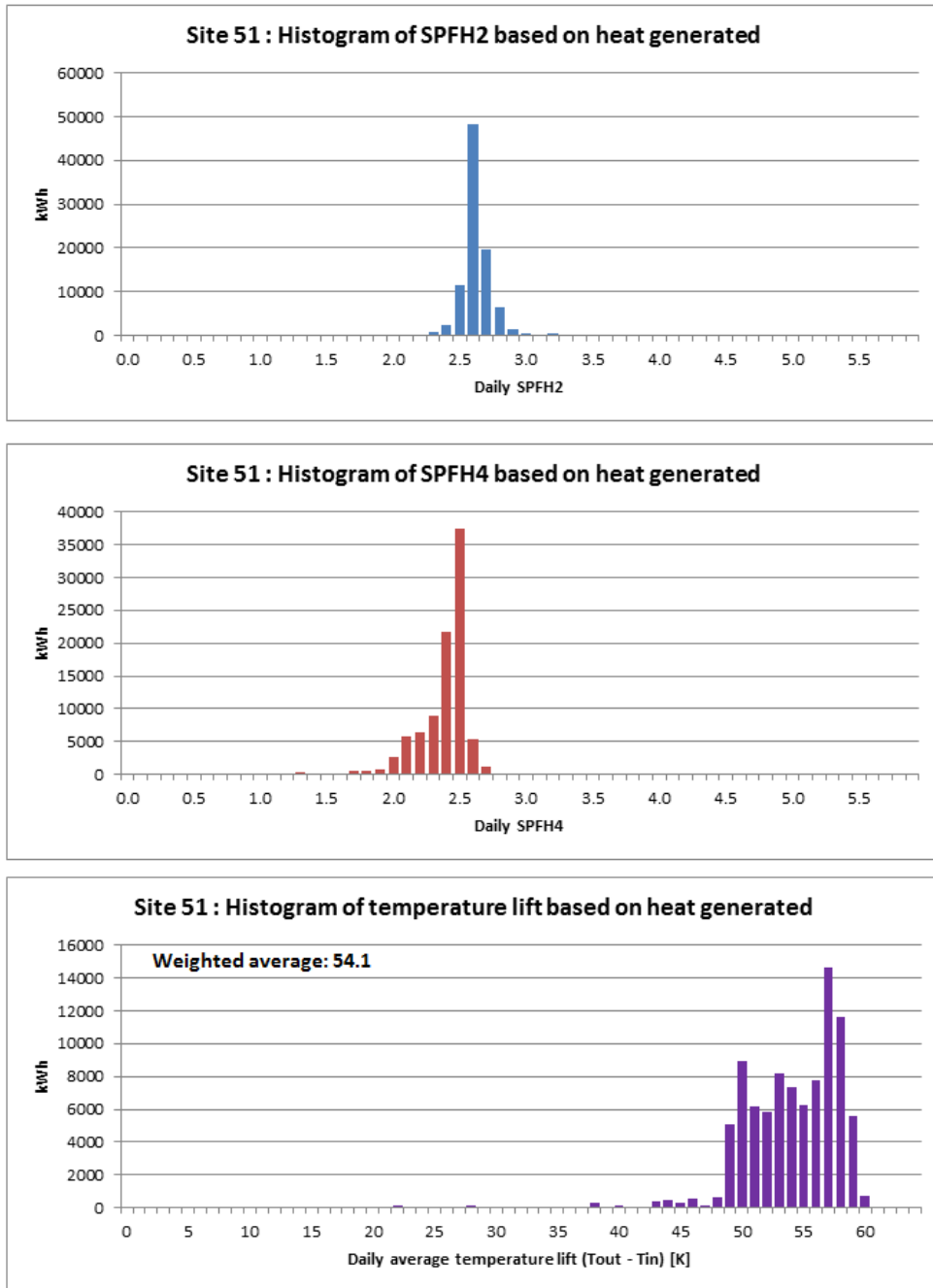
Figure T 162 – Site 51 histograms of SPF H2 , SPF H4 and temperature lift
