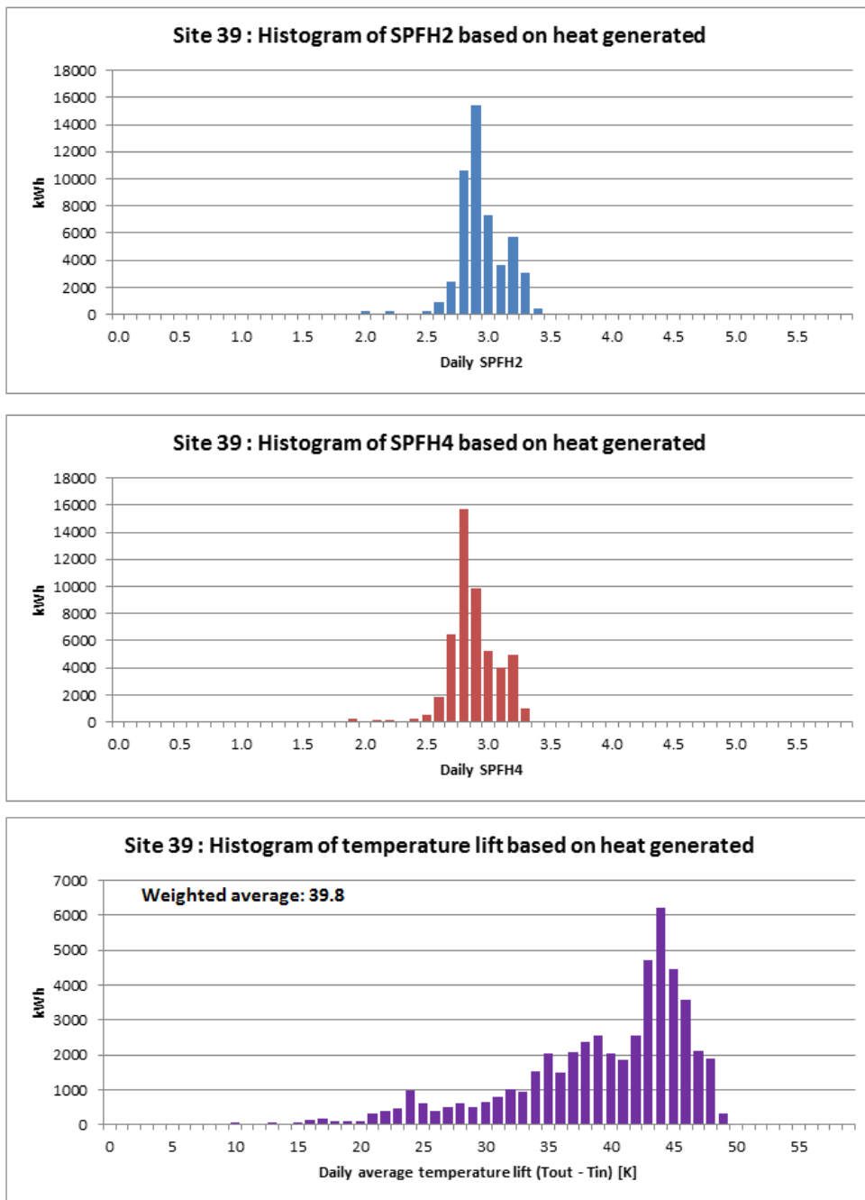
Figure T 159 – Site 39 histograms of SPF H2 , SPF H4 and temperature lift
