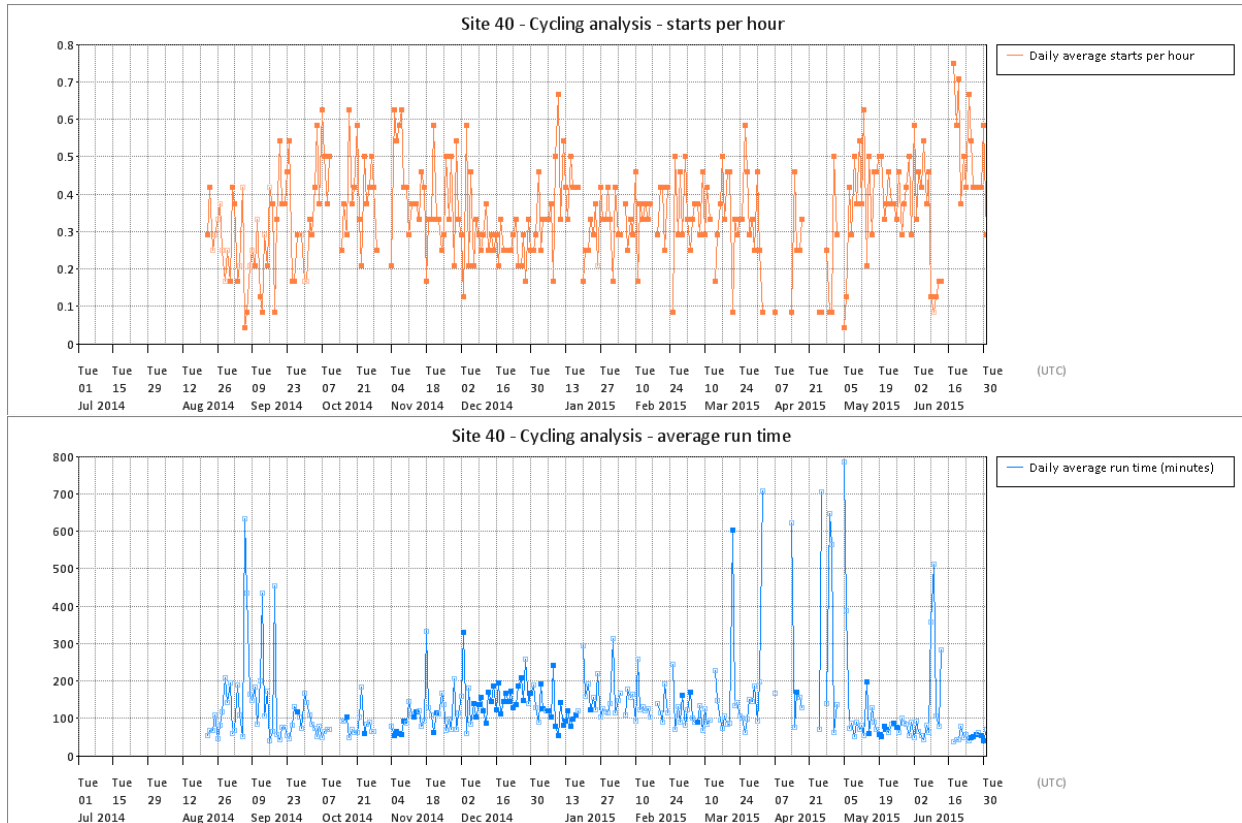
Figure T 132 – Site 40 cycling analysis
