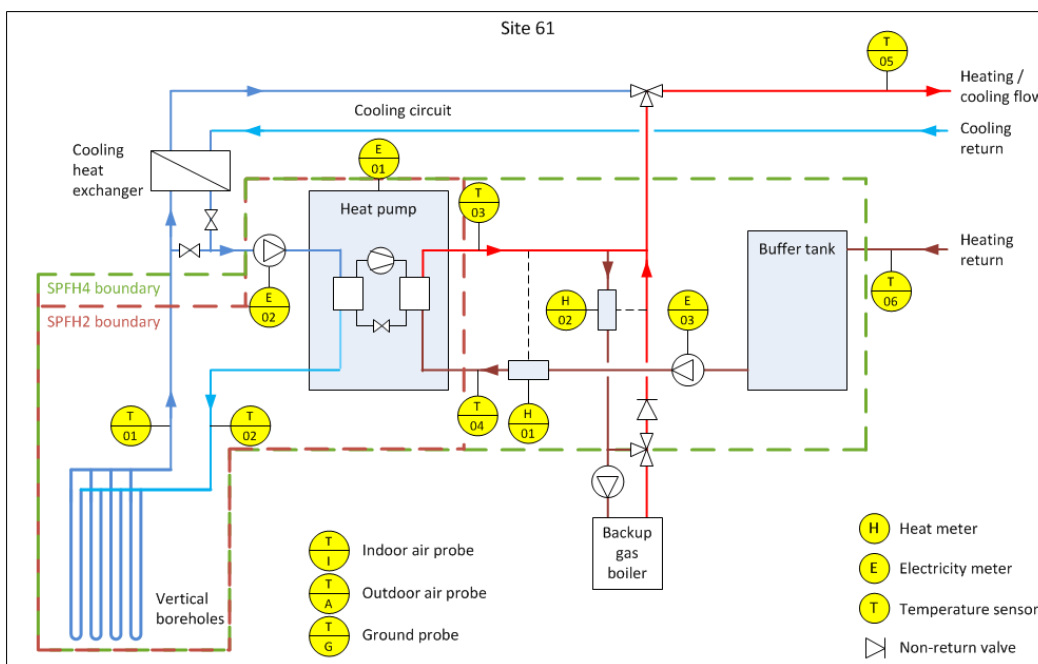
Figure T 28 – Site 61 system schematic
