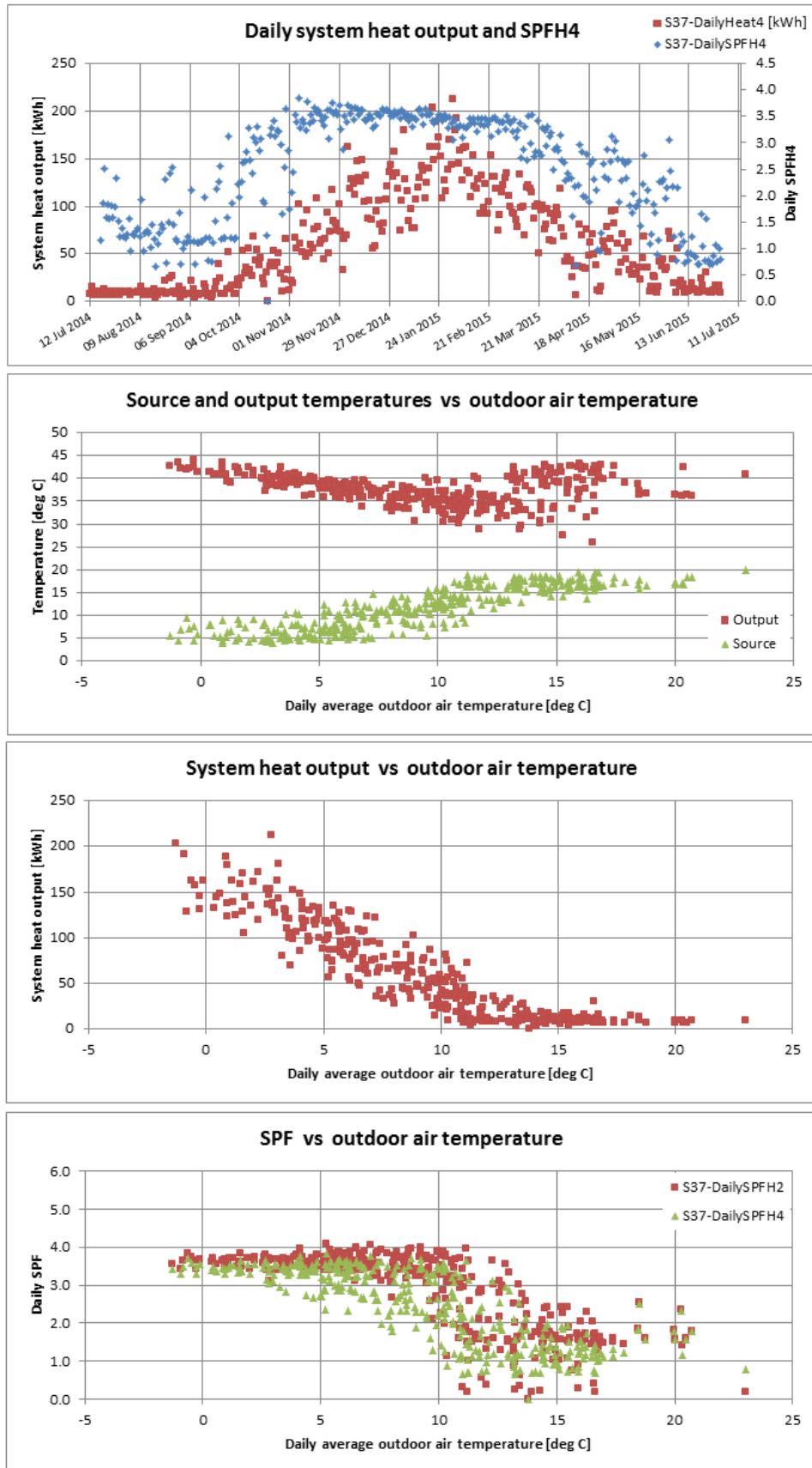
Figure T 63 – Site 37 system efficiency charts (1)
