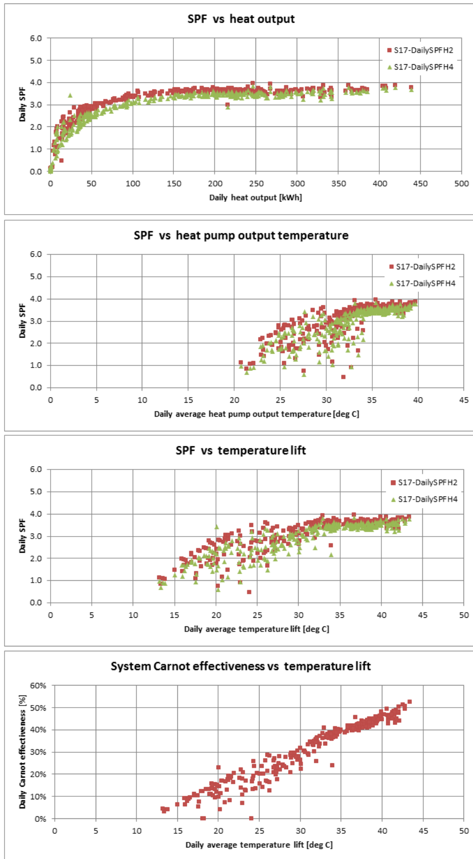
Figure T 46 – Site 17 system efficiency charts (2)
