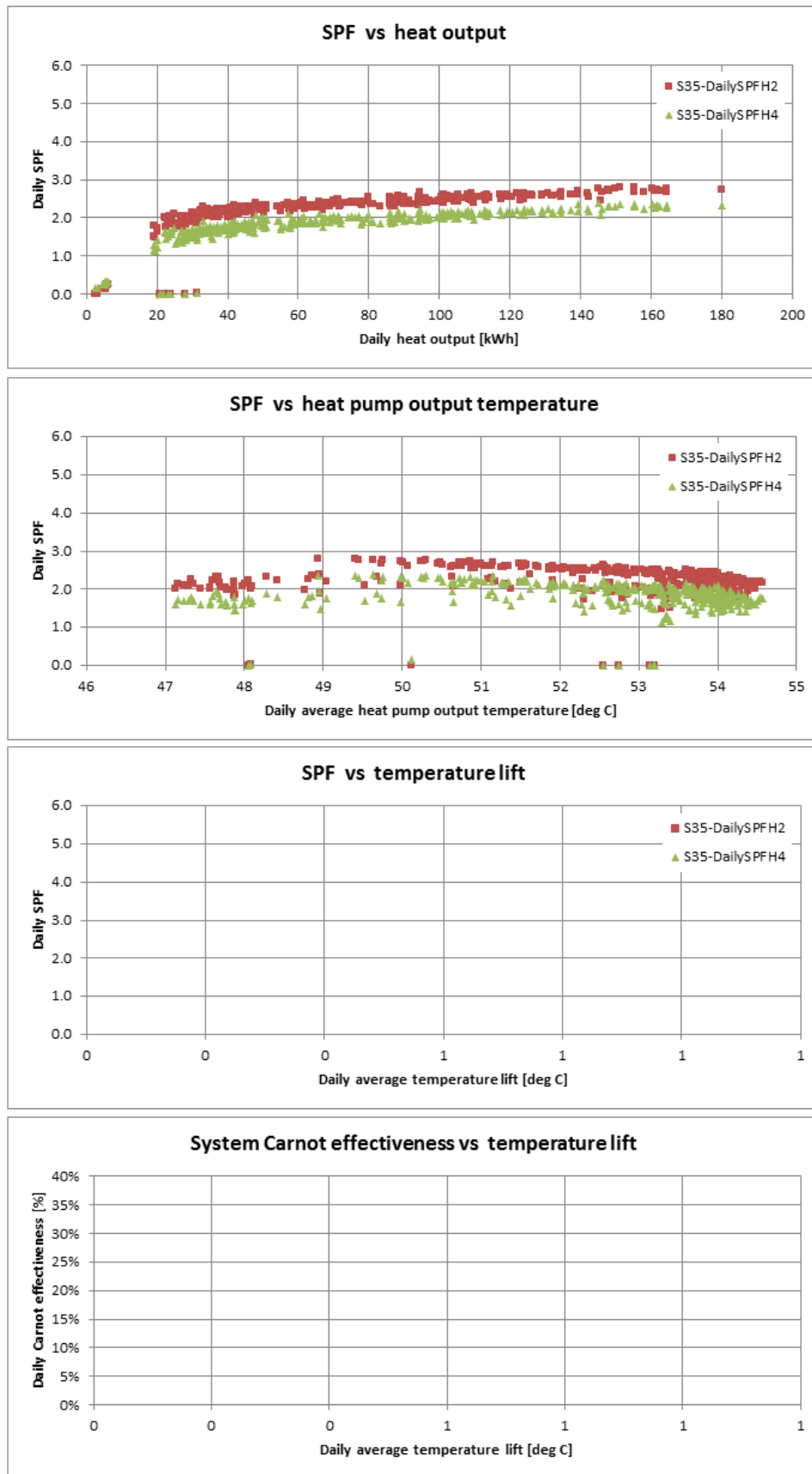
Figure T 62 – Site 35 system efficiency charts (2)
