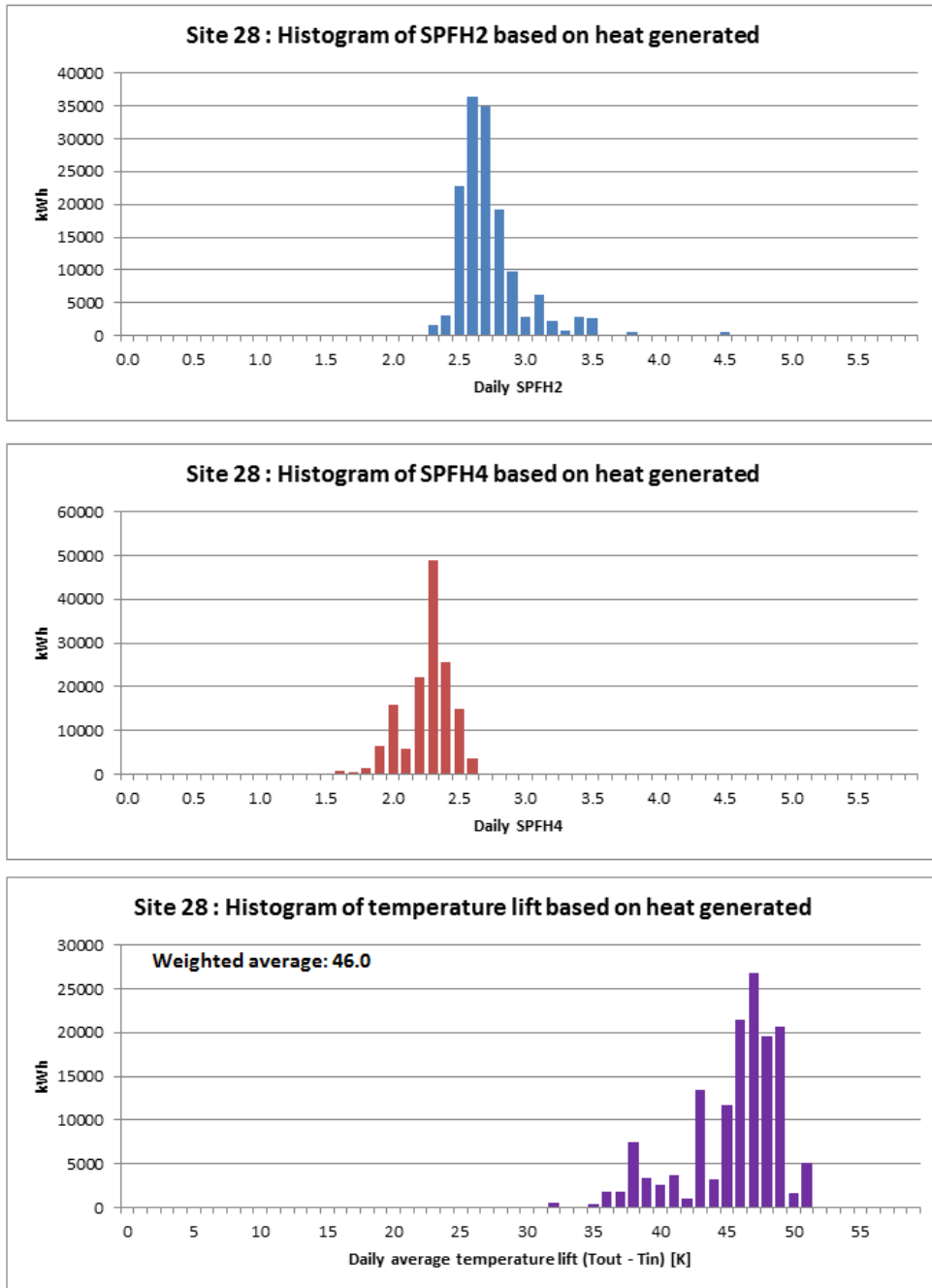
Figure T 152 – Site 28 histograms of SPF H2 , SPF H4 and temperature lift
