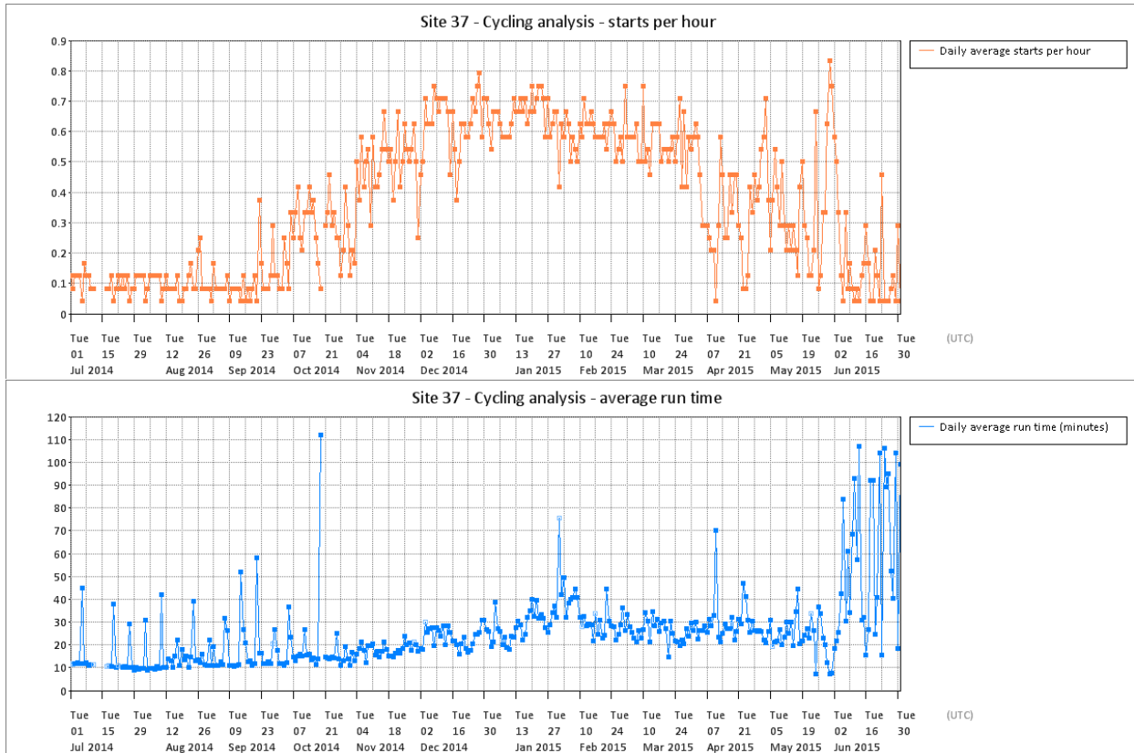
Figure T 130 – Site 37 cycling analysis
