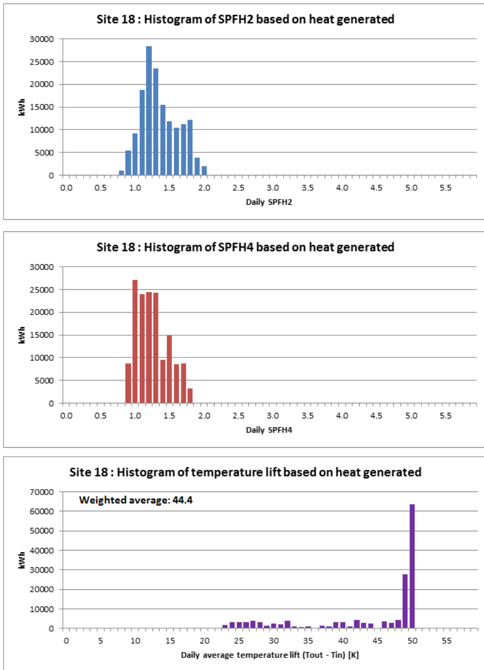
Figure T 150 – Site 18 histograms of SPF H2 , SPF H4 and temperature lift
