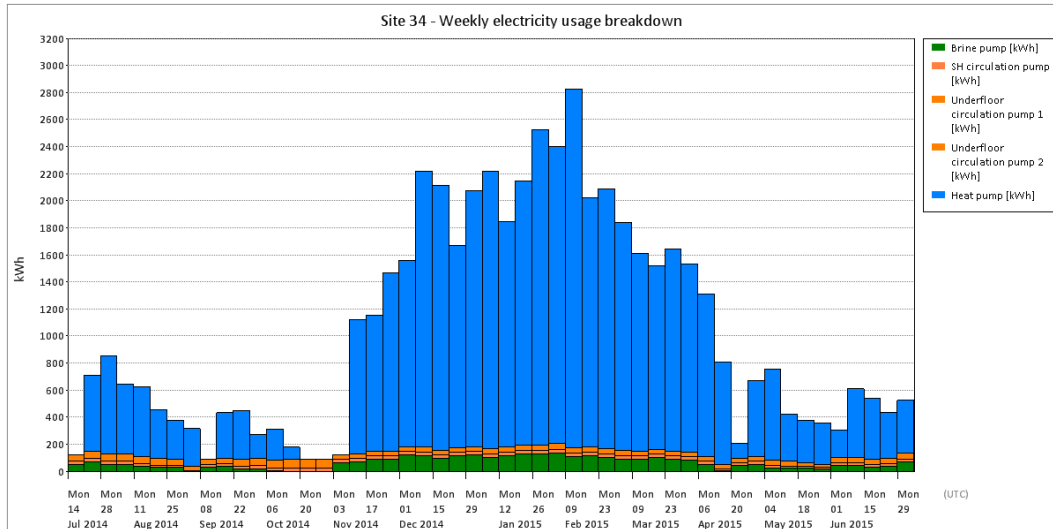
Figure T 181 – Site 34 electricity breakdown
