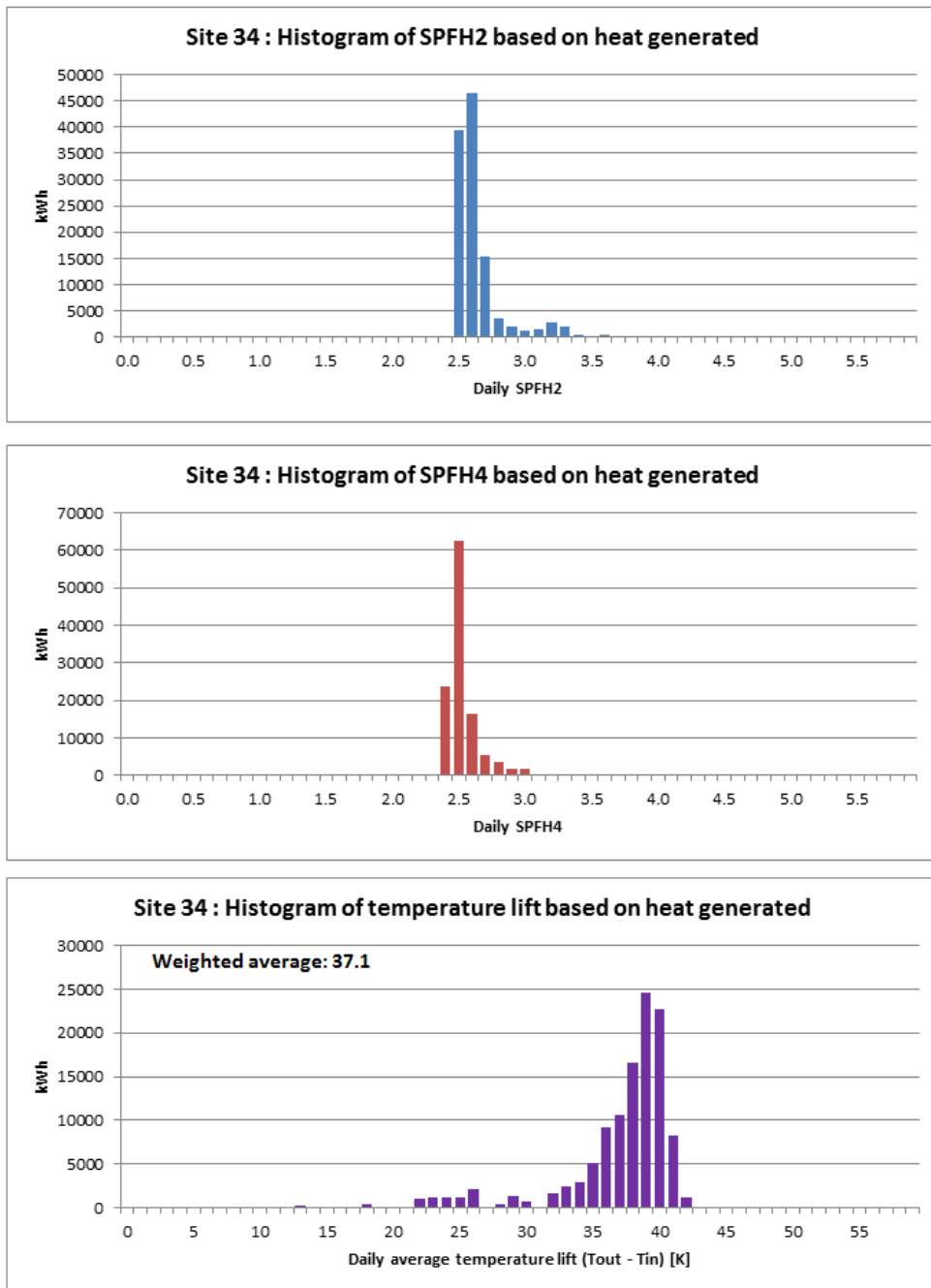
Figure T 156 – Site 34 histograms of SPF H2 , SPF H4 and temperature lift
