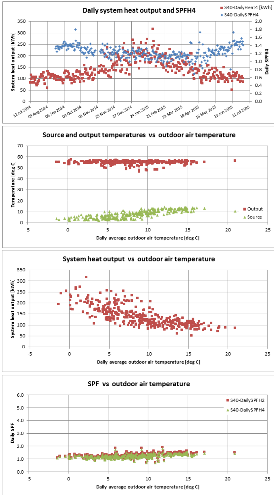
Figure T 67 – Site 40 system efficiency charts (1)
