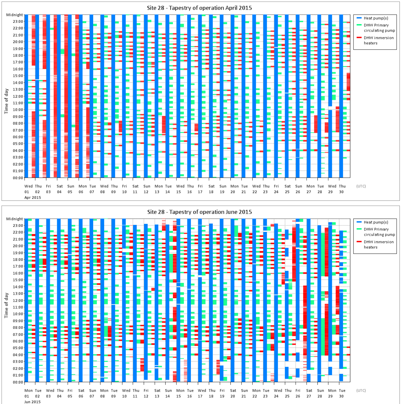
Figure T 96 – Site 28 tapestries of operation
