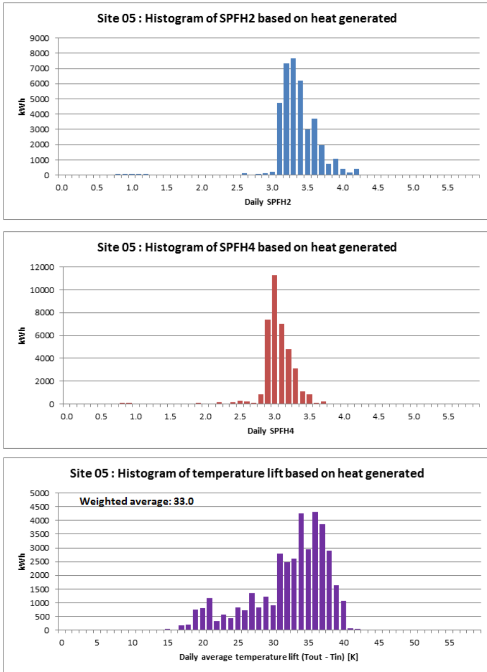
Figure T 144 – Site 05 histograms of SPF H2 , SPF H4 and temperature lift
