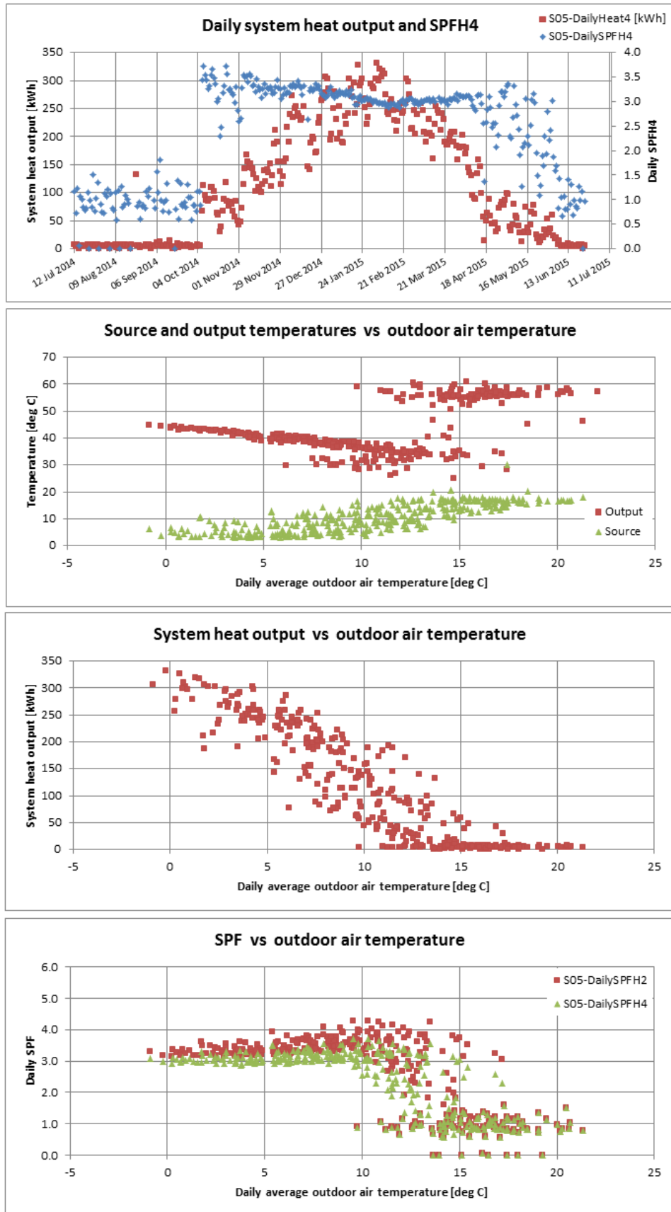
Figure T 35 – Site 05 system efficiency charts (1)
