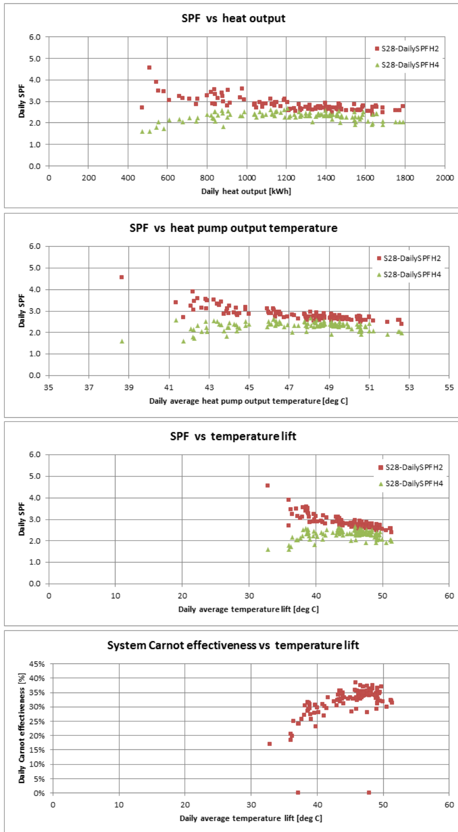
Figure T 52 – Site 28 system efficiency charts (2)
