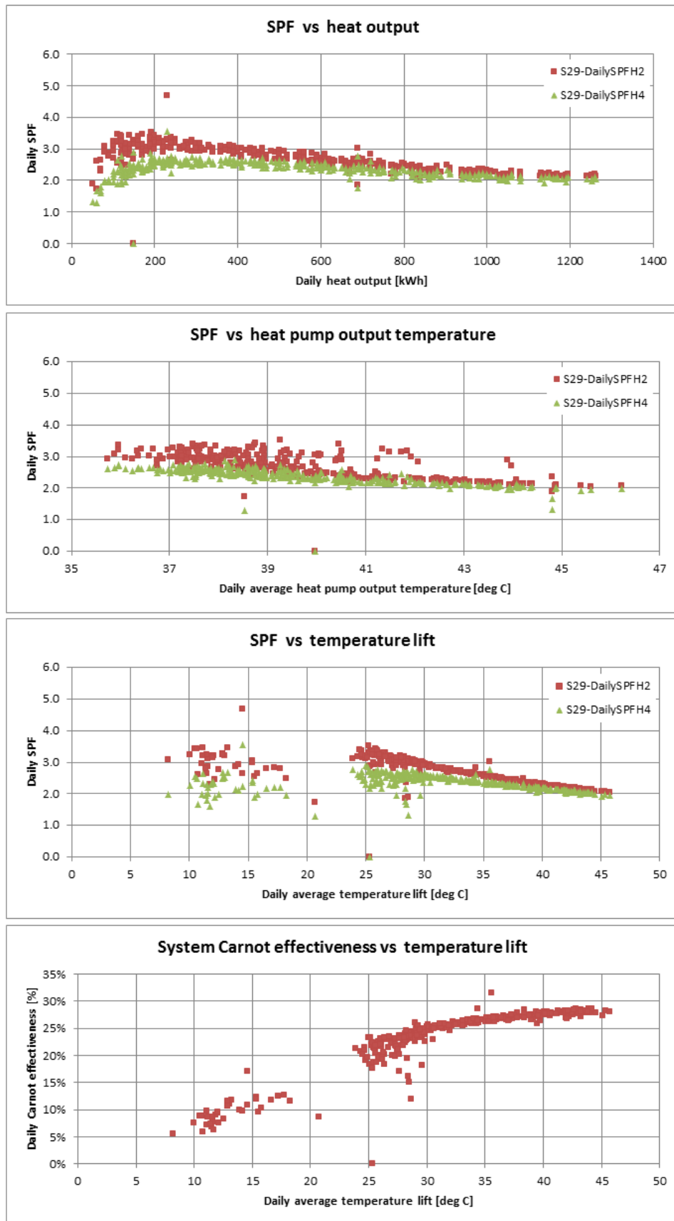
Figure T 54 – Site 29 system efficiency charts (2)
