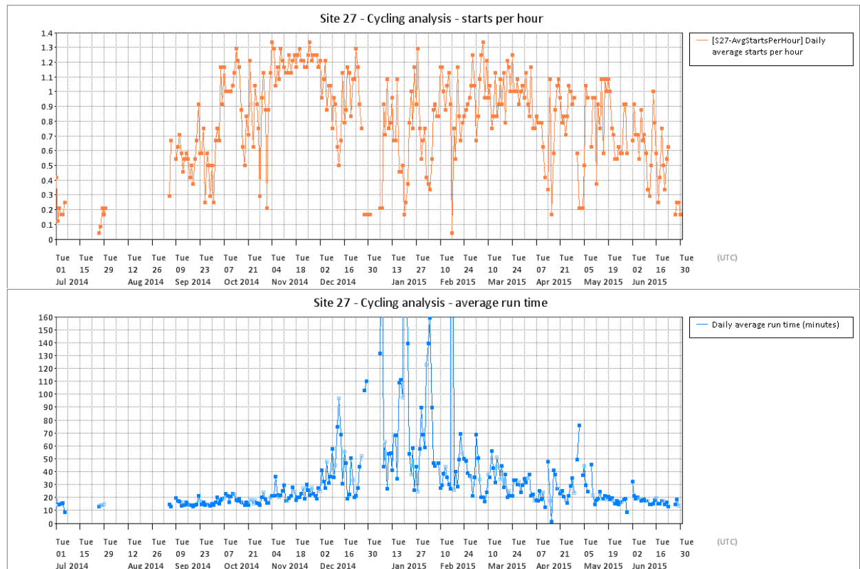
Figure T 123 – Site 27 cycling analysis
