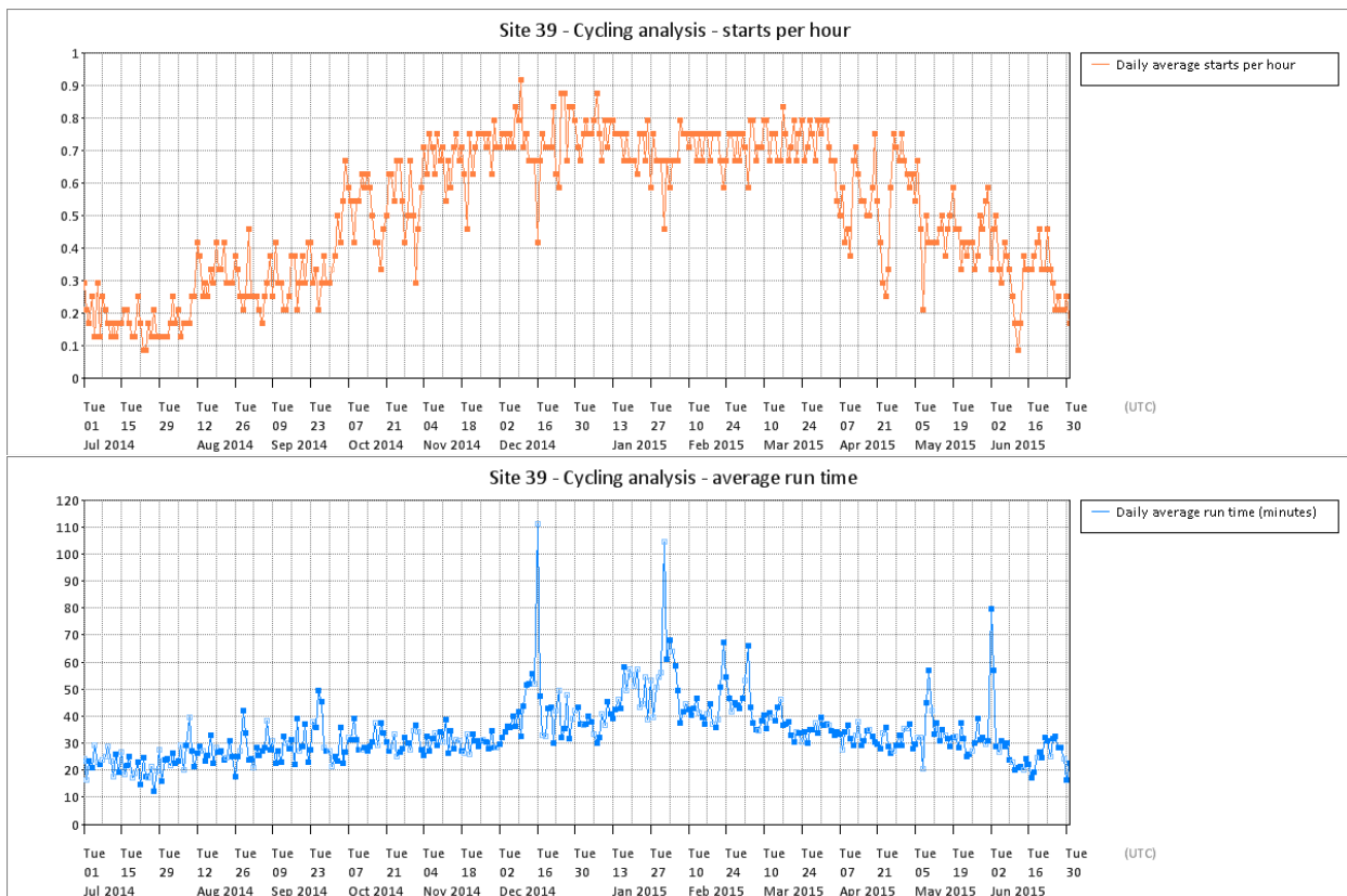
Figure T 131 – Site 39 cycling analysis
