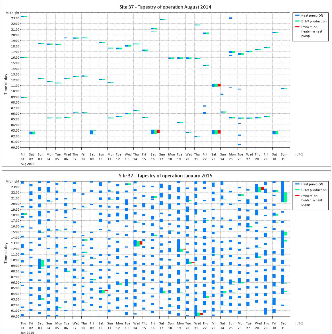
Figure T 102 – Site 37 tapestries of operation
