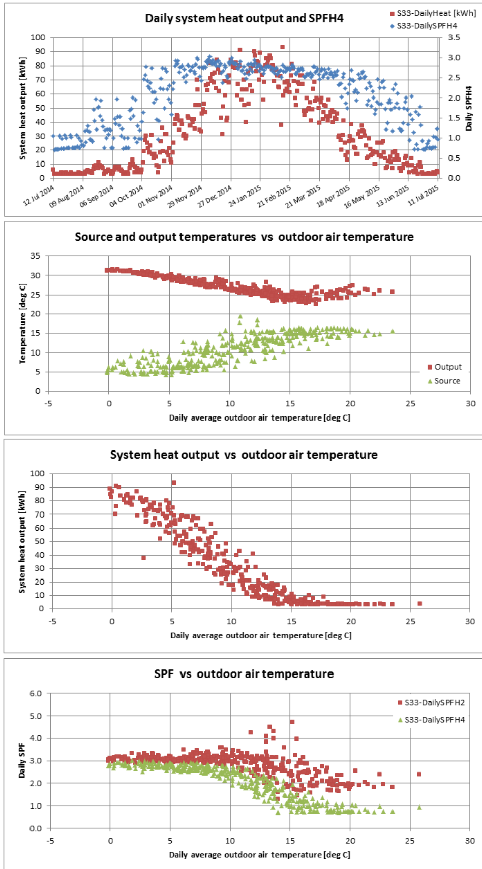
Figure T 57 – Site 33 system efficiency charts (1)
