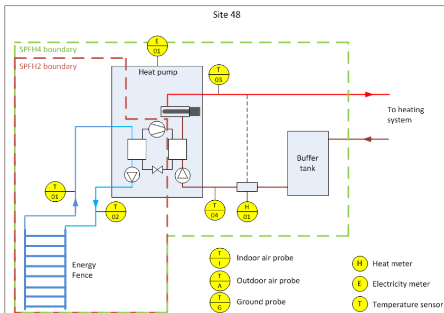
Figure T 22 – Site 48 system schematic
