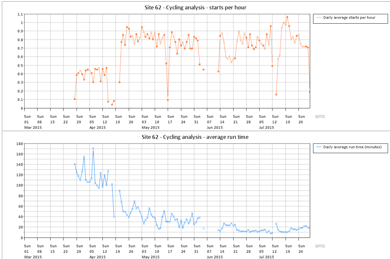
Figure T 140 – Site 62 cycling analysis
