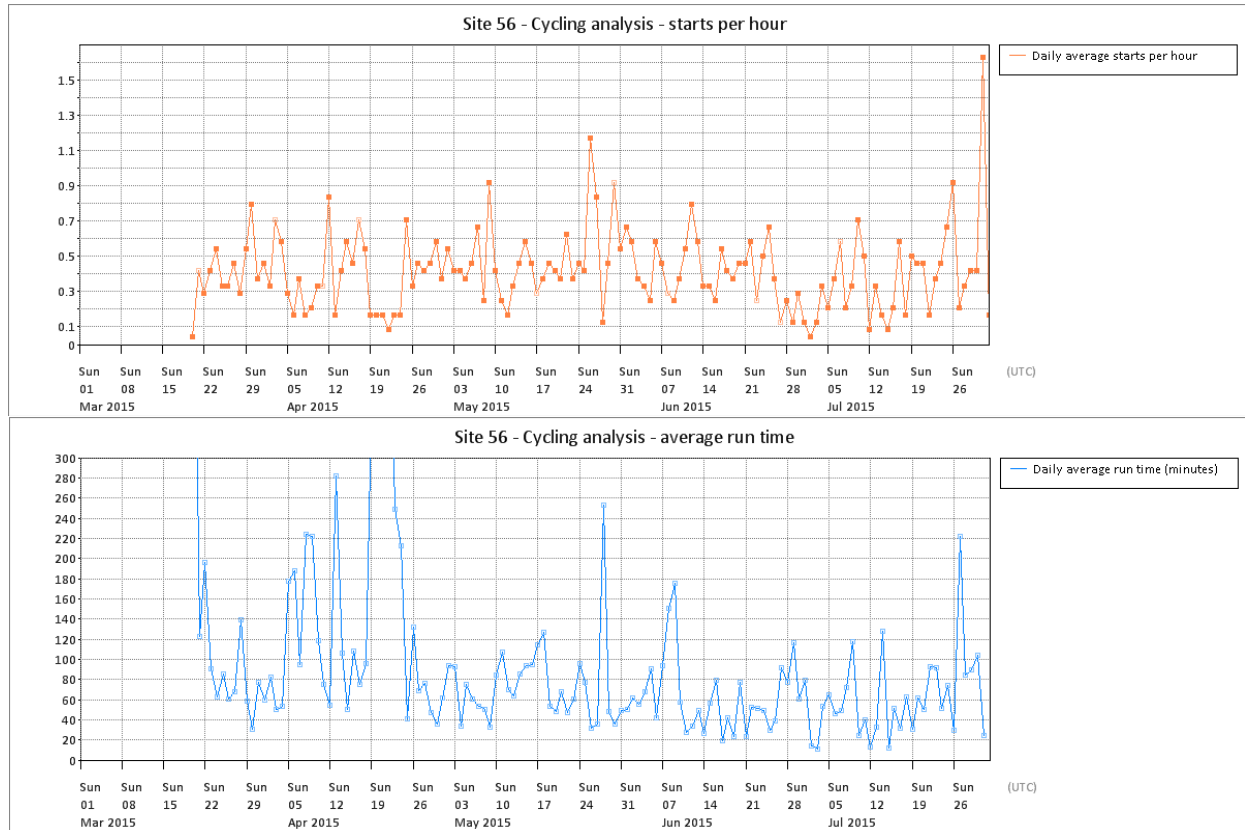
Figure T 136 – Site 56 cycling analysis
