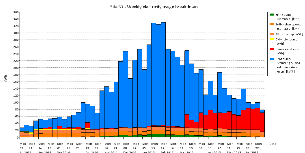
Figure T 183 – Site 37 electricity breakdown
