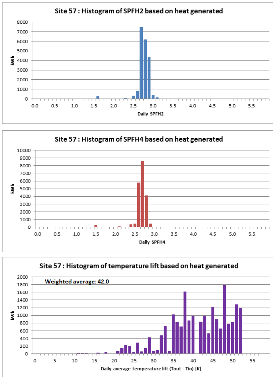
Figure T 165 – Site 57 histograms of SPF H2 , SPF H4 and temperature lift
