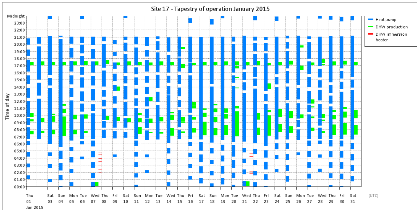
Figure T 93 – Site 17 tapestries of operation
