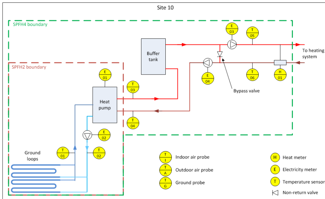
Figure T 6 – Site 10 system schematic
