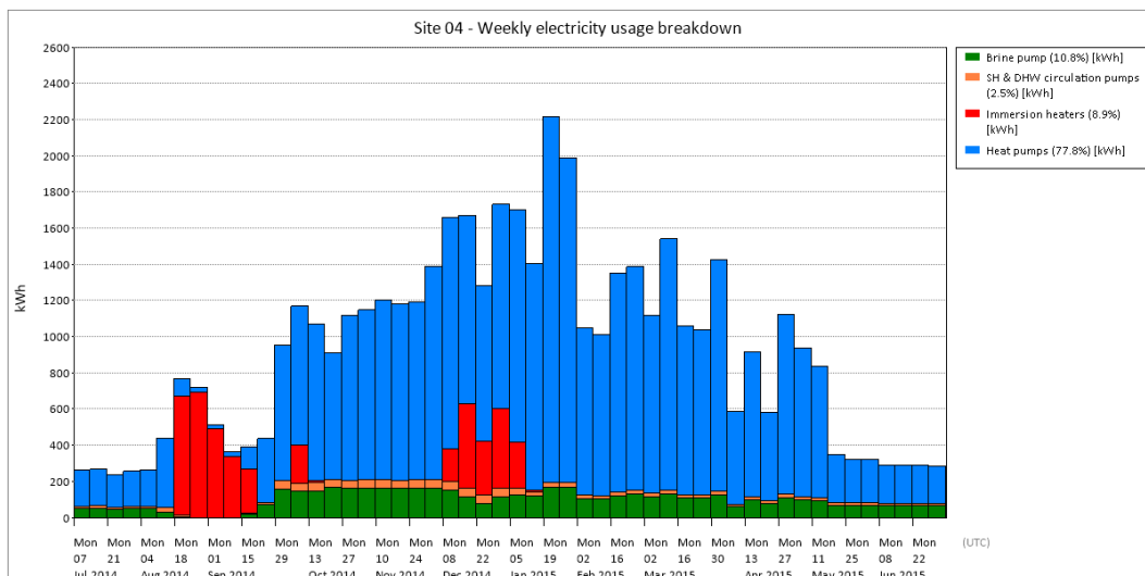
Figure T 170 – Site 04 electricity breakdown
