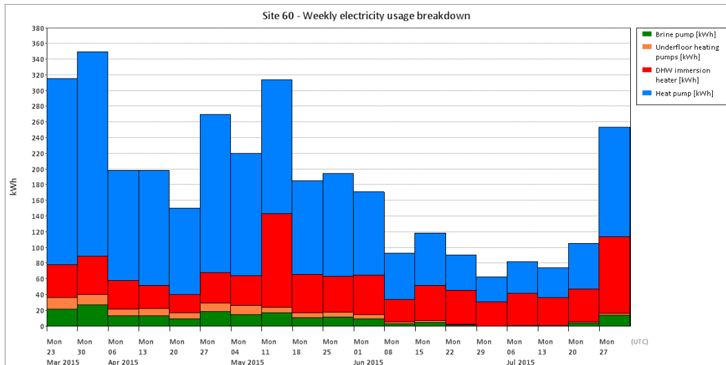
Figure T 187 – Site 60 electricity breakdown
