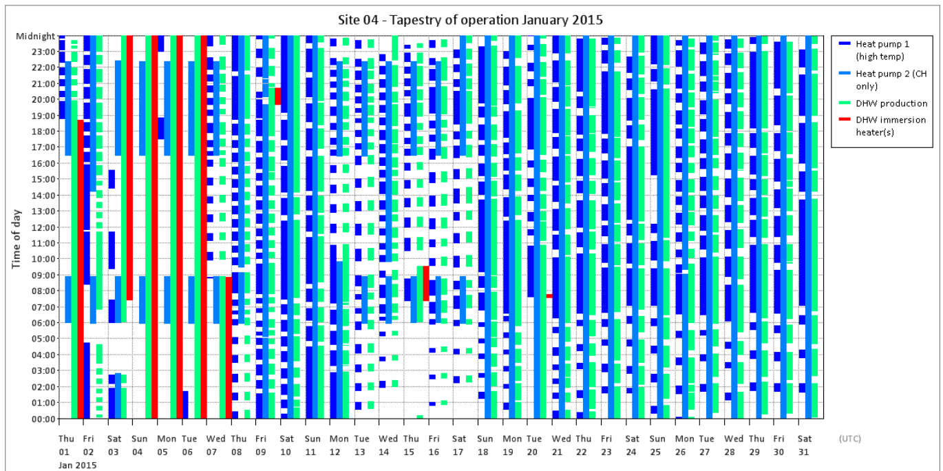
Figure T 87 – Site 04 tapestries of operation
