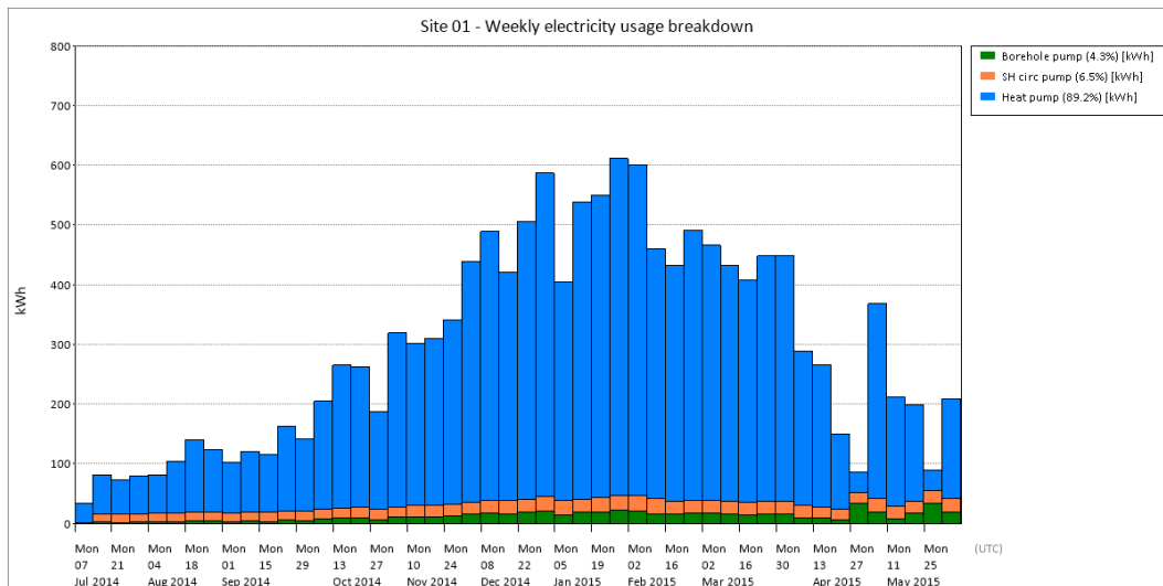
Figure T 169 – Site 01 electricity breakdown
