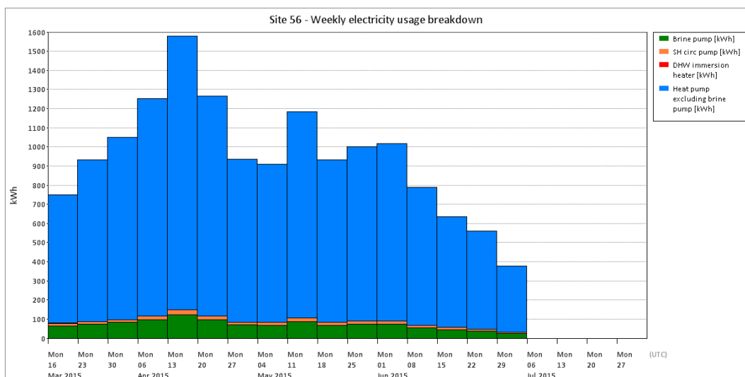
Figure T 185 – Site 56 electricity breakdown
