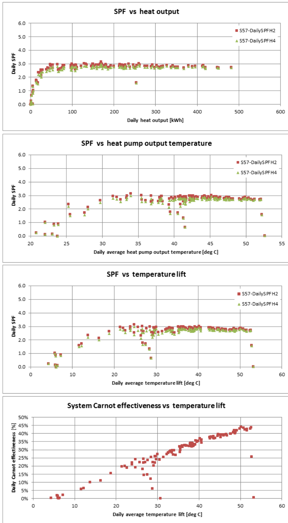
Figure T 78 – Site 57 system efficiency charts (2)
