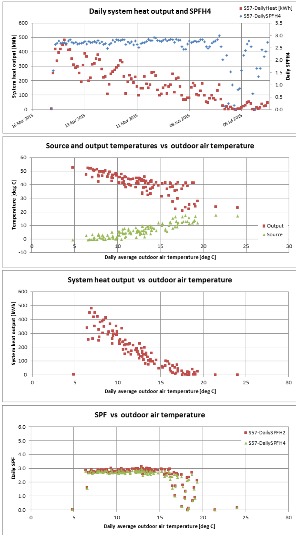
Figure T 77 – Site 57 system efficiency charts (1)
