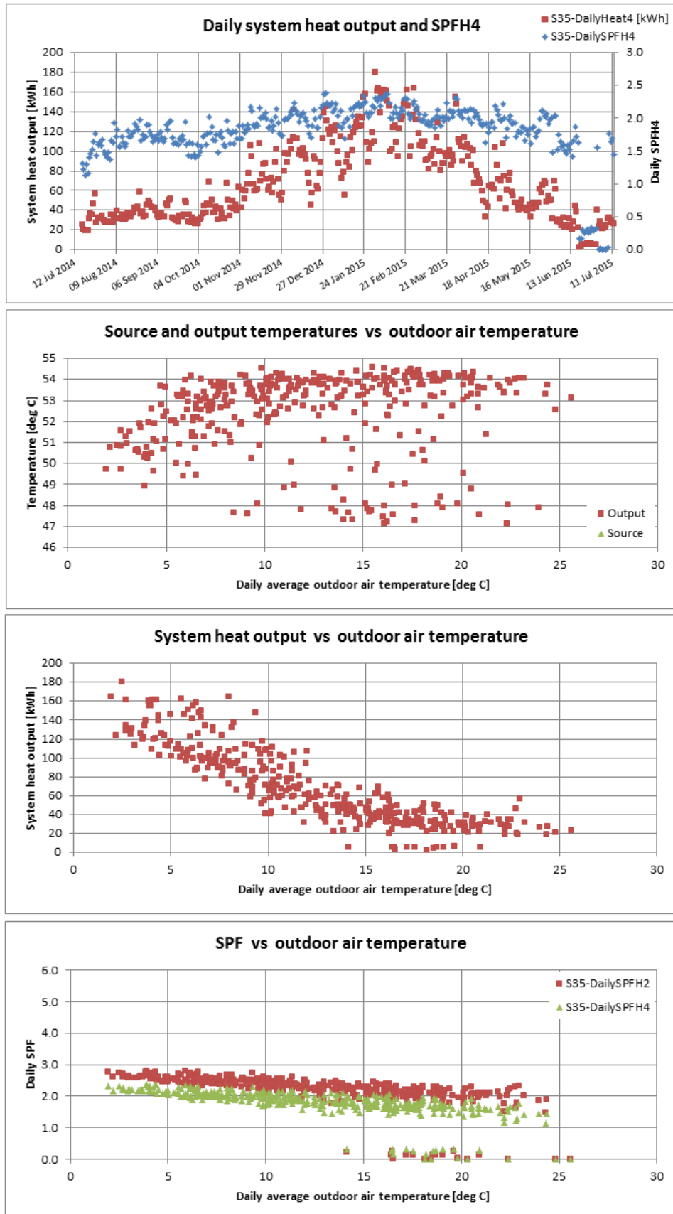
Figure T 61 – Site 35 system efficiency charts (1)
