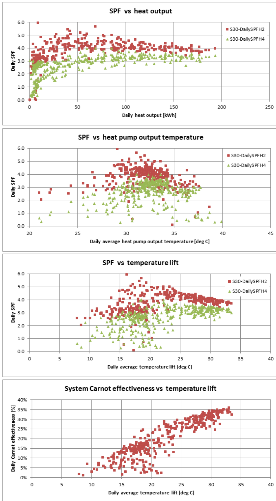
Figure T 56 – Site 30 system efficiency charts (2)
