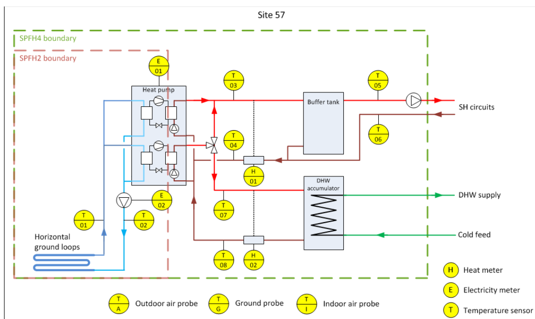
Figure T 26 – Site 57 system schematic
