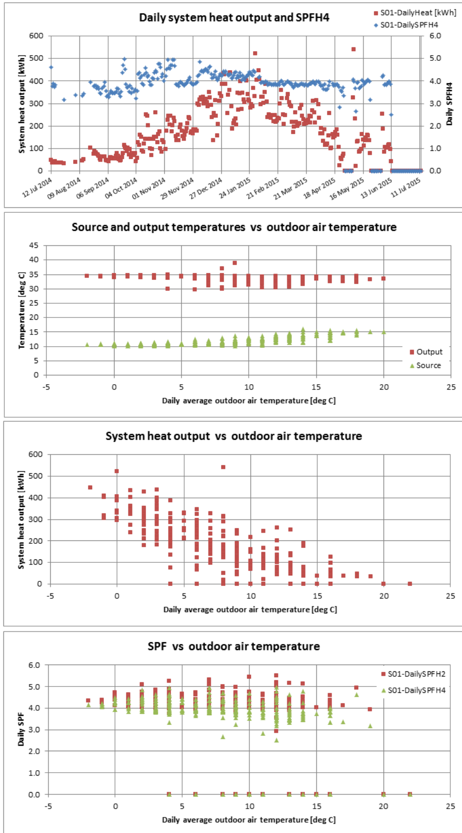
Figure T 29 – Site 01 system efficiency charts (1)
