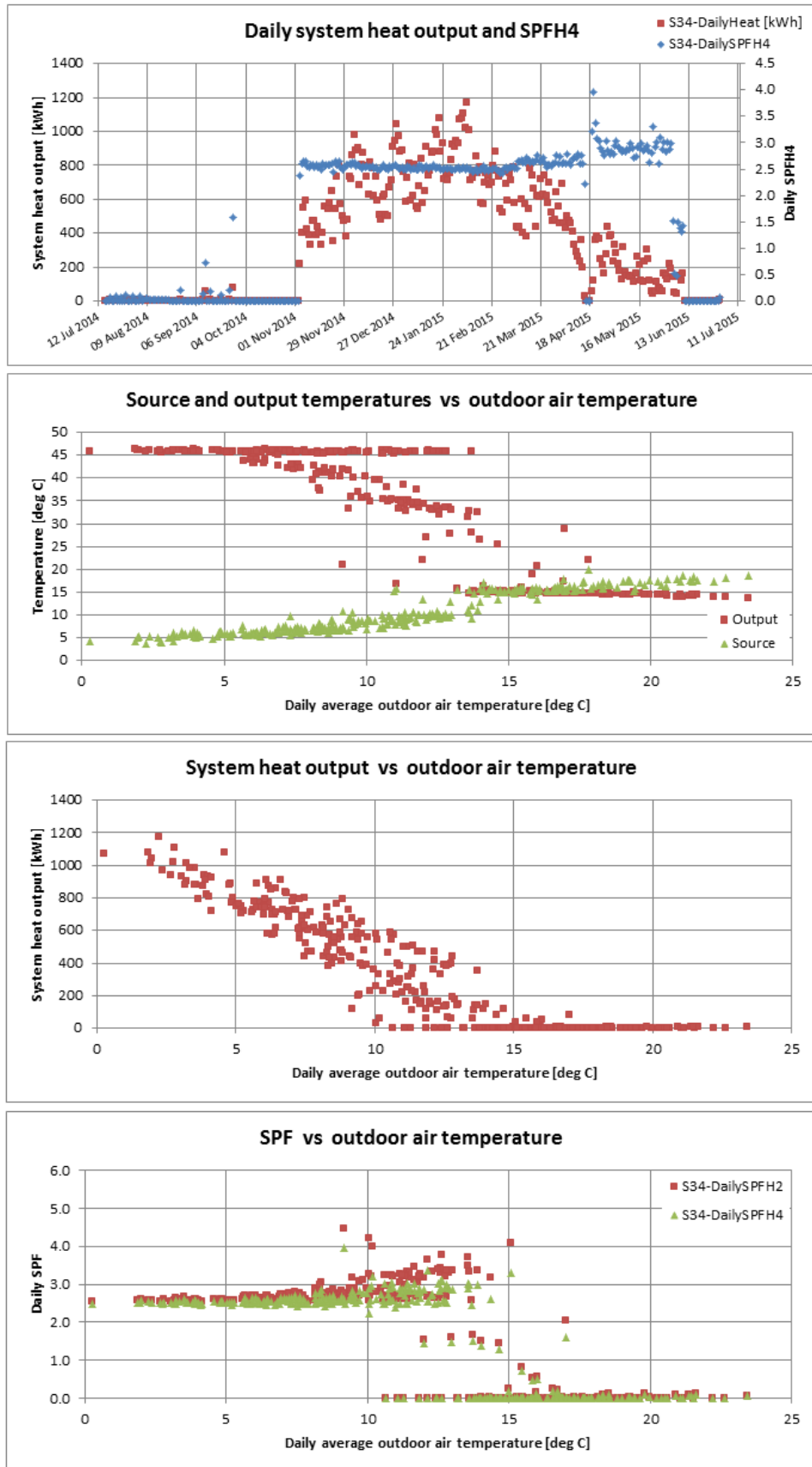
Figure T 59 – Site 34 system efficiency charts (1)
