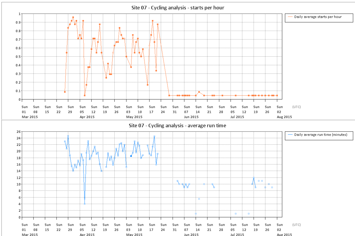
Figure T 117 – Site 07 cycling analysis
