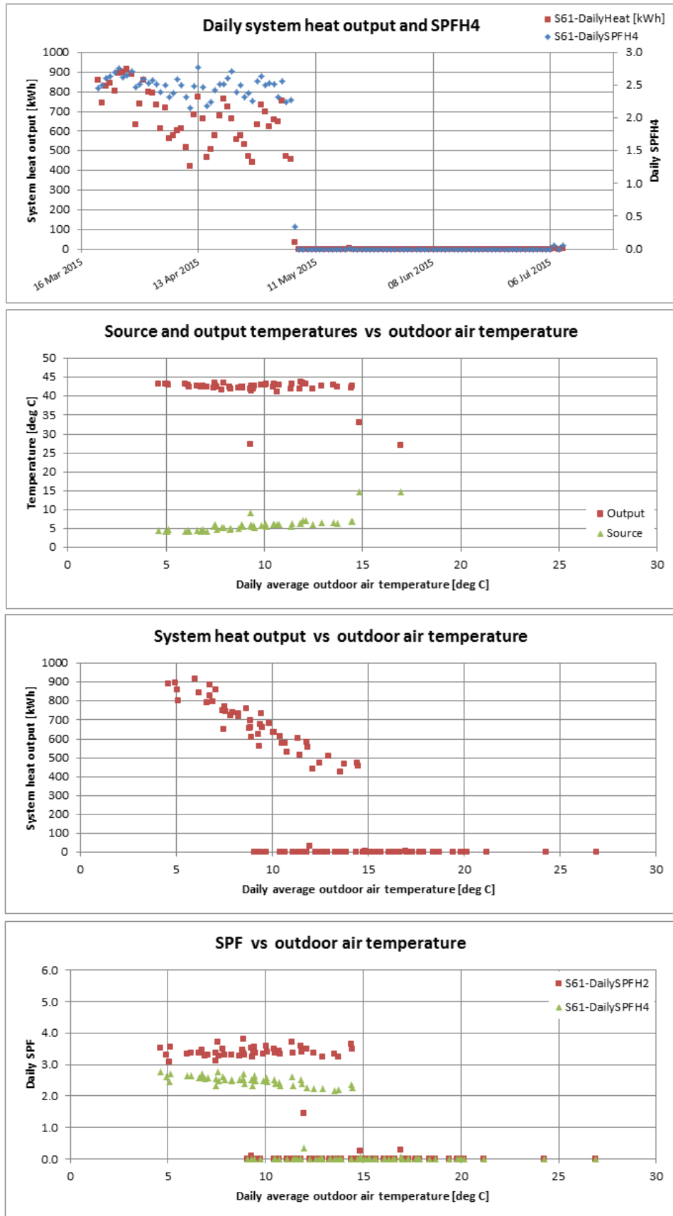
Figure T 81 – Site 61 system efficiency charts (1)
