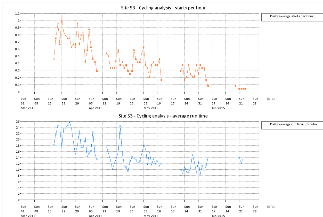
Figure T 135 – Site 53 cycling analysis
