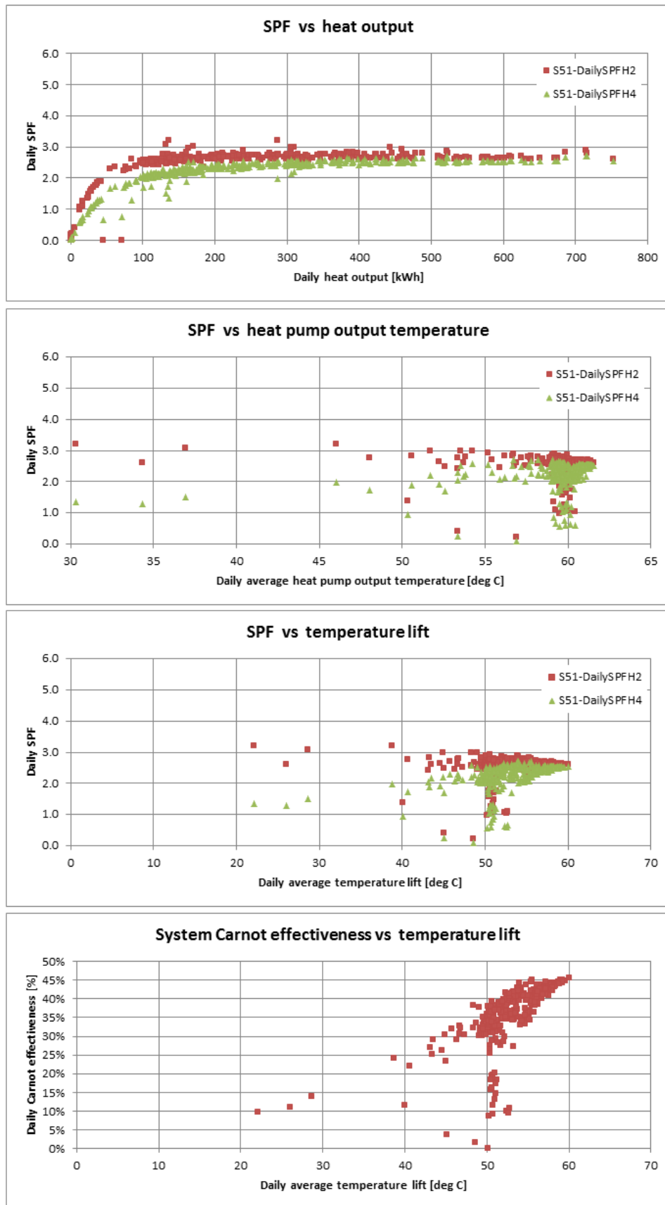
Figure T 72 – Site 51 system efficiency charts (2)
