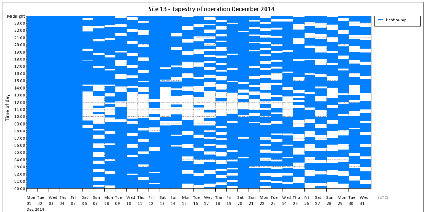
Figure T 91 – Site 13 tapestries of operation
