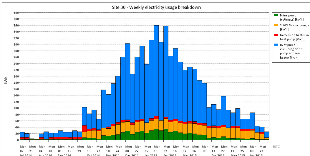
Figure T 180 – Site 30 electricity breakdown
