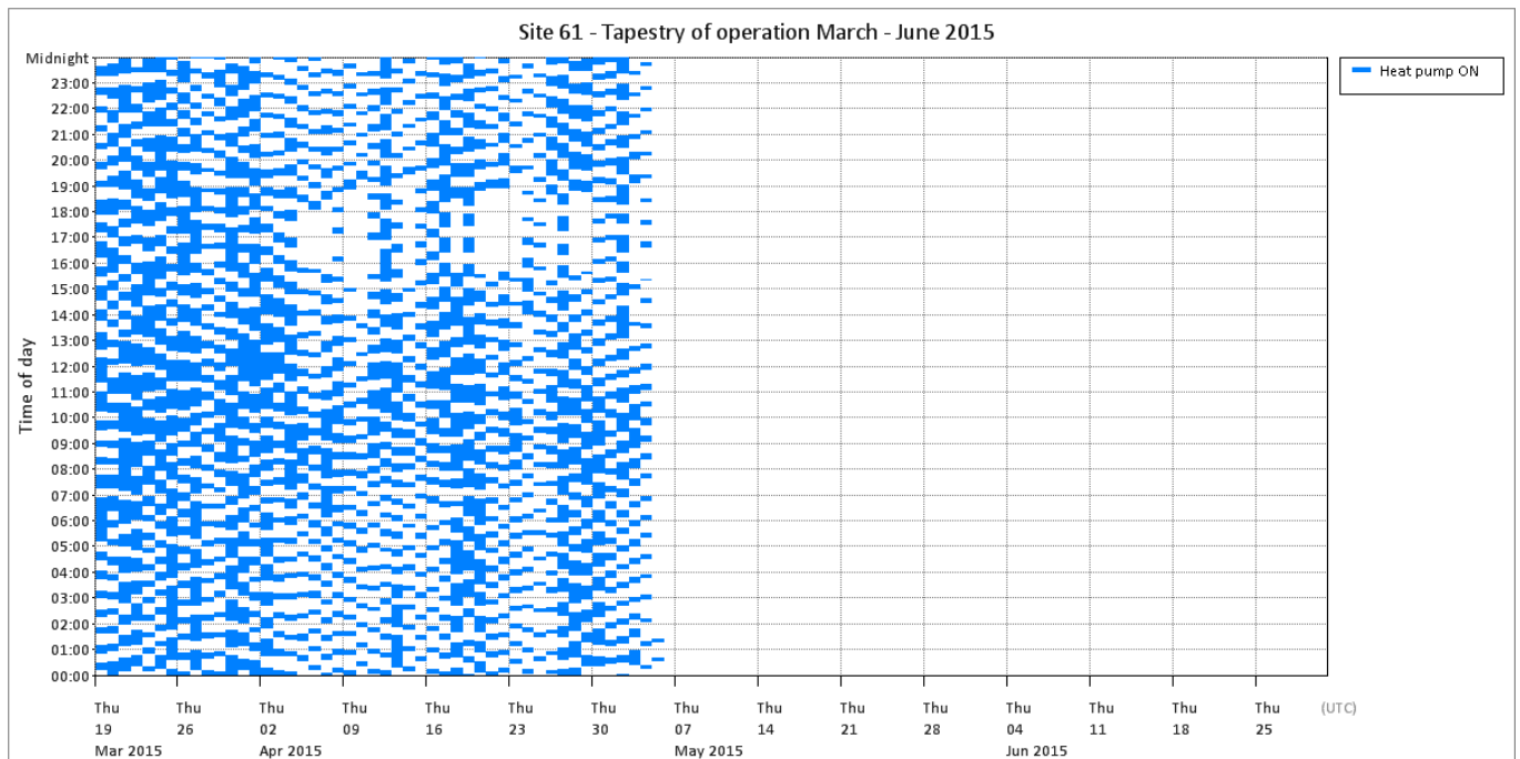
Figure T 111 – Site 61 tapestry of operation
