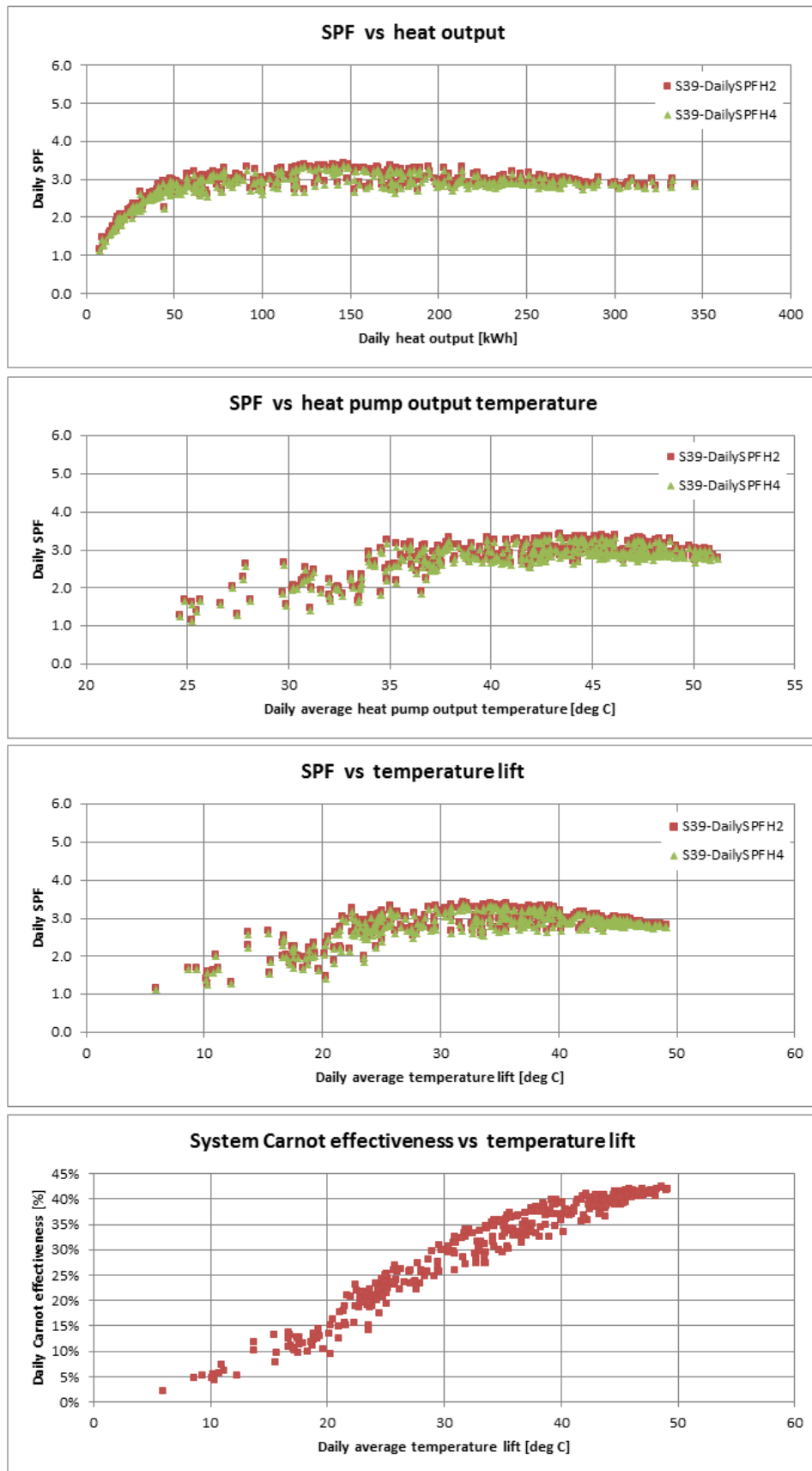
Figure T 66 – Site 39 system efficiency charts (2)
