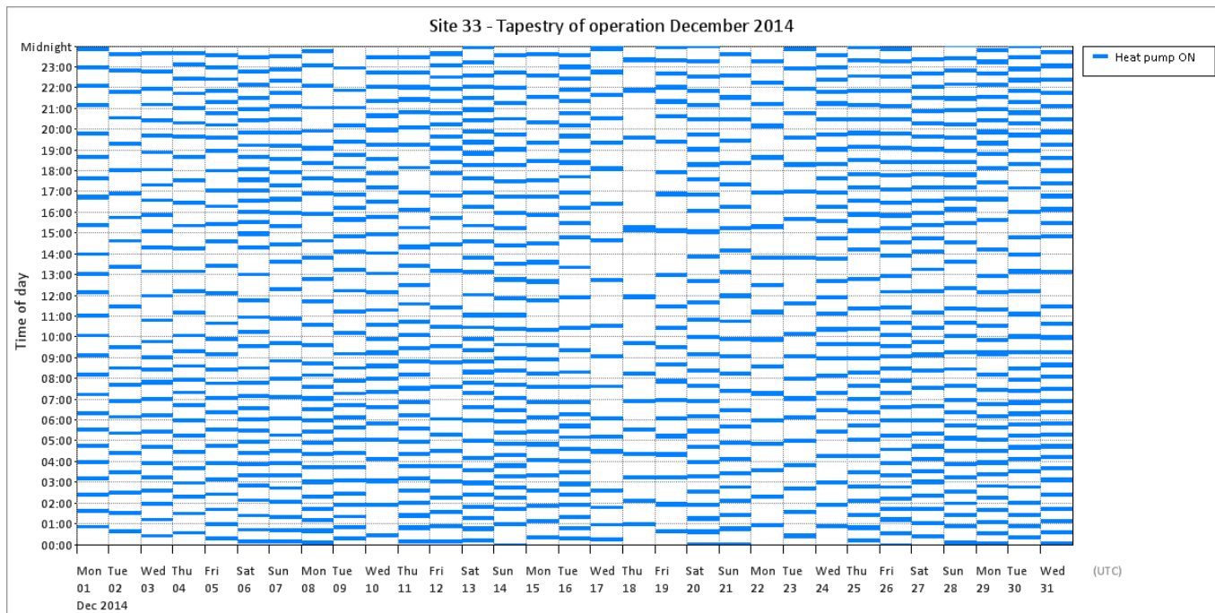
Figure T 99 – Site 33 tapestries of operation
