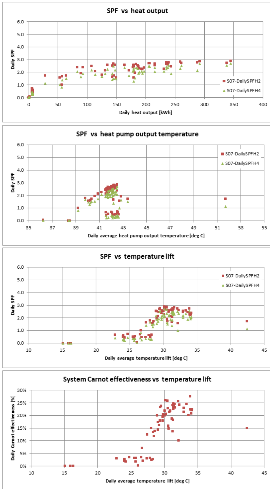
Figure T 38 – Site 07 system efficiency charts (2)
