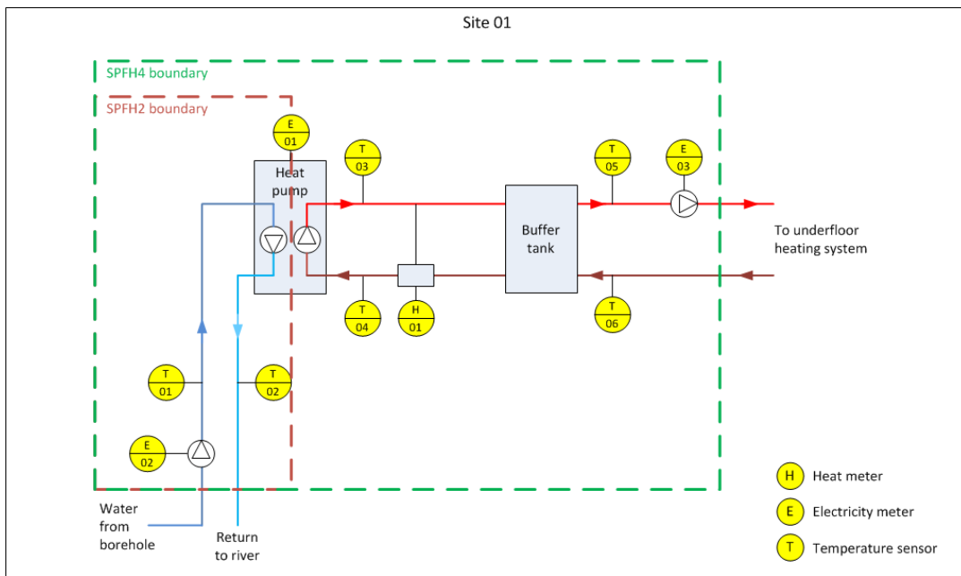
Figure T 1 – Site 01 system schematic
