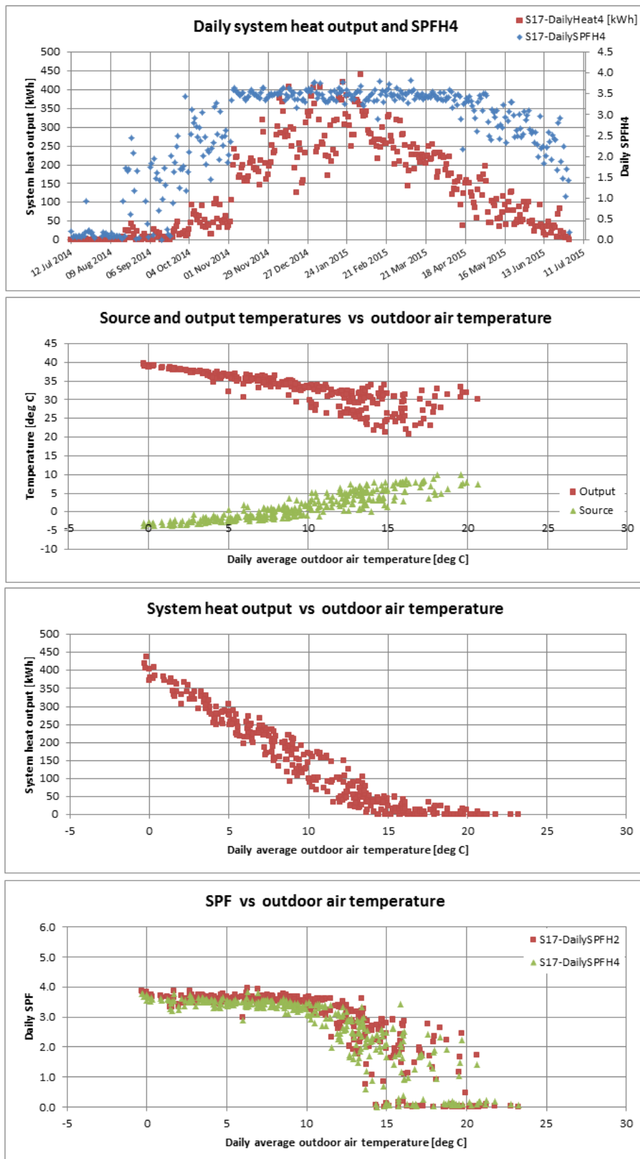
Figure T 45 – Site 17 system efficiency charts (1)
