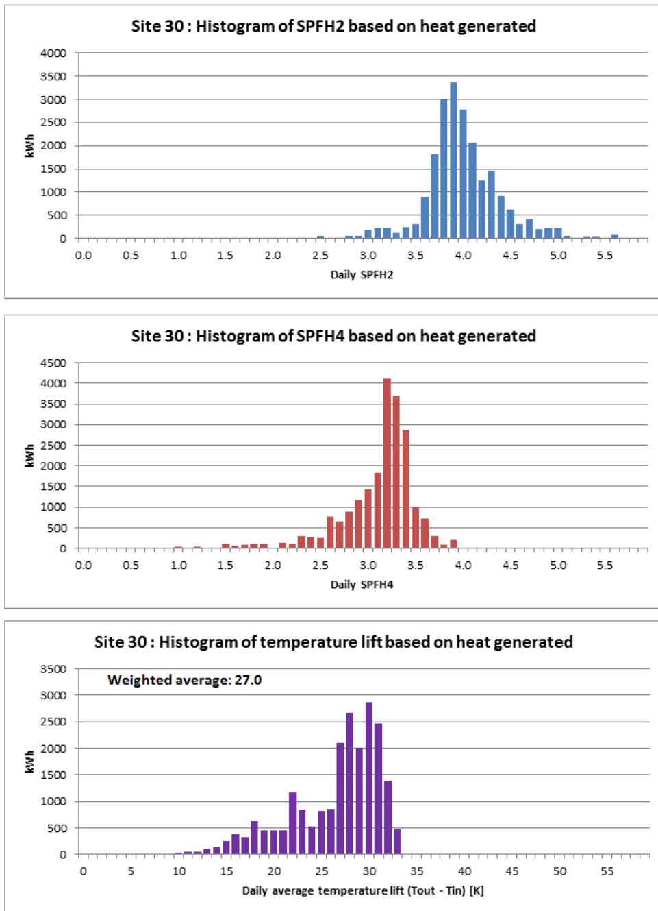
Figure T 154 – Site 30 histograms of SPF H2 , SPF H4 and temperature lift
