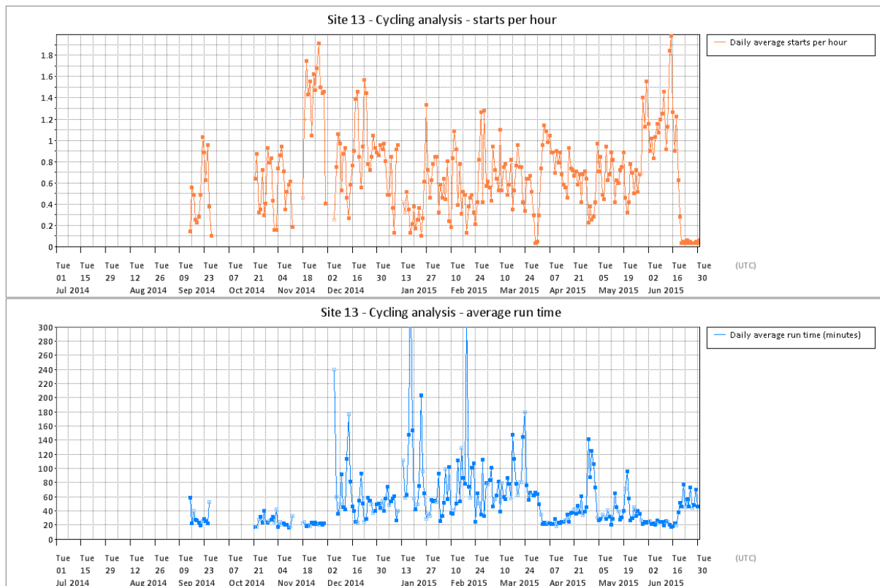
Figure T 119 – Site 13 cycling analysis
