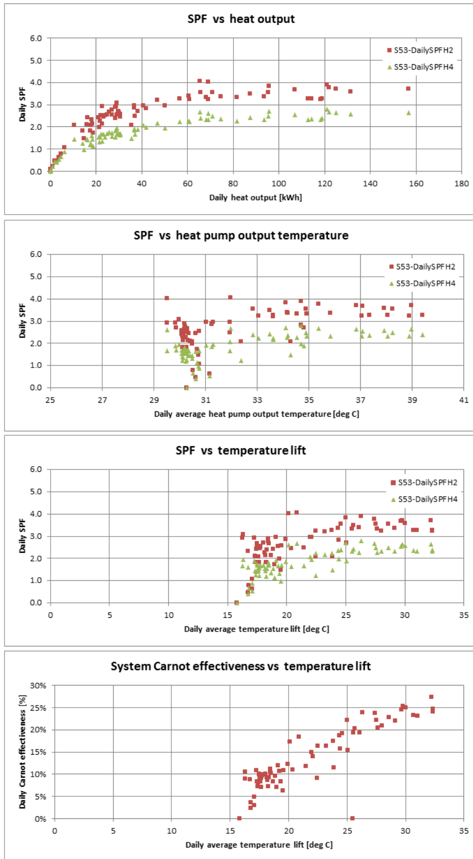
Figure T 74 – Site 53 system efficiency charts (2)
