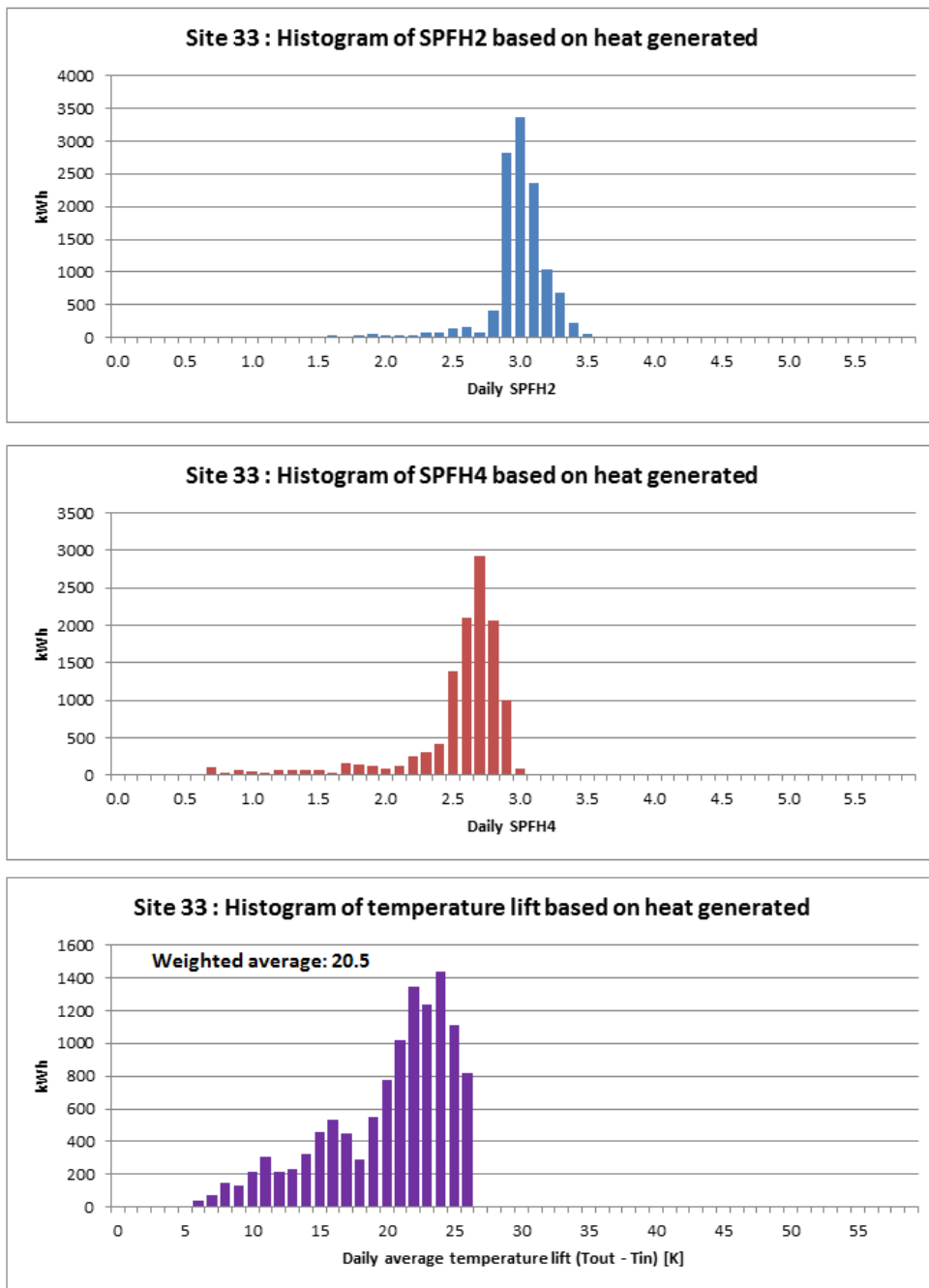
Figure T 155 – Site 33 histograms of SPF H2 , SPF H4 and temperature lift
