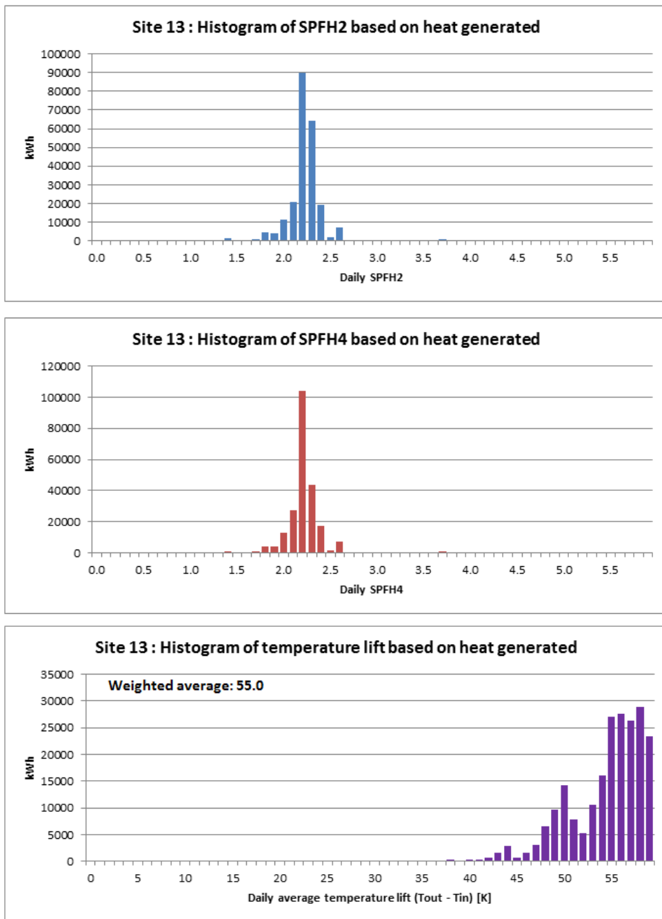
Figure T 147 – Site 13 histograms of SPF H2 , SPF H4 and temperature lift
