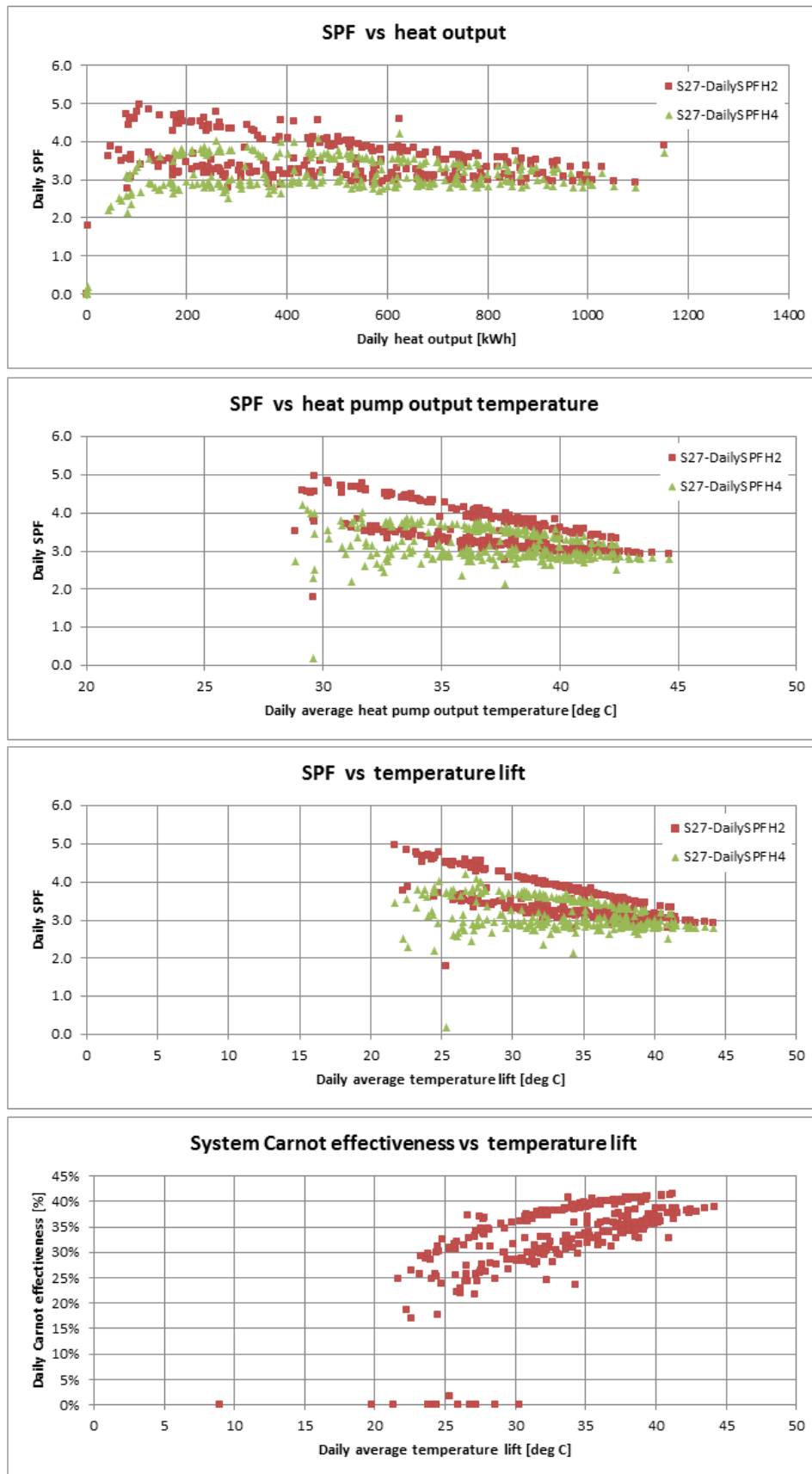
Figure T 50 – Site 27 system efficiency charts (2)
