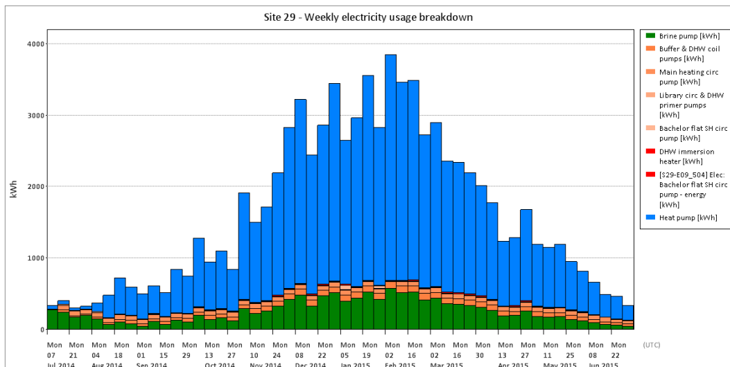
Figure T 179 – Site 29 electricity breakdown
