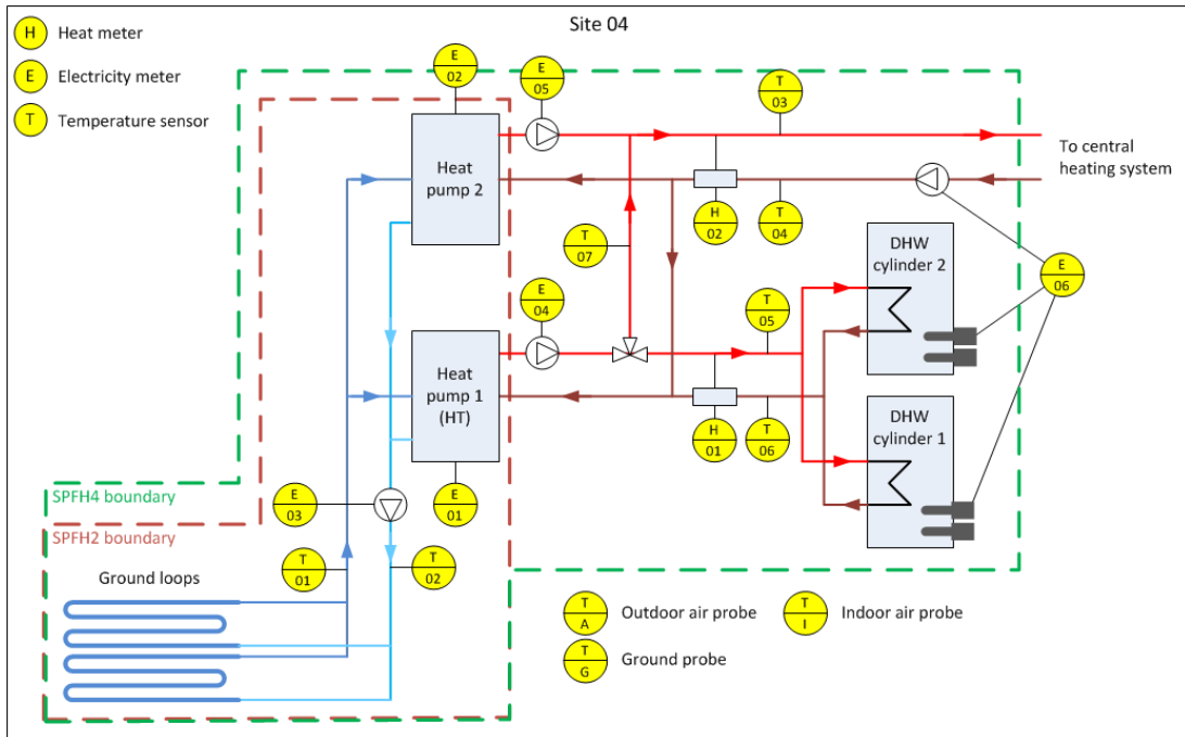
Figure T 3 – Site 04 system schematic
