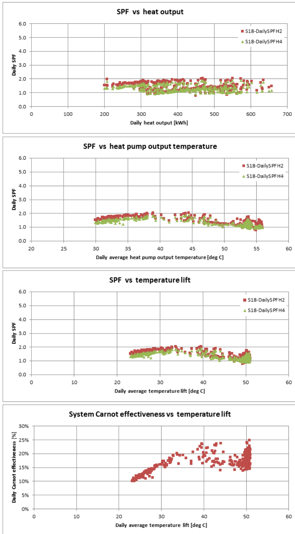
Figure T 48 – Site 18 system efficiency charts (2)
