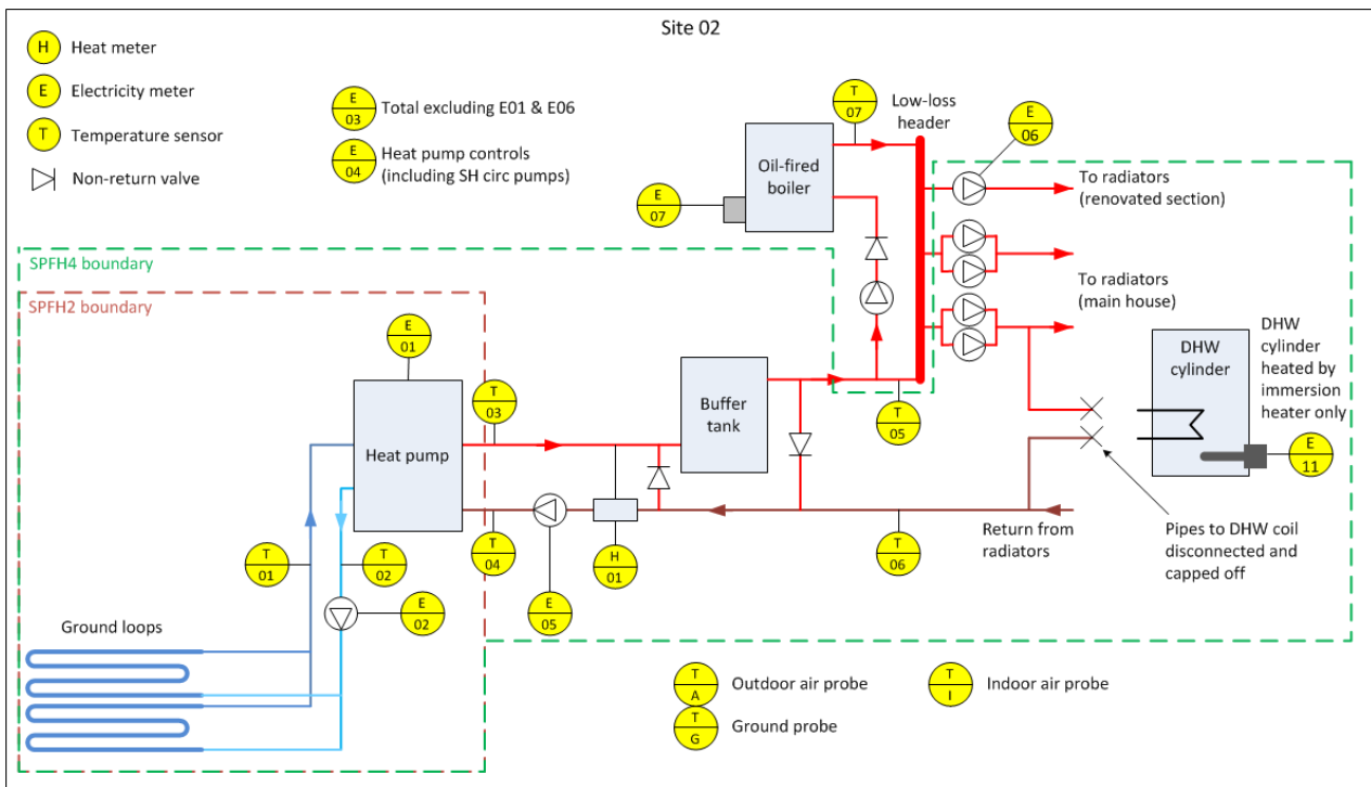
Figure T 2 – Site 02 system schematic
