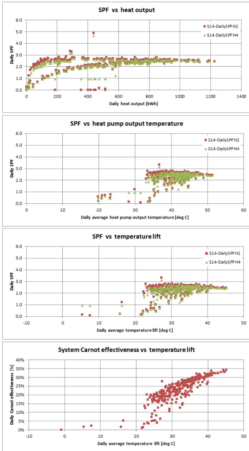
Figure T 44 – Site 14 system efficiency charts (2)
