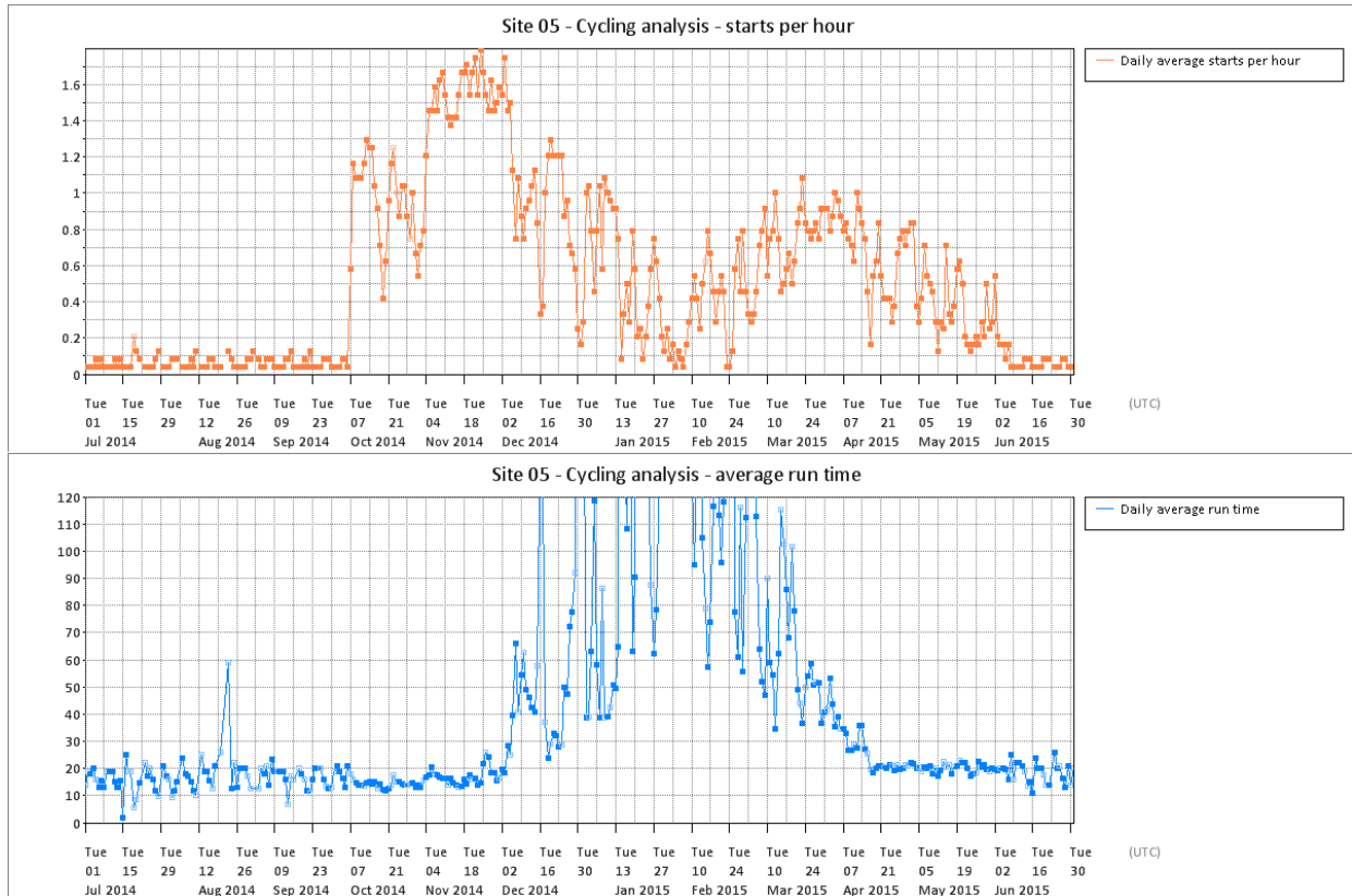
Figure T 116 – Site 05 cycling analysis
