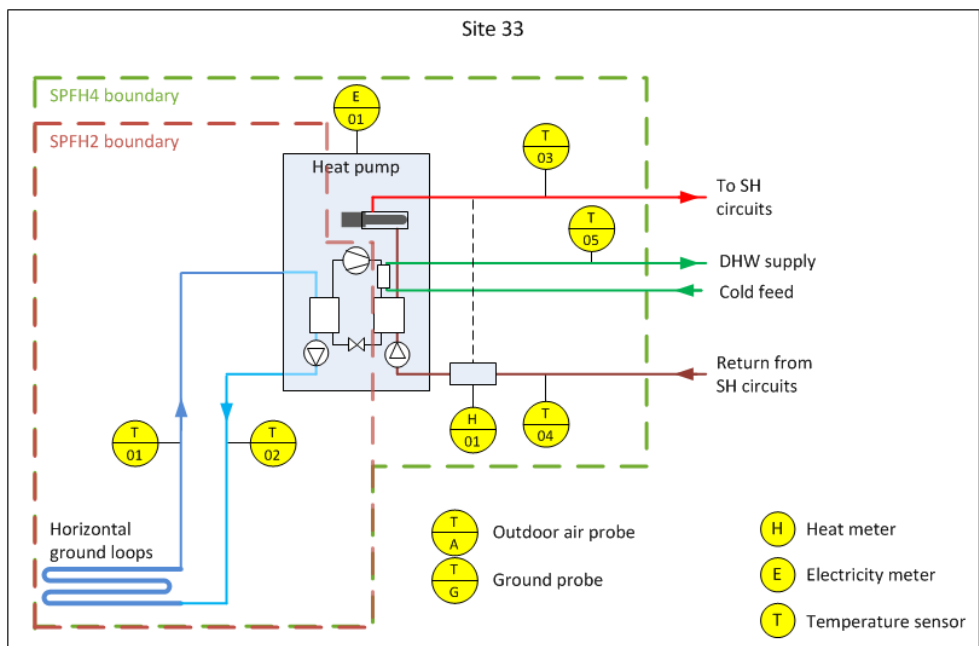
Figure T 15 – Site 33 system schematic
