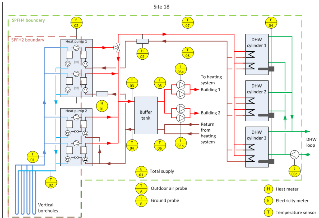
Figure T 10 – Site 18 system schematic
