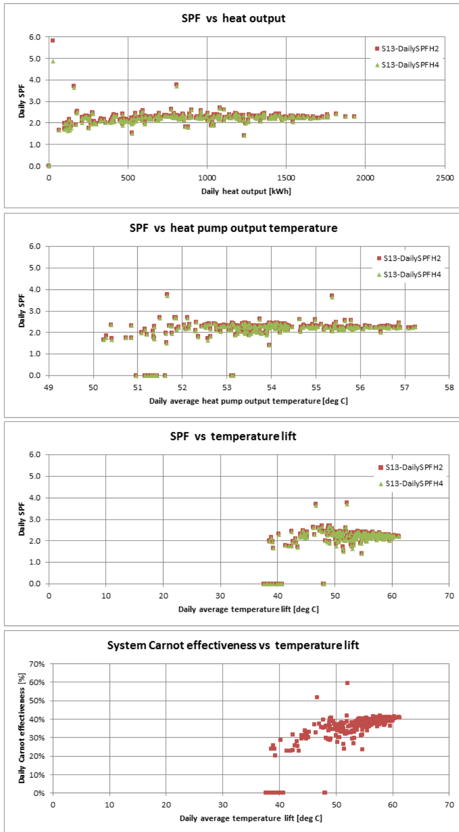
Figure T 42 – Site 13 system efficiency charts (2)
