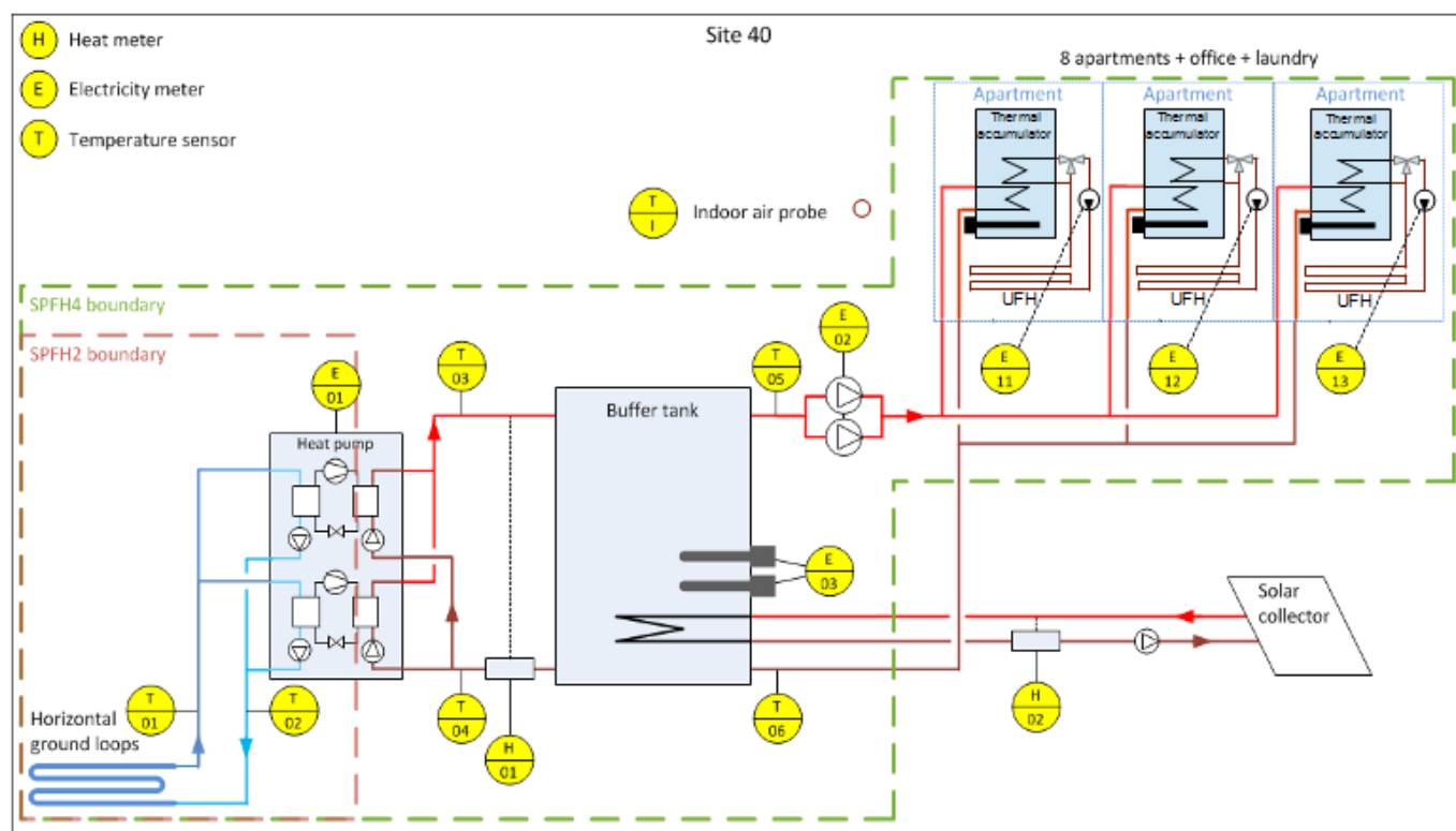
Figure T 20 – Site 40 system schematic
