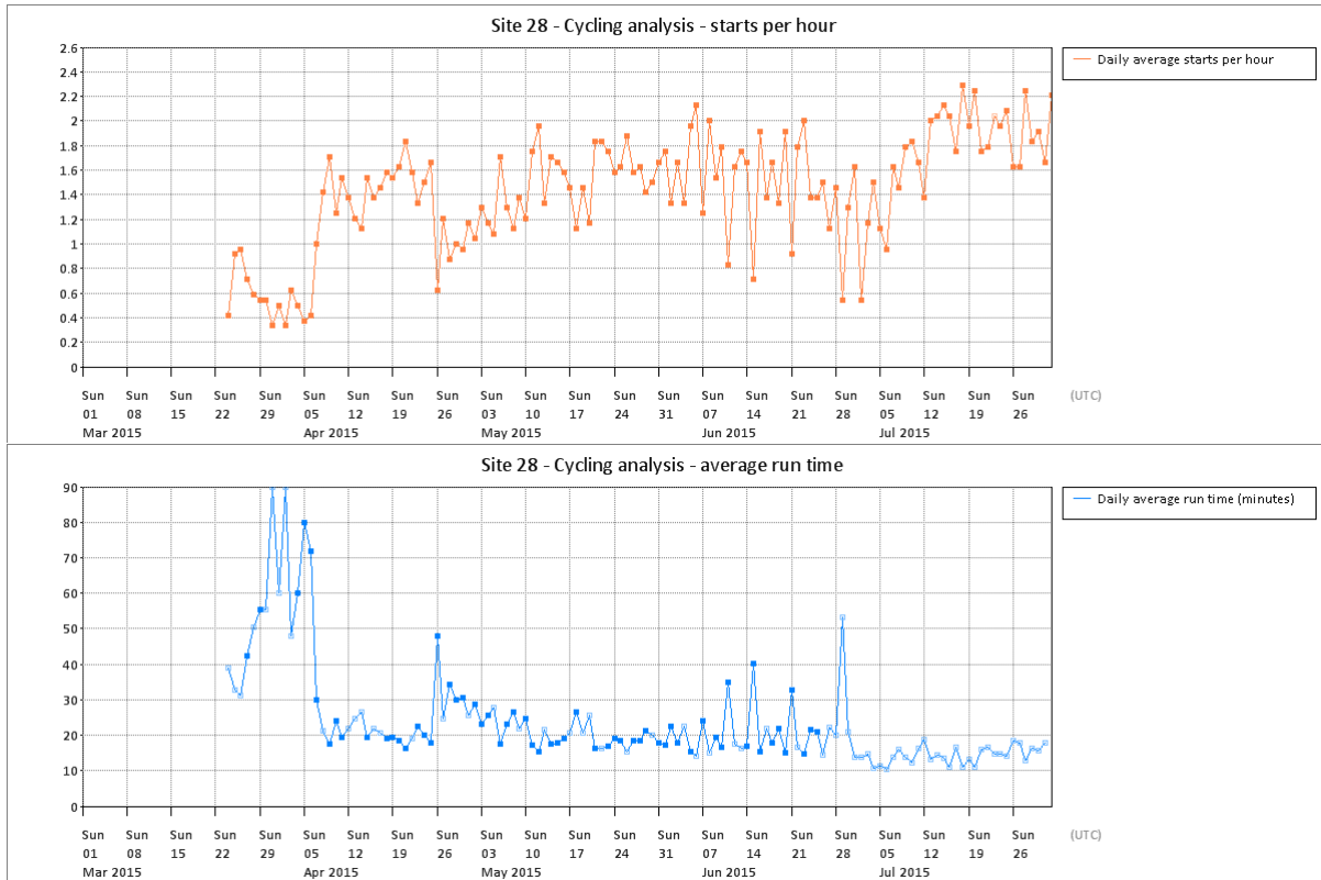
Figure T 124 – Site 28 cycling analysis
