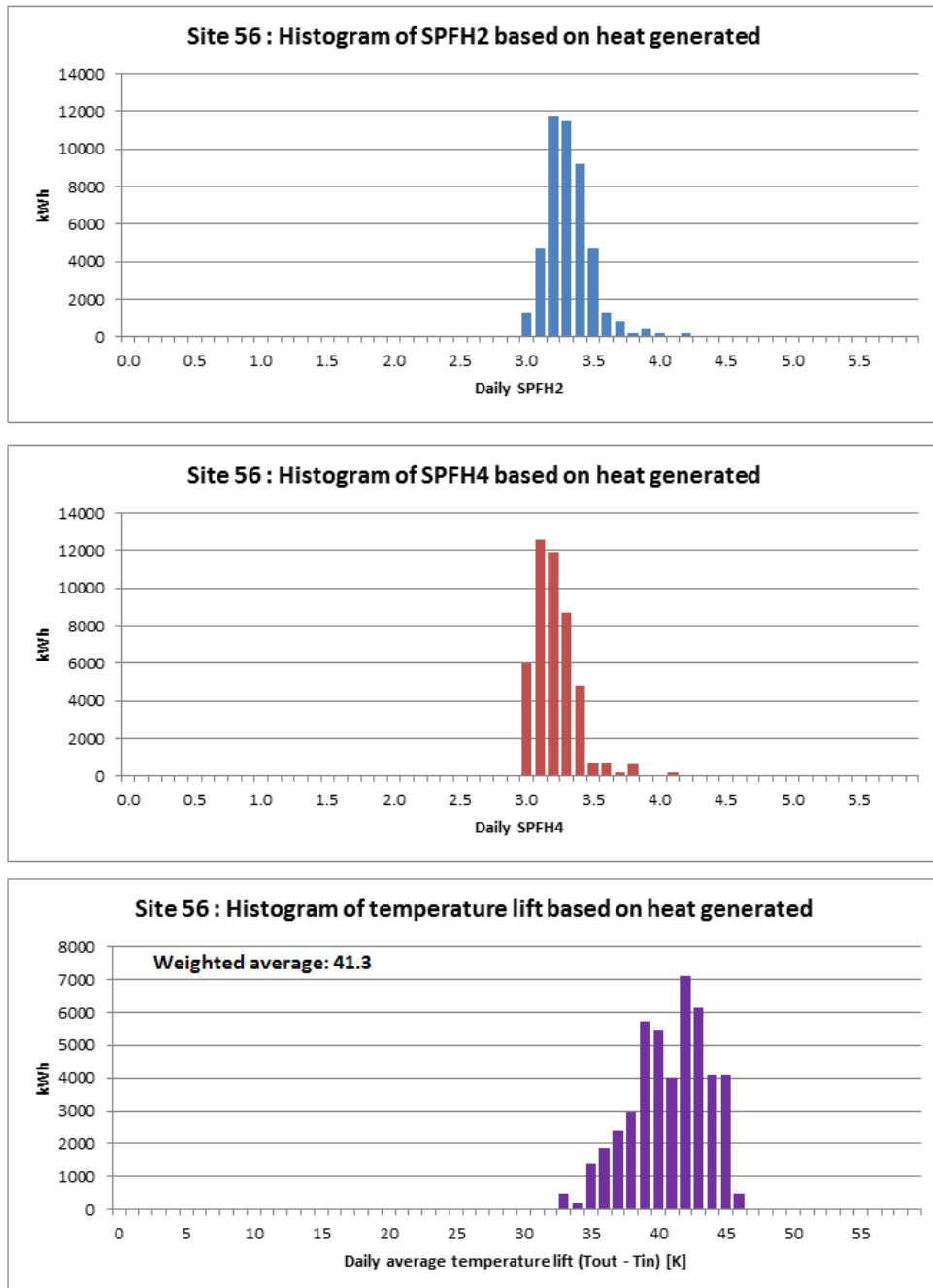
Figure T 164 – Site 56 histograms of SPF H2 , SPF H4 and temperature lift
