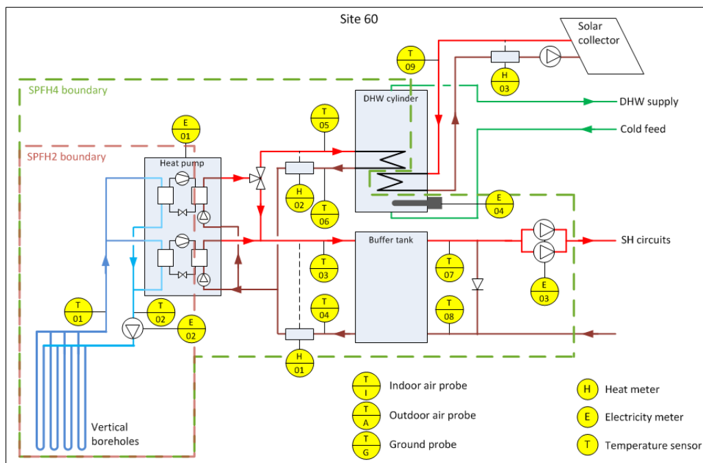
Figure T 27 – Site 60 system schematic
