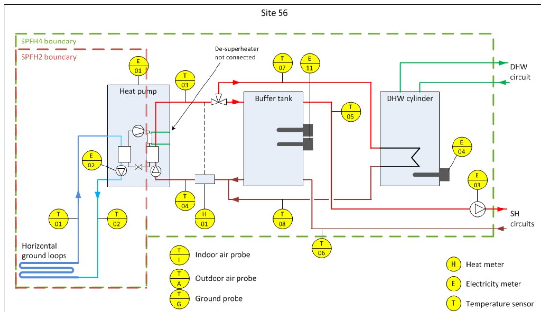
Figure T 25 – Site 56 system schematic
