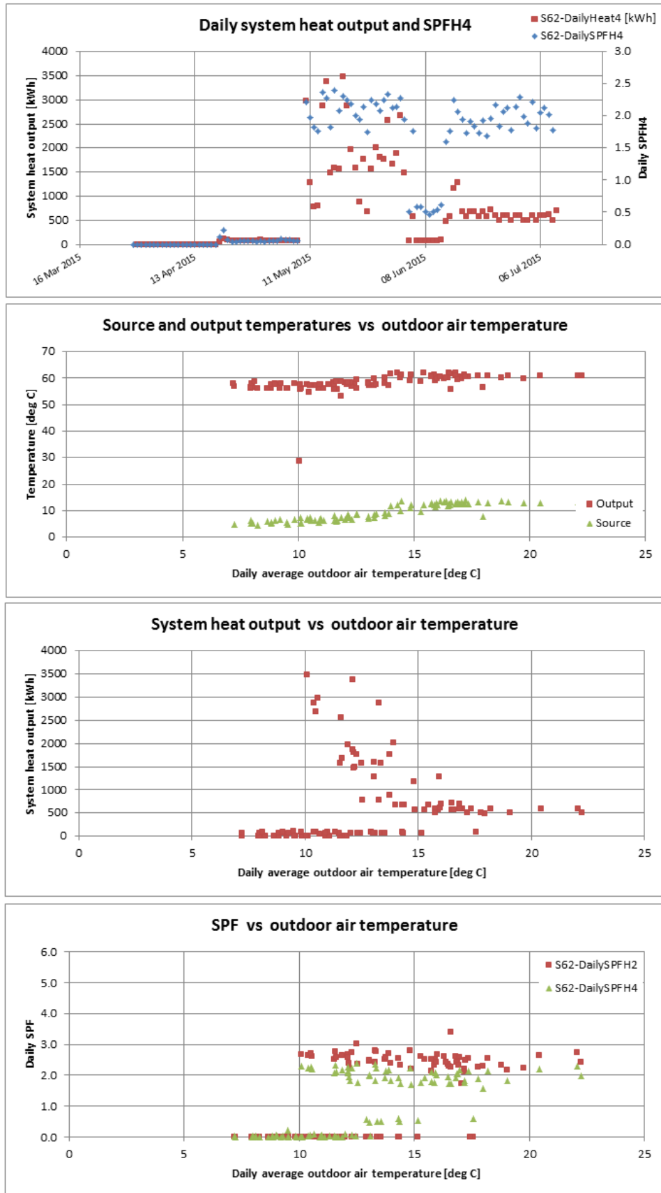
Figure T 83 – Site 62 system efficiency charts (1)
