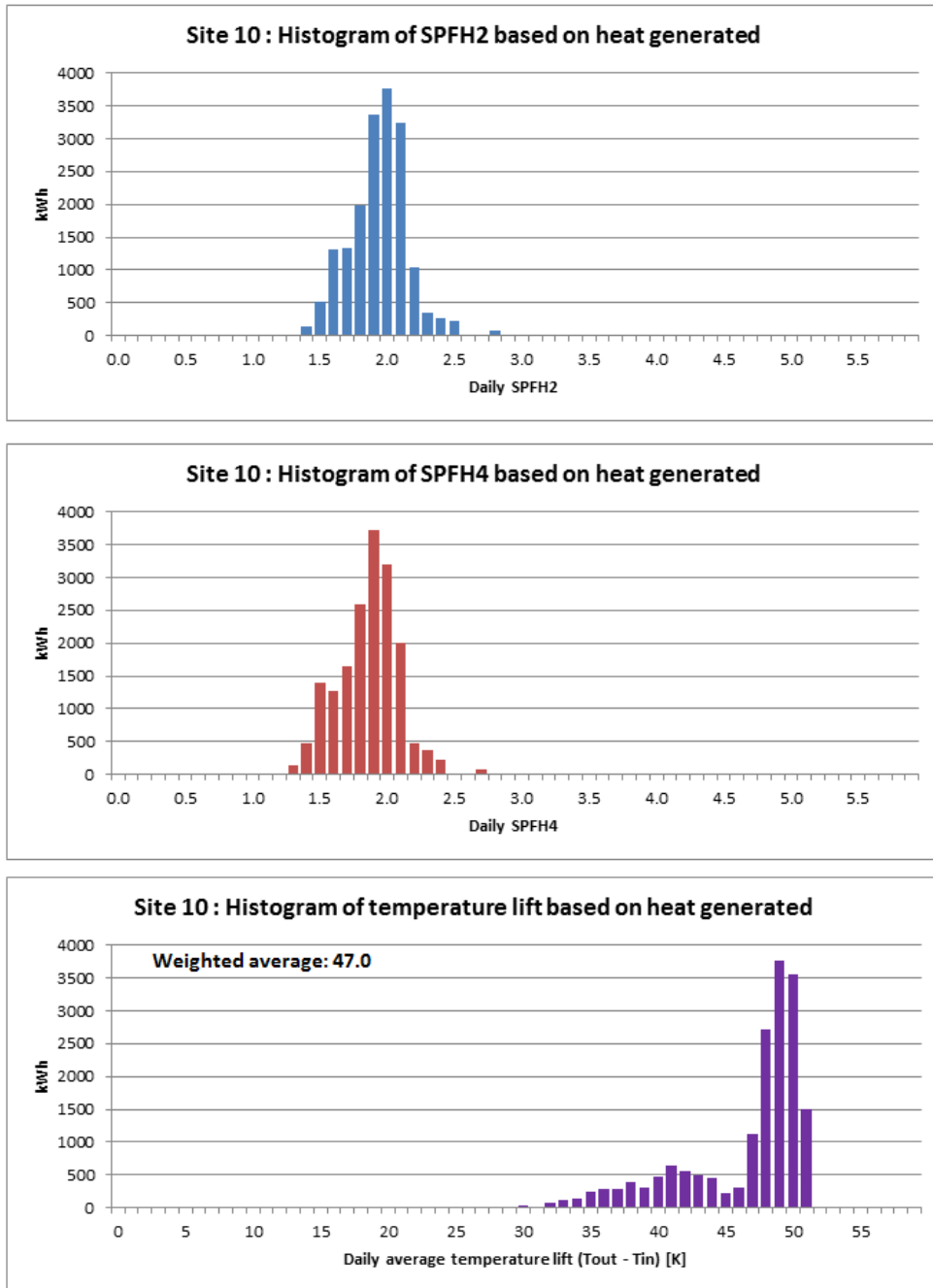
Figure T 146 – Site 10 histograms of SPF H2 , SPF H4 and temperature lift
