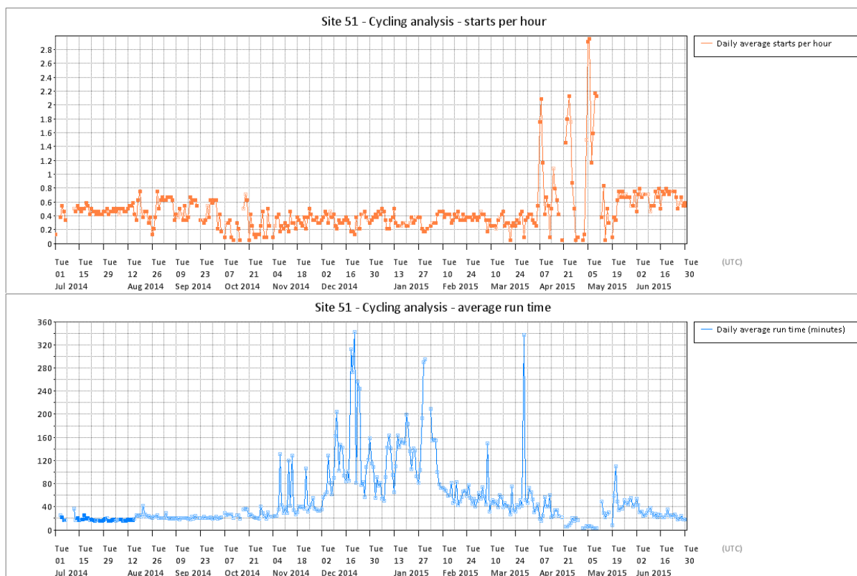
Figure T 134 – Site 51 cycling analysis
