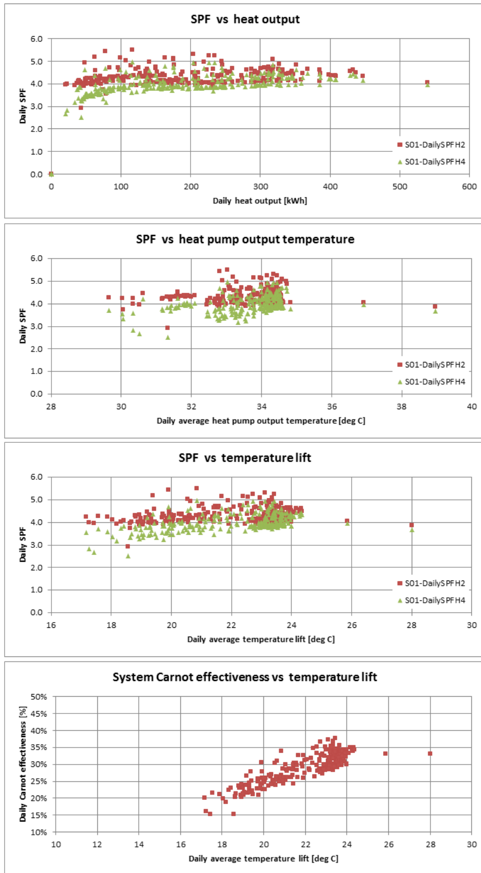
Figure T 30 – Site 01 system efficiency charts (2)
