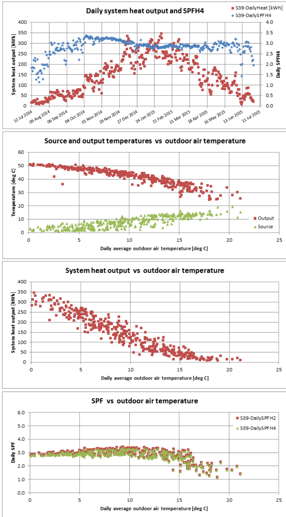
Figure T 65 – Site 39 system efficiency charts (1)
