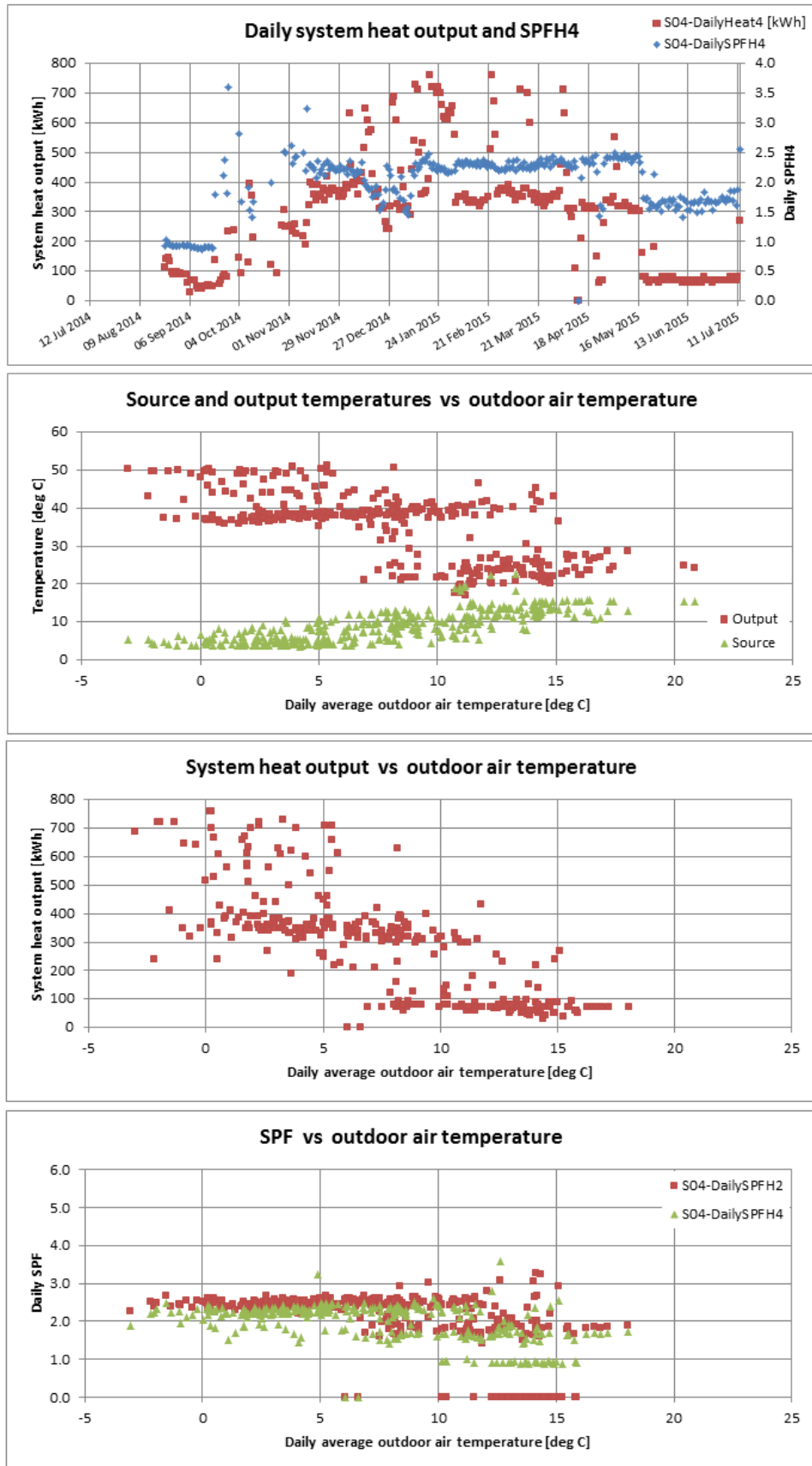
Figure T 33 – Site 04 system efficiency charts (1)
