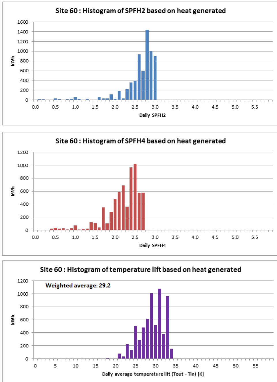
Figure T 166 – Site 60 histograms of SPF H2 , SPF H4 and temperature lift
