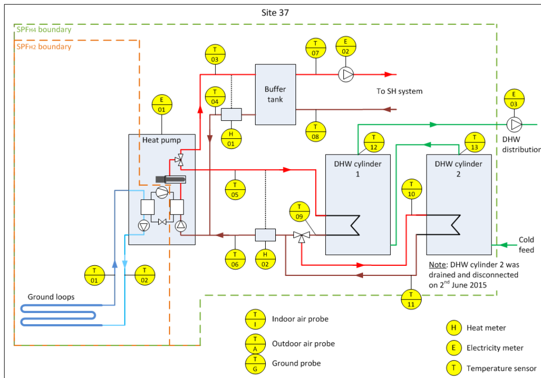
Figure T 18 – Site 37 system schematic
