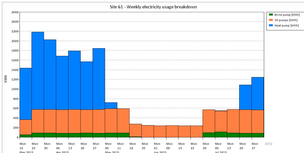
Figure T 188 – Site 61 electricity breakdown
