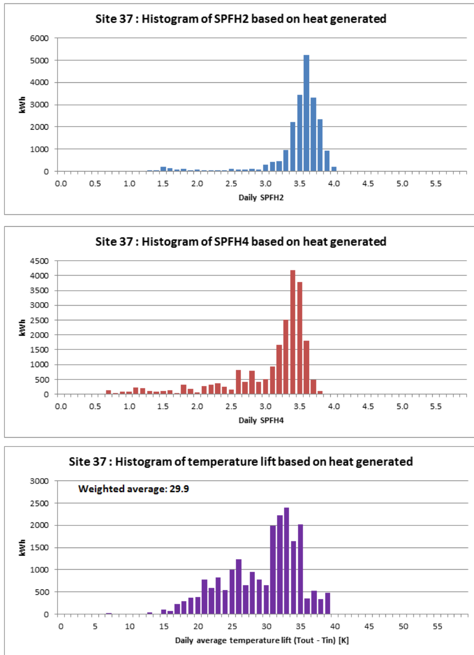
Figure T 158 – Site 37 histograms of SPF H2 , SPF H4 and temperature lift
