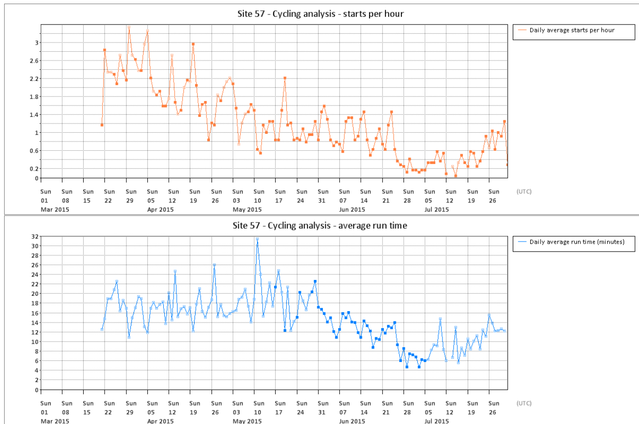
Figure T 137 – Site 57 cycling analysis
