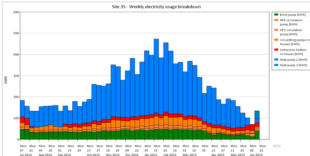
Figure T 182 – Site 35 electricity breakdown
