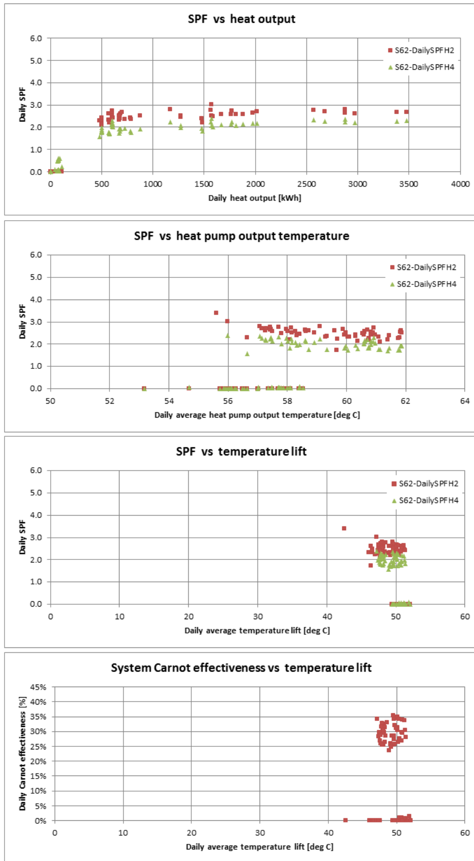
Figure T 84 – Site 62 system efficiency charts (2)
