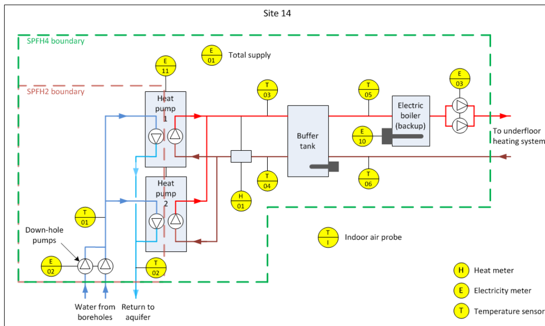
Figure T 8 – Site 14 system schematic
