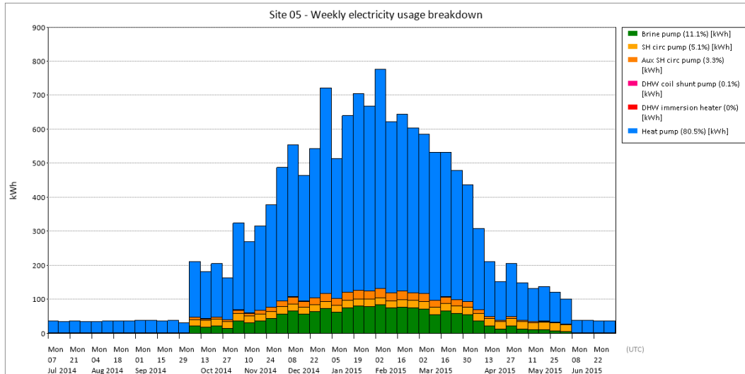
Figure T 171 – Site 05 electricity breakdown
