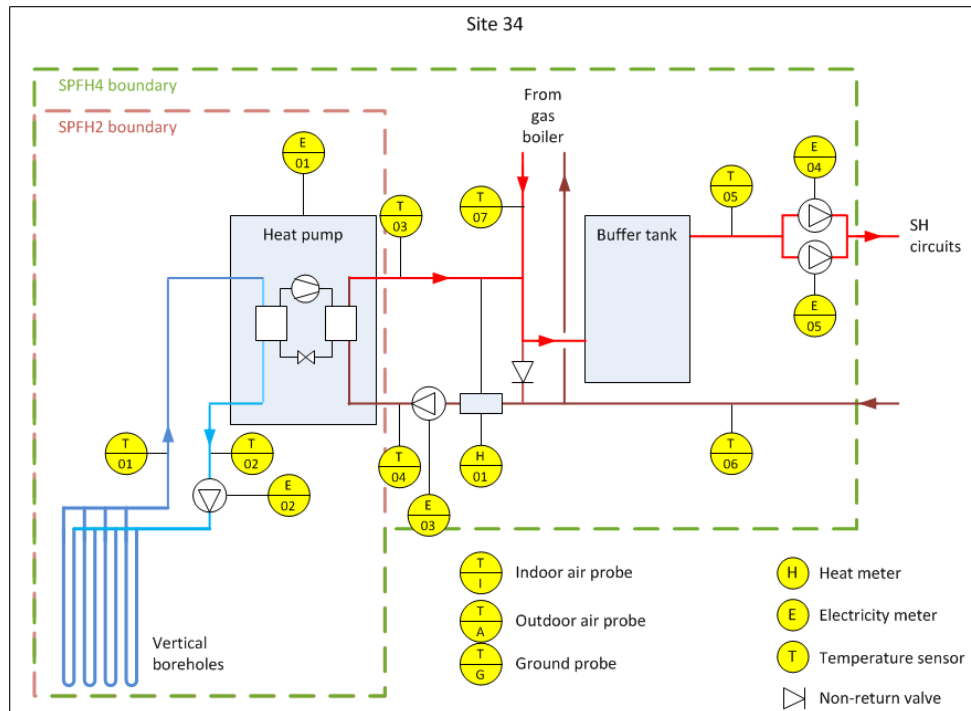
Figure T 16 – Site 34 system schematic
