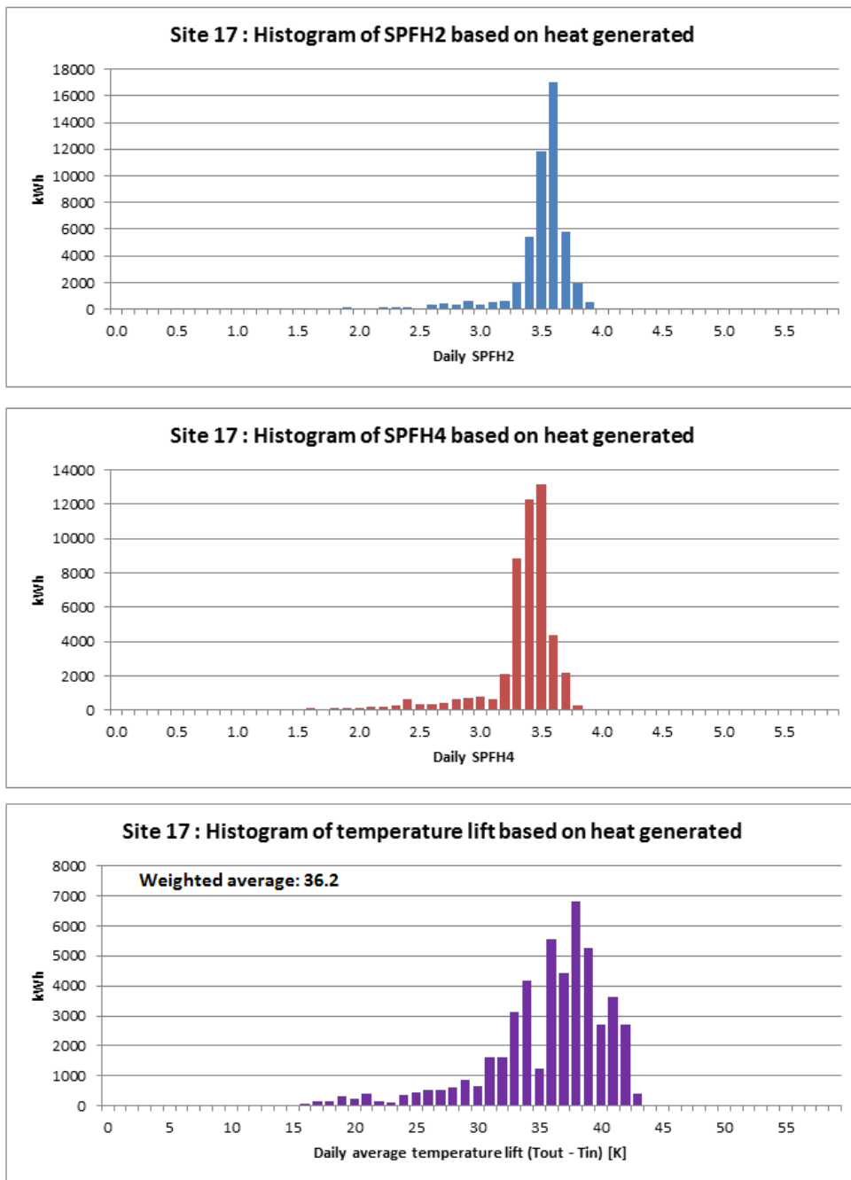
Figure T 149 – Site 17 histograms of SPF H2 , SPF H4 and temperature lift
