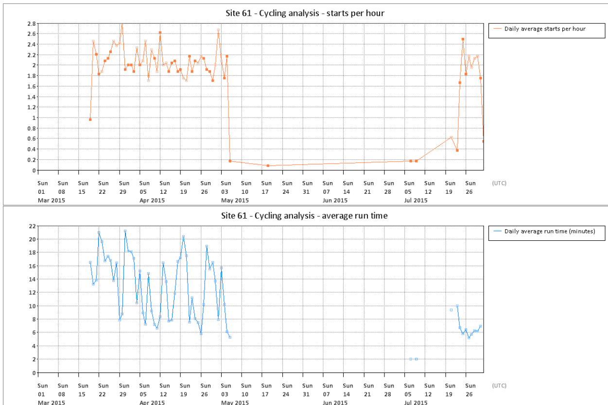
Figure T 139 – Site 61 cycling analysis
