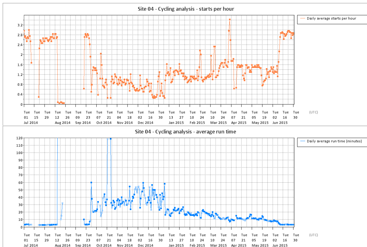
Figure T 115 – Site 04 cycling analysis
