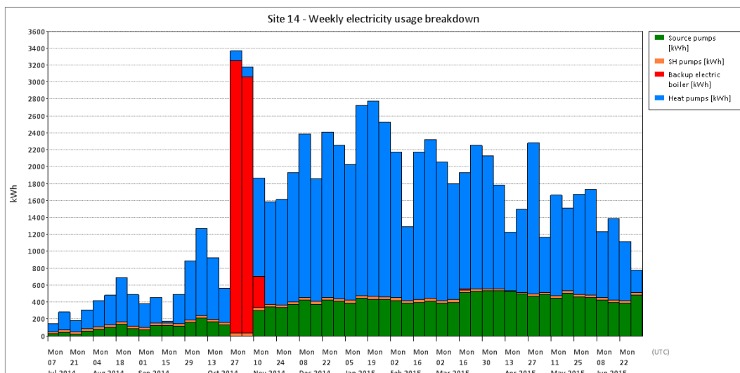
Figure T 175 – Site 14 electricity breakdown
