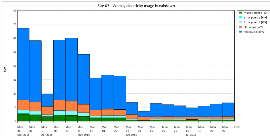
Figure T 189 – Site 62 electricity breakdown
