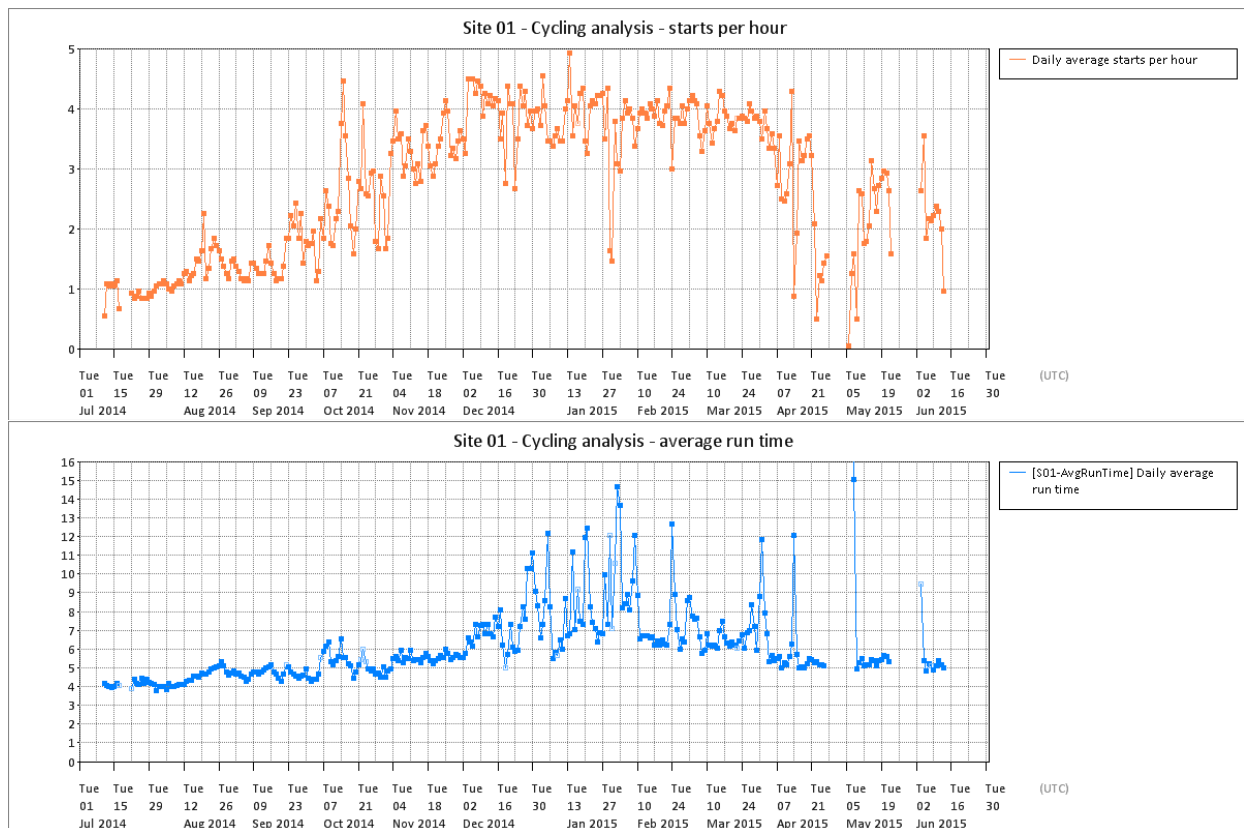
Figure T 113 – Site 01 cycling analysis
