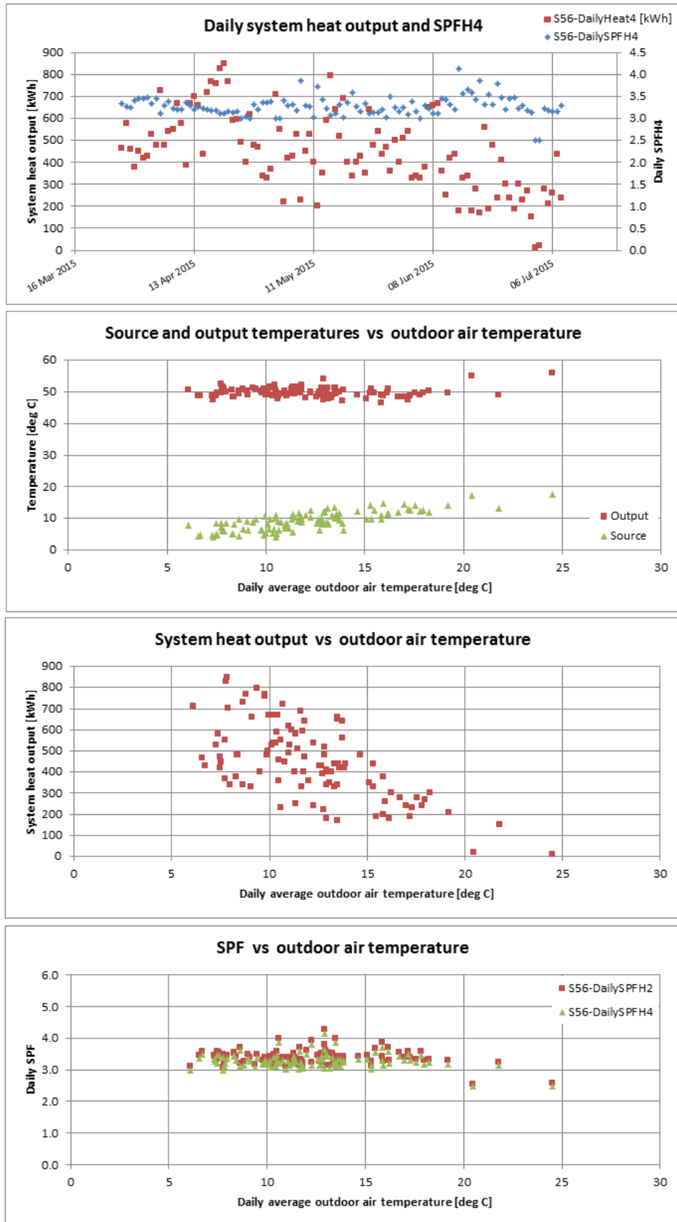
Figure T 75 – Site 56 system efficiency charts (1)
