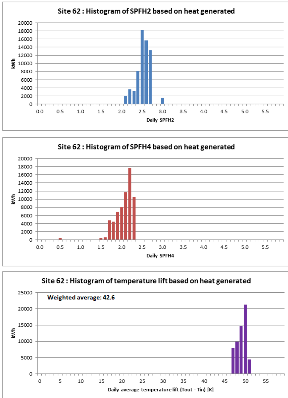
Figure T 168 – Site 62 histograms of SPF H2 , SPF H4 and temperature lift
