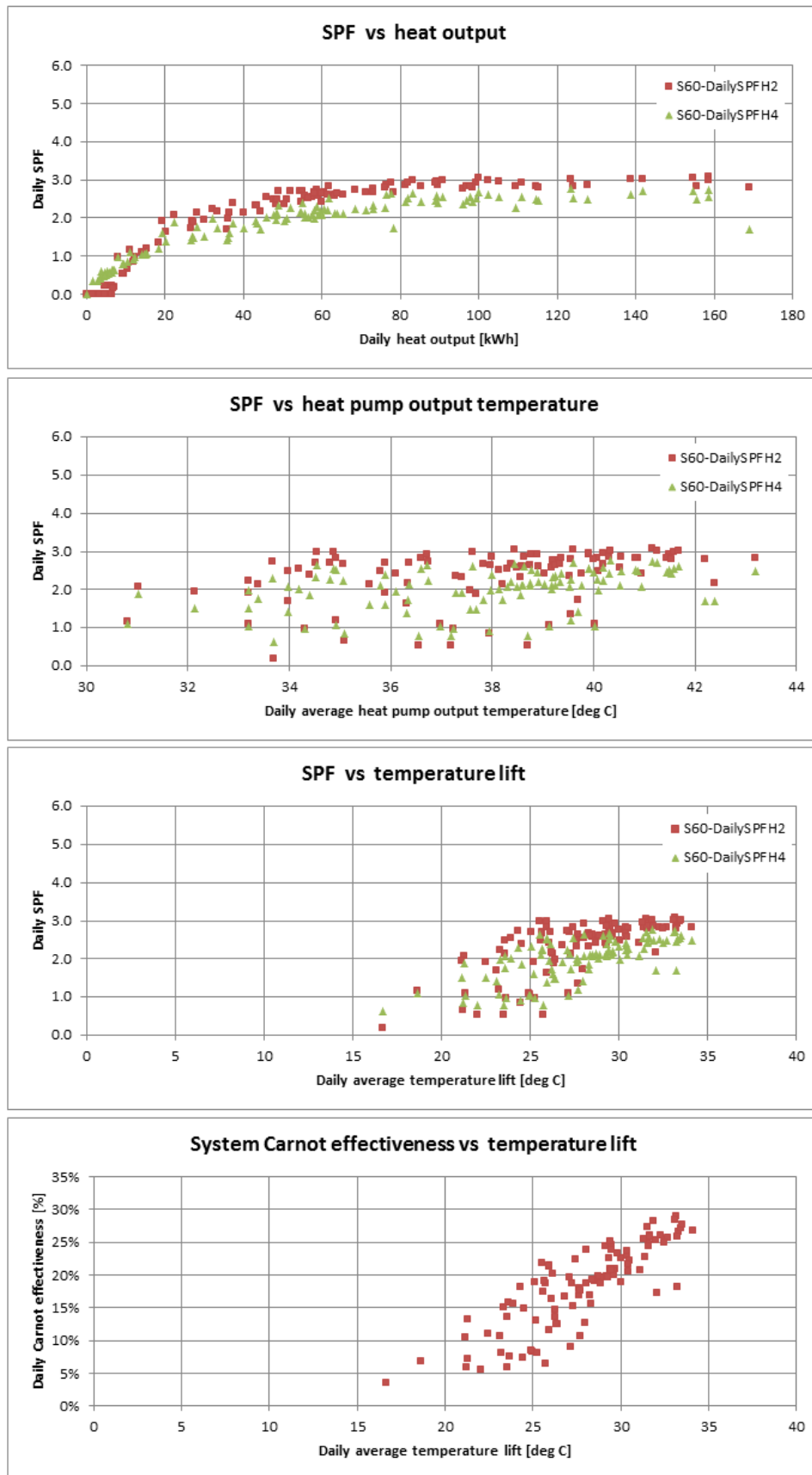
Figure T 80 – Site 60 system efficiency charts (2)
