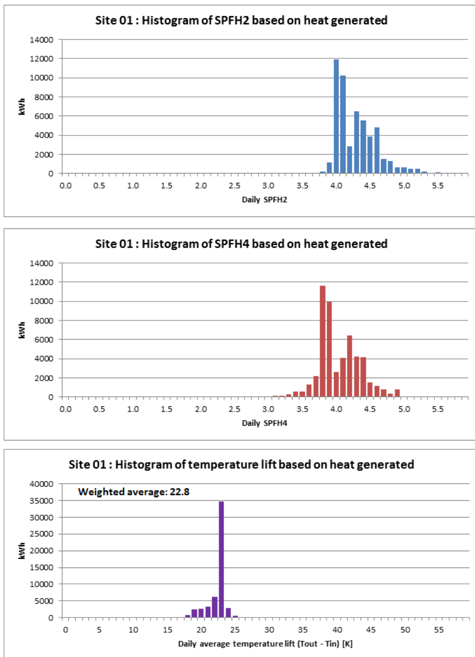
Figure T 141 – Site 01 histograms of SPF H2 , SPF H4 and temperature lift
