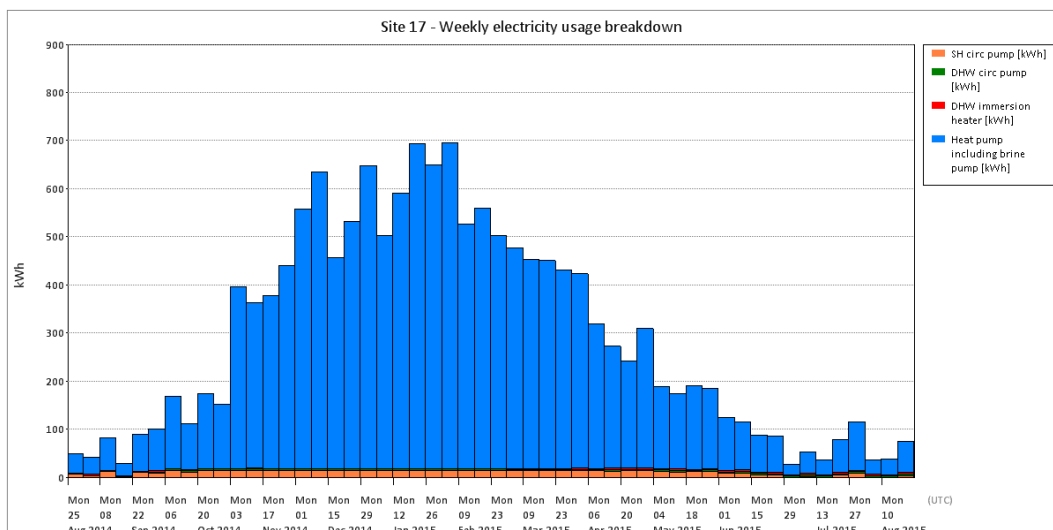
Figure T 176 – Site 17 electricity breakdown
