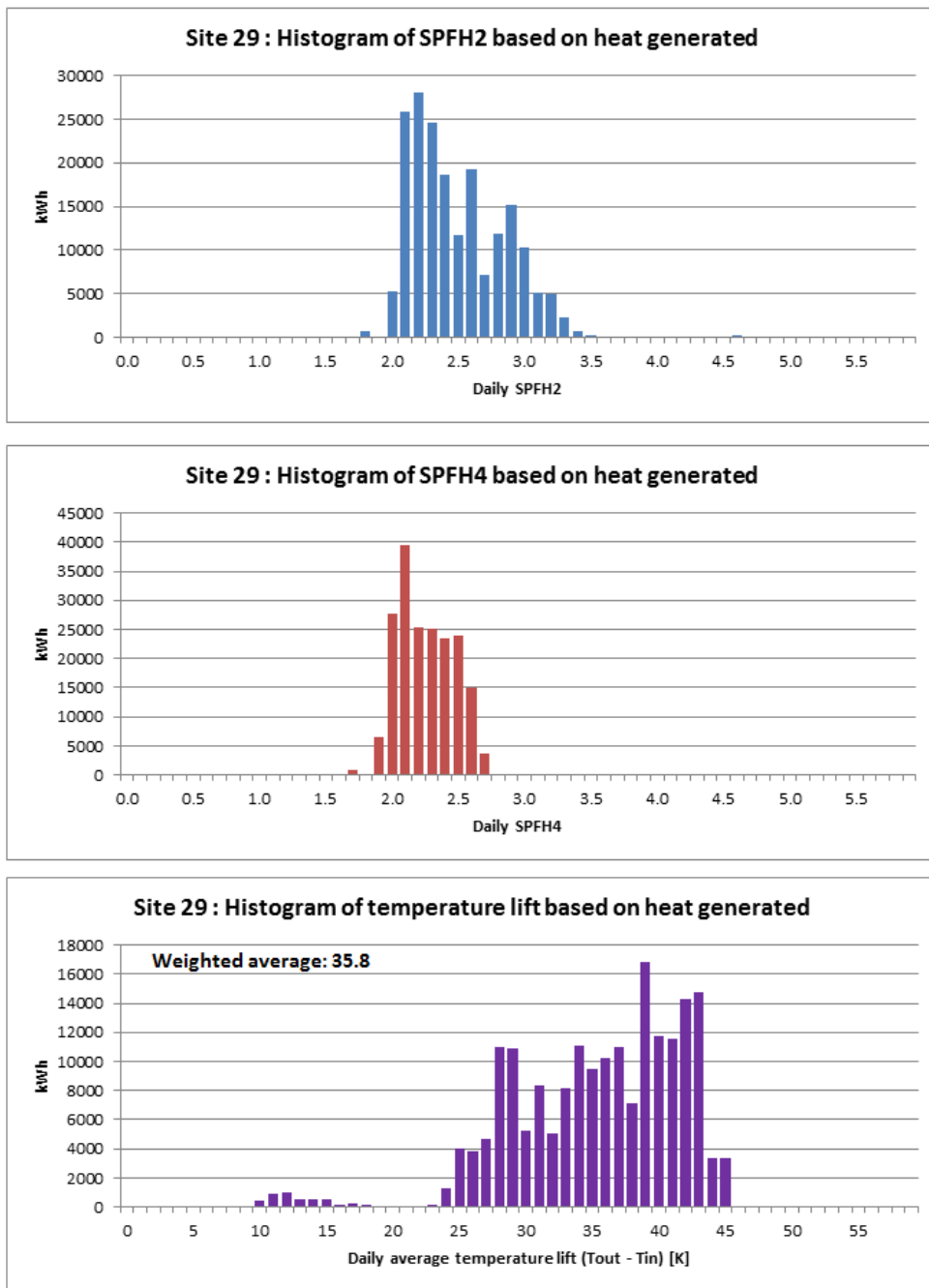
Figure T 153 – Site 29 histograms of SPF H2 , SPF H4 and temperature lift
