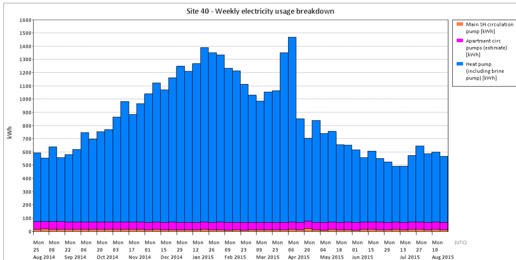
Figure T 184 – Site 40 electricity breakdown
