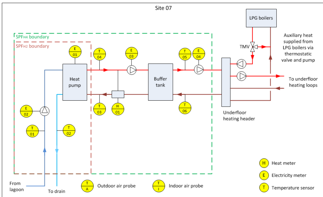
Figure T 5 – Site 07 system schematic
