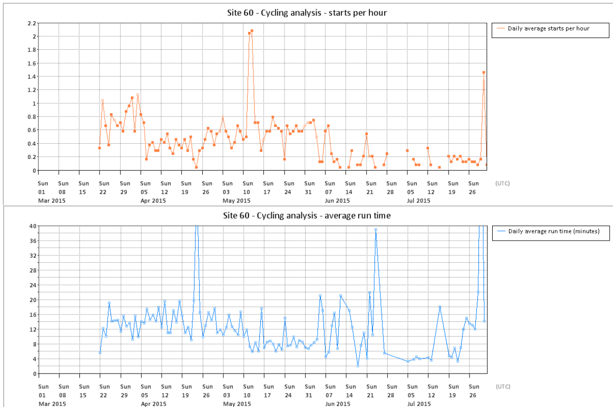
Figure T 138 – Site 60 cycling analysis
