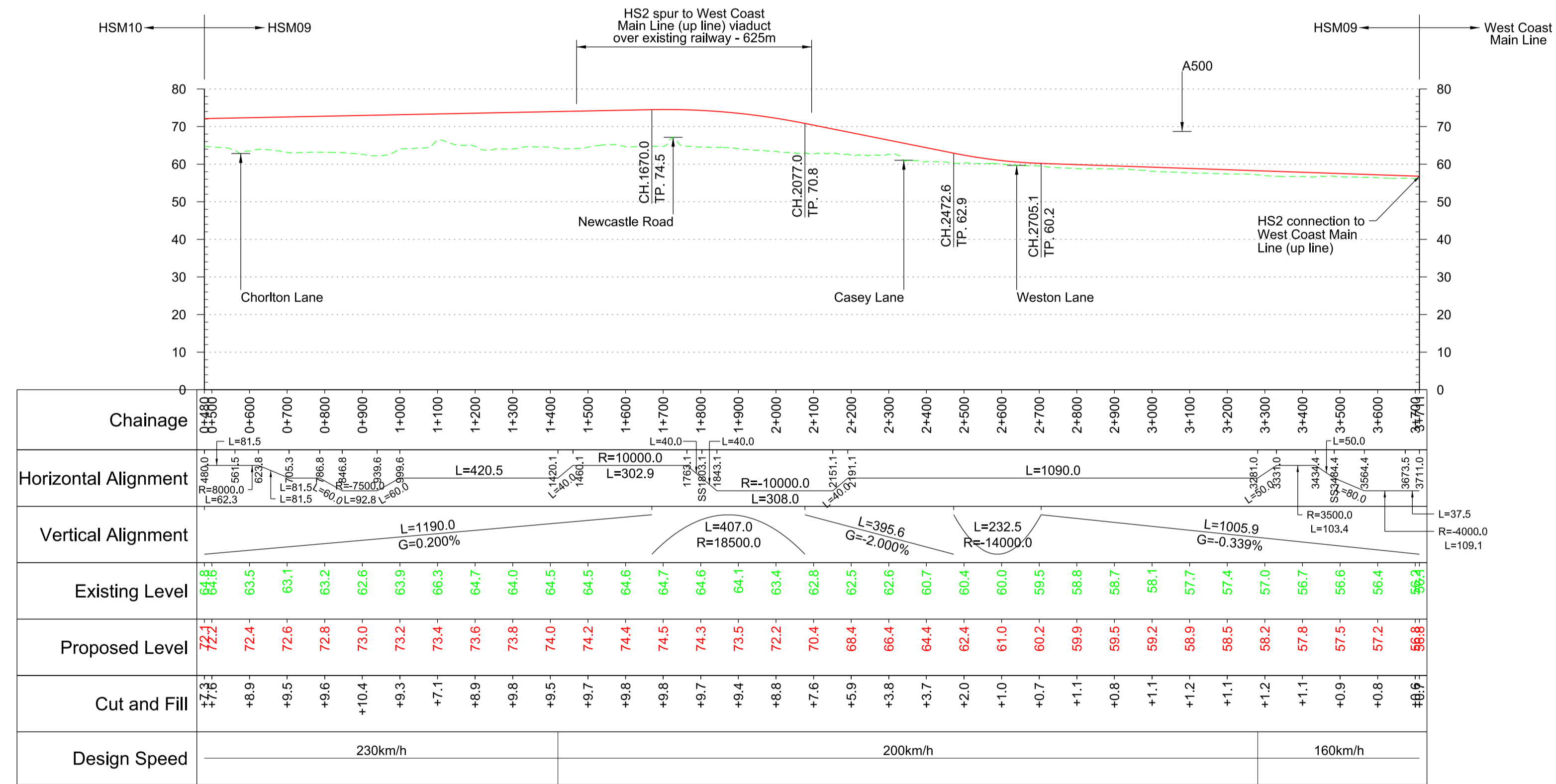
Profile - Up Line Scale H:1:10,000 V:1:1000 @ A1
