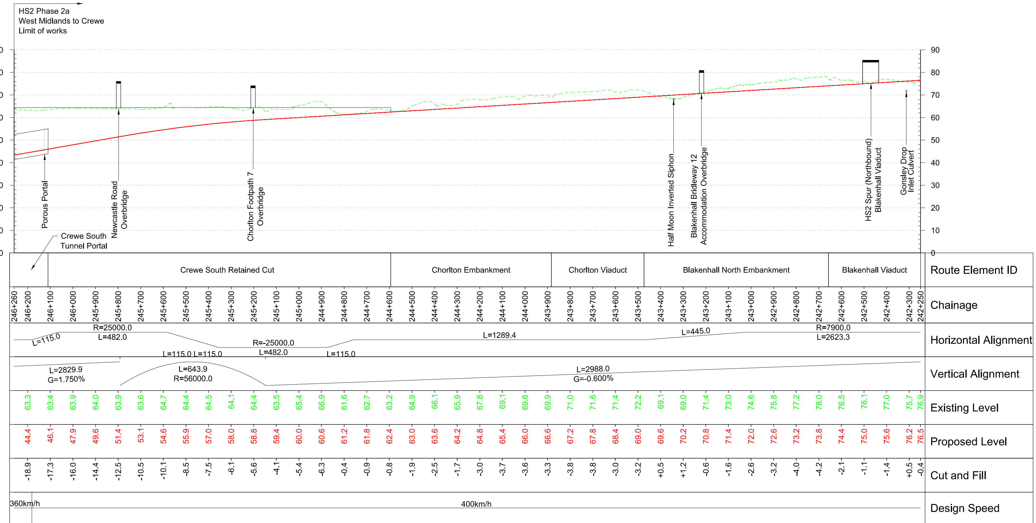
Profile Scale H:1:10,000 V:1:1000 @ A1
