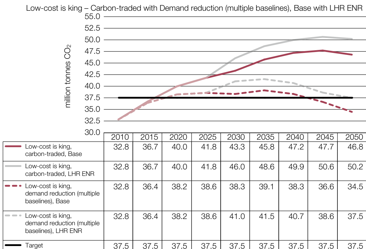
Figure 7.8: Heathrow Extended Northern Runway demand reduction test, low-cost is king, CO 2 emissions 2010-2050
