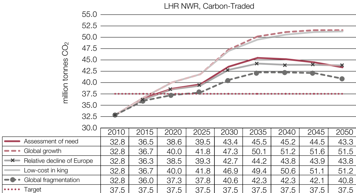
Figure 6.8: Heathrow Airport Northwest Runway option national UK departing flight CO 2 emissions
