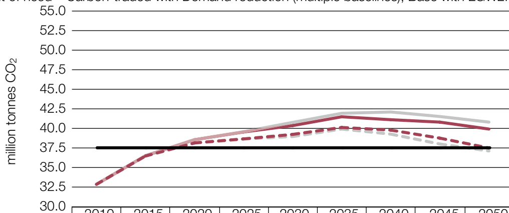
Figure 7.3: Gatwick Airport Second Runway demand reduction test, assessment of need, CO 2 emissions 2010-2050
