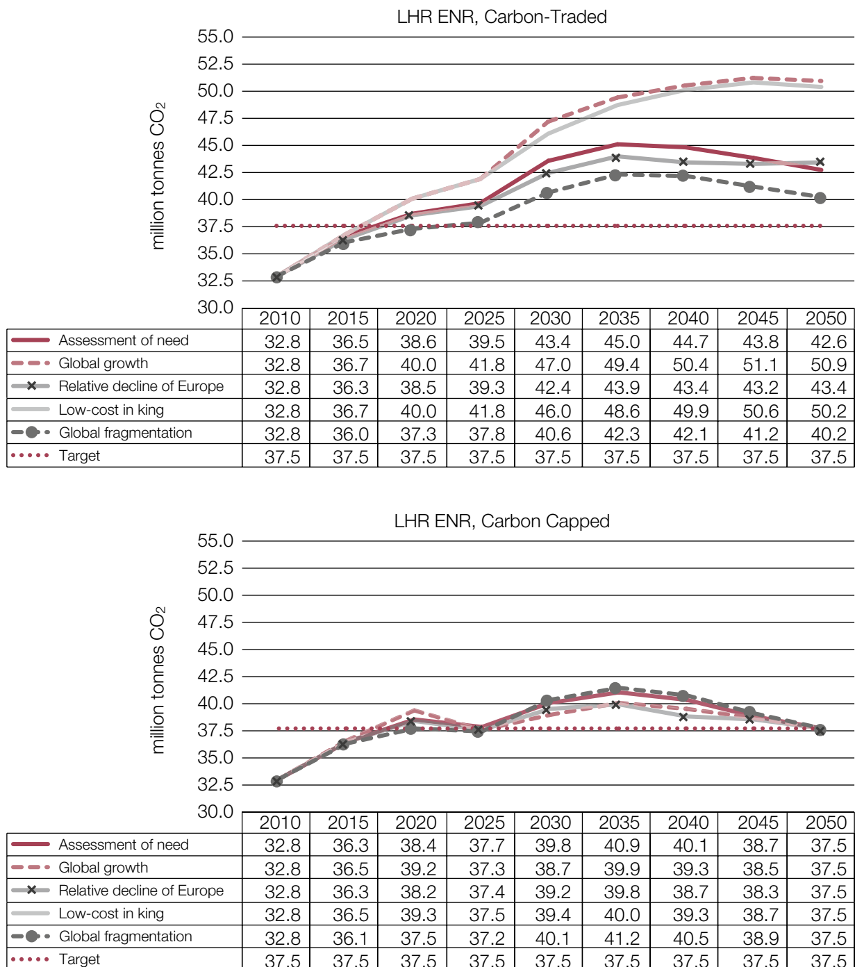
Figure 6.9: Heathrow Airport Extended Northern Runway option national UK departing flight CO 2 emissions
