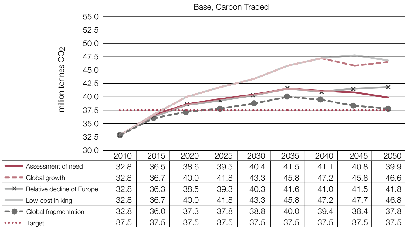
Figure 4.2: Departing UK CO 2 forecasts without a carbon cap
