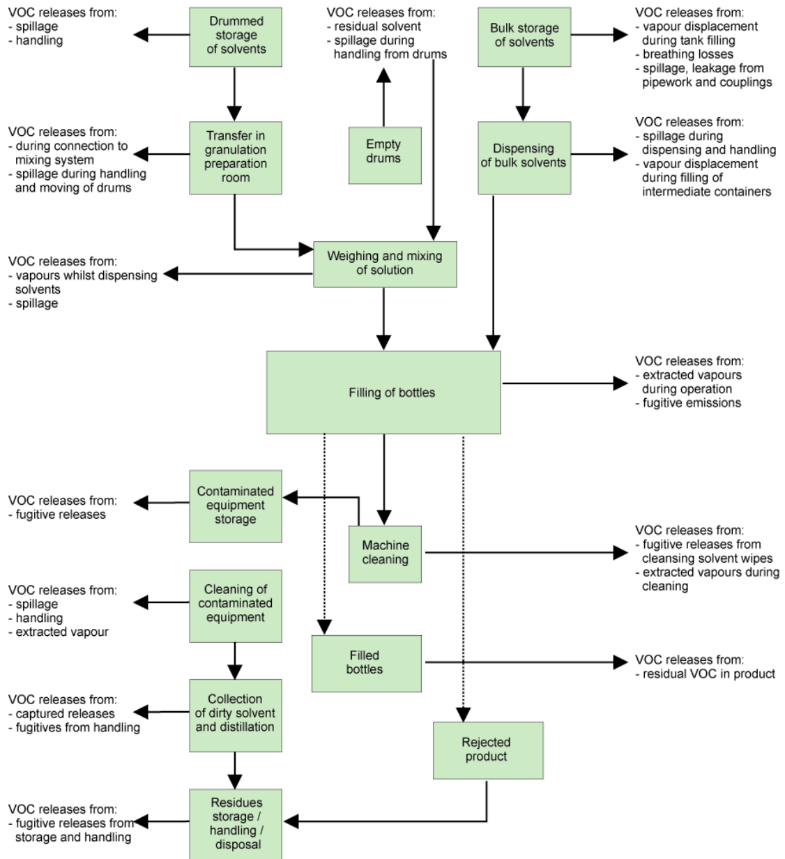
Figure 3.2 - VOC releases from a typical aerosol manufacturing process
