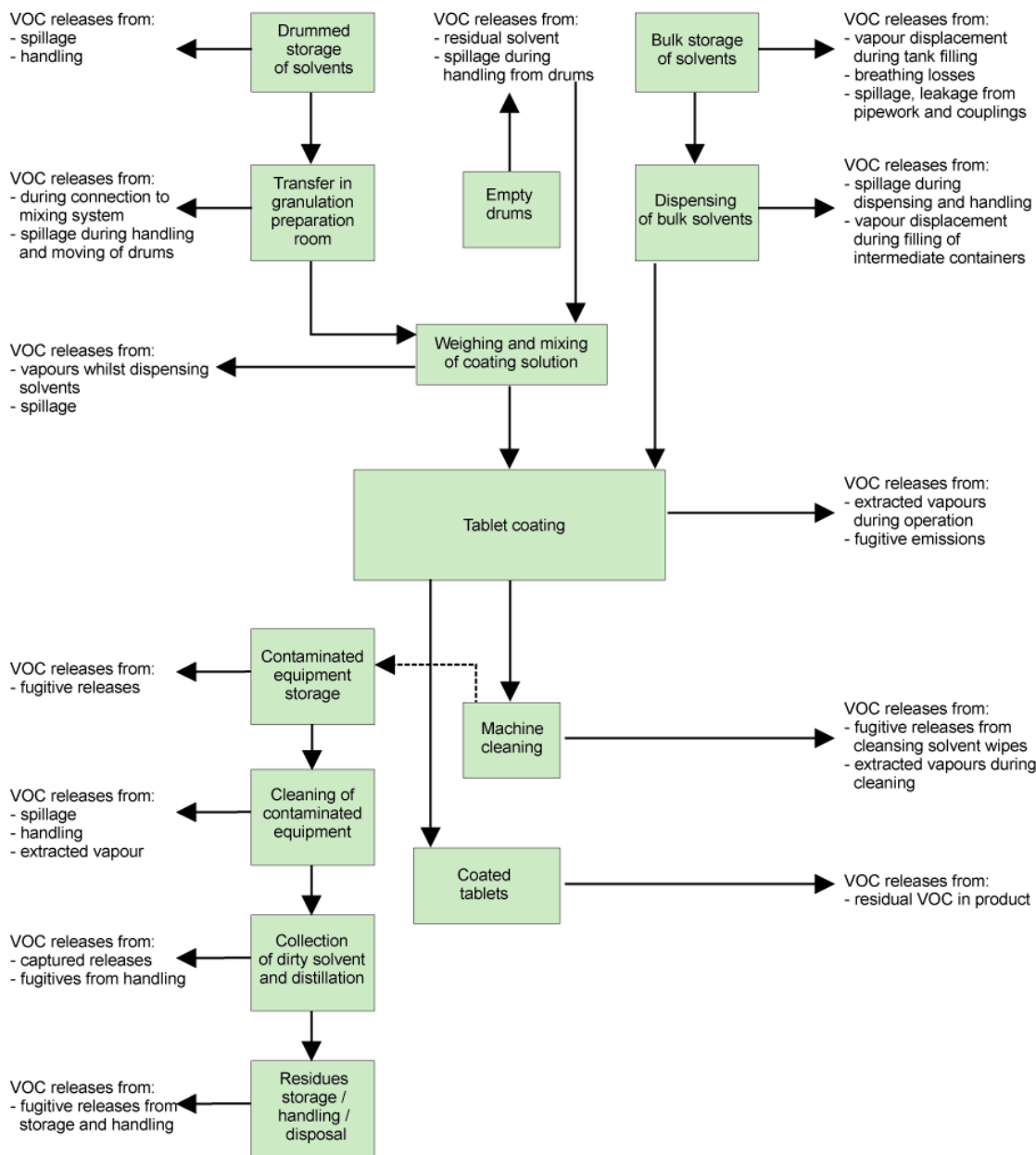
Figure 3.4 - VOC releases from a typical tablet manufacturing process
