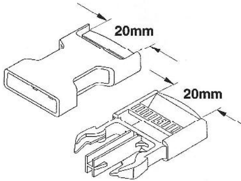
SR 20 NSN 8315-99-738-8560
