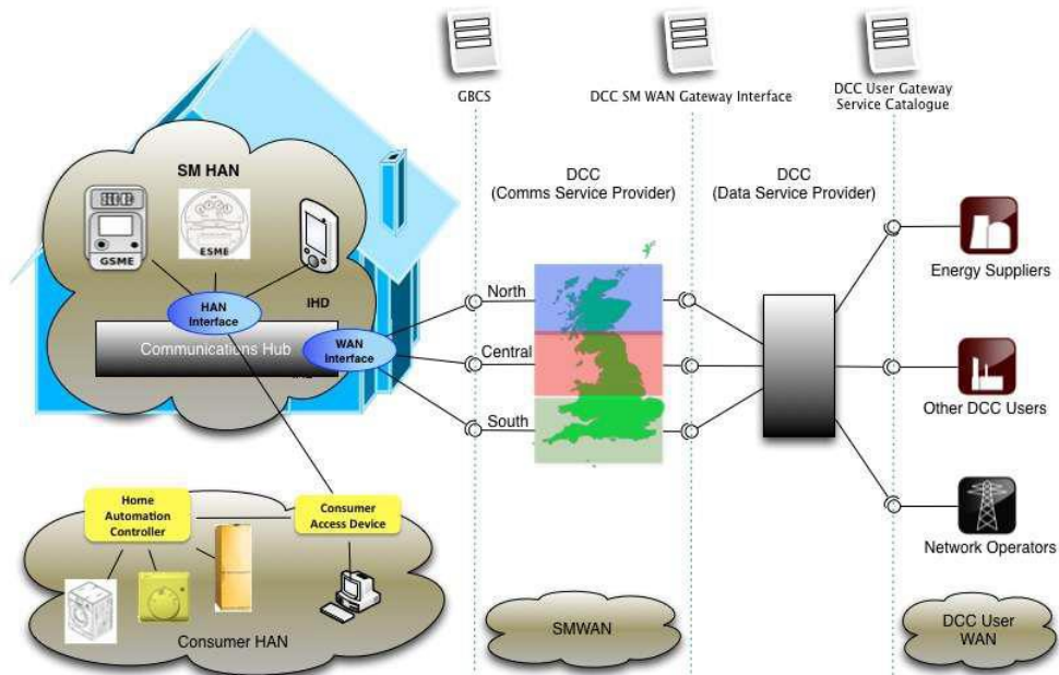
Figure 44. Smart meter communications infrastructure
