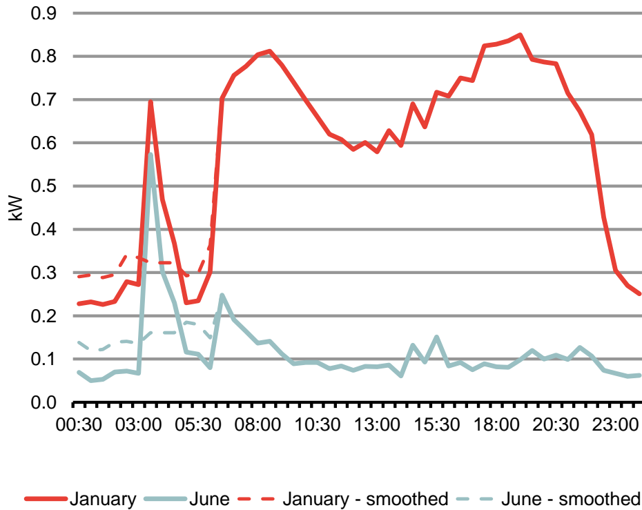
Figure 31. Heat pump profiles from CLNR project
