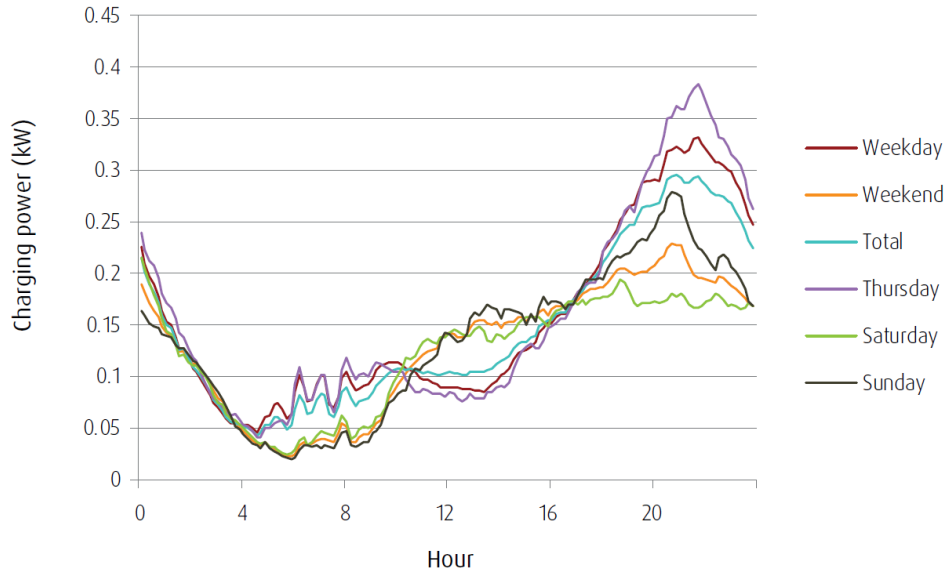
Figure 34. Average charging profiles per EV for different days of the week - residential
