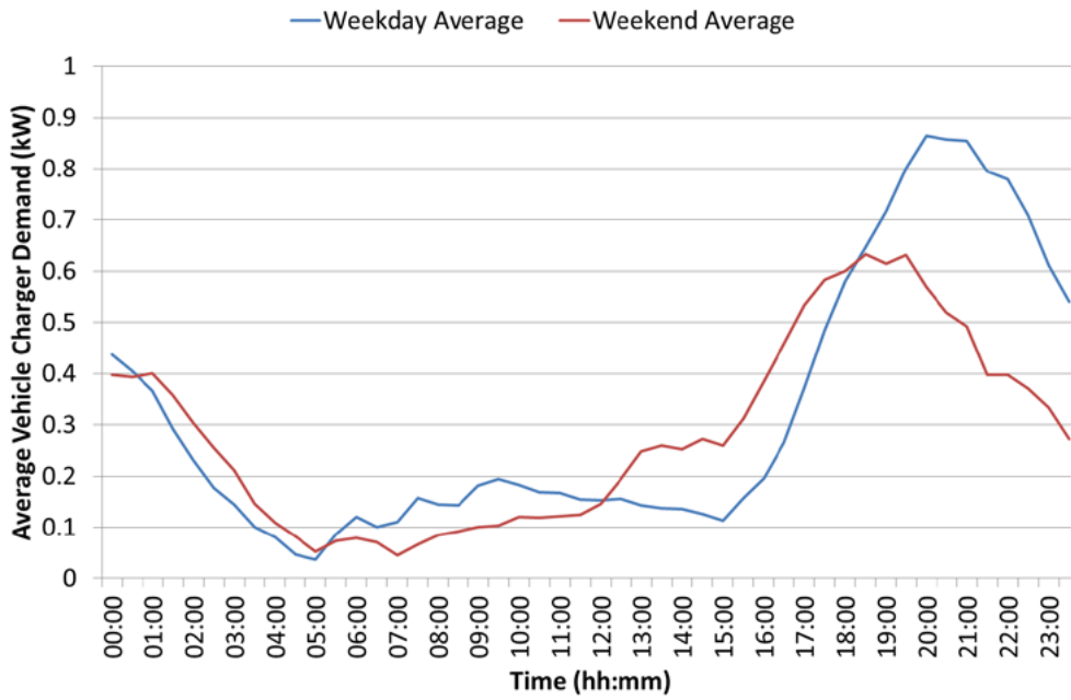
Figure 37. February 2014 EV Charger Weekday and Weekend Average Diurnal Profile
