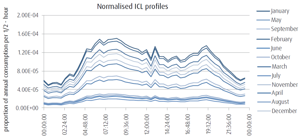
Figure 32. Normalised heat pump profiles
