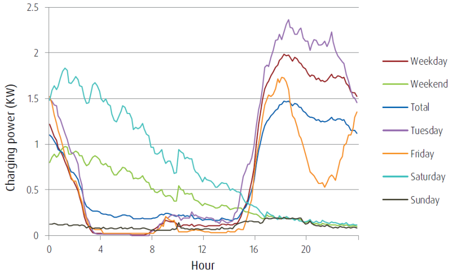
Figure 36. Average charging profiles per user among the 3-phase commercial participants (delivery vans) for different days of the week
