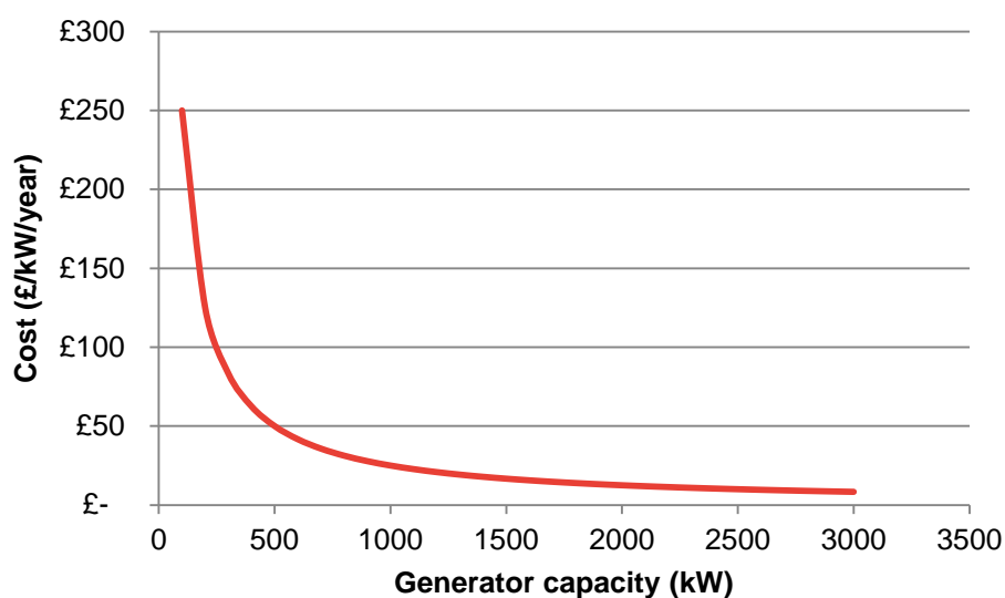
Figure 15. Illustrative set-up costs per kW per year for diesel back-up generation
