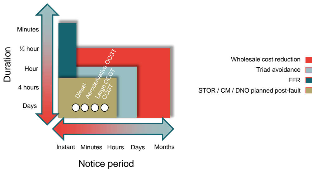
Figure 8. Illustrative DSR capabilities of distributed thermal generation, based on time to full power from a warm start
