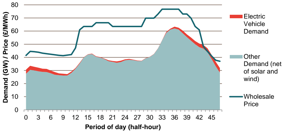
Figure 49. Load profile for electric vehicles, residual demand and wholesale price
