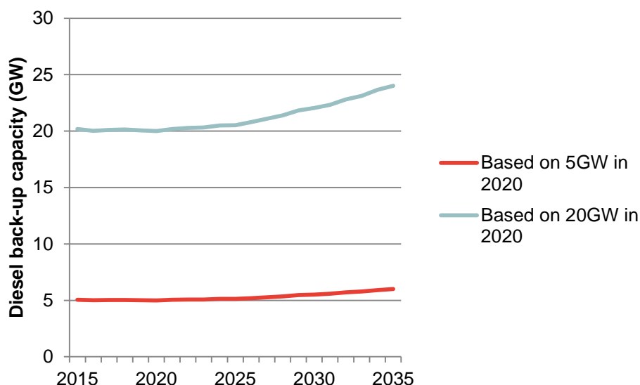
Figure 14. Potential capacity of diesel back-up generation
