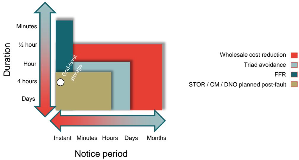
Figure 47. Illustrative DSR capabilities of grid-level storage
