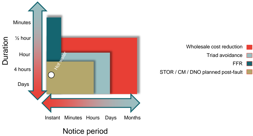
Figure 18. Illustrative DSR capabilities of immersion heaters with storage
