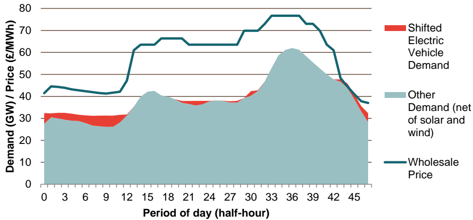
Figure 50. Shifted load profile for electric vehicles, residual demand and wholesale price
