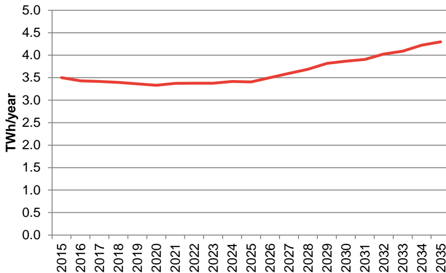
Figure 19. Indicative yearly energy usage for commercial hot water
