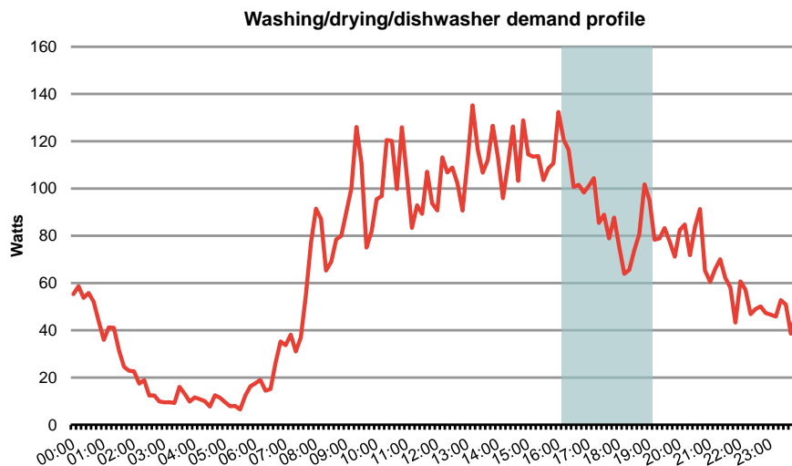
Figure 40. Domestic wet goods load profile
