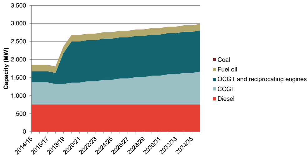
Figure 4. National Grid "Gone Green" projection for distributed thermal capacity
