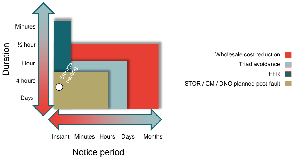
Figure 26. Illustrative DSR capabilities of domestic electric storage heating
