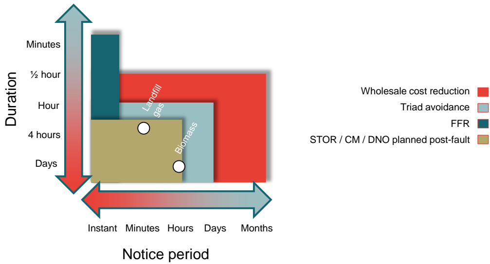
Figure 10. Illustrative DSR capabilities of distributed renewable generation
