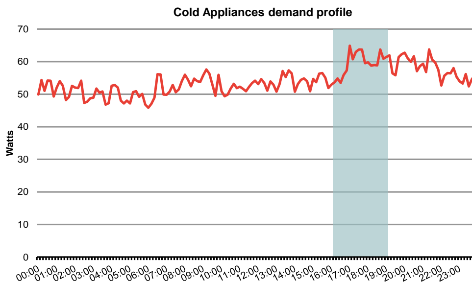
Figure 42. Domestic cold goods load profile
