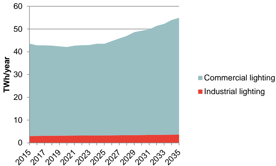
Figure 23. Indicative yearly energy usage for I&C lighting
