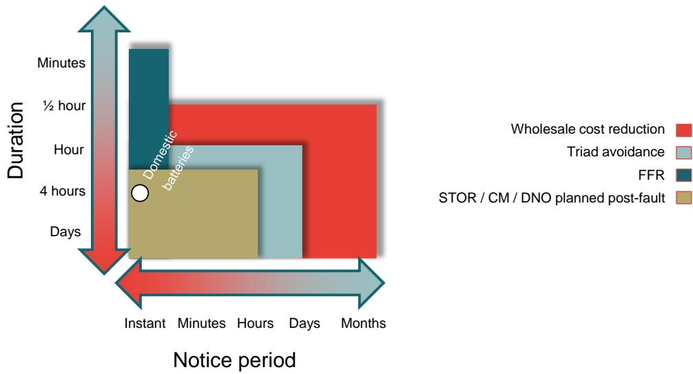
Figure 43. Illustrative DSR capabilities of domestic batteries
