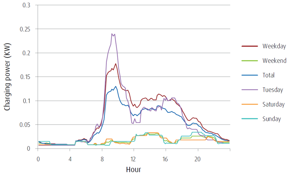
Figure 35. Average charging profiles per EV for single-phase commercial vehicles for different days of the week
