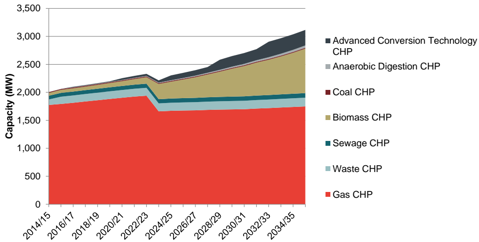
Figure 11. National Grid "Gone Green" projection for distributed CHP capacity
