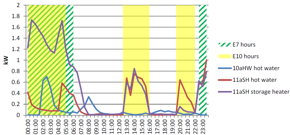
Figure 28. Electric resistive space heating load profile
