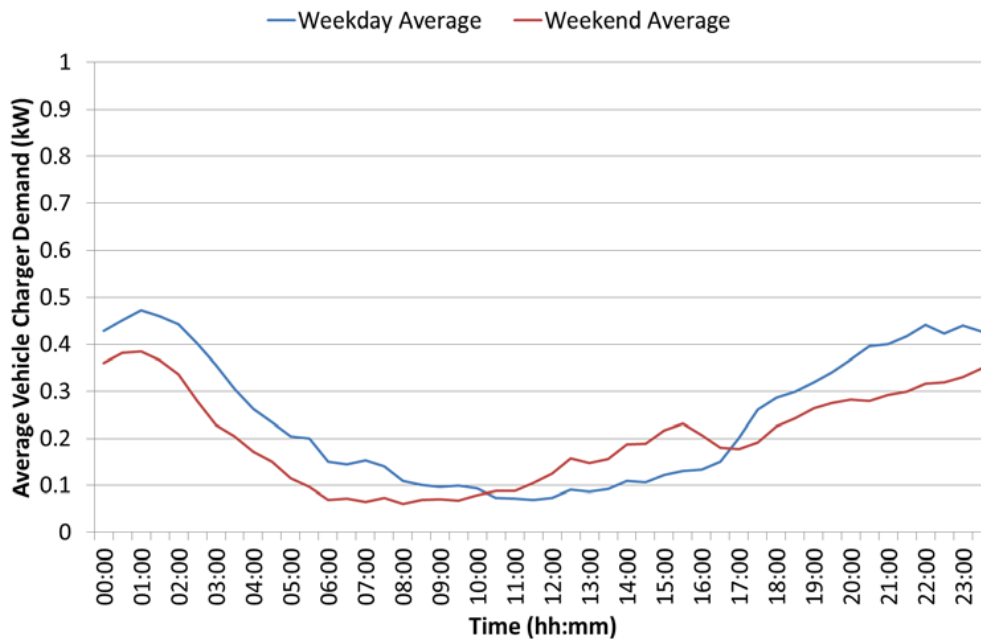
Figure 38. June 2014 EV Charger Weekday and Weekend Average Diurnal Profile
