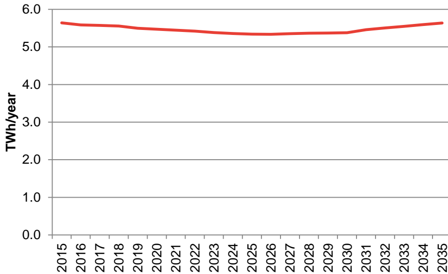
Figure 21. Indicative yearly energy usage for industrial refrigeration
