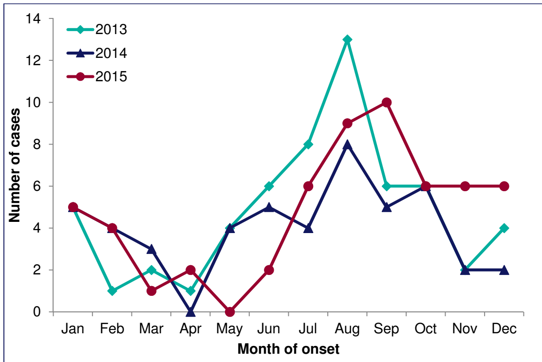
Figure 3: Number of confirmed Legionnaires' disease cases in residents of London by month and year of onset 2013 to 2015
