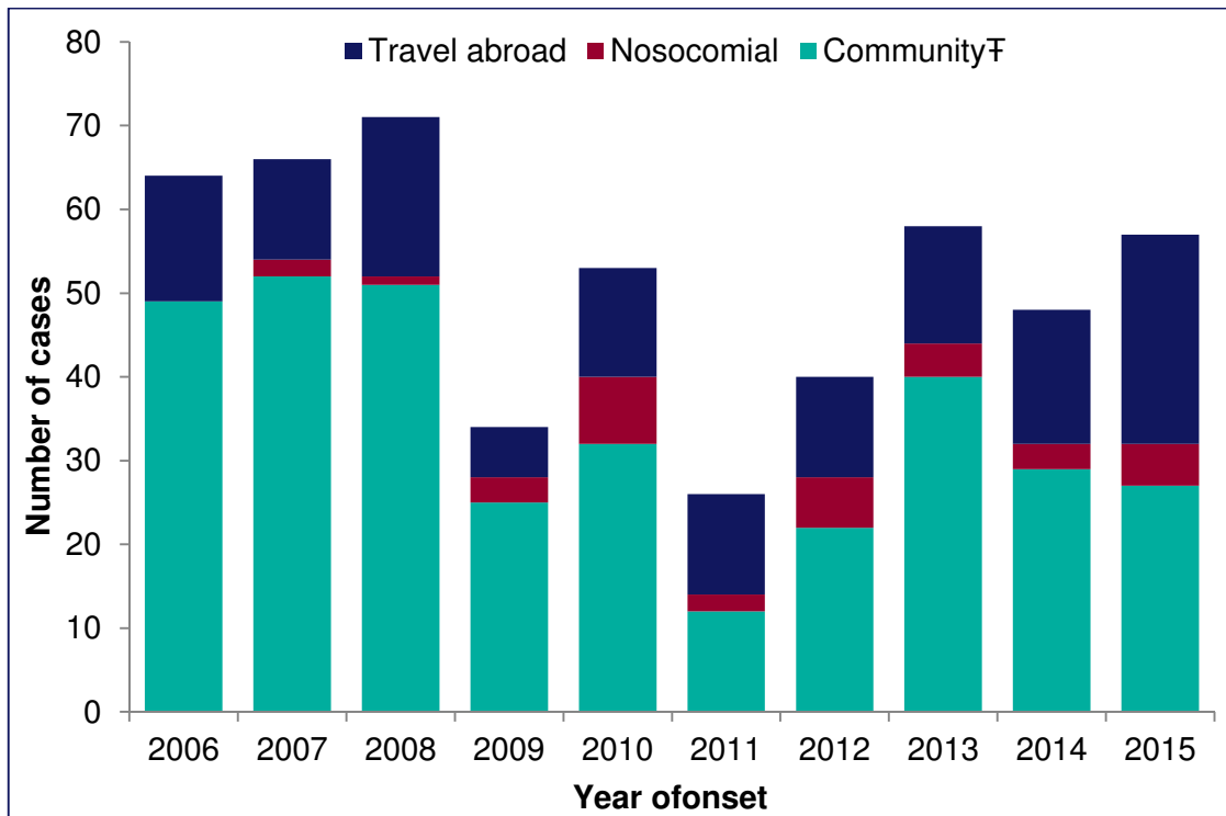
Figure 2: Number of confirmed Legionnaires' disease cases o in residents of London by year of onset and category 2006 to 2015
