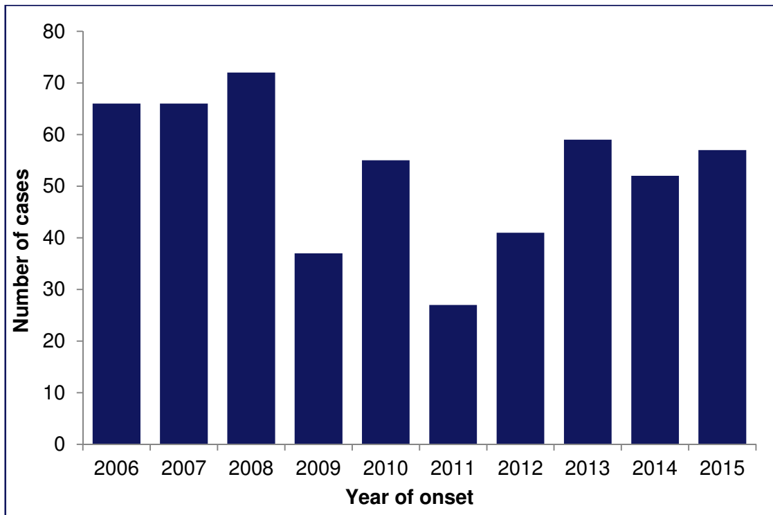
Figure 1: Number of cases of legionellosis (confirmed and presumptive) in residents of London by year of onset of symptoms 2006 to 2015
