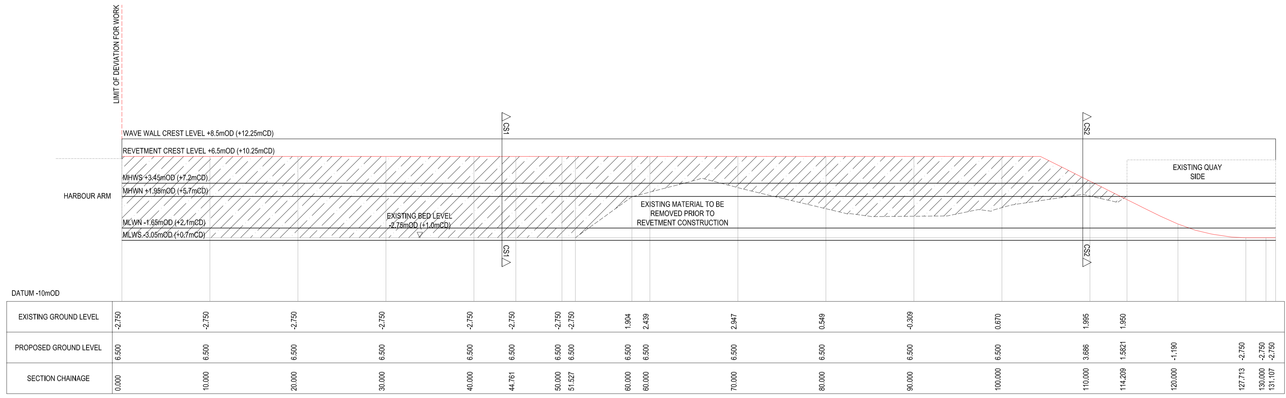
LONG SECTION LS1 - WAVE WALL HORIZONTAL SCALE 1:250 VERTICAL SCALE 1:250
