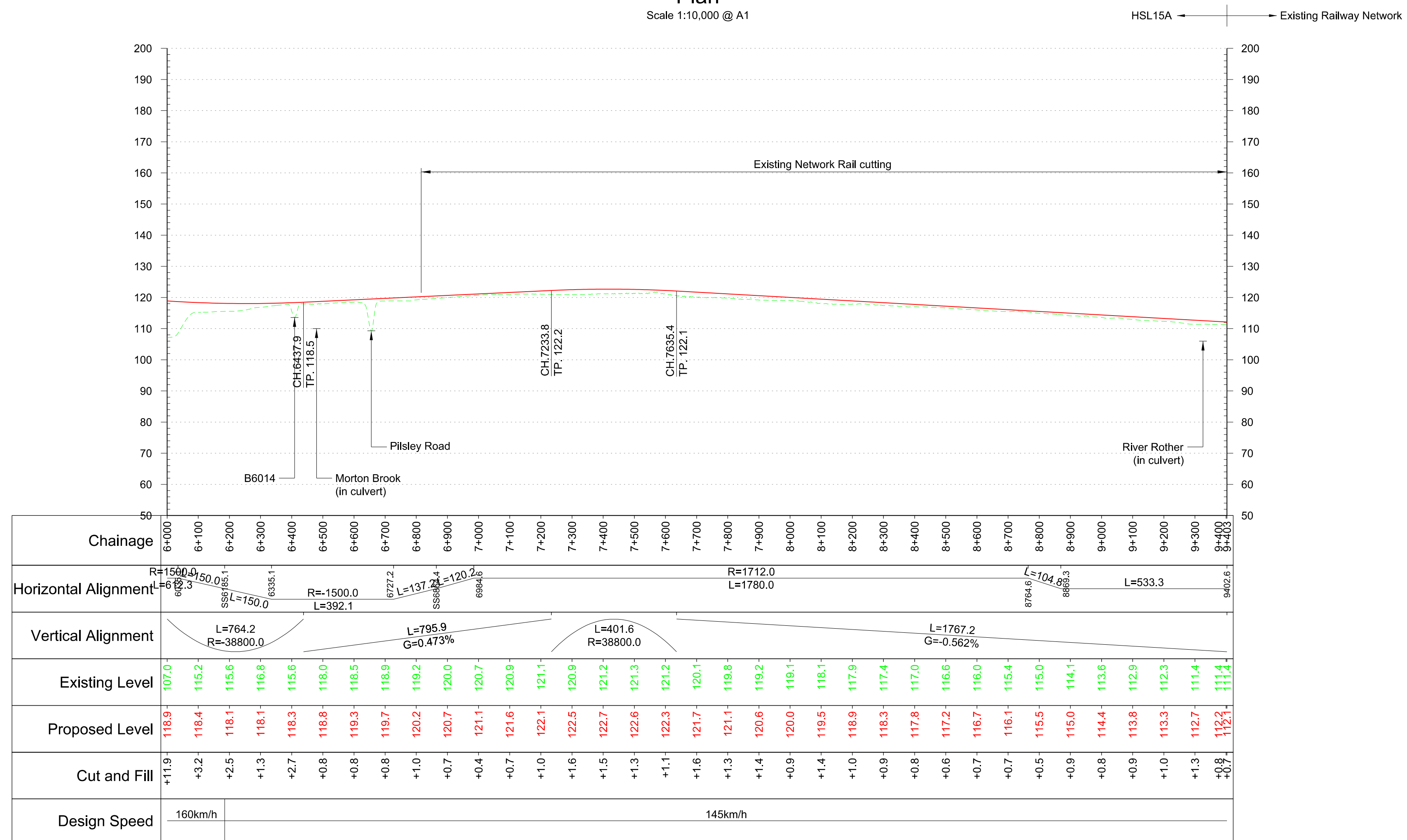
Profile Scale H:1:10,000 V:1:1000 @ A1
