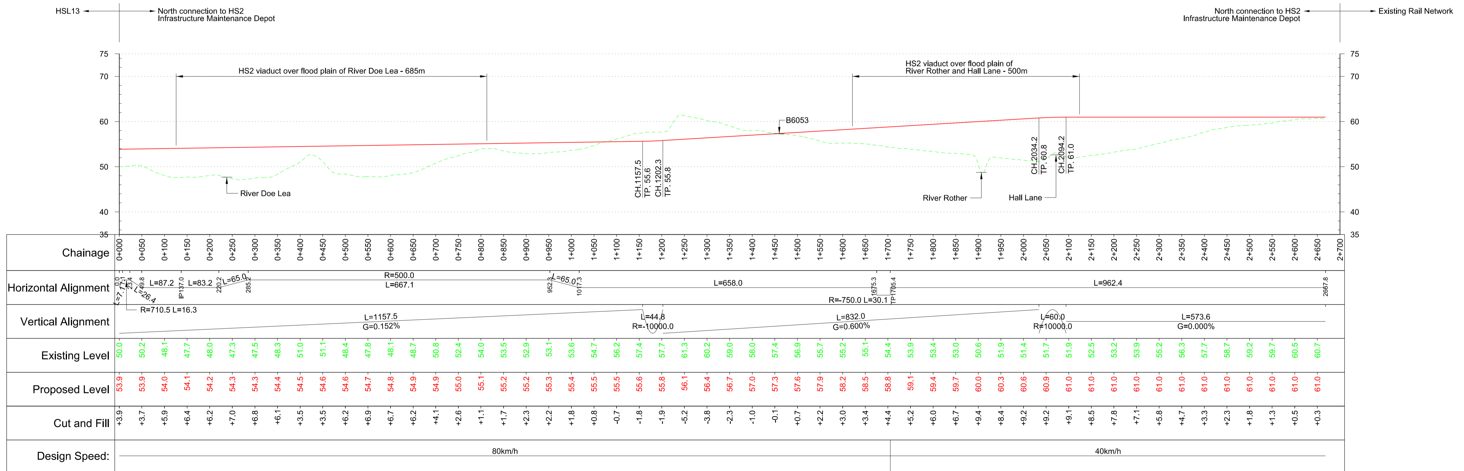
Profile Scale H:1:5,000 V:1:500 @ A1
