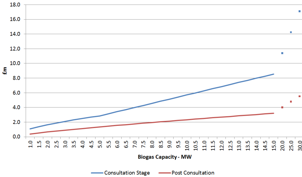
Chart E – Anaerobic Digester Capex
