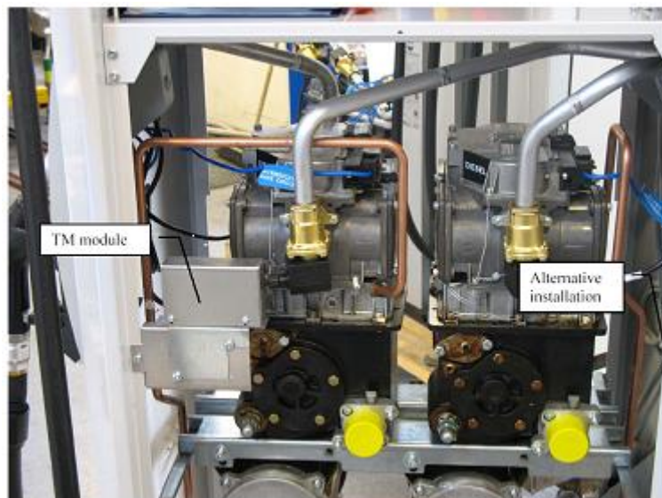
Figure 32 Wayne ATC – Global Century Installation
