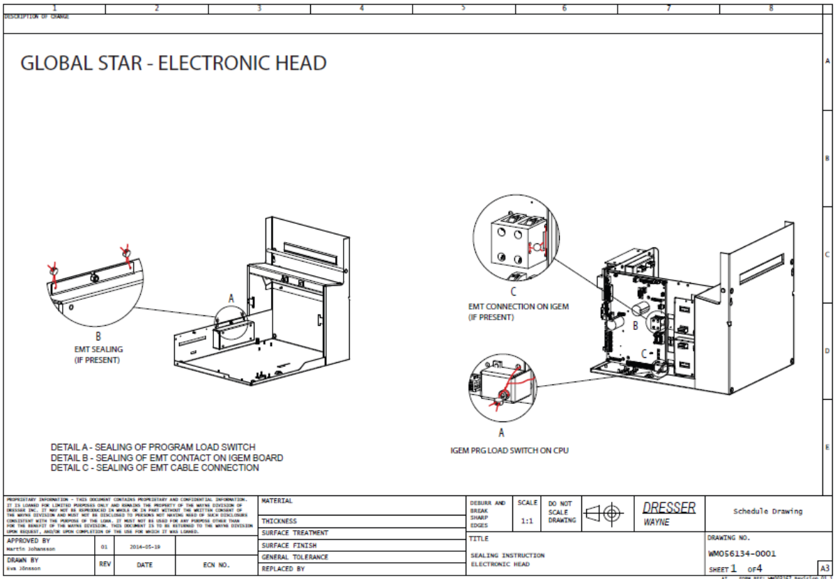
Figure 41 Alternative sealing electronic head
