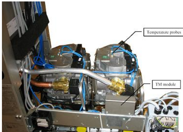
Figure 31 Wayne ATC – Global Star Installation
