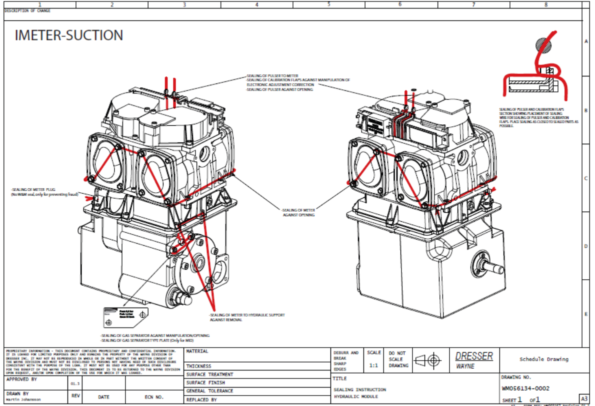
Figure 42 Alternative sealing electronics
