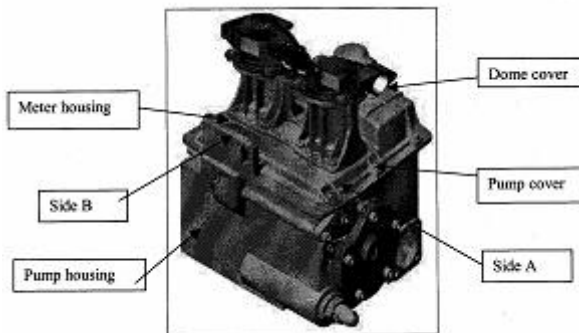
Figure 21 X-Flo Suction Unit
