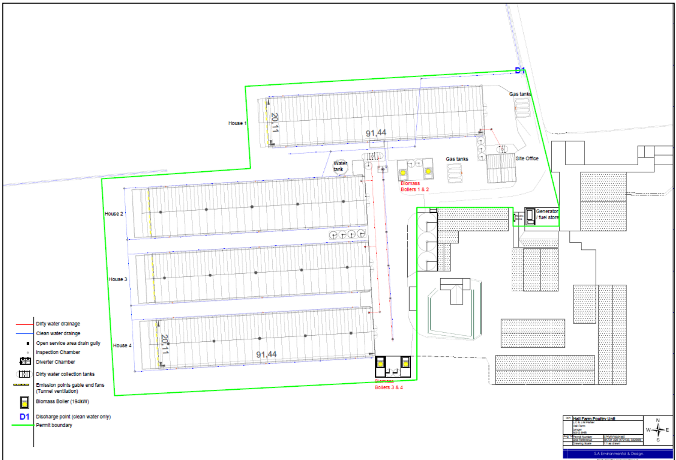
Installation boundary plan
