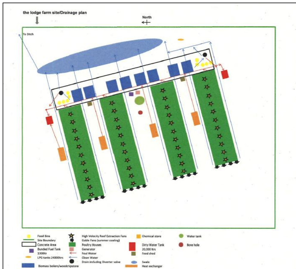
Installation boundary plan
